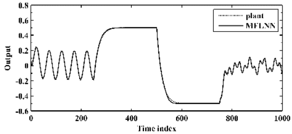
Figure 3.8. Outputs of the plant and the MFLNN for the first data set
