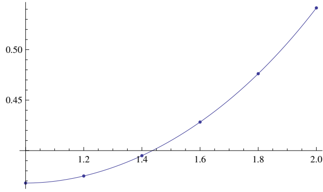
Figure 5.20: Graphs of ordinary Runge Kutta Method and the exact function for n = 5
