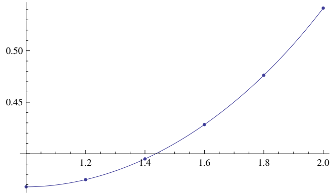
Figure 5.14: Graphs of ordinary Runge Kutta Method and the exact function for n = 5
