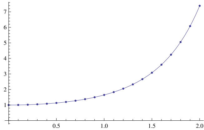
Figure 5.3: Graphs of multiplicative Runge Kutta Method and the exact function for n = 20
