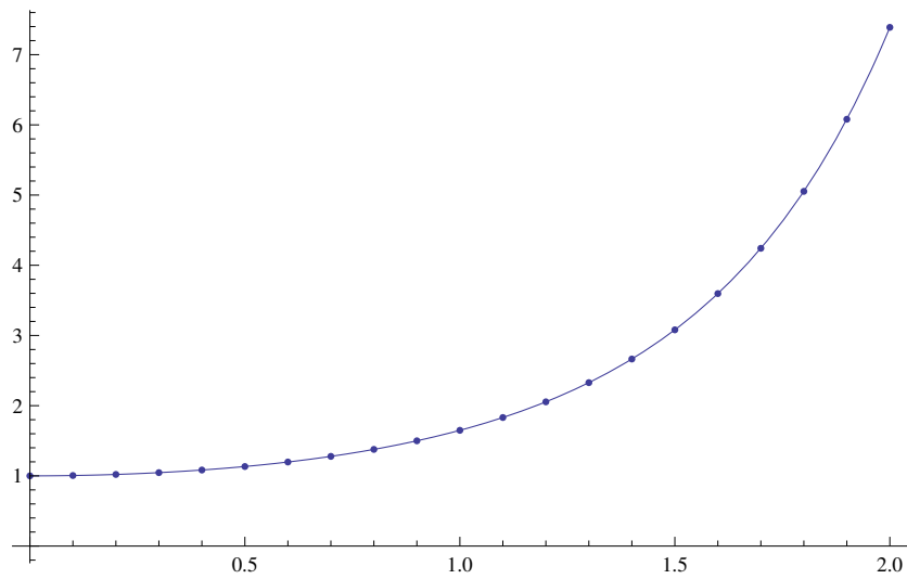
Figure 5.9: Graphs of multiplicative Runge Kutta Method and the exact function for n = 20
