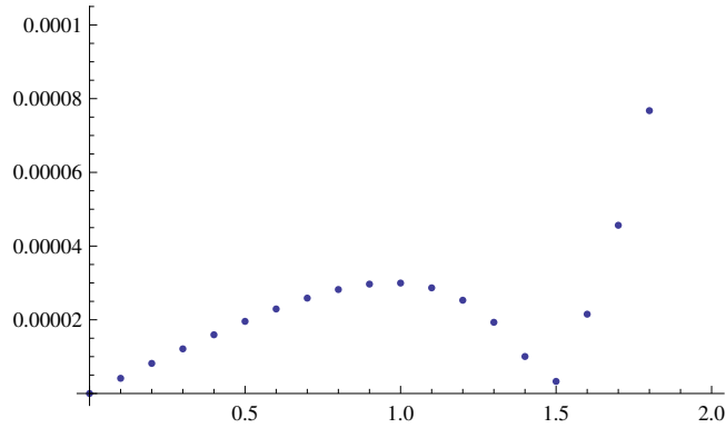
Figure 5.6: Error of Ordinary Runge Kutta Method for the ordinary Differential Equation y' = y \cdot x for n = 20
