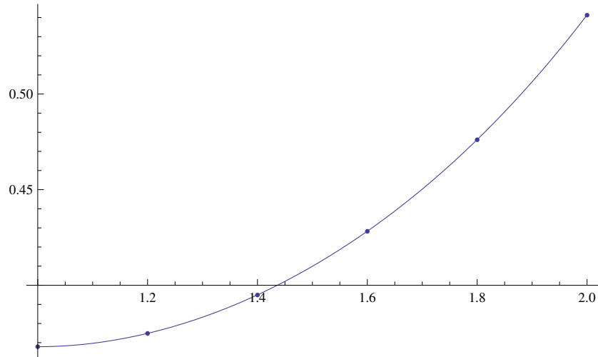
Figure 5.19: Graphs of multiplicative Runge Kutta Method and the exact function for n = 5
