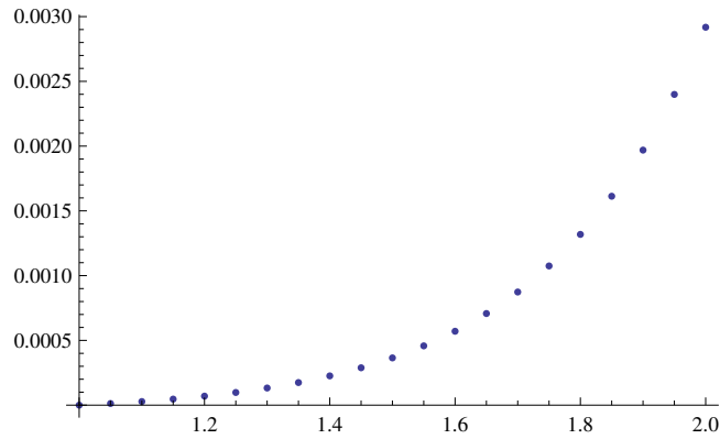
Figure 5.30: Error of Ordinary Runge Kutta Method for the ordinary Differential Equation y' = y \cdot e^x for n = 20
