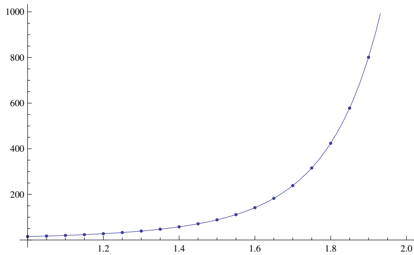
Figure 5.33: Graphs of multiplicative Runge Kutta Method and the exact function for n = 20
