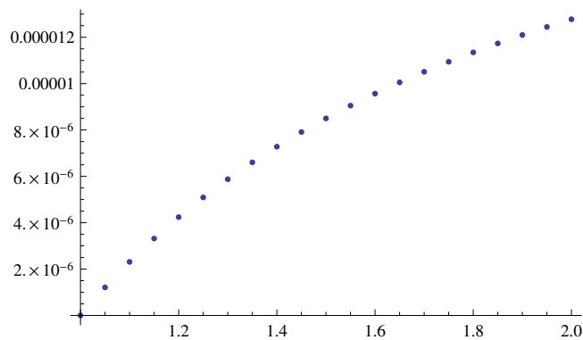
Figure 5.23: Error of Multiplicative Runge Kutta Method for the multiplicative Differential Equation y^* = x for n = 20
