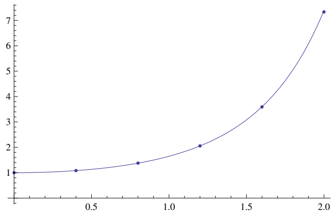
Figure 5.2: Graphs of Ordinary Runge Kutta Method and the exact function for n = 5
