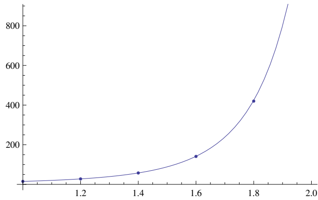
Figure 5.32: Graphs of ordinary Runge Kutta Method and the exact function for n = 5
