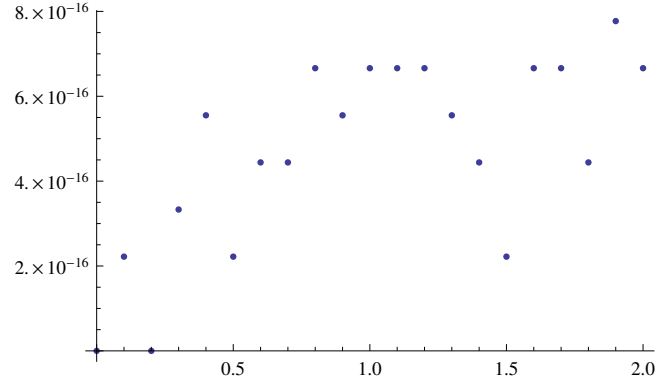
Figure 5.11: Error of Multiplicative Runge Kutta Method for the multiplicative Differential Equation y^* = e^x for n = 20
