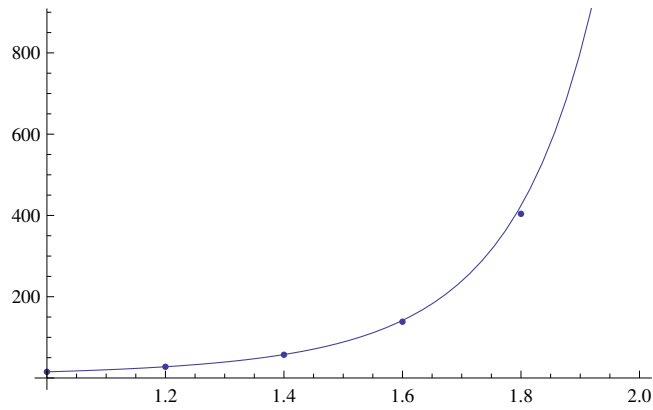
Figure 5.26: Graphs of ordinary Runge Kutta Method and the exact function for n = 5
