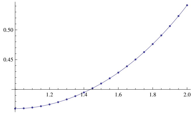
Figure 5.16: Graphs of ordinary Runge Kutta Method and the exact function for n = 20
