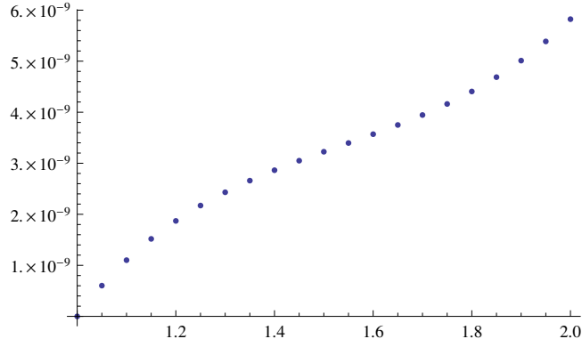
Figure 5.24: Error of Ordinary Runge Kutta Method for the ordinary Differential Equation y' = y \cdot \ln x for n = 20
