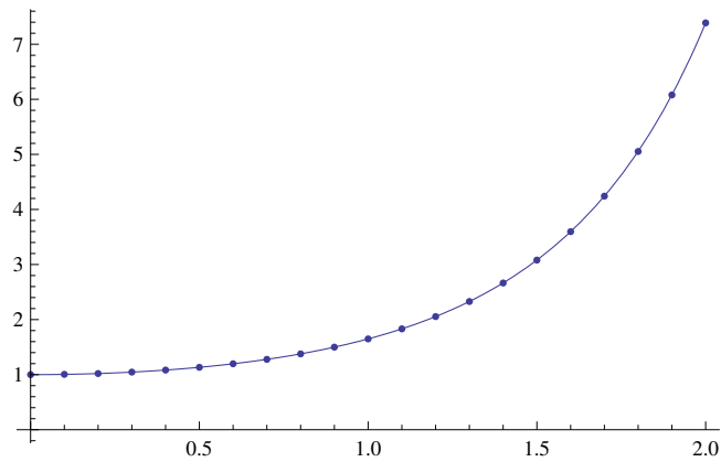
Figure 5.4: Graphs of Ordinary Runge Kutta Method and the exact function for n = 20
