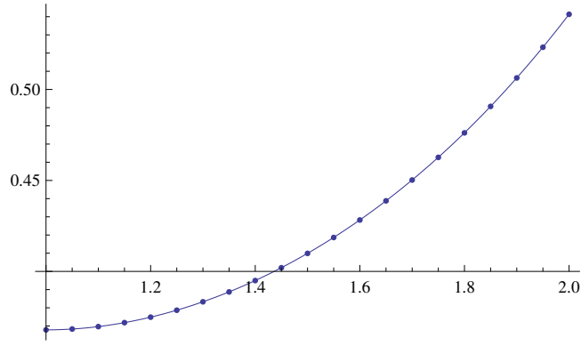
Figure 5.15: Graphs of multiplicative Runge Kutta Method and the exact function for n = 20
