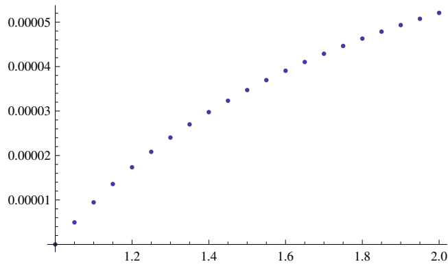
Figure 5.17: Error of Multiplicative Runge Kutta Method for the multiplicative Differential Equation y^* = x for n = 20
