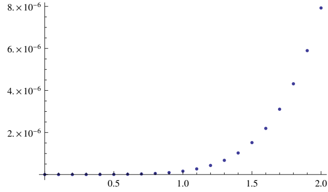
Figure 5.12: Error of Ordinary Runge Kutta Method for the ordinary Differential Equation y' = y \cdot x for n = 20
