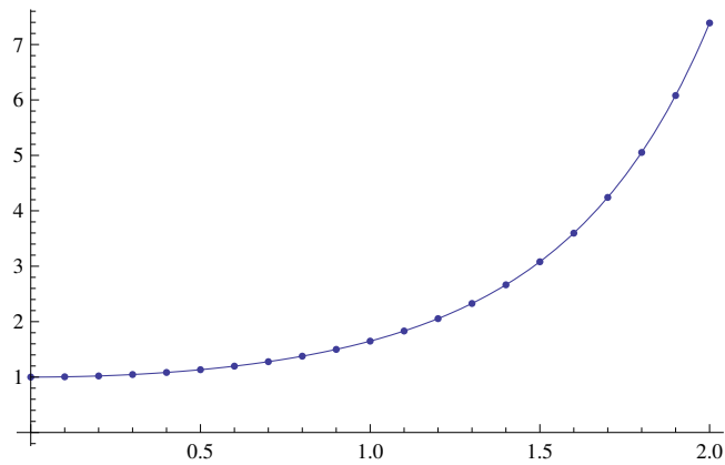
Figure 5.10: Graphs of Ordinary Runge Kutta Method and the exact function for n = 20
