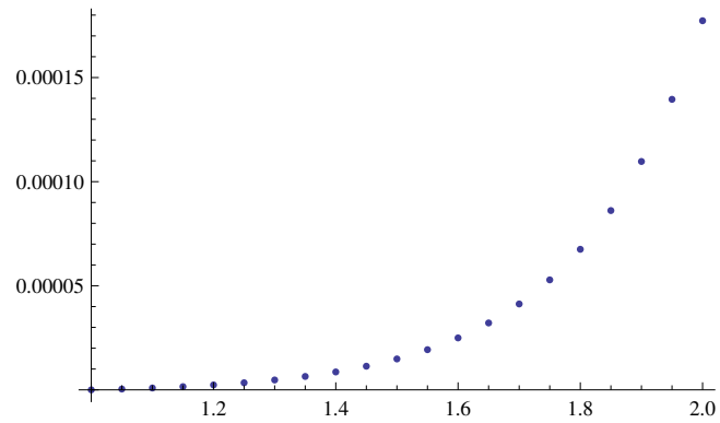
Figure 5.36: Error of Ordinary Runge Kutta Method for the ordinary Differential Equation y' = y \cdot e^x for n = 20
