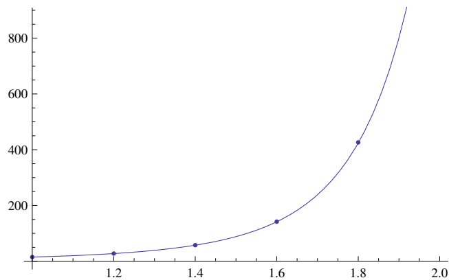
Figure 5.25: Graphs of multiplicative Runge Kutta Method and the exact function for n = 5
