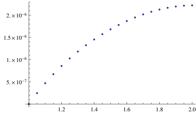
Figure 5.18: Error of Ordinary Runge Kutta Method for the ordinary Differential Equation y' = y \cdot \ln x for n = 20
