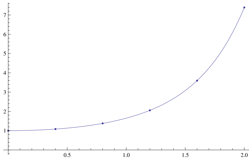
Figure 5.7: Graphs of multiplicative Runge Kutta Method and the exact function for n = 5
