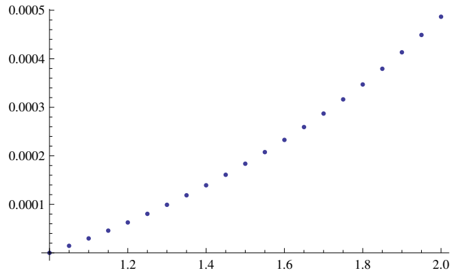
Figure 5.29: Error of Multiplicative Runge Kutta Method for the multiplicative Differential Equation y^* = e^{e^x} for n = 20
