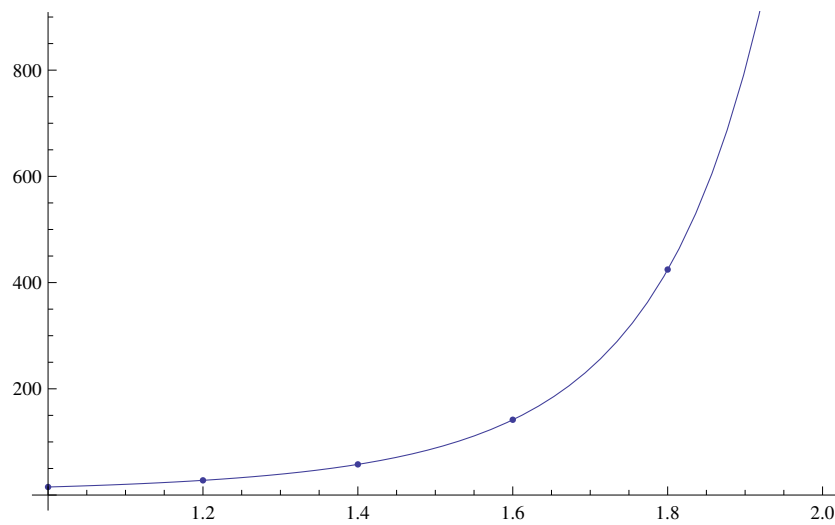
Figure 5.31: Graphs of multiplicative Runge Kutta Method and the exact function for n = 5
