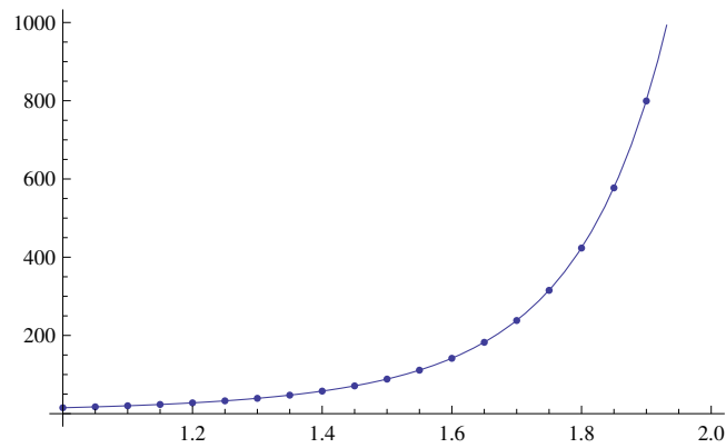
Figure 5.28: Graphs of ordinary Runge Kutta Method and the exact function for n = 20
