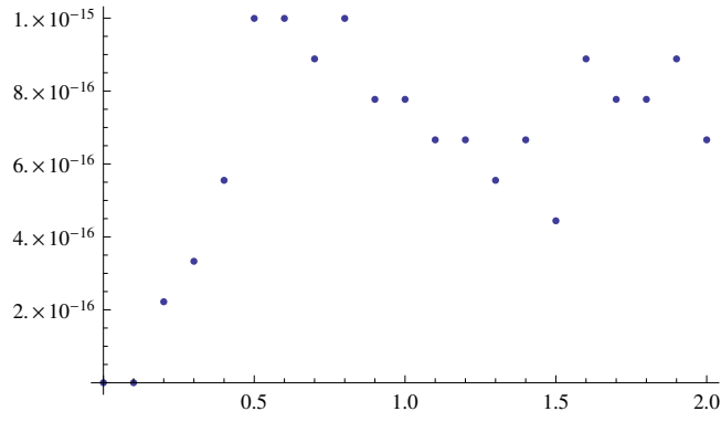
Figure 5.5: Error of Multiplicative Runge Kutta Method for the multiplicative Differential Equation y^* = e^x for n = 20
