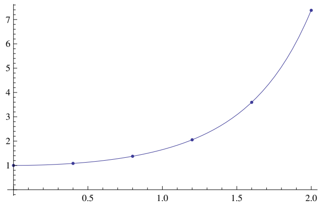
Figure 5.8: Graphs of Ordinary Runge Kutta Method and the exact function for n = 5
