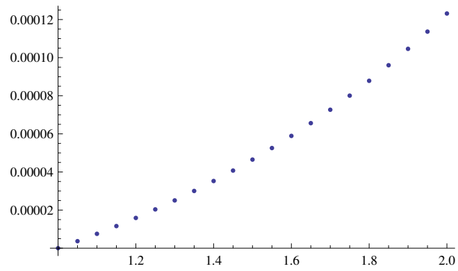
Figure 5.35: Error of Multiplicative Runge Kutta Method for the multiplicative Differential Equation y^* = e^{e^x} for n = 20
