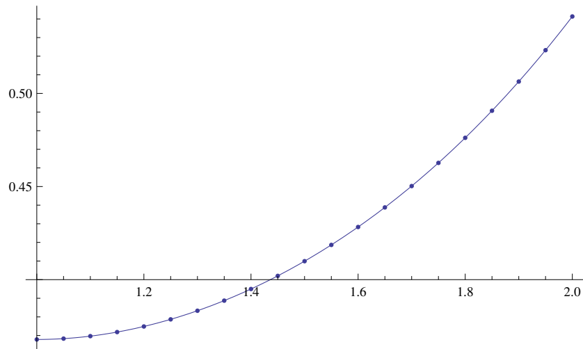
Figure 5.21: Graphs of multiplicative Runge Kutta Method and the exact function for n = 20
