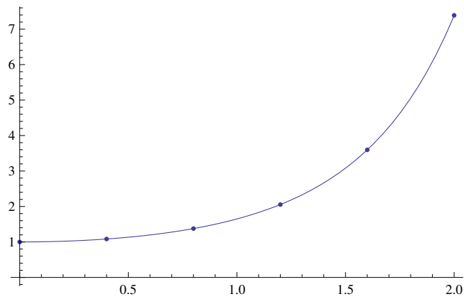
Figure 5.1: Graphs of multiplicative Runge Kutta Method and the exact function for n = 5
