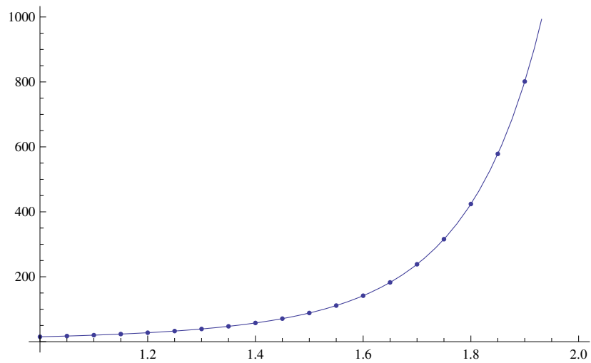
Figure 5.27: Graphs of multiplicative Runge Kutta Method and the exact function for n = 20
