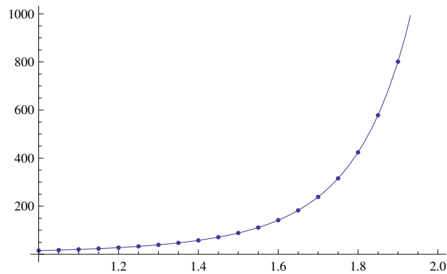
Figure 5.34: Graphs of ordinary Runge Kutta Method and the exact function for n = 20
