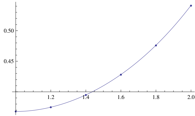
Figure 5.13: Graphs of multiplicative Runge Kutta Method and the exact function for n = 5
