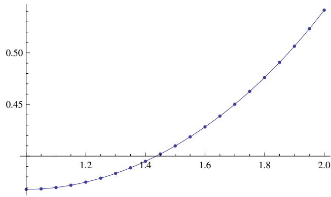
Figure 5.22: Graphs of ordinary Runge Kutta Method and the exact function for n = 20
