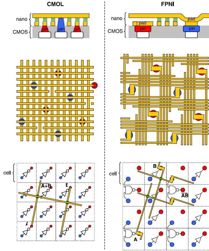
Figure 2.3 : CMOL and FPNI [3]
