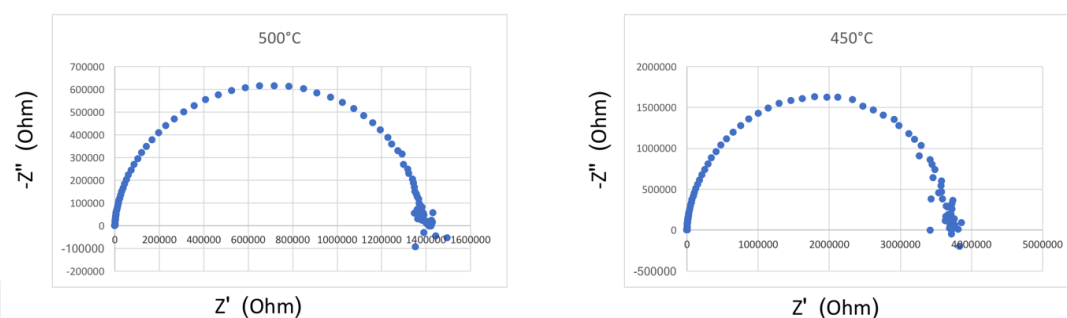
Figure: Impedance analyses of 10%Na 2 CO 3 -90%TiO 2 (reduced at 850°C-4 hours) taken at 500°C and 450°C.
