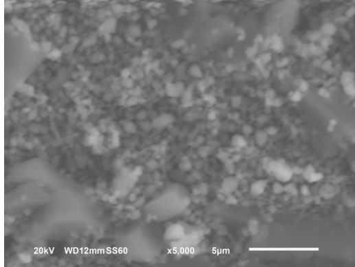
Figure 3.12. TiO 2 reduced at 850 °C for 4 hours. Composite TiO 2 -Na 2 CO 3 10 wt%. Pellet was heat treated at 700 °C for 1 hour.
