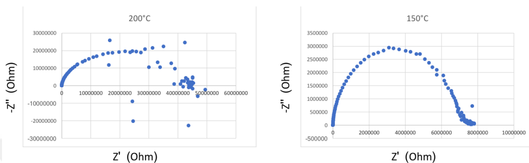
Figure: Impedance analyses of 10%Na 2 CO 3 -90%TiO 2 (reduced at 850°C-4 hours) taken at 200°C and 150°C.
