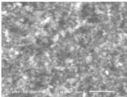
Figure 3.11. \text{TiO}_2 reduced at 800 °C for 4 hours. Composite \text{TiO}_2\text{-Na}_2\text{CO}_3 10 wt%. Pellet was heat treated at 700 °C for 1 hour.
