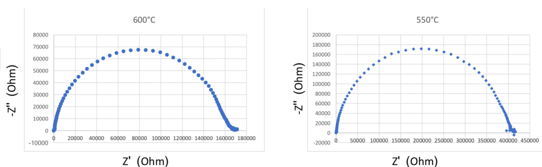
Figure 3.13. Impedance analyses of 10wt%Na 2 CO 3 -90wt%TiO 2 (reduced at 700 °C-4 hours) taken at 600 °C and 550 °C.
