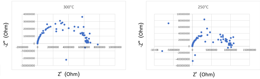
Figure: Impedance analyses of 10%Na 2 CO 3 -90%TiO 2 (reduced at 700°C-4 hours) taken at 300°C and 250°C.
