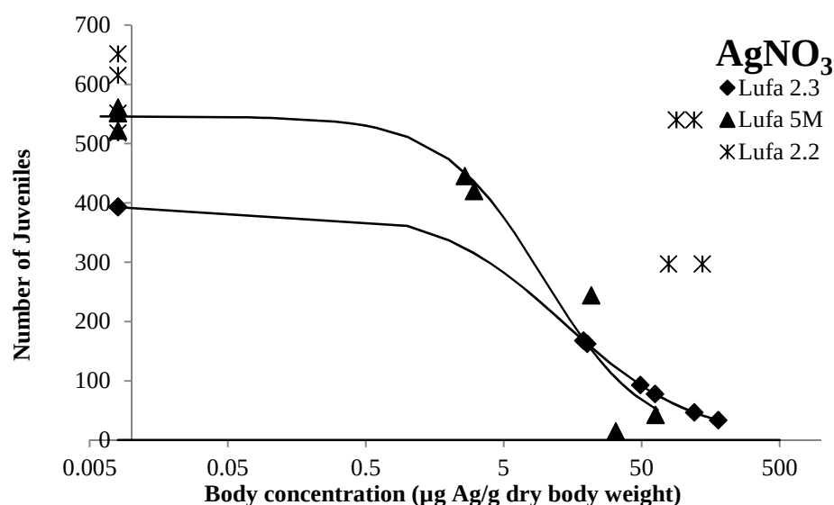
Figure 5.6a : Effects of AgNO 3 on the reproduction of Enchytraeus crypticus exposed for 21 days in Lufa 2.2, Lufa 2.3, and Lufa 5M soils. Effects are related to Ag concentrations measured in surviving animals. Data points show the number of juveniles produced in the four replicates of each concentration. Solid lines show the fit of a 3-parameter log-logistic dose-response model.
