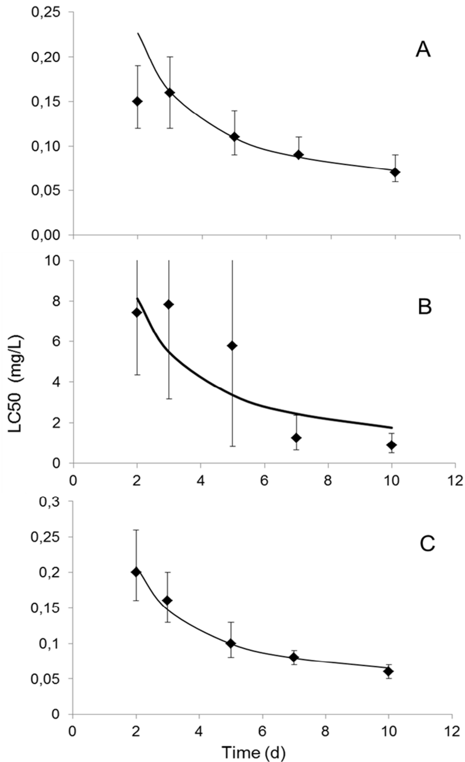
Figure 4.3 : Median lethal concentration (LC50) for the effect of a) AgNO 3 , b) AgNP-Cit, and c) AgNP-PVP on the survival of Enchytraeus crypticus upon exposure in sand-solution media for different periods of time. Data points show the LC50 values calculated with the trimmed Spearman-Kärber model (Hamilton et al., 1977) expressed on the basis of average measured concentrations in the solution phase of the test media (see Table S3); the solid lines represent the fit of Equation 4 to the data.
