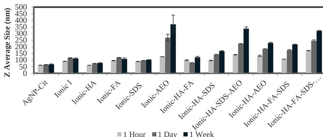
Figure 2.3a : Z Average Size of AgNP-Cit suspended in freshwater simulated media for the time points 1 hour, 1 day and 1 week (Ionic media were given in Table S2, HA and FA: 5 mg/L, SDS and AEO: 1 mg/L).
