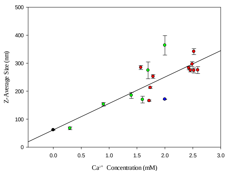
Figure 3.5a : Correlation of Z-Average size of AgNP-Cit and Ca 2+ concentration in unfiltered samples after 1 horur (Error bars represents the standard deviation of triplicates. Green data points represent surface water samples and red data points represent the wastewater samples. Blue data points show Z-average size of AgNP-Cit in freshwater simulated medium which was reported in Topuz et al.2014).
