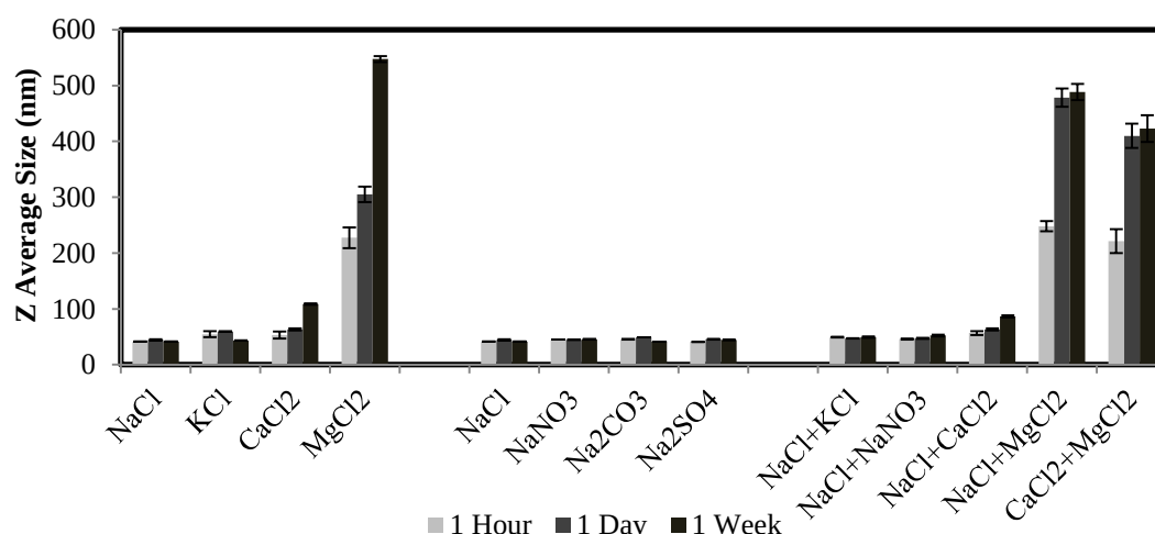
Figure 2.1b : Z Average Size of AgNP-PVP suspended in ionic media (Table S2) for the time points 1 hour, 1 day and 1 week.
