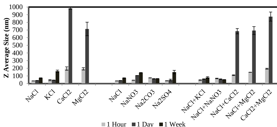
Figure 2.1a : Z Average Size of AgNP-Cit suspended in ionic media (Table S2) for the time points 1 hour, 1 day and 1 week.
