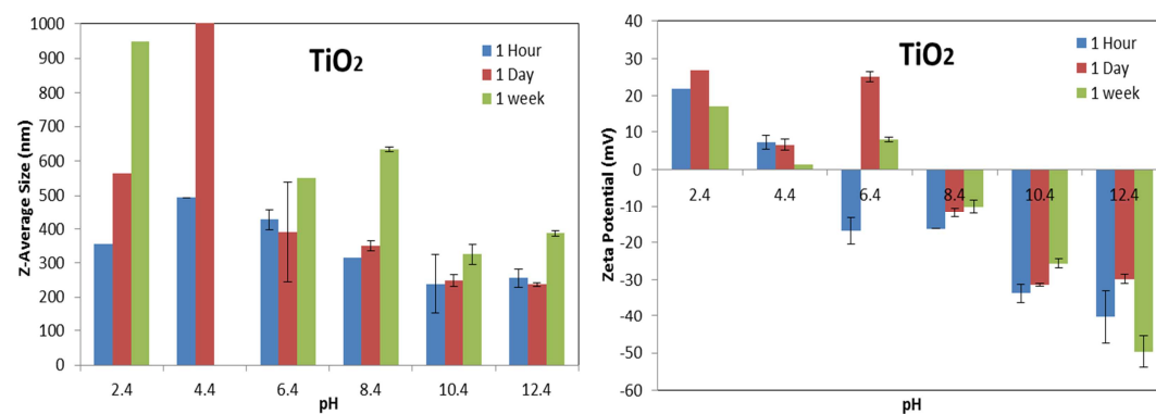
Figure A.1c : Effect of pH on the agglomeration of TiO 2 .
