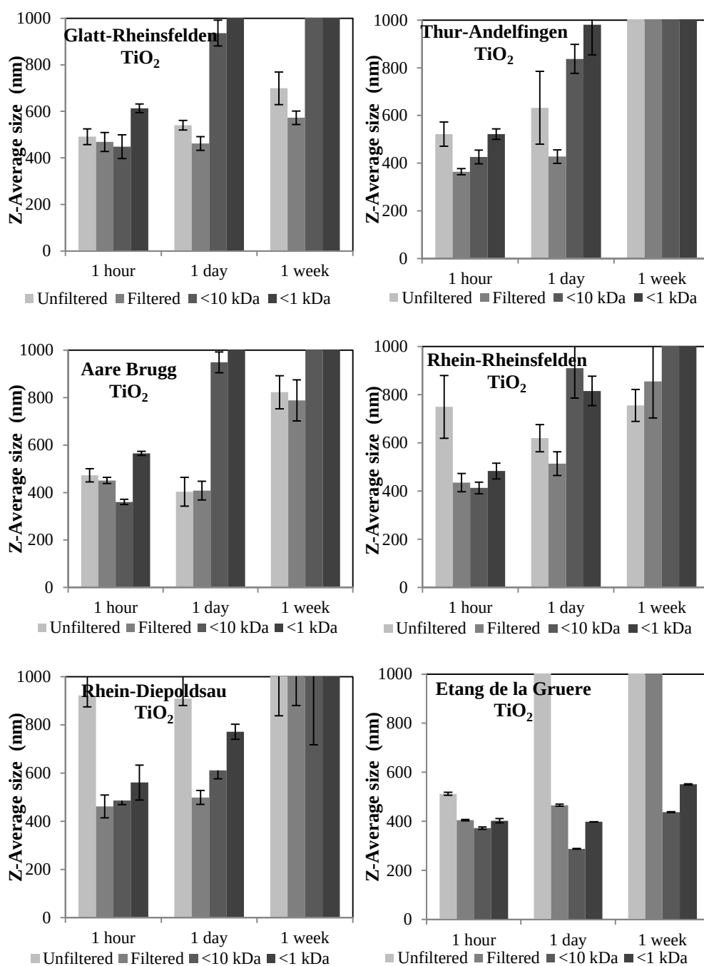
Figure 3.3 : Z-Average size levels of \text{TiO}_2 in different fractions of surface water samples (Error bars represents the standard deviation of triplicates).
