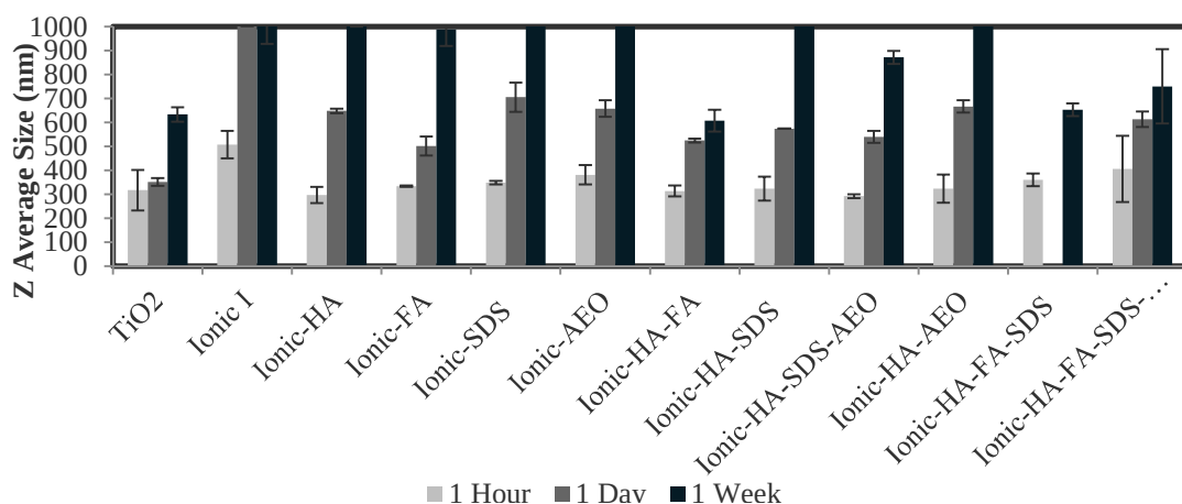
Figure 2.3c : Z Average Size of TiO 2 suspended in freshwater simulated media for the time points 1 hour, 1 day and 1 week (Ionic media were given in Table S2, HA and FA: 5 mg/L, SDS and AEO: 1 mg/L).
