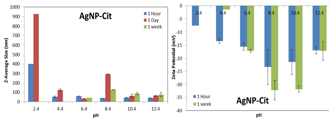
Figure A.1a : Effect of pH on the agglomeration of AgNP-Cit.
