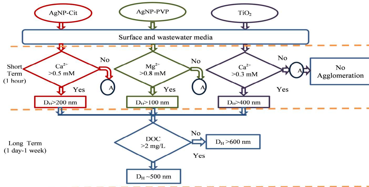
Figure 3.7 : A generalized scheme for the agglomeration behavior of AgNP-Cit, AgNP-PVP and TiO 2 in surface and wastewater.
