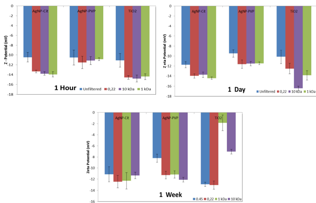
Figure B.8 : Zeta Potential of ENPs in the fractions of Thur Andelfingen sample over time (Error bars represent the standard deviation of duplicate samples).
