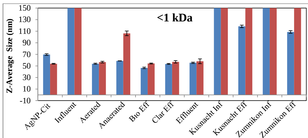
Figure B.17 : Z-Average size levels of AgNP-PVP in the fractions of wastewater samples .
