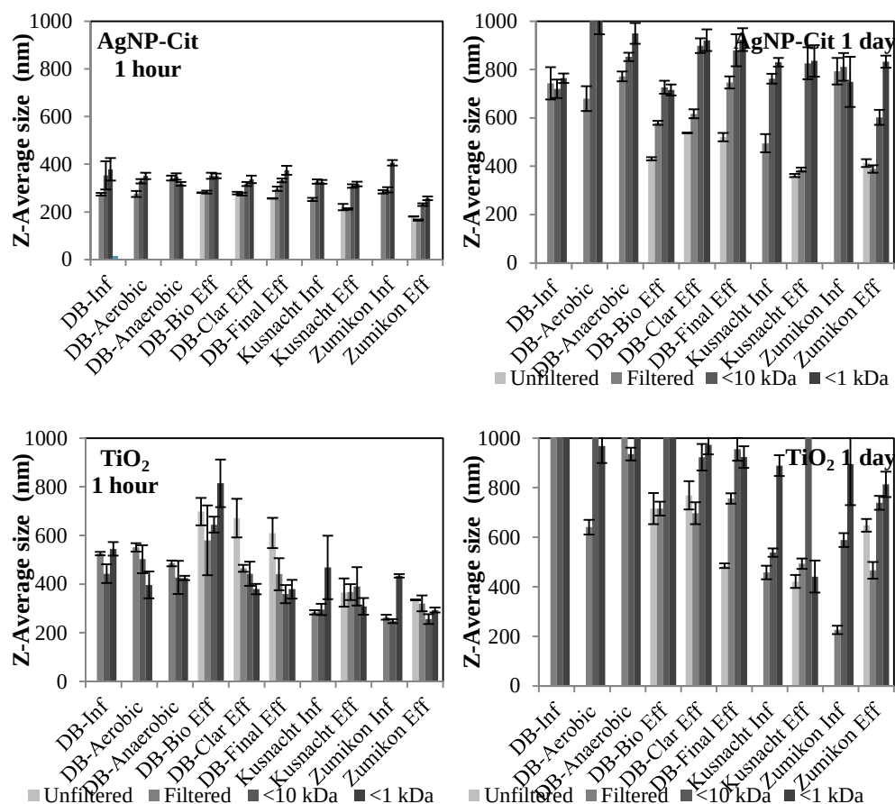
Figure 3.4 : Z-Average size levels in different fractions of wastewater samples (Error bars represents the standard deviation of triplicates).
