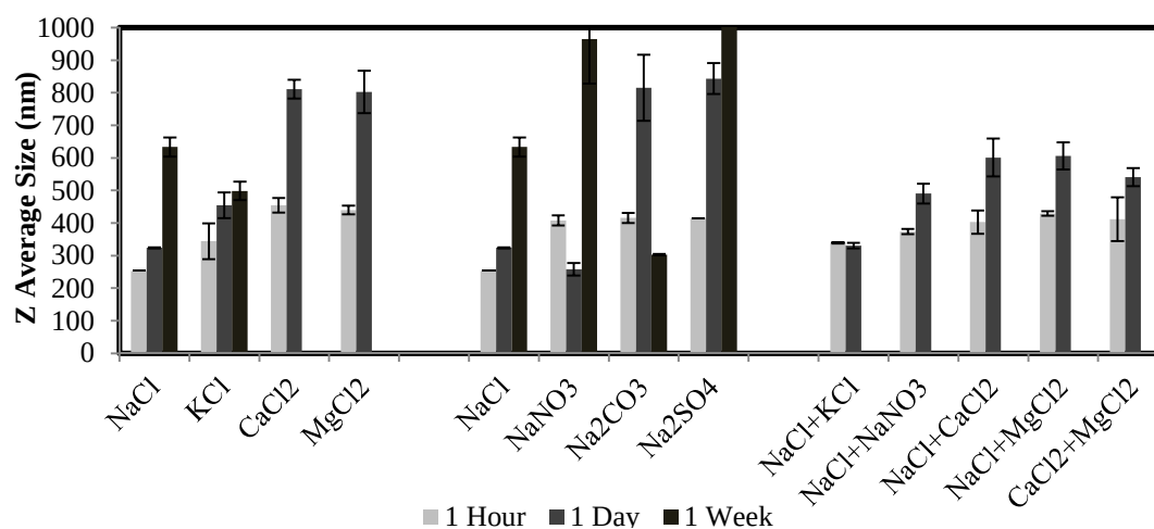
Figure 2.1c : Z Average Size of TiO 2 suspended in ionic media (Table S2) for the time points 1 hour, 1 day and 1 week.
