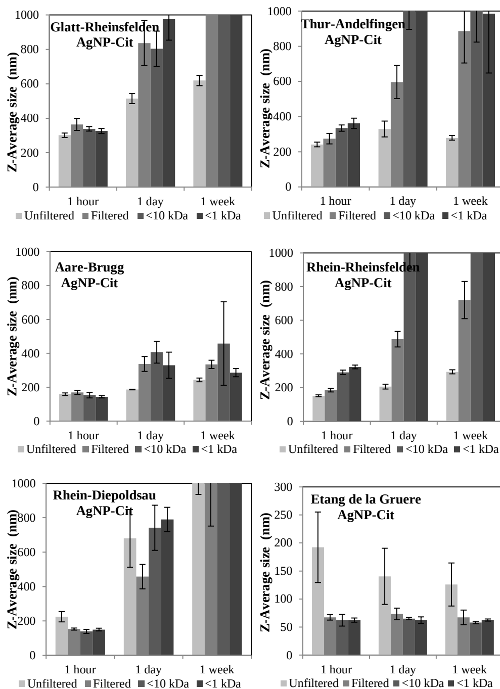
Figure 3.1 : Z-Average size levels of AgNP-Cit in different fractions of surface water samples (Error bars represents the standard deviation of triplicates).
