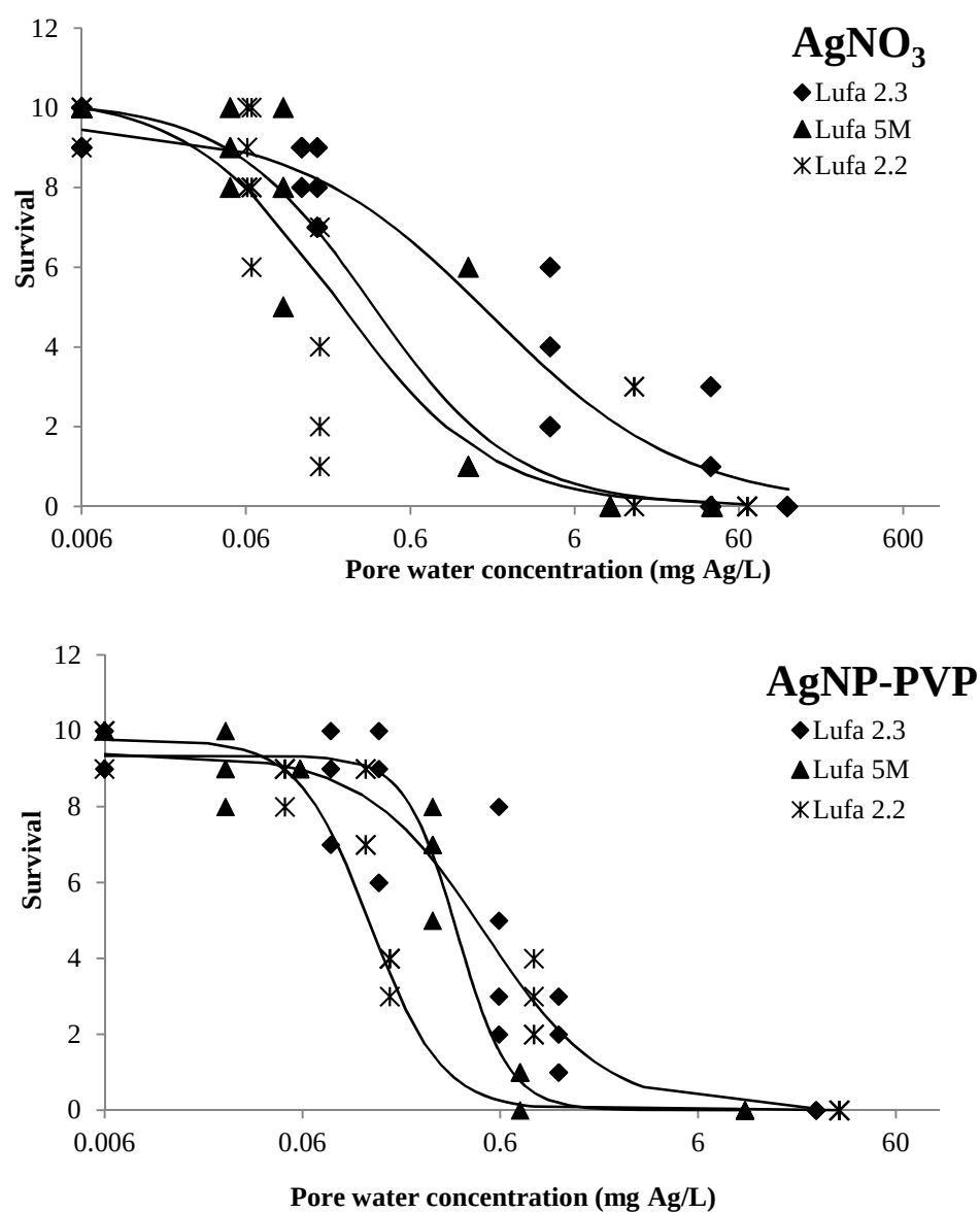
Figure D.8 : Effects of ENPs on the survival of Enchytraeus crypticus after 21 days exposure in Lufa 2.2, Lufa 2.3 and Lufa 5M soils, related to porewater concentrations measured in the soils at the end of the exposures. Data points show survival (out of 10 individuals) in the four replicates for each test concentration. Solid line shows the fit to the data of a 3-parameter logistic dose-response model.
