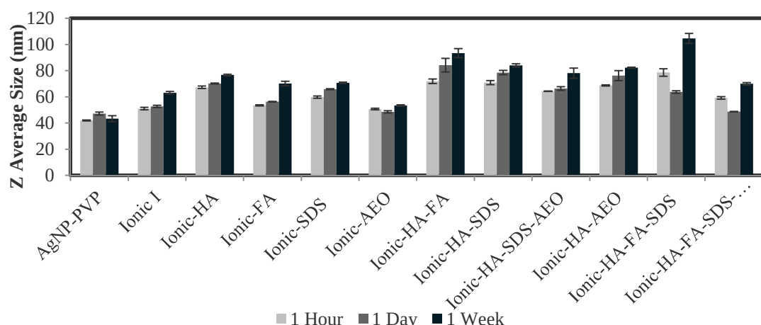
Figure 2.3b : Z Average Size of AgNP-PVP suspended in freshwater simulated media for the time points 1 hour, 1 day and 1 week (Ionic media were given in Table S2, HA and FA: 5 mg/L, SDS and AEO: 1 mg/L).
