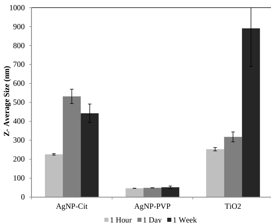
Figure 2.1 : Z Average Size of ENPs in Chriesbach river water sample for the time points 1 hour, 1 day and 1 week.
