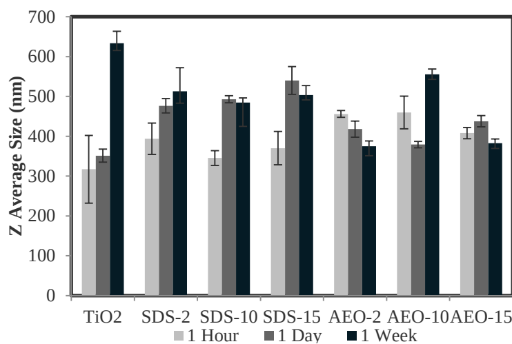
Figure A. 5: Z-Average Size of ENPs suspended in different surfactant media.
