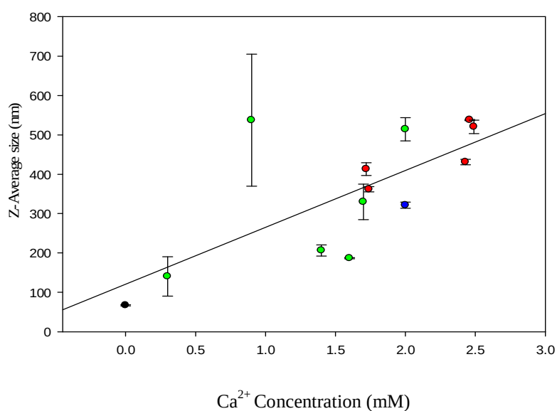
Figure 3.5a : Correlation of Z-Average size of AgNP-Cit and Ca 2+ concentration in unfiltered samples after 1 day (Error bars represents the standard deviation of triplicates. Green data points represent surface water samples and red data points represent the wastewater samples. Blue data points show Z-average size of AgNP-Cit in freshwater simulated medium which was reported in Topuz et al.2014).
