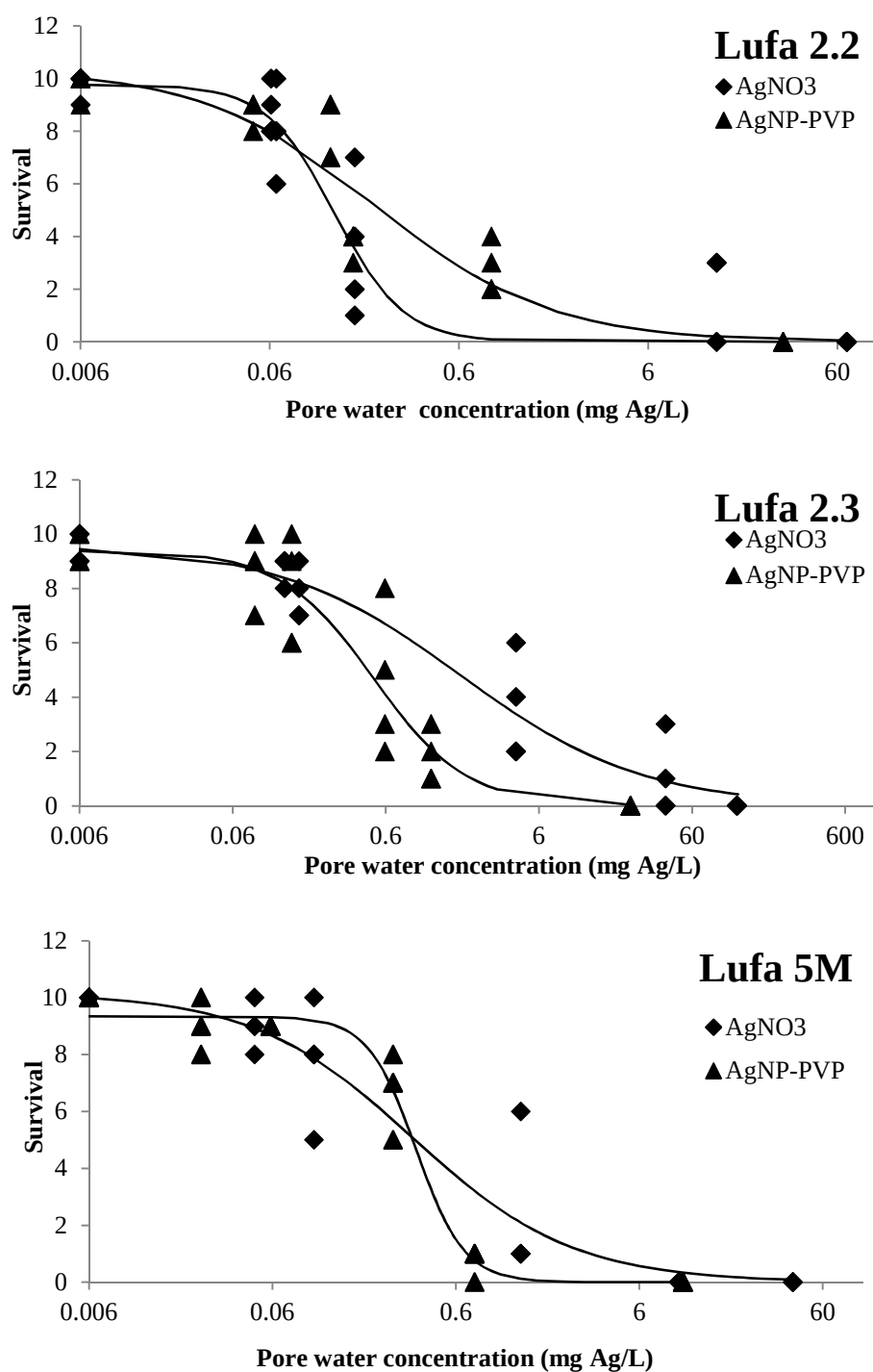
Figure D.4 : Comparison of dose-response curves for the effect of AgNO 3 and AgNP-PVP on the survival of Enchytraeus crypticus exposed for 21 days in Lufa 2.2, Lufa 2.3, and Lufa 5M soils. Effects are related to porewater Ag concentrations measured at the end of the exposures. Data points show survival (out of 10 individuals) in the four replicates of each concentration. Solid lines show the fit of a 3-parameter logistic dose-response model.
