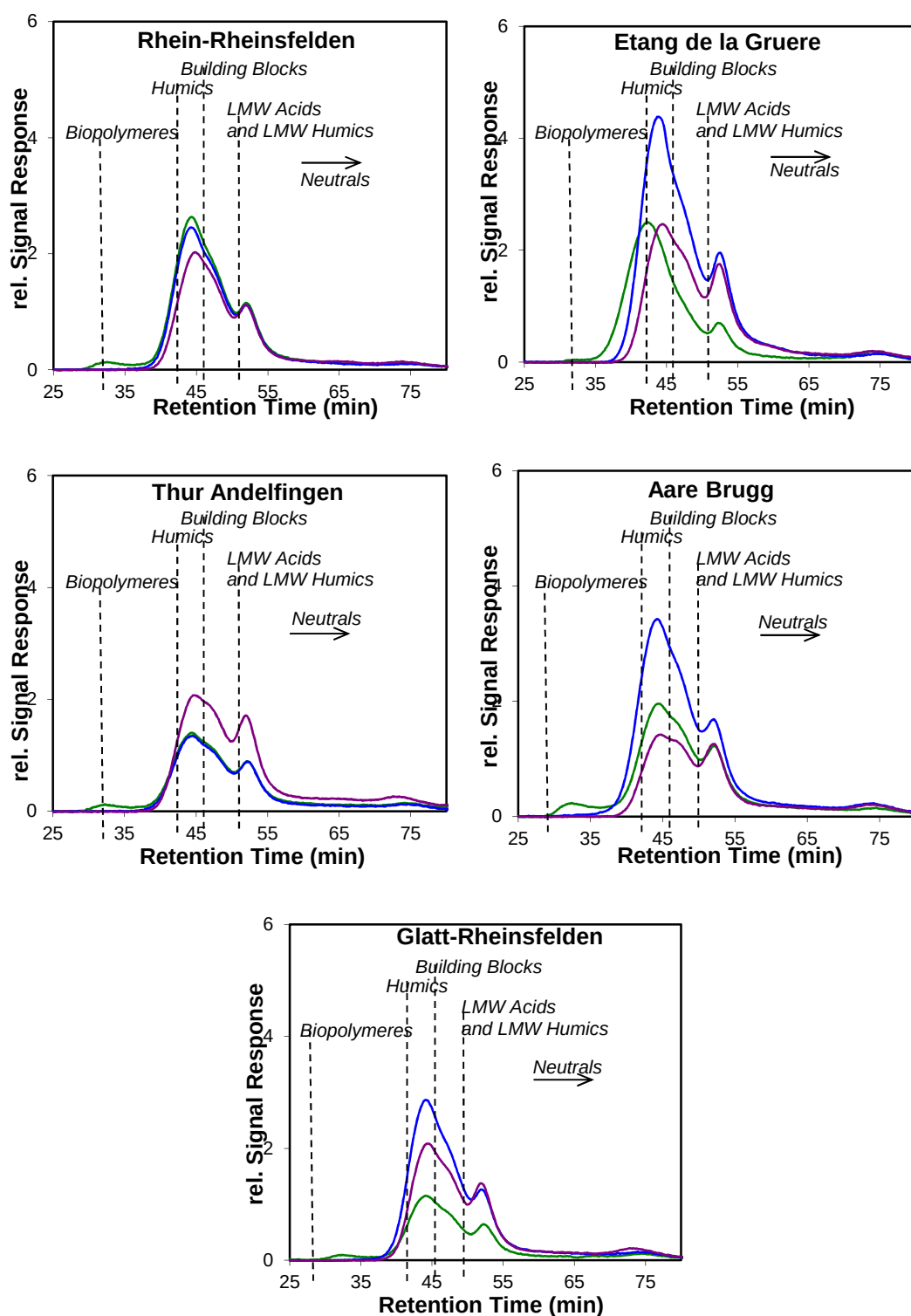
Figure B.3 : LC-OCD-OND chromatograms for the filtered (0.2 µm) surface water samples.
