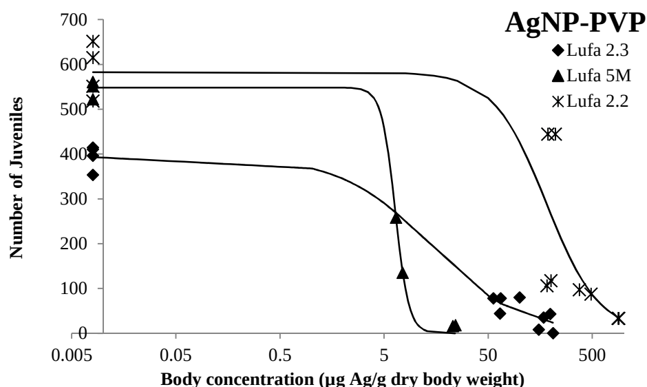
Figure 5.7b : Effects of AgNP-PVP on the reproduction of Enchytraeus crypticus exposed for 21 days in Lufa 2.2, Lufa 2.3, and Lufa 5M soils. Effects are related to Ag concentrations measured in surviving animals. Data points show the number of juveniles produced in the four replicates of each concentration. Solid lines show the fit of a 3-parameter log-logistic dose-response model.
