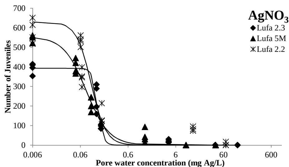
Figure 5.4a : Effects of AgNO 3 on the reproduction of Enchytraeus crypticus exposed for 21 days in Lufa 2.2, Lufa 2.3, and Lufa 5M soils. Effects are related to Ag concentrations measured in pore water at the end of the exposures. Data points show the number of juveniles produced in the four replicates of each concentration. Solid lines show the fit of a 3-parameter logistic dose-response model.
