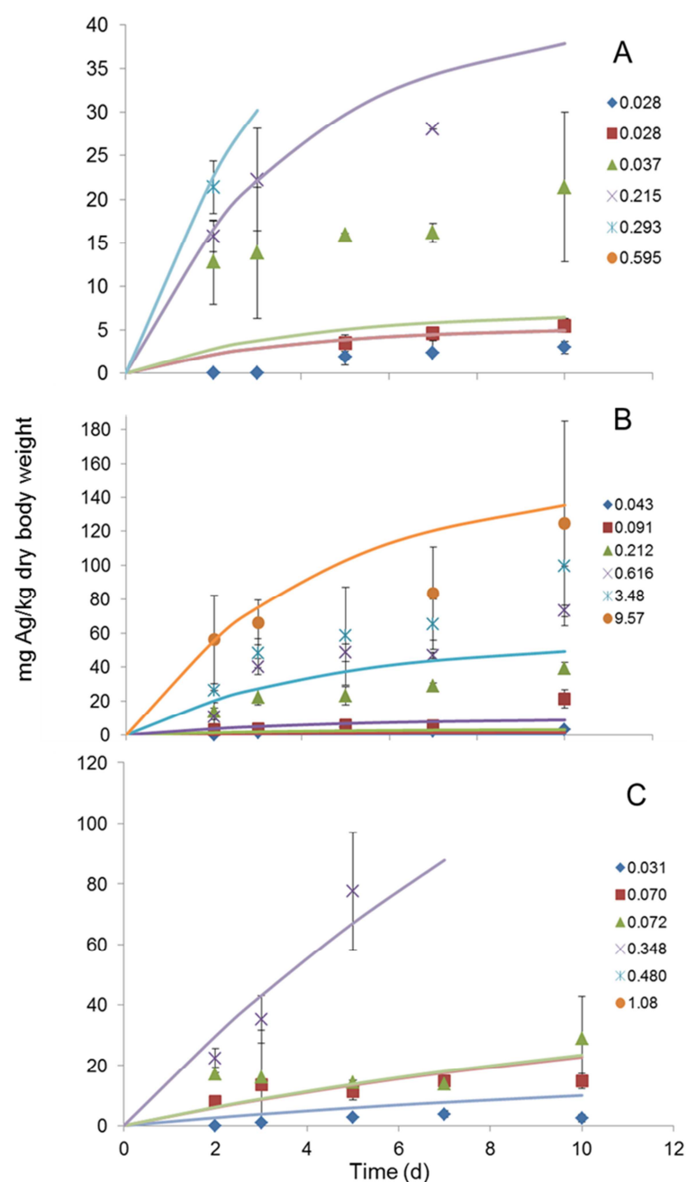
Figure 4.2 : Development with time of internal total Ag concentrations in Enchytraeus crypticus exposed to a) AgNO 3 , b) AgNP-Cit, and c) AgNP-PVP in a sand-solution medium. Data points show the measured total Ag concentrations in E. crypticus at each sampling time, the solid lines represent the fit of the one-compartment model (Equation 1) to the data for the different measured exposure concentrations in the solution phase of the sand-solution medium (in mg Ag/L; obtained after 0.45 \mu m filtration). Error bars represent the standard deviations of the concentrations measured in triplicate samples.
