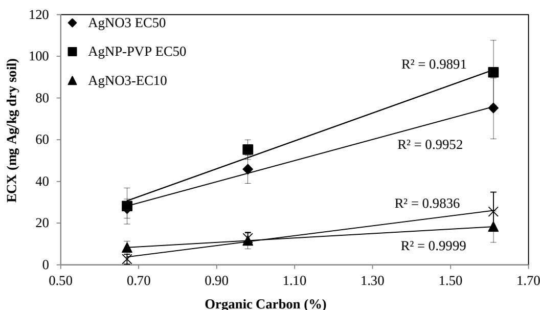
Figure 5.3 : Effect of soil organic carbon content on toxicity of AgNO 3 and AgNP-PVP to Enchytraeus crypticus after 21 days exposure in three different soils. Data points show the EC 50 and EC 10 values for the effects on reproduction calculated with a 3-parameter logistic dose-response model. Solid lines represent trend lines relating EC 50 and EC 10 values to organic carbon content of the soils and R 2 shows the goodness of fit. Error bars represent the 95% confidence intervals for EC 50 and EC 10 values.
