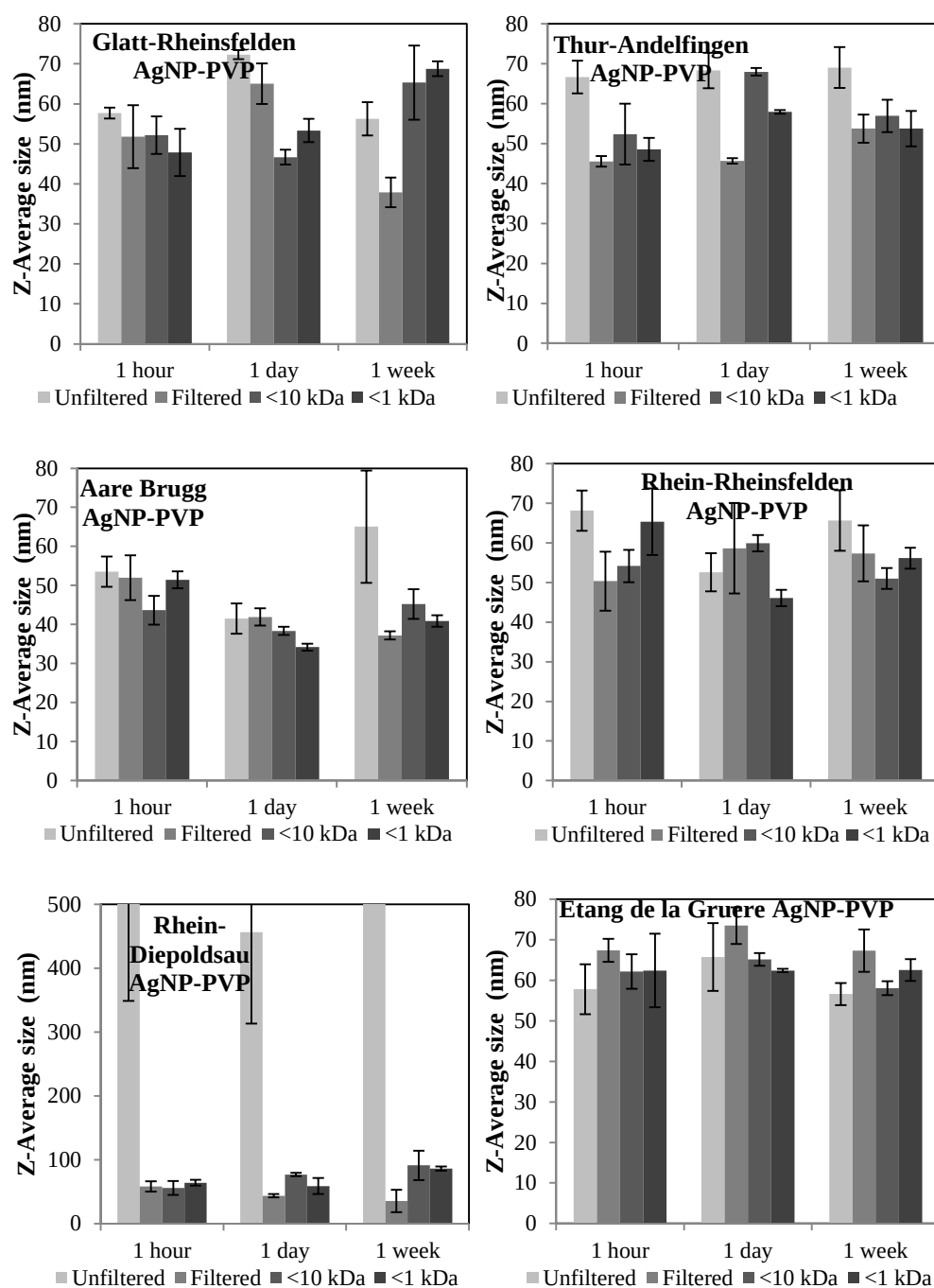
Figure 3.2 : Z-Average size levels of AgNP-PVP in different fractions of surface water samples (Error bars represents the standard deviation of triplicates).
