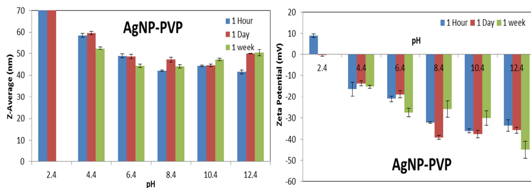
Figure A.1b : Effect of pH on the agglomeration of AgNP-PVP.
