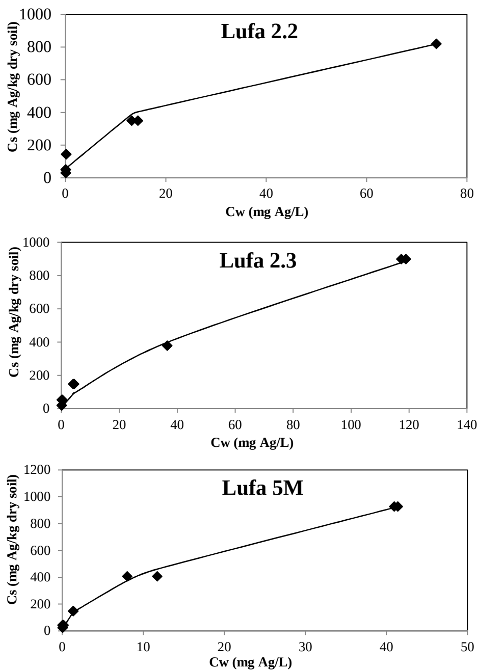
Figure D.1 : The relation between total Ag concentration in soil and the concentration in pore water of Lufa 2.2, Lufa 2.3, and Lufa 5M soils spiked with \text{AgNO}_3 . Data points show the measured concentrations. Solid lines represent the fit of a Freundlich isotherm to the data.
