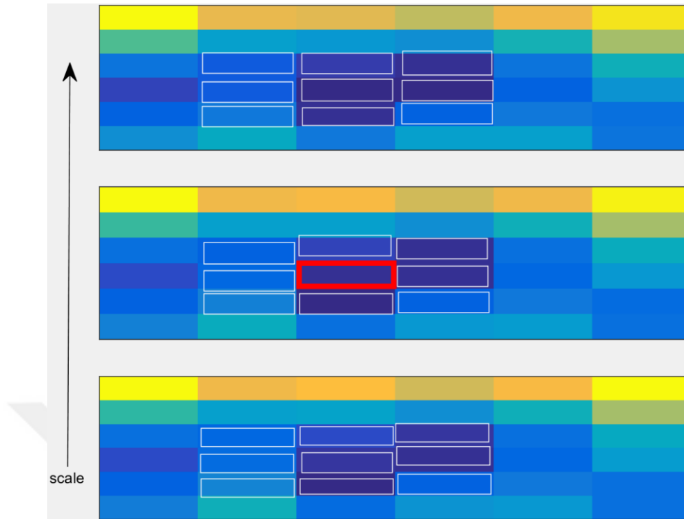
Figure 4. 2 . A pixel (red boundary), 8 neighbors in the same octave and 18 pixels from one above and below octaves.
