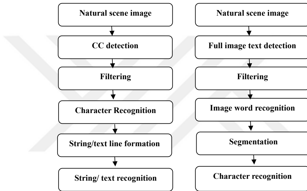
Figure 2.1. (a). Connected component and (b). Sliding window based approach
