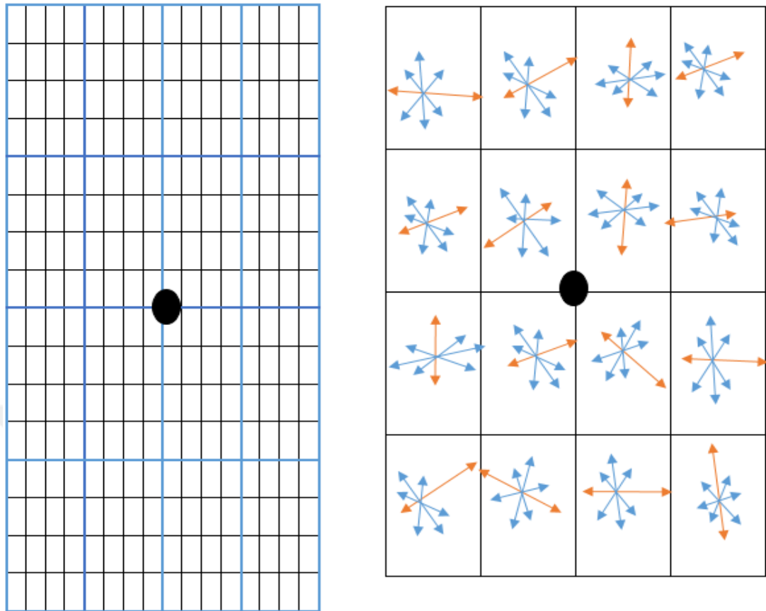
Figure 4.6. 16x16 window (left) and gradient direction per window (right)
