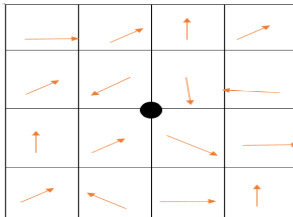
Figure 4.7. Dominant direction selection for a keypoint
