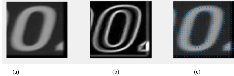
Figure 4.3. Gaussian blurred image (a), Gradient magnitude (b) and Gradient orientation(c)
