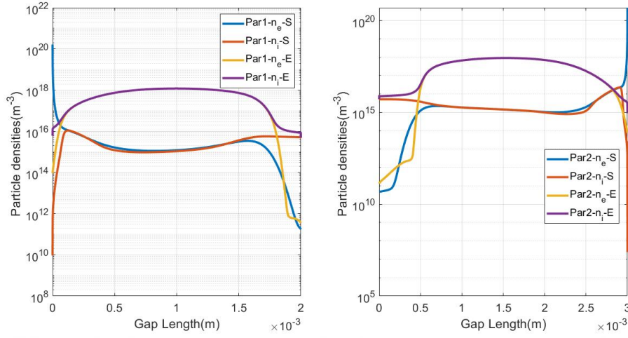
Figure 4.11: Particle densities vs position where voltage value 750 V in driving source is 750 V. ParS1, ParS2 is an abbreviation from Table 4.1 and Table 4.2 respectively. S, E stand for simple model, extended model approach respectively. .
