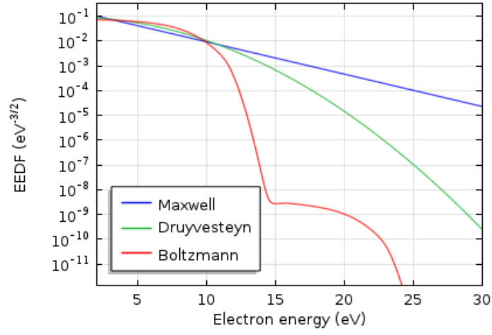
Figure 3.1: Comparison of EEDF vs electron energy. The mean electron energy is 5 eV, the electron density is 10^{16}(\text{m}^{-3}) , ionization degree is 10^{-9} [43]
