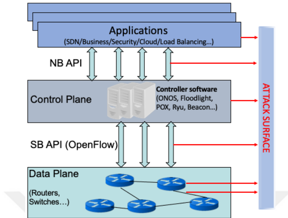
Figure 2.1: Software-defined networking (SDN) Architecture and Attack Surface.
