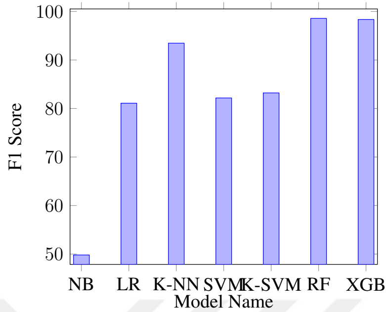
Figure 5.5: Model comparison.
