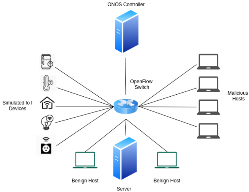
Figure 5.1: Testbed environment for the first dataset.
