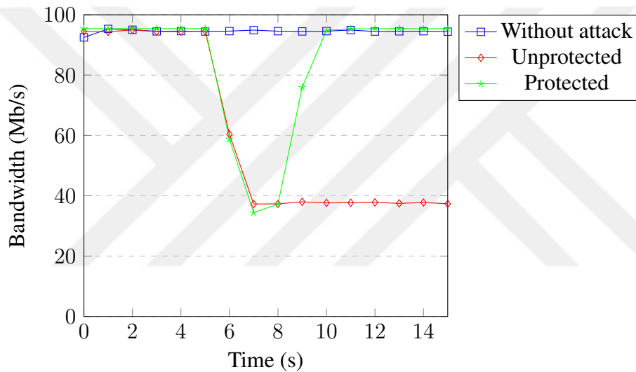
Figure 6.9: Available bandwidth under UDP flood without spoofing.
