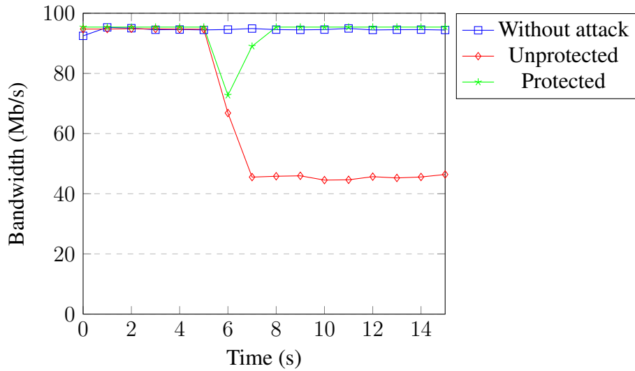
Figure 6.10: Available bandwidth under UDP flood with spoofing.
