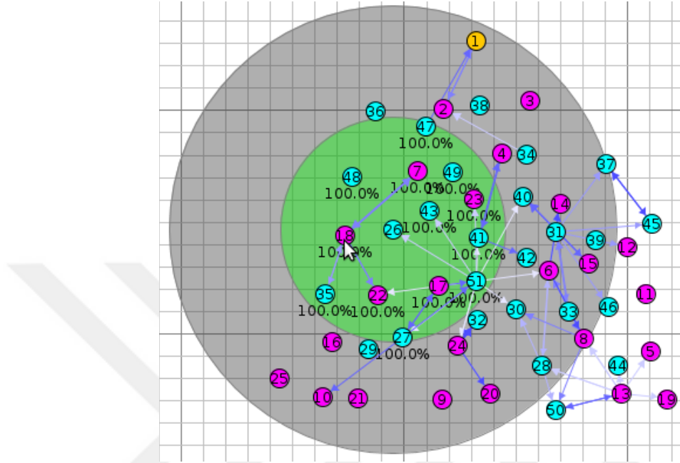
Figure 3.8: Sample RPL network topology 1 built in COOJA. The node 1 is the sink node while all other are source nodes which transmit data to sink node. The arrows represent the flow of radio messages. The green circle represents transmission area and grey circle shows the radio collision region. The percentages represent the reception ratio.
