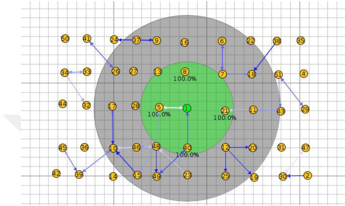
Figure 3.9: Sample RPL network topology 2 built in COOJA. The node 1 is the sink node while all other are source nodes which transmit data to sink node. The arrows represent the flow of radio messages. The green circle represents transmission area and grey circle shows the radio collision region. The percentages represent the reception ratio.
