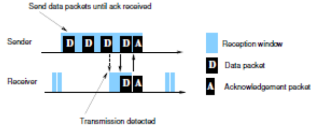
Figure 3.3: ContikiMAC [3]
