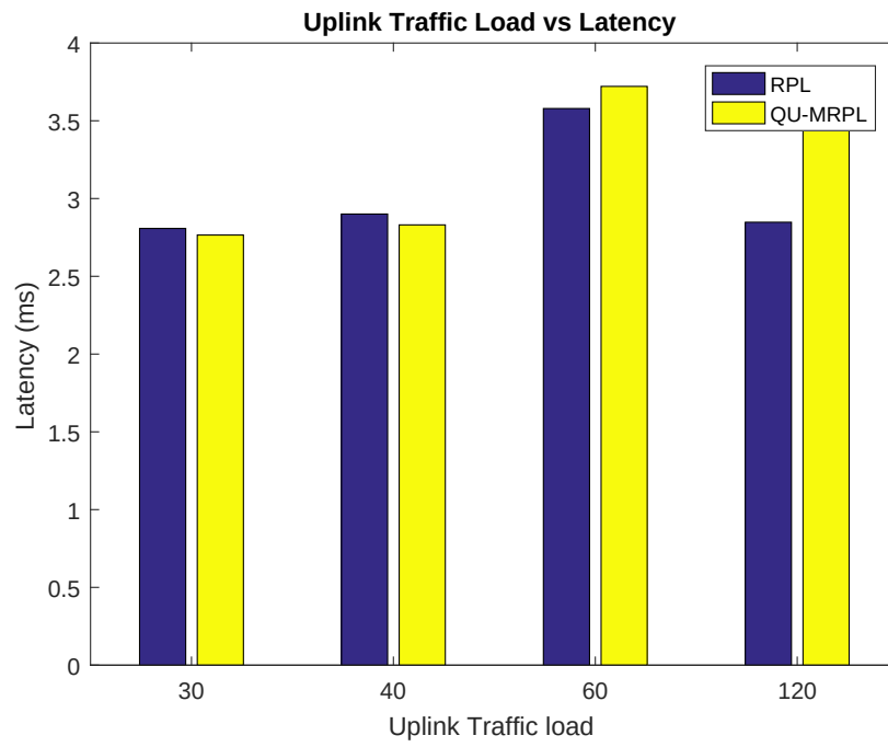
Figure 4.11: Latency of RPL and QU-MRPL in Topology 1 with varying data rates with OF0
