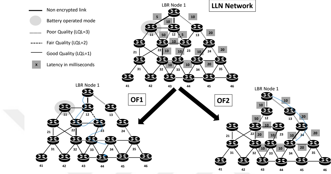
Figure 2.2: An illustration of DODAG with two different objective functions [2]
