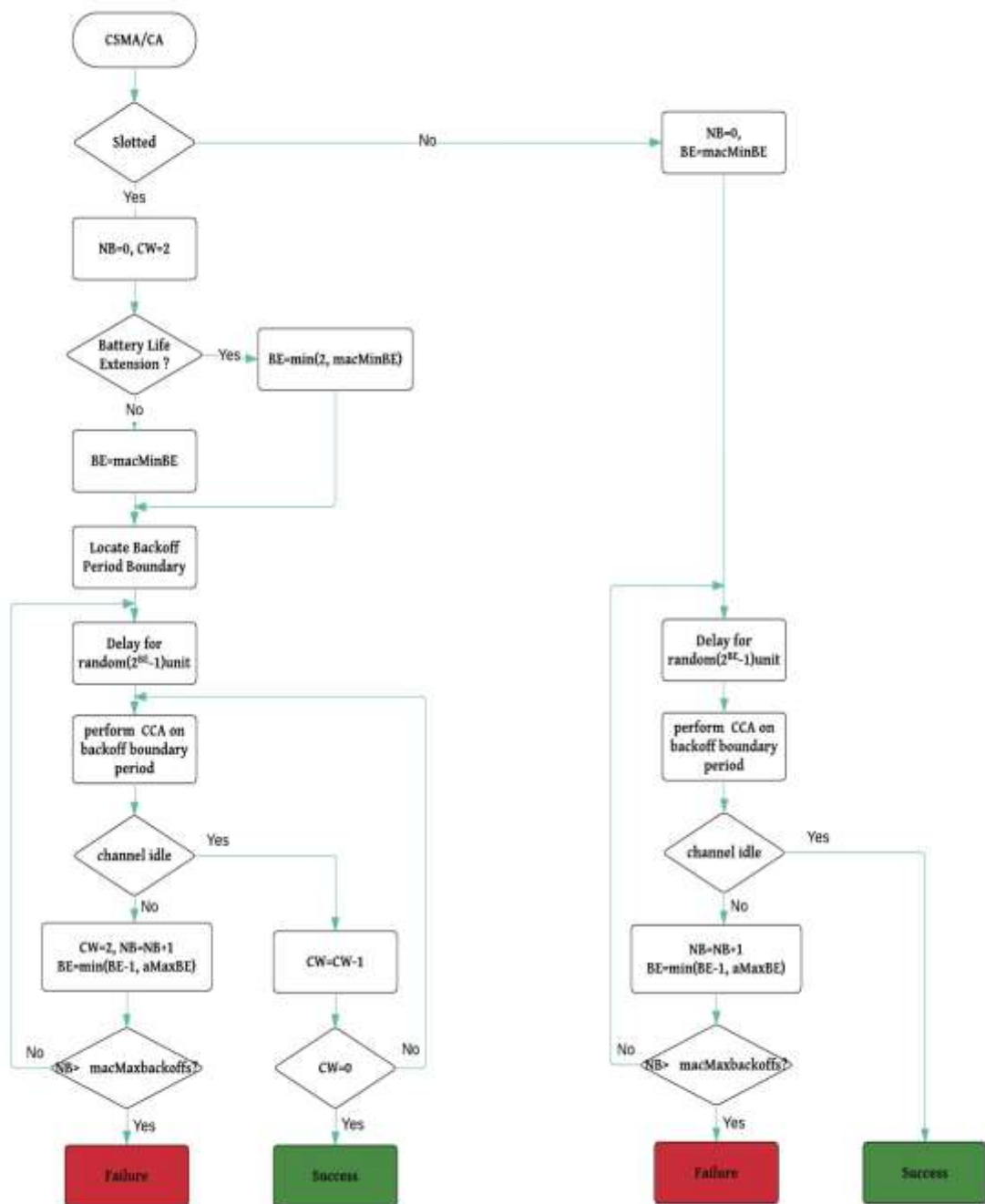
Figure 3.5. CSMA/CA Algorithm
