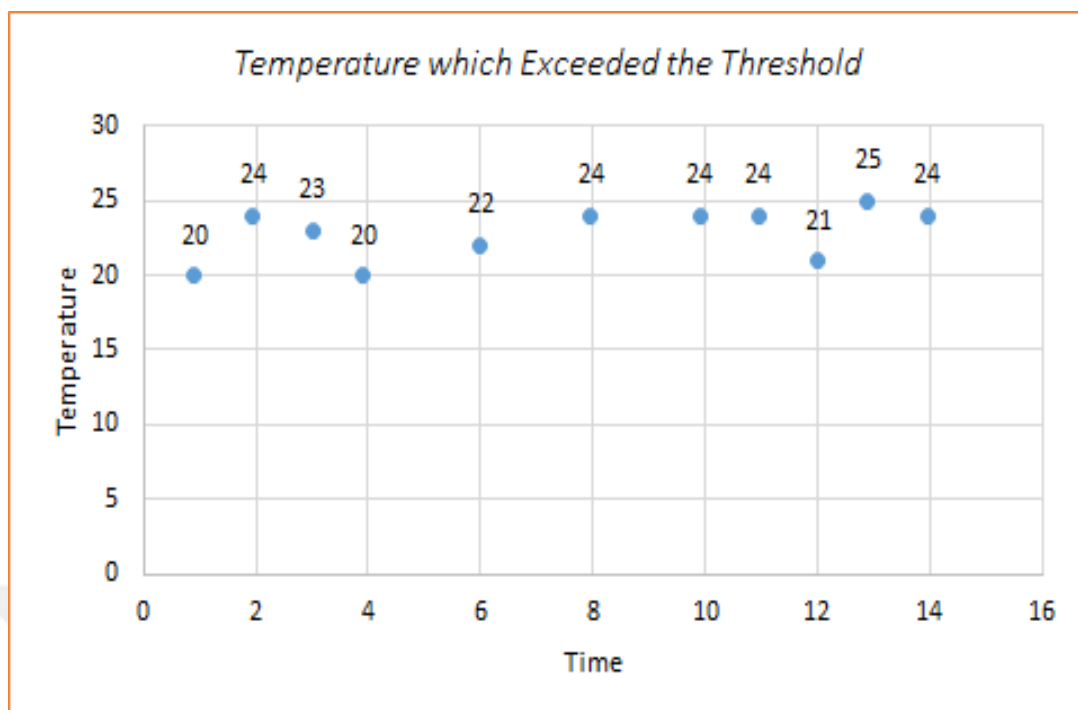
Figure 4.14. The value of temperature which exceeded the pre-defined threshold
