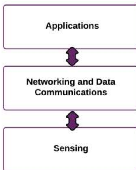
Figure 2.2. Three-tiered architecture
