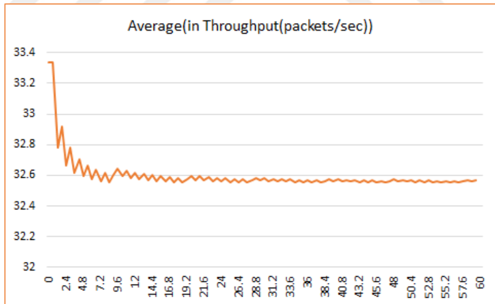
Figure 4.10. Throughput
