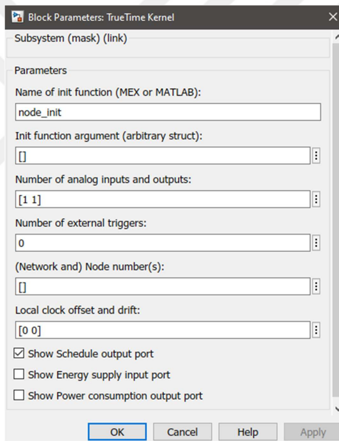
Figure 17: TrueTime Kernel Block Configuration
