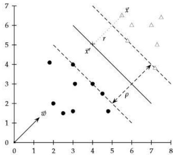
Figure 4.2 The support vectors linear separable case
