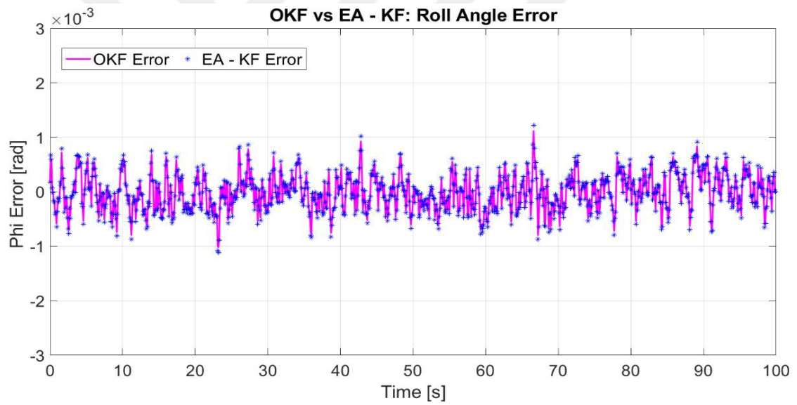
Figure 5.34. Mean EA - KF error vs. OKF error comparison for roll angle
