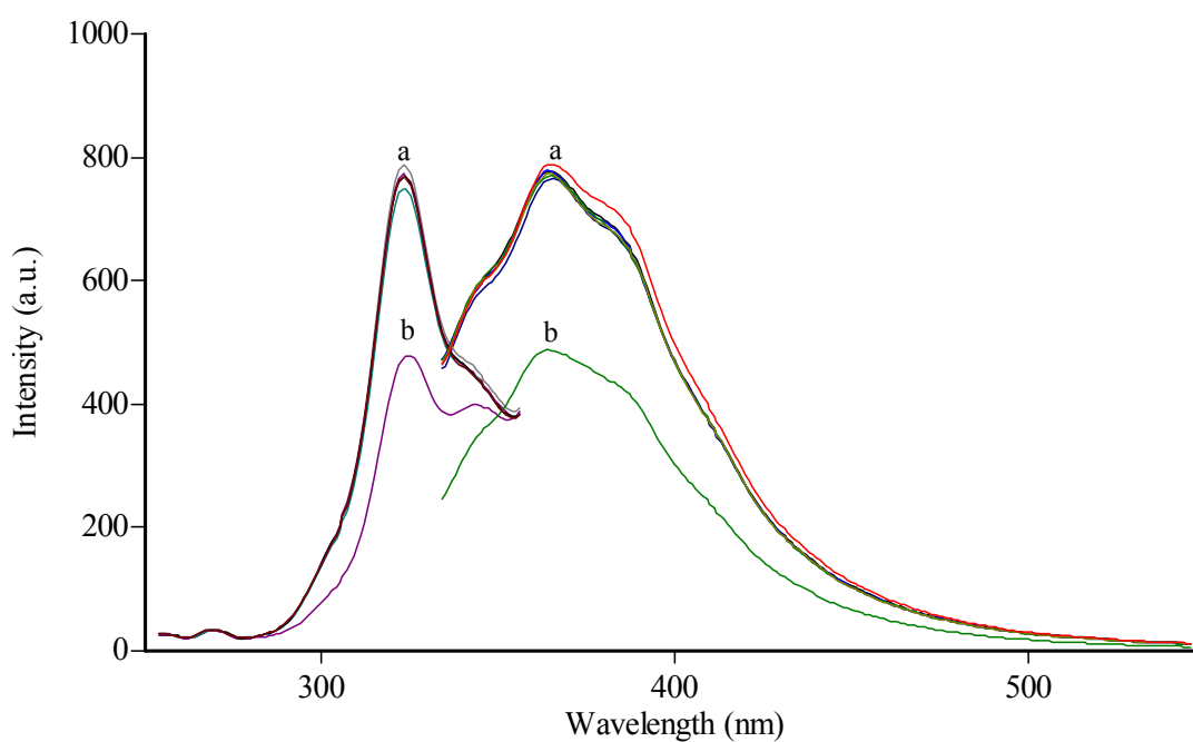
Figure 7.18 pH induced emission based spectral response of the EC doped MY4 in the pH range of 7.00-4.00. pH: a) 7.00, 6.50, 6.00, 5.50, 5.00, 4.50 b) 4.00.
