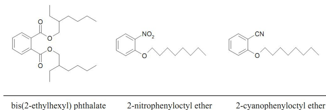
Figure 2.13 Chemical structures of lipophilic and polar plasticizers (taken from Mohr, 2006).
