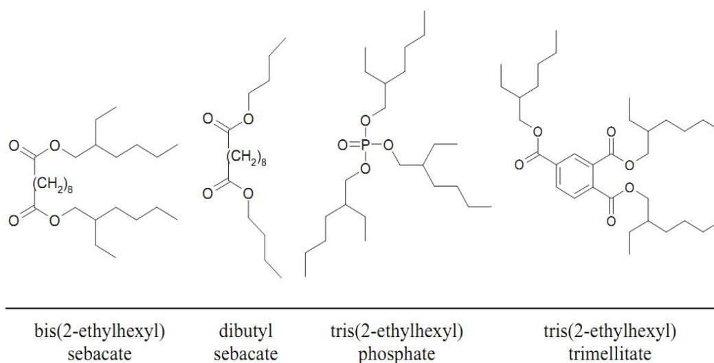
Figure 2.12 Chemical structures of some lipophilic plasticizers (taken from Mohr, 2006).
