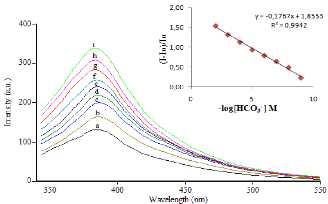
Figure 7.29 Emission spectra of immobilized MY4 in EC nano fibers after exposure to different \text{HCO}_3^- concentrations; (a) bicarbonate free water (b) 1.00 \times 10^{-9} \text{ M} (c) 1.00 \times 10^{-8} \text{ M} (d) 1.00 \times 10^{-7} \text{ M} (e) 1.00 \times 10^{-6} \text{ M} (f) 1.00 \times 10^{-5} \text{ M} (g) 1.00 \times 10^{-4} \text{ M} (h) 1.00 \times 10^{-3} \text{ M} (i) 1.00 \times 10^{-2} \text{ M} .
