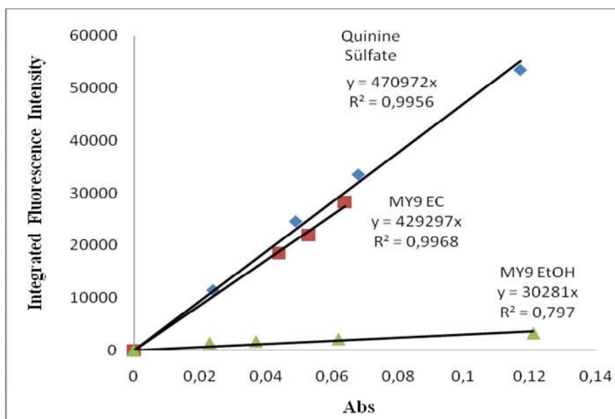
Figure 6.6 The integrated fluorescence intensities vs absorbance for the reference standard; quinine sulphate in \text{H}_2\text{SO}_4 , MY9 dye in EC and EtOH matrices.
