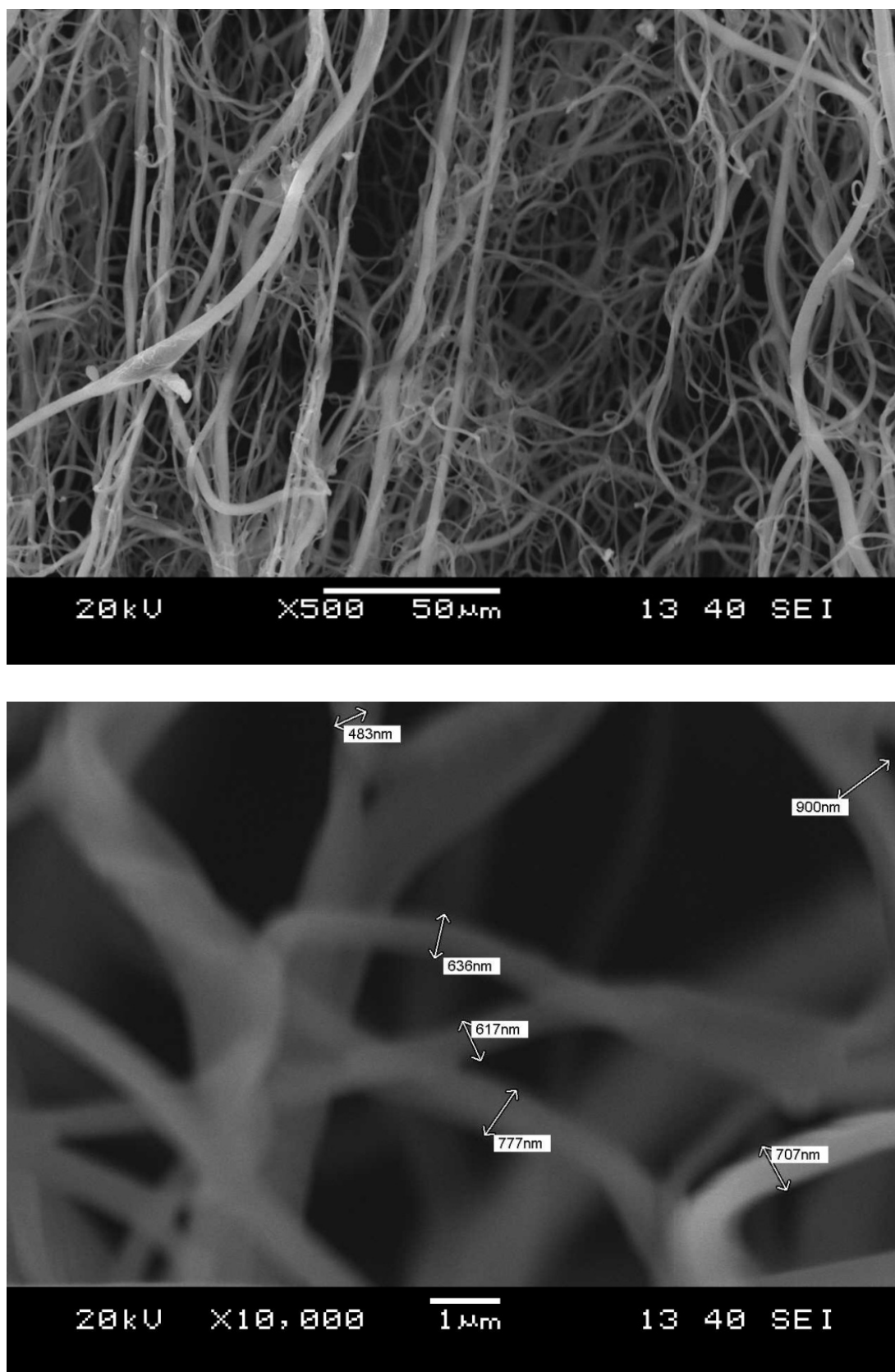
Figure 6.22 SEM images of EC based electrospun nanofibers for MY10 dye at different magnifications such as \times 500 and \times 10\,000 . Fiber diameters were between 483-900 nm.
