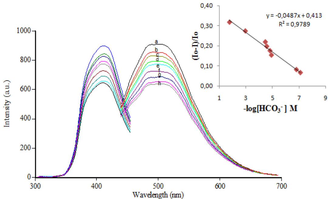
Figure 6.28 Emission spectra of immobilized MY10 in PMMA based nanofibers matrix after exposure to different \text{HCO}_3^- concentrations; (a) bicarbonate free water (b) 8.00 \times 10^{-8} \text{ M} (c) 1.60 \times 10^{-7} \text{ M} (d) 1.20 \times 10^{-5} \text{ M} (e) 1.57 \times 10^{-5} \text{ M} (f) 2.75 \times 10^{-5} \text{ M} (g) 3.50 \times 10^{-5} \text{ M} (h) 1.13 \times 10^{-3} ; 1.80 \times 10^{-2} \text{ M} .
