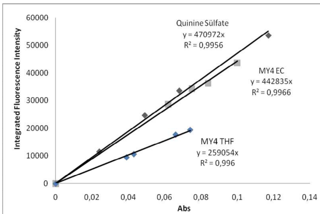
Figure 7.9 The integrated fluorescence intensities vs absorbance for the reference standard; quinine sulphate in \text{H}_2\text{SO}_4 , MY4 dye in EC and THF matrices.
