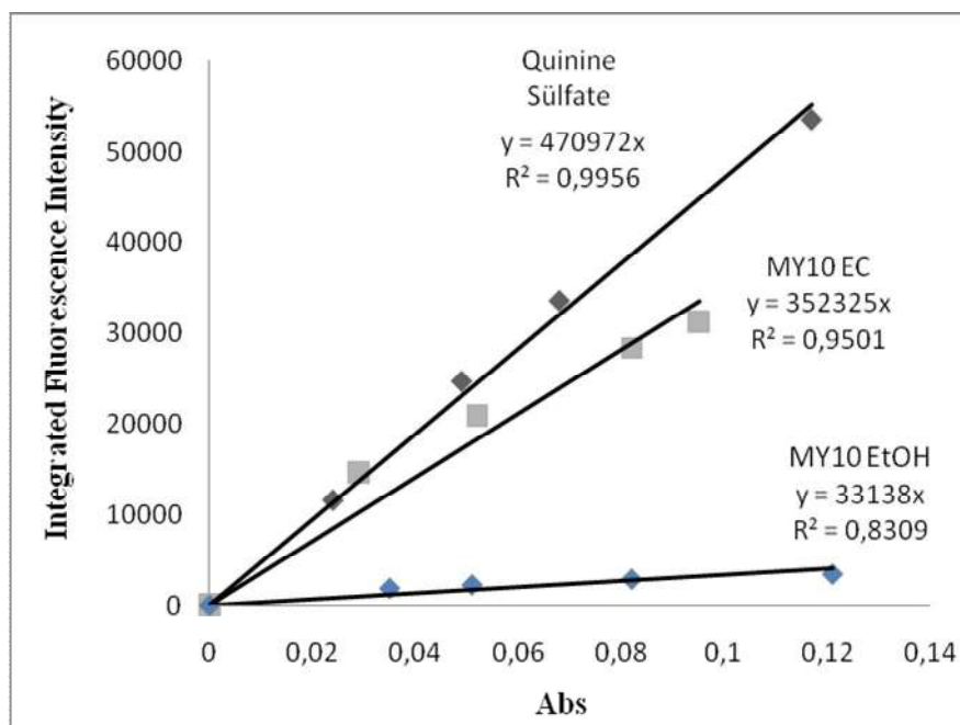
Figure 6.7 The integrated fluorescence intensities vs absorbance for the reference standard; quinine sulphate in \text{H}_2\text{SO}_4 , MY10 dye in EC and EtOH matrices.
