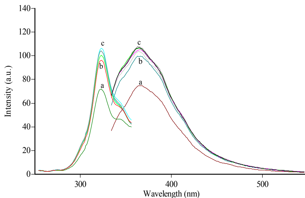
Figure 7.16 pH induced emission based spectral response of the EC doped MY2 in the pH range of 7.00-10.00. pH: a) 7.00 b) 7.50 c) 8.00, 8.50, 9.00, 9.50, 10.00.
