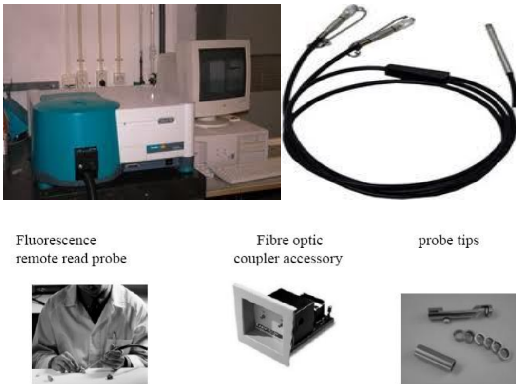
Figure 4.1 Varian Cary Eclipse Spectrofluorometer, fiber optic probe and fiber optical system accessories.
