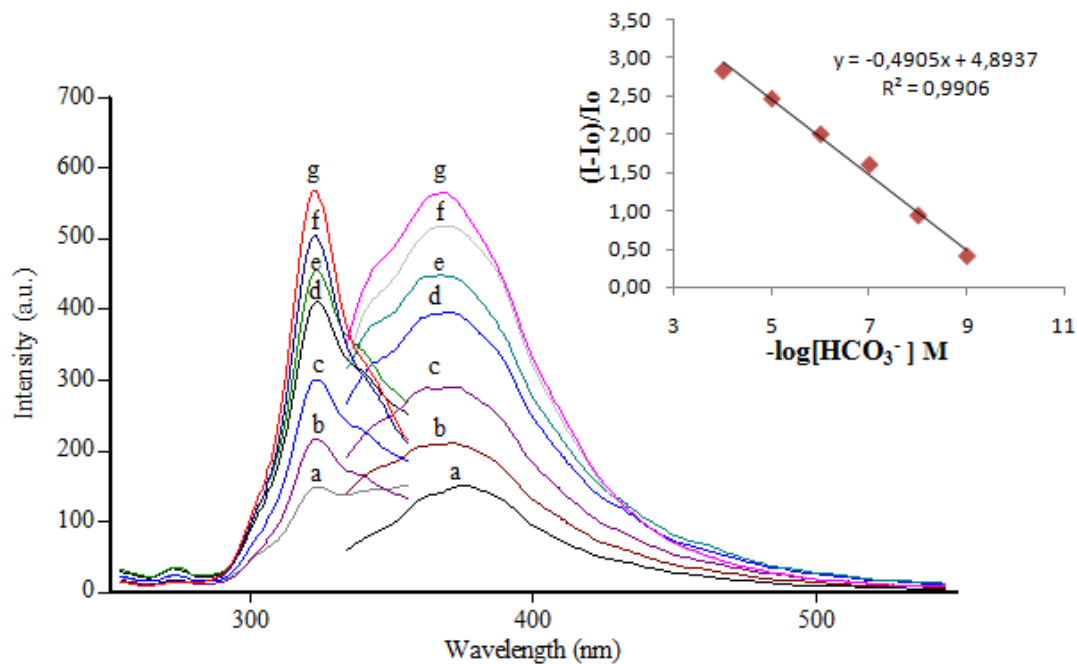
Figure 7.30 Emission spectra of immobilized MY5 in EC based nanofibers after exposure to different \text{HCO}_3^- concentrations; (a) bicarbonate free water (b) 1.00 \times 10^{-9} \text{ M} (c) 1.00 \times 10^{-8} \text{ M} (d) 1.00 \times 10^{-7} \text{ M} (e) 1.00 \times 10^{-6} \text{ M} (f) 1.00 \times 10^{-5} \text{ M} (g) 1.00 \times 10^{-4} \text{ M} .
