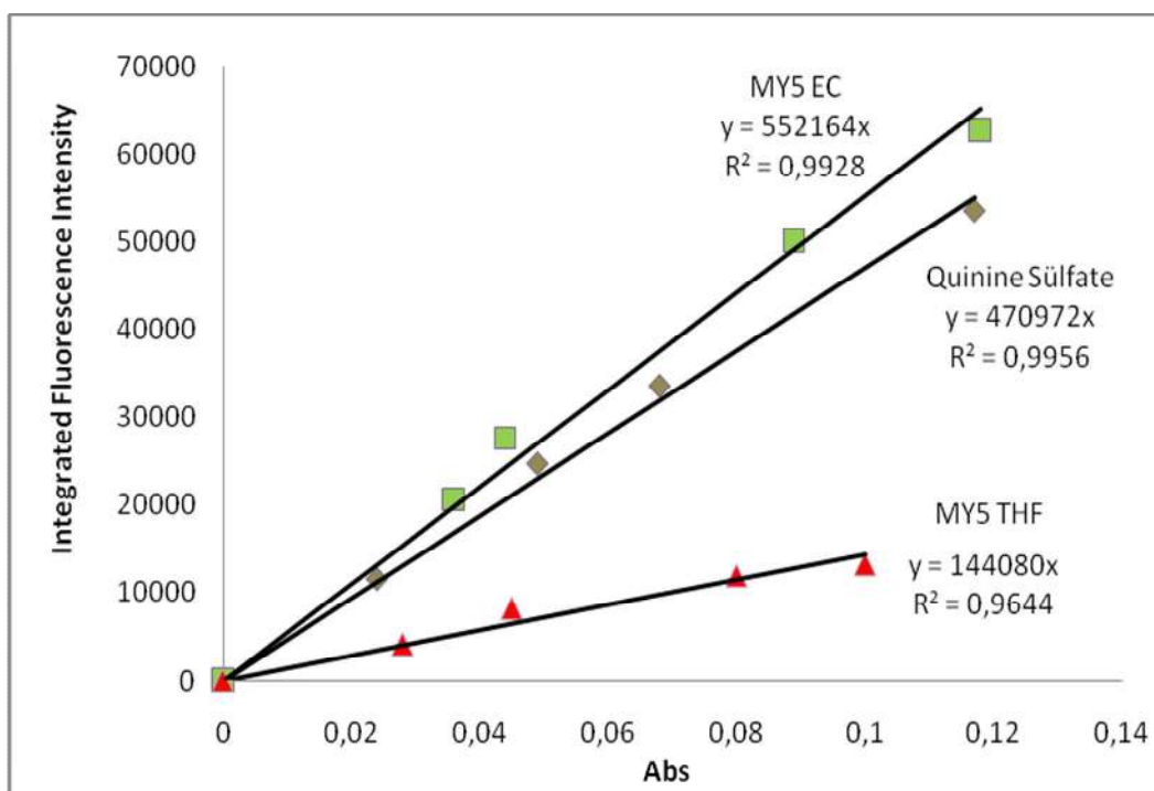
Figure 7.10 The integrated fluorescence intensities vs absorbance for the reference standard; quinine sulphate in \text{H}_2\text{SO}_4 , MY5 dye in EC and THF matrices.
