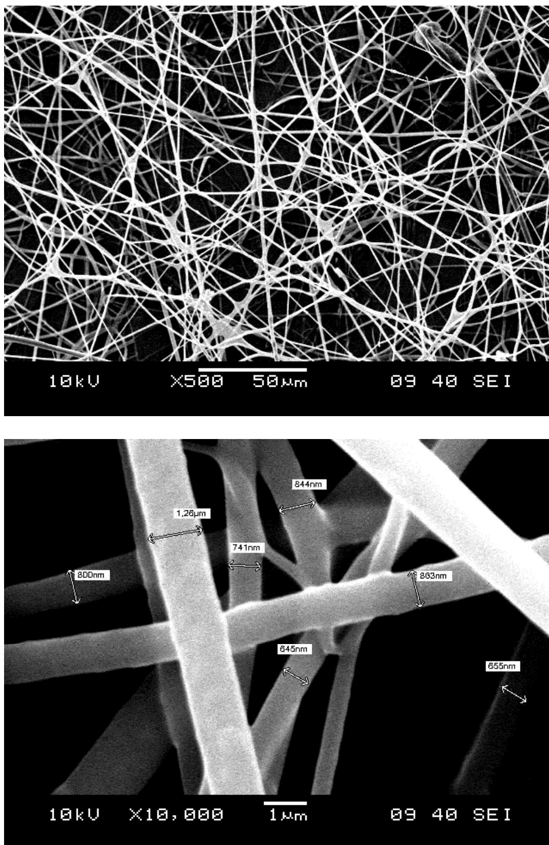
Figure 7.26 SEM images of EC based electrospun nanofibers for MY4 dye at different magnifications such as \times 500 and \times 10\,000 .
