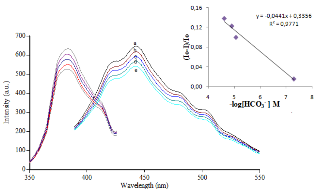
Figure 6.25 Emission spectra of immobilized MY9 in EC based nanofibers after exposure to different \text{HCO}_3^- concentrations; (a) bicarbonate free water (b) 5.00 \times 10^{-8} \text{ M} (c) 8.50 \times 10^{-6} \text{ M} (d) 1.24 \times 10^{-5} \text{ M} (e) 2.42 \times 10^{-5} \text{ M} .
