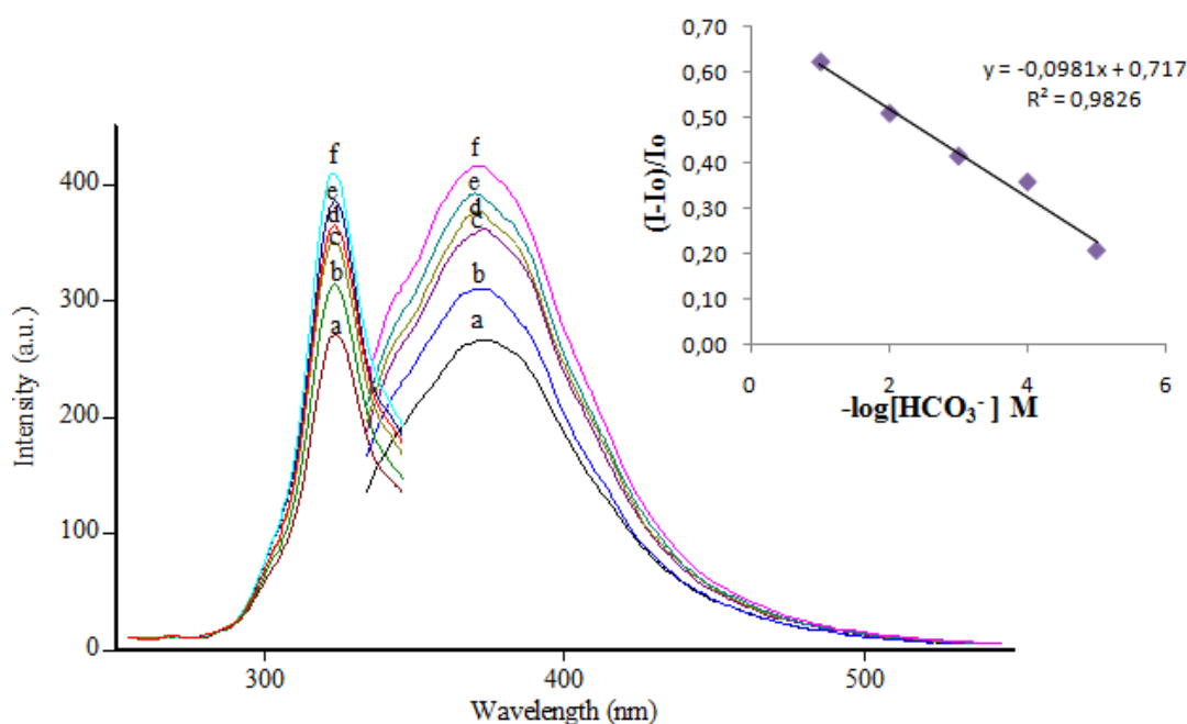
Figure 7.24 Emission spectra of immobilized MY5 in EC based thin film matrix after exposure to different \text{HCO}_3^- concentrations; (a) bicarbonate free water (b) 1.00 \times 10^{-5} \text{ M} (c) 1.00 \times 10^{-4} \text{ M} (d) 1.00 \times 10^{-3} \text{ M} (e) 1.00 \times 10^{-2} \text{ M} (f) 1.00 \times 10^{-1} \text{ M} .
