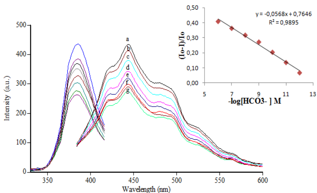
Figure 6.27 Emission spectra of immobilized MY9 in PMMA based nanofibers matrix after exposure to different \text{HCO}_3^- concentrations; (a) bicarbonate free water (b) 1.00 \times 10^{-12} \text{ M} (c) 1.00 \times 10^{-11} \text{ M} (d) 1.00 \times 10^{-10} \text{ M} (e) 1.00 \times 10^{-9} \text{ M} (f) 1.00 \times 10^{-8} \text{ M} (g) 1.00 \times 10^{-7} ; 1.00 \times 10^{-6} \text{ M} .
