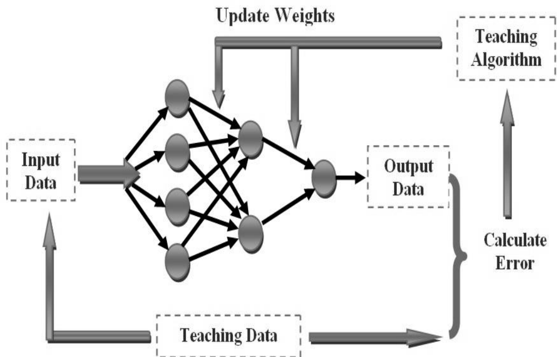
Figure 23: Classification with artifitial nural network
