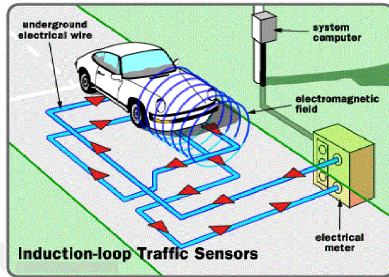
Figure 2.4. Inductive loop detection [14]
