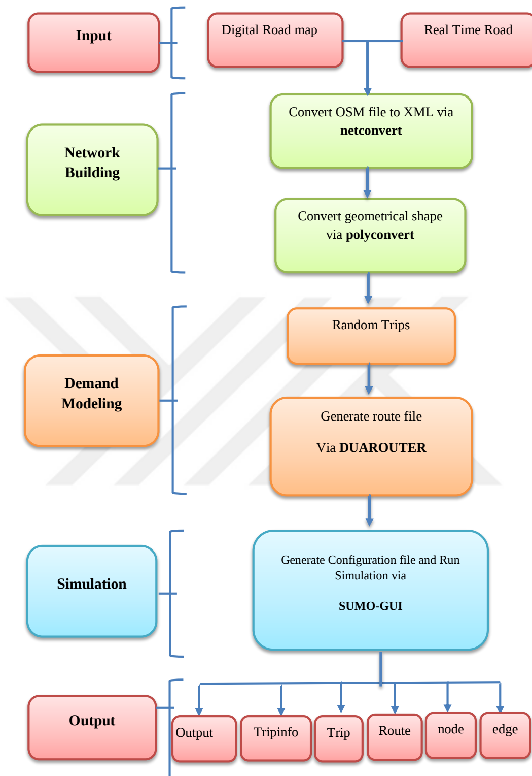
Figure 4.2. The SUMO architecture
