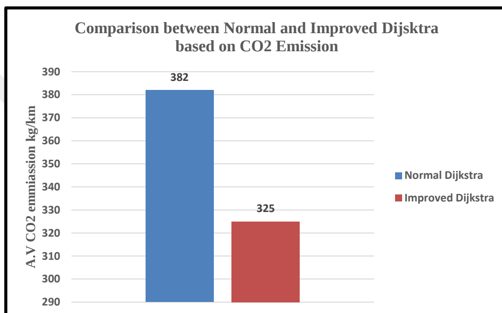
Figure 4.13. Comparison between normal and improved Dijkstra based on CO 2 emission
