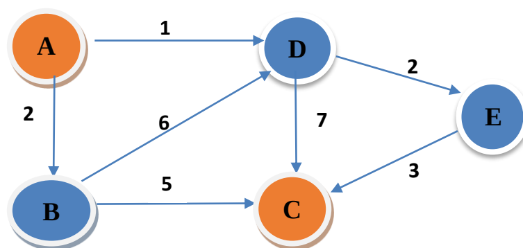
Figure 2.11. Dijkstra example [54]
