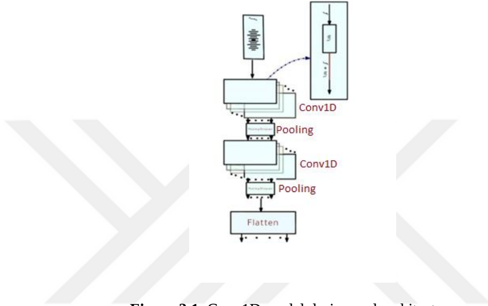
Figure 3.1. Conv1D model design and architecture
