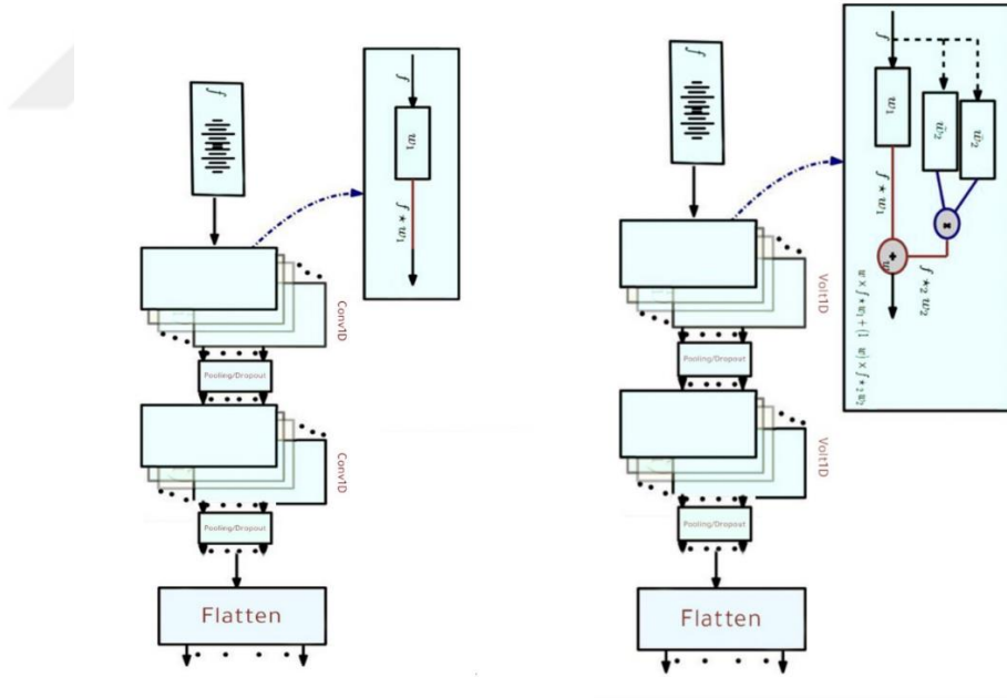
Figure 4.2. Difference between the Conv1D and Volt1D
