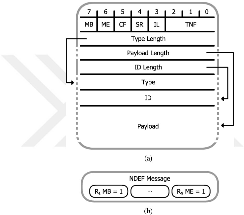
Figure 7: NDEF Message Format [30]
