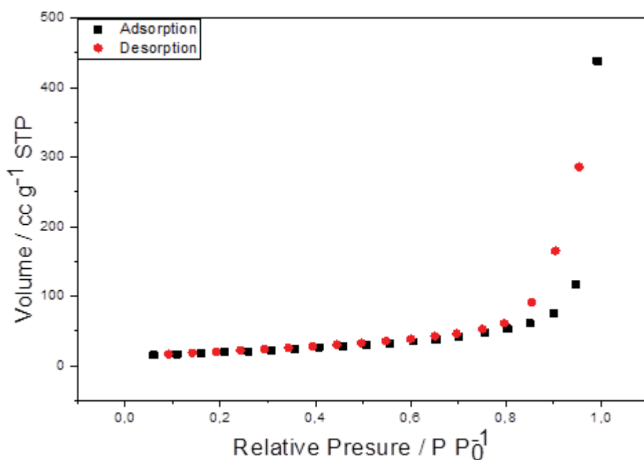
Figure 3.5. BET isotherm of NiZnO nanoparticles
