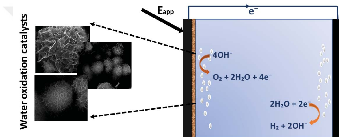
Figure 1.6. Schematic representation of electrochemical water oxidation
