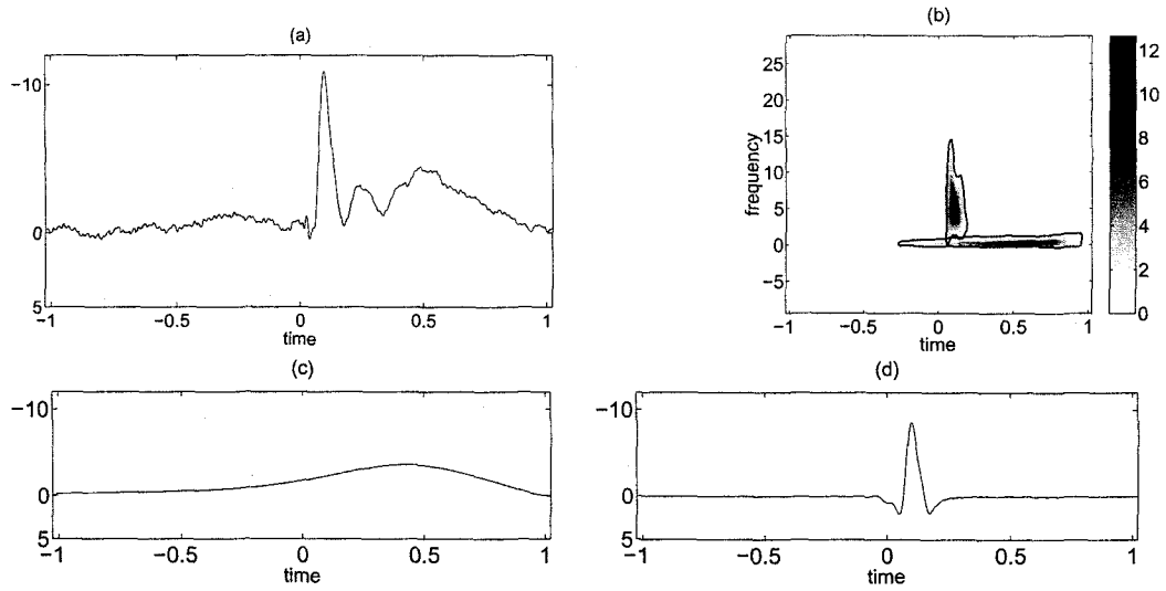
Figure 5.14: Original ERP signal (a), time–frequency representation obtained by TFCA (b) and estimated individual time–domain components (c) and (d) for the ensemble target average under MMN paradigm.
