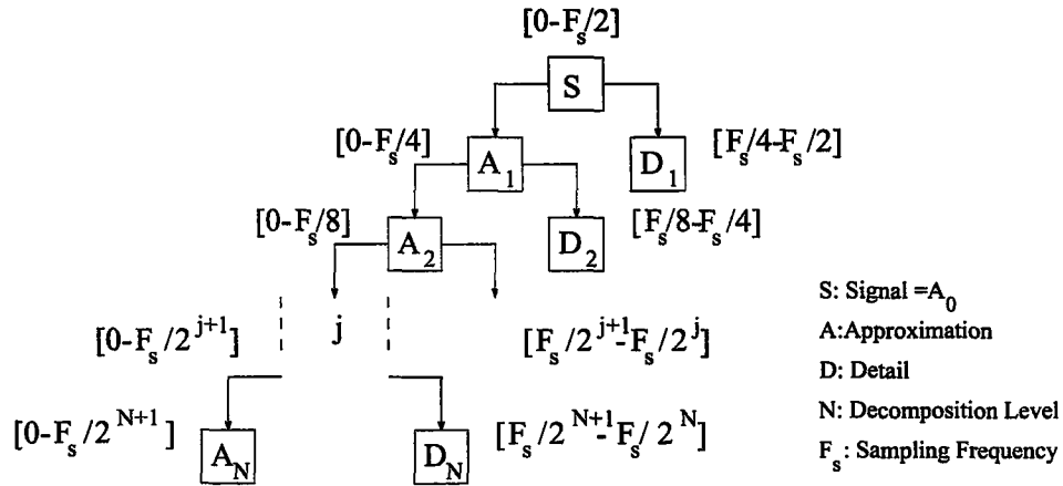
Figure 3.6: Successive decomposition of a signal into approximations and details.
