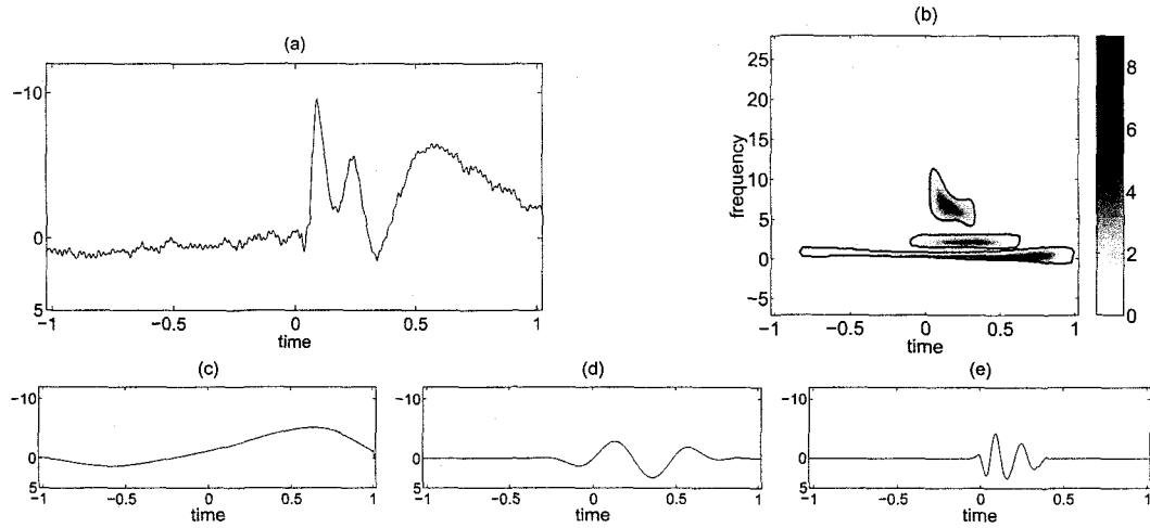
Figure 5.16: Original ERP signal (a), time-frequency representation obtained by TFCA (b) and estimated time-domain components (c), (d) and (e) for the ensemble target average under OB-HD paradigm.
