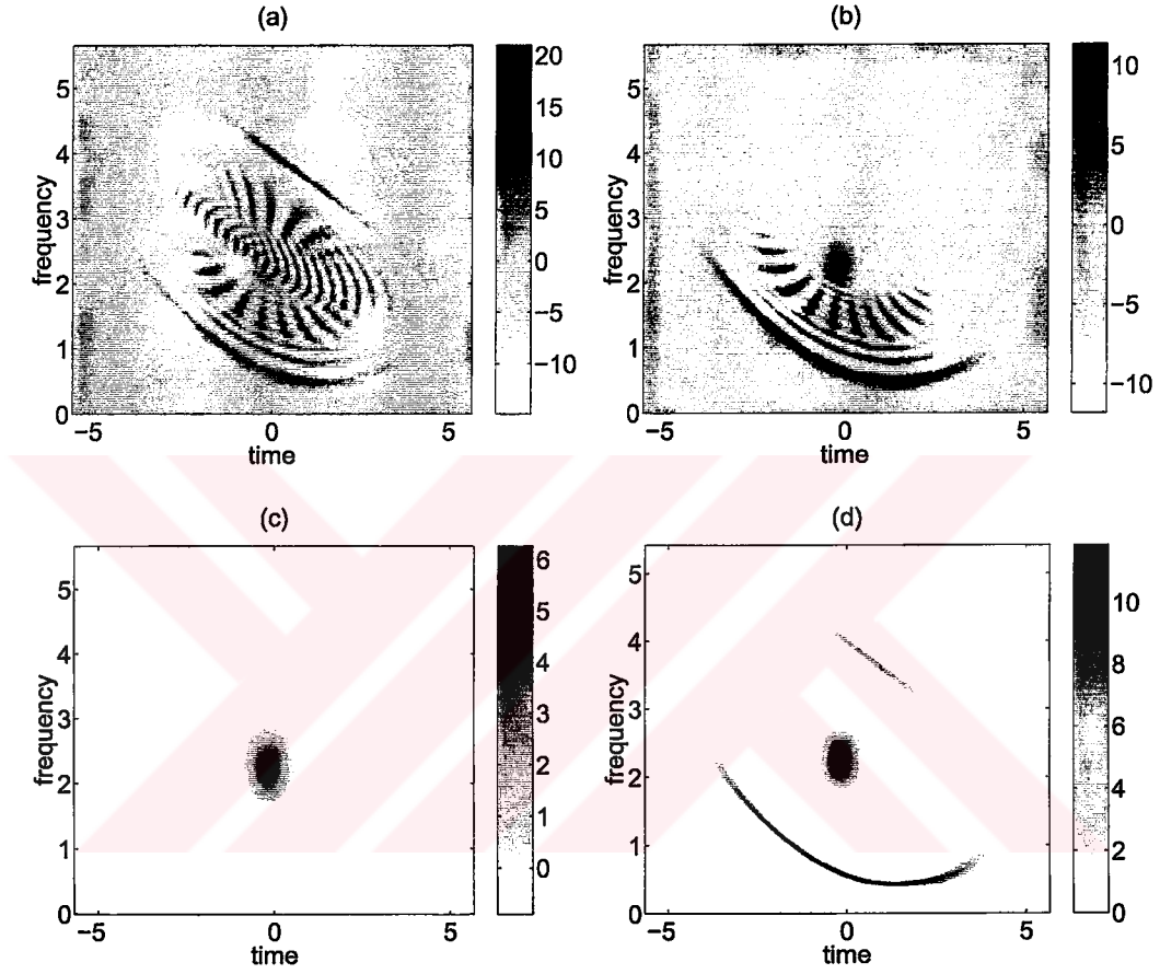
Figure 4.9: In the WD of the synthetic signal given in Fig. 4.8 (d), s_3(t) is immersed under cross-cross term interference. WD of the residual signals after the extraction of \hat{s}_1(t) and \hat{s}_2(t) are given in (b) and (c), respectively. TFCA provides high-resolution time-frequency distribution of the synthetic multi-component signal as shown in (d).
