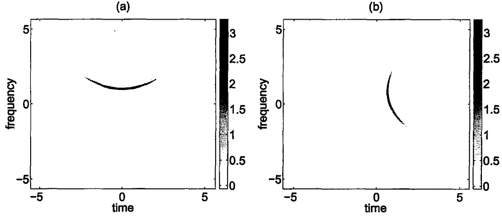
Figure 4.7: When the rotation effect of the FrFT is removed from the directionally smoothed WD given in (a) by rotating it -\pi/2 (76.5 degrees) radians clock-wise, the high resolution time-frequency distribution of the original signal given in (b) is obtained.
