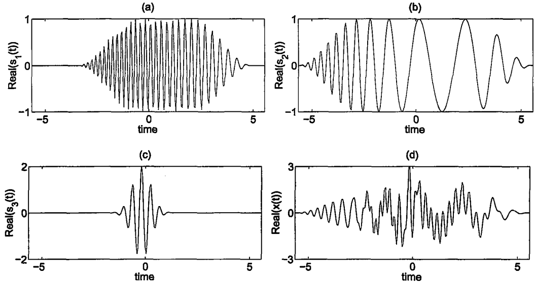
Figure 4.8: Synthetic signal x(t) = \sum_{i=1}^3 s_i(t) (d) used in the performance illustration of the TFCA is composed of a linear chirp (a), s_1(t) , a non-linear chirp (b), s_2(t) , and a constant frequency modulated signal (c), s_3(t) .
