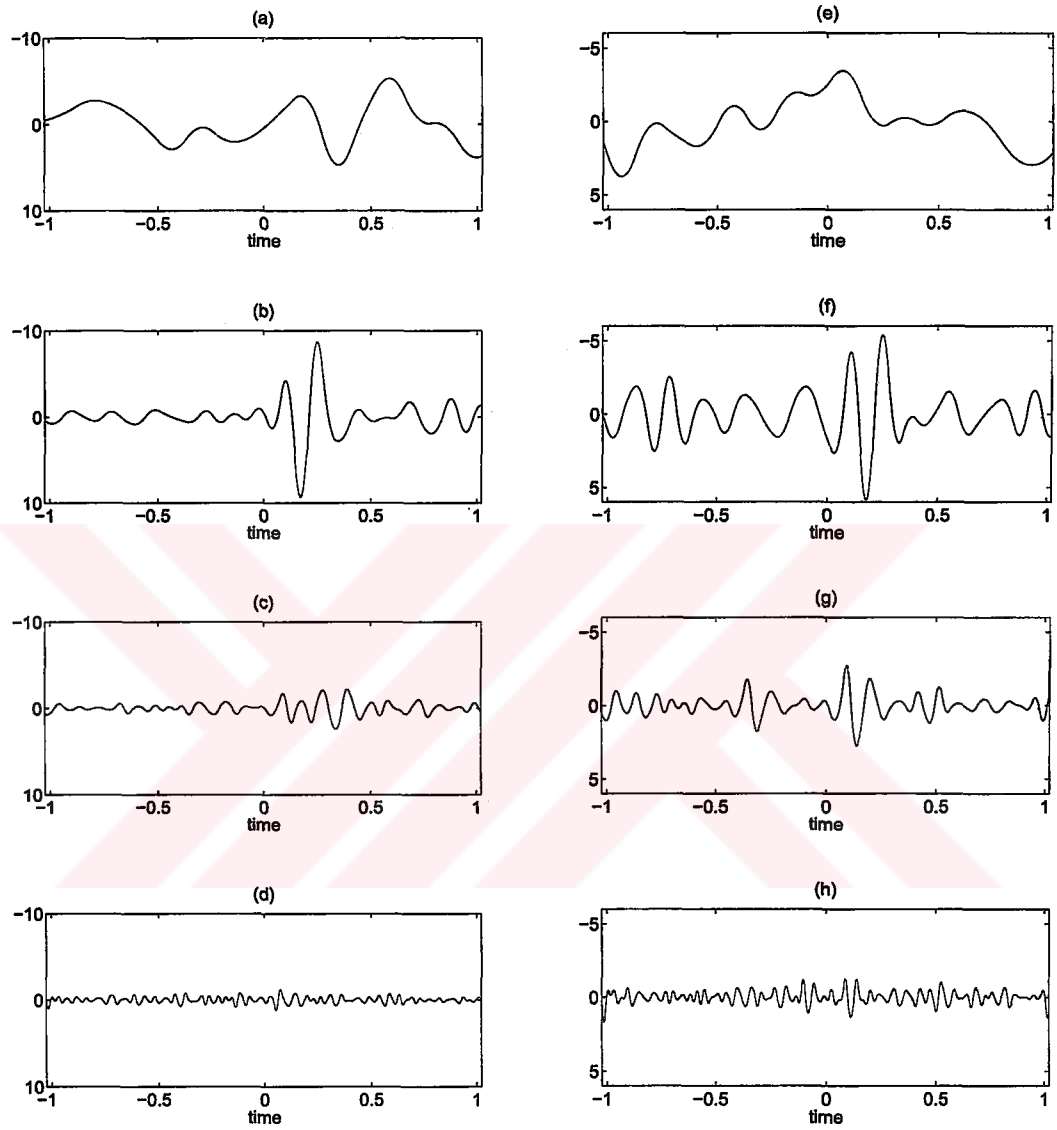
Figure 3.7: Quadratic B-spline wavelet based ERP signal analysis results for 'FEBE' target and nontarget frames. Delta, theta, alpha and beta signals in the approximate frequency bands given in Table 3.4 are reconstructed for both the target ( shown in (a), (b), (c), (d) ) and nontarget frames ( shown in (e), (f), (g), (h) ), respectively.
