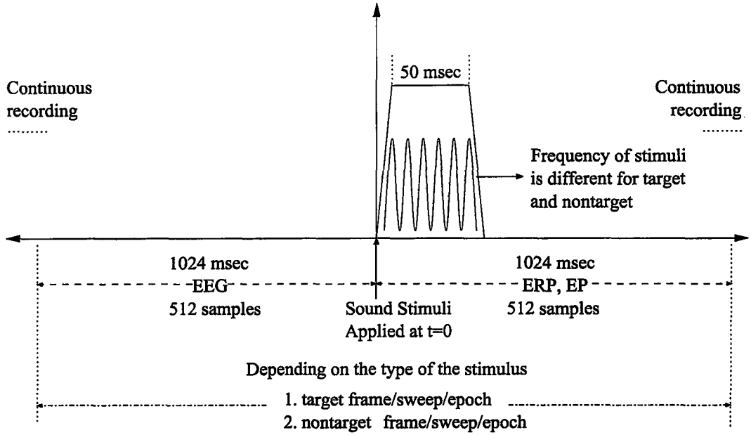
Figure 2.2: Data acquisition scheme of the EEG-ERP signals.
