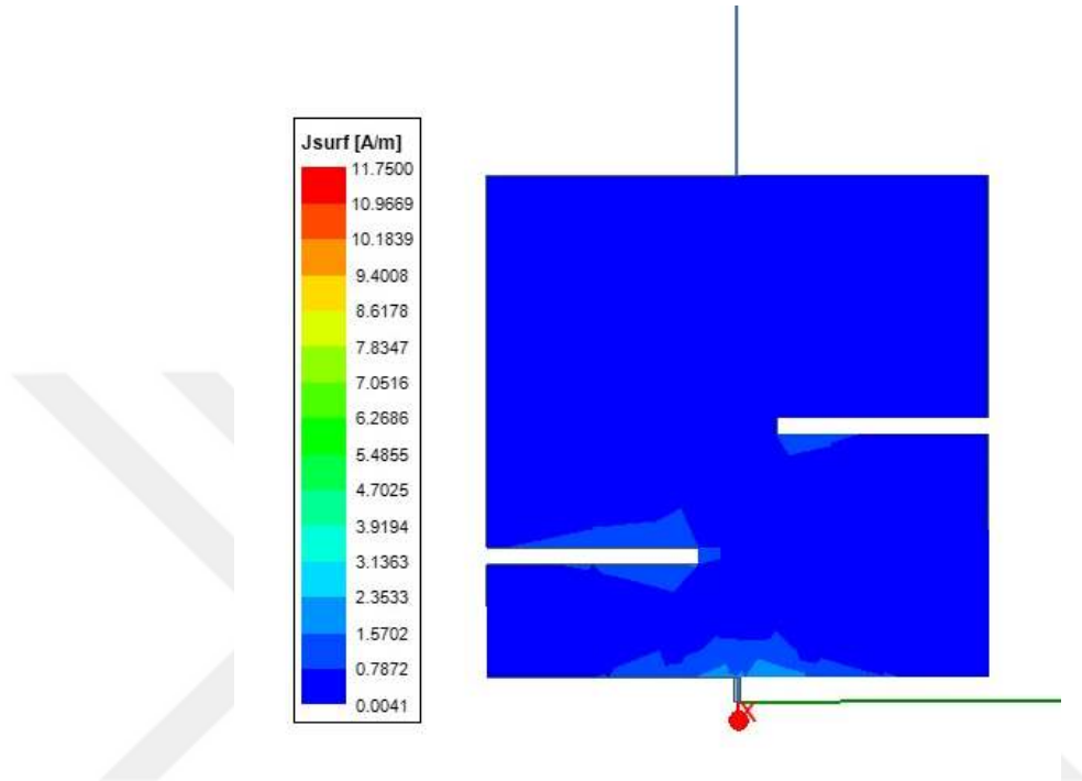
Figure 2. 12 The surface current distribution of the two notches
