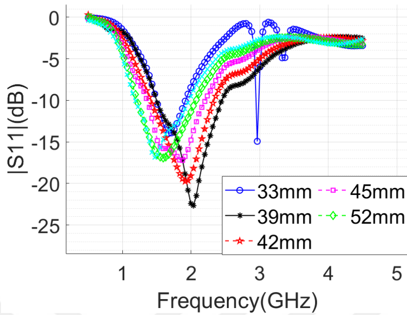
Figure 2. 19 Comparison of Notched Square Monopole Antenna
