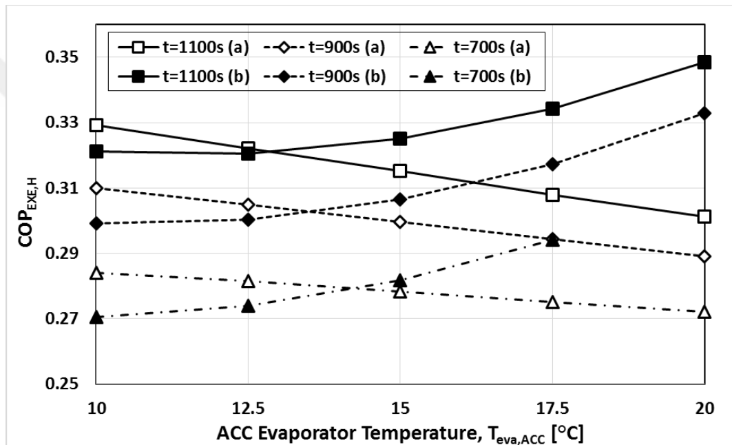
Figure 4. 22. Comparisons of the variation of \text{COP}_{\text{EXE,H}} with respect to ACC evaporator temperature for three different cycle times and the two system configurations (a) and (b).
