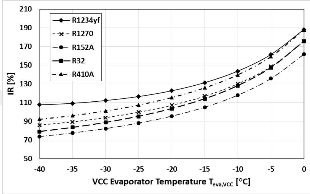
Figure 4. 9. Comparisons of the variation of IR with respect to VCC evaporator temperatures when VCC system works with ACC and alone for different refrigerants.
