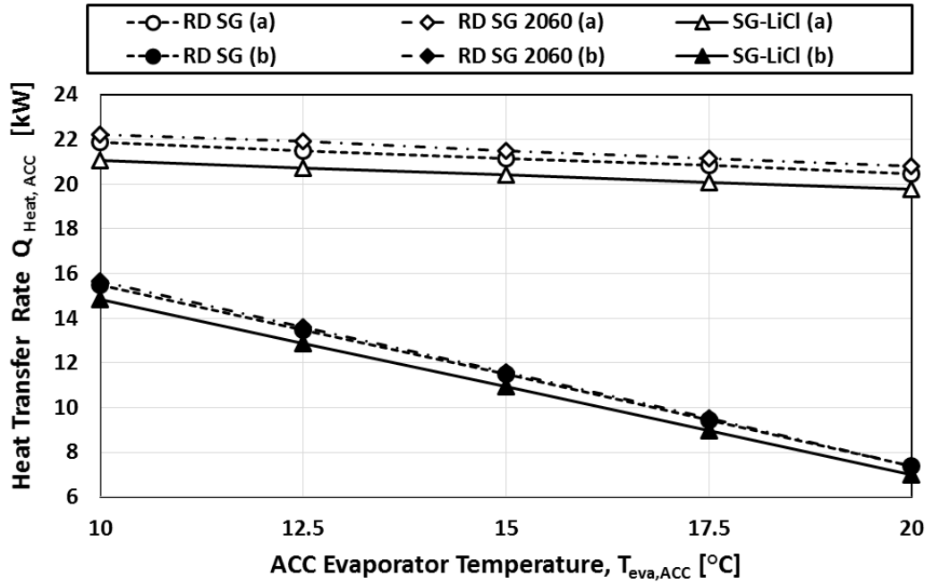
Figure 4. 15. Comparisons of the variation of \dot{Q}_{heat,ACC} with respect to ACC evaporator temperature for different adsorbents and the two system configurations (a) and (b).
