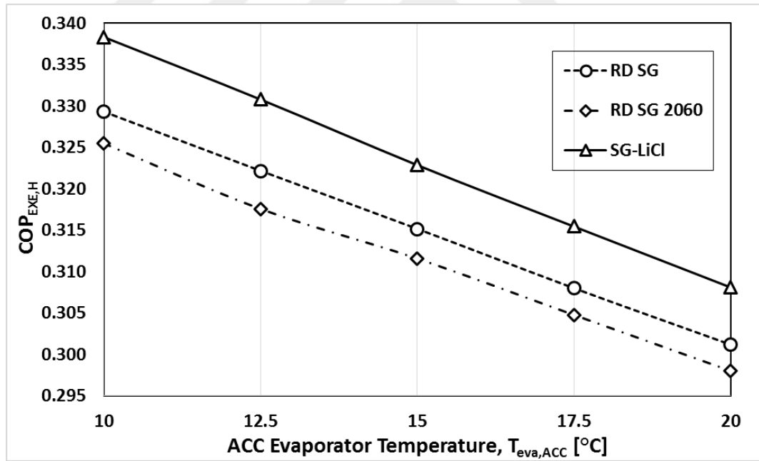
Figure 4. 17. Comparisons of the variation of COP_{EXE,H} with respect to ACC evaporator temperature for various adsorbents and the series configuration (a).
