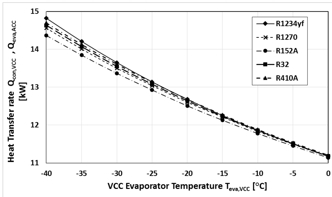
Figure 4. 3. Comparisons of the variation of heat transfer rates in the intermediate heat exchanger with respect to VCC evaporator temperature for the various refrigerants.
