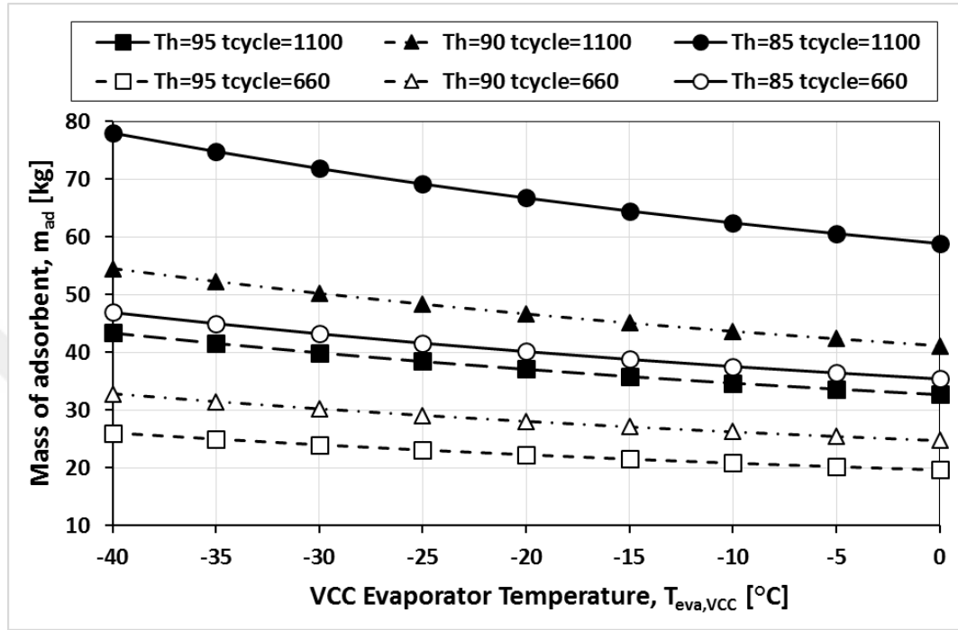
Figure 4. 10. Required amount of mass in a bed with respect to VCC evaporator temperatures, heating temperatures, and two different cycle time values.
