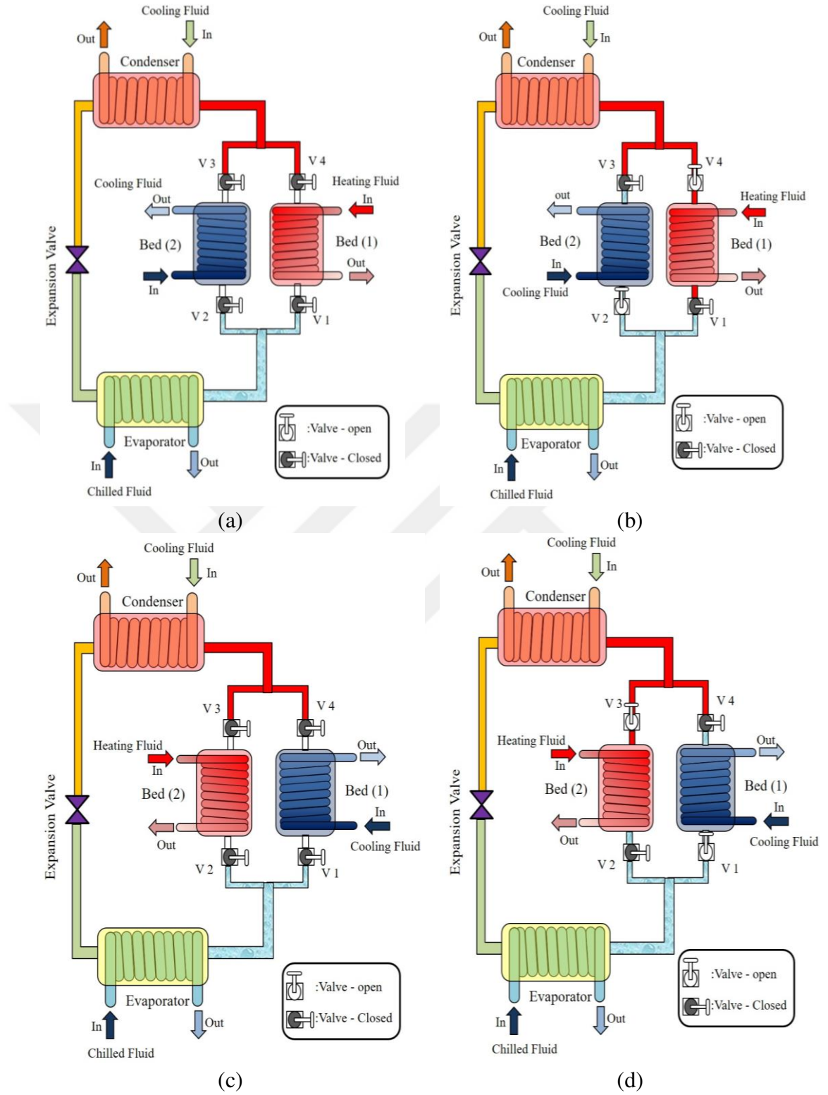
Figure 2. 5. Schematic of the single-stage adsorption cooling unite modes (a, b, c, d).
