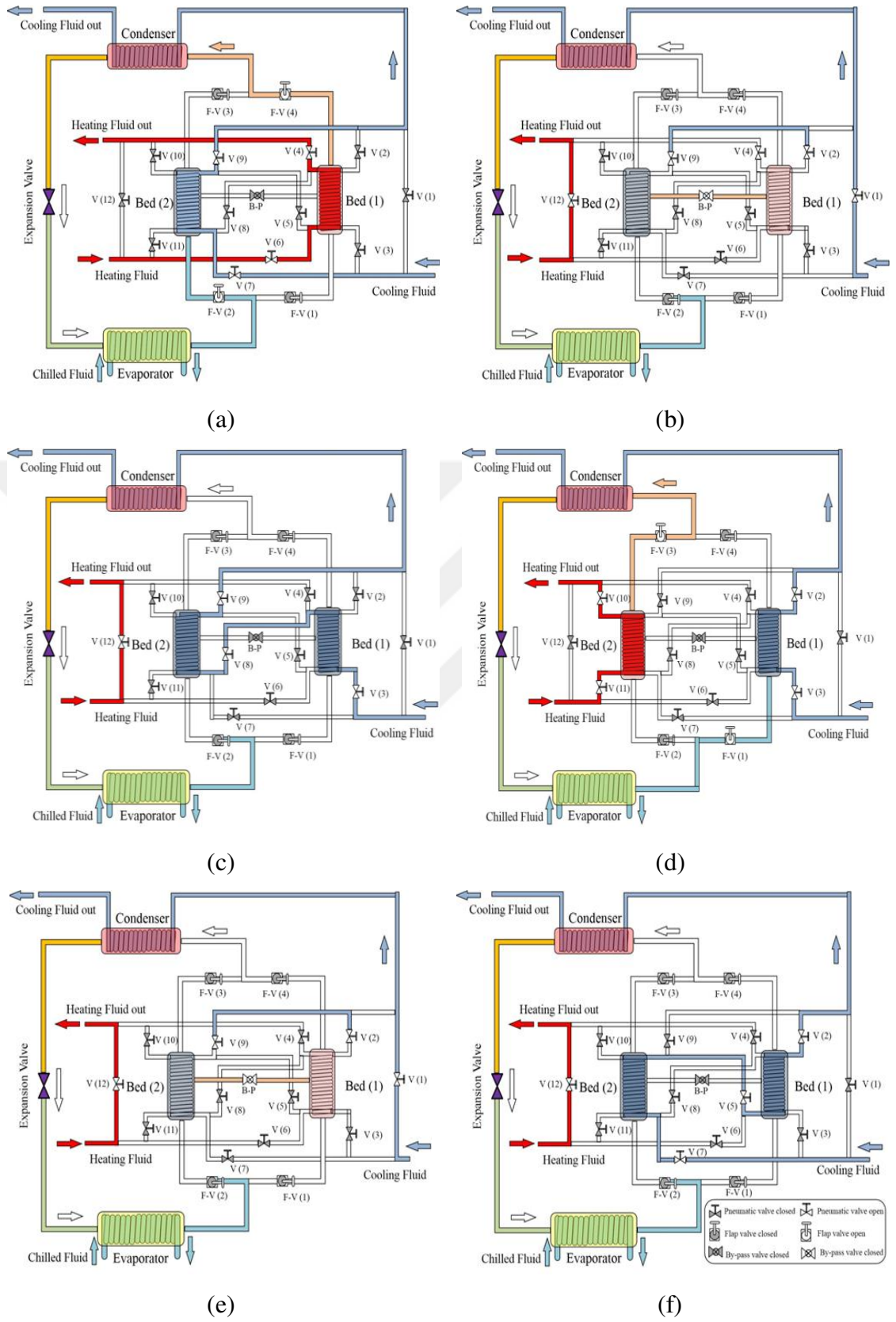
Figure 2. 8. The operating modes of the adsorption cooling system.
