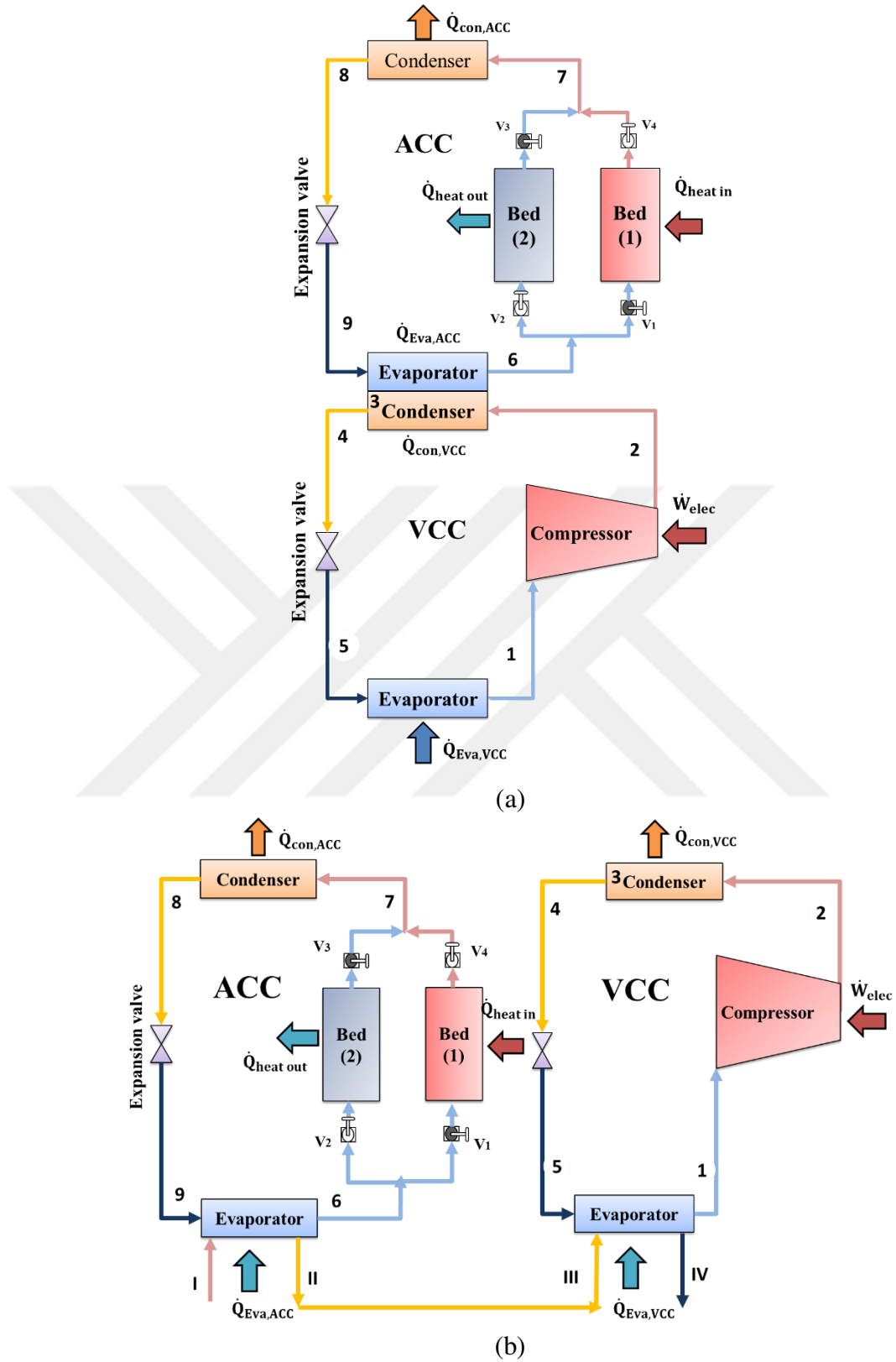
Figure 2. 12. Schematic of (ACC-VCC) combined chiller: (a) series connection, (b) parallel connection.
