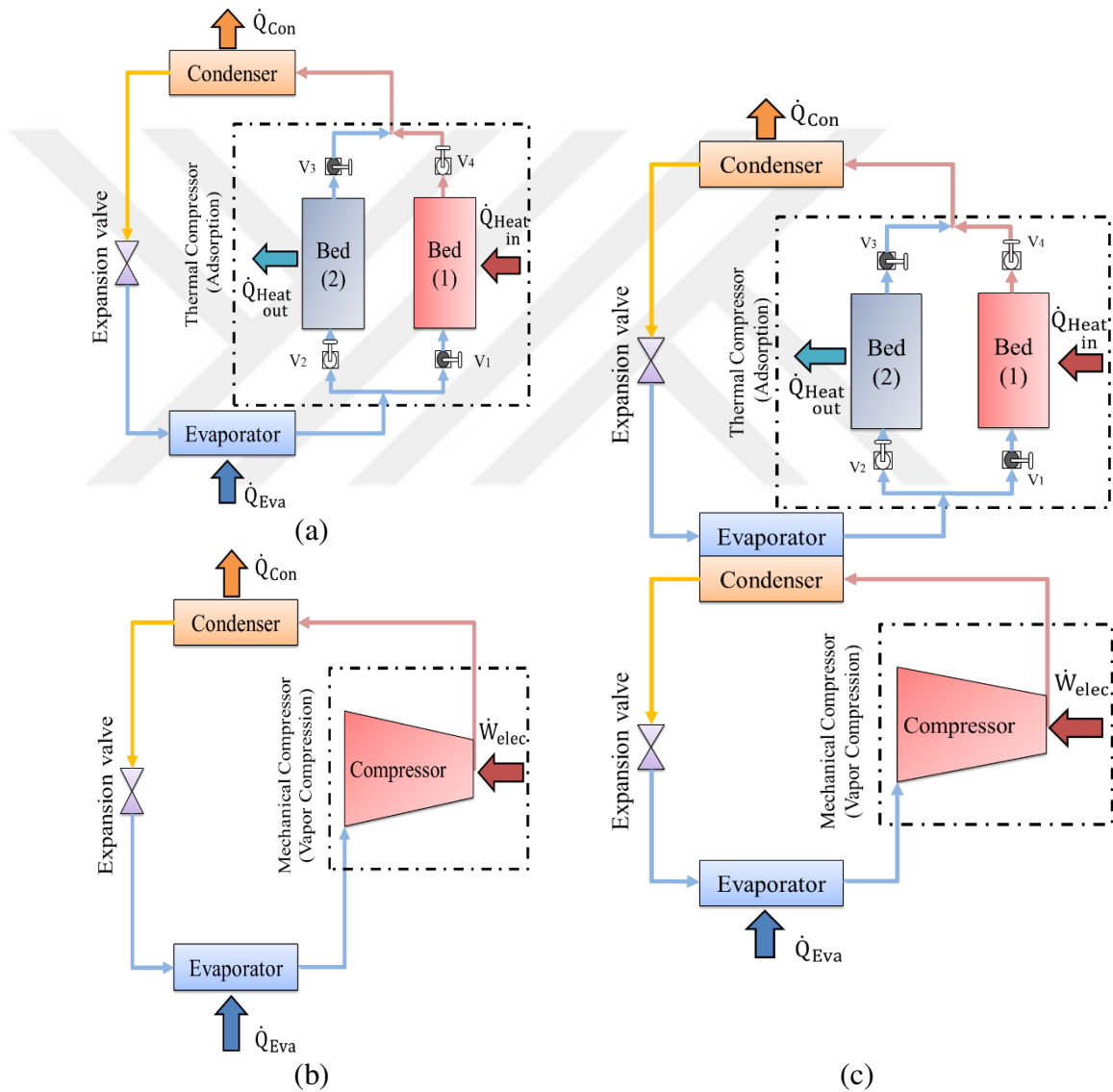
Figure 2. 11. General schematic of (a) adsorption cooling system (ACC), (b) vapor compression cooling system (VCC), (c) ACC-VCC combined cooling system.
