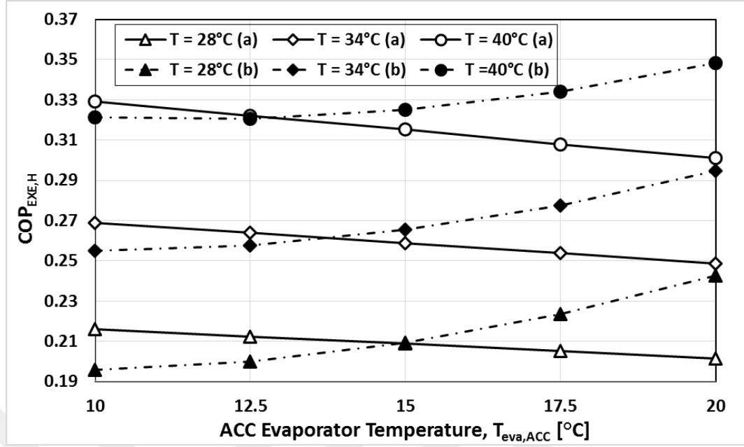
Figure 4. 23. Comparisons of the variation of COP_{EXE,H} with respect to ACC evaporator temperature for three different ambient temperatures and the configurations (a) and (b).
