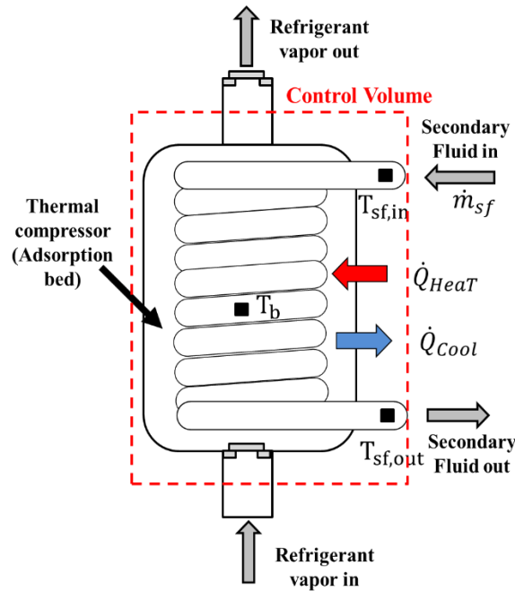
Figure 3. 1. Schematic design of the thermal compressor basic components.
