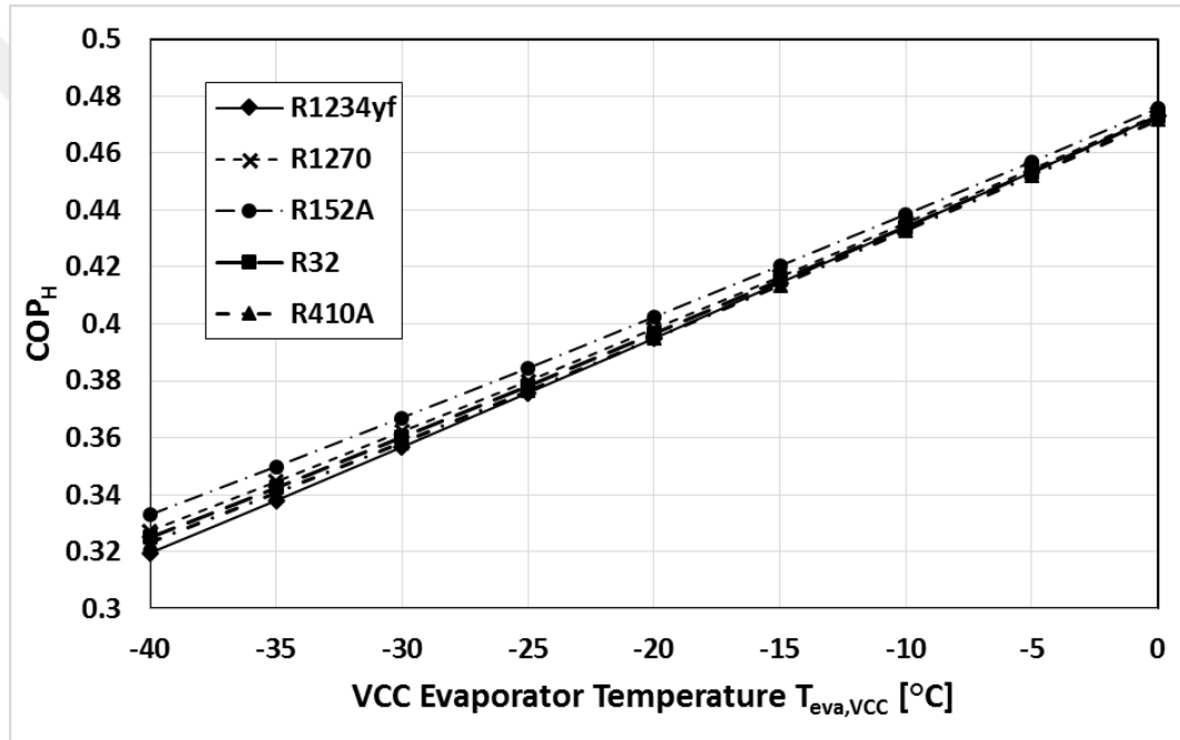
Figure 4. 6. Comparisons of the variation of COP_H with respect to VCC evaporator temperatures for various refrigerants.
