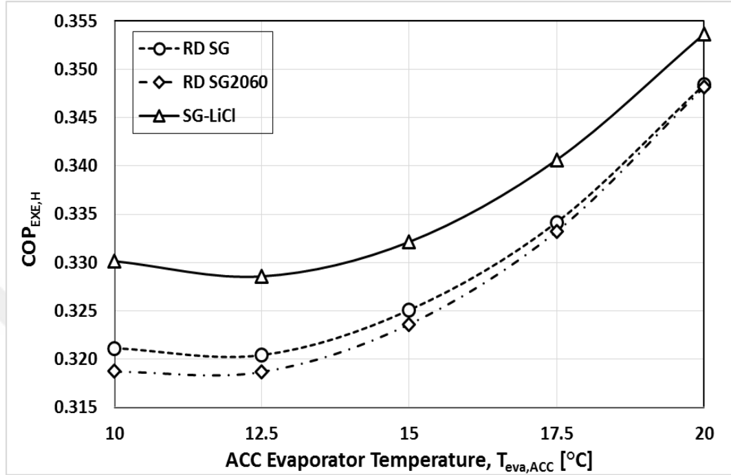
Figure 4. 18. Comparisons of the variation of \text{COP}_{\text{EXE,H}} with respect to ACC evaporator temperature for various adsorbents and the parallel configuration (b).
