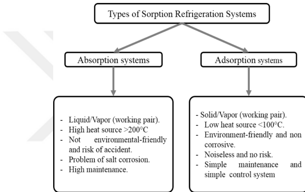
Figure 2. 9. Types of sorption refrigeration systems.
