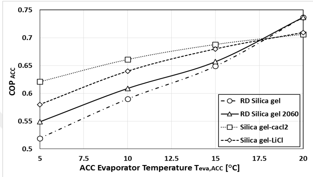
Figure 4. 11. Comparison of the variation of COP ACC with respect to ACC evaporator temperatures for different adsorbents.
