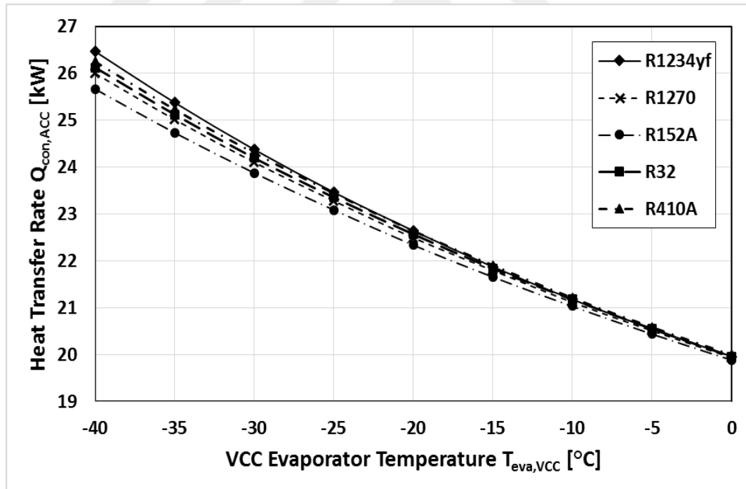
Figure 4. 4. Comparisons of the variation of heat transfer rate in the ACC condenser with respect to VCC evaporator temperature for different refrigerants.
