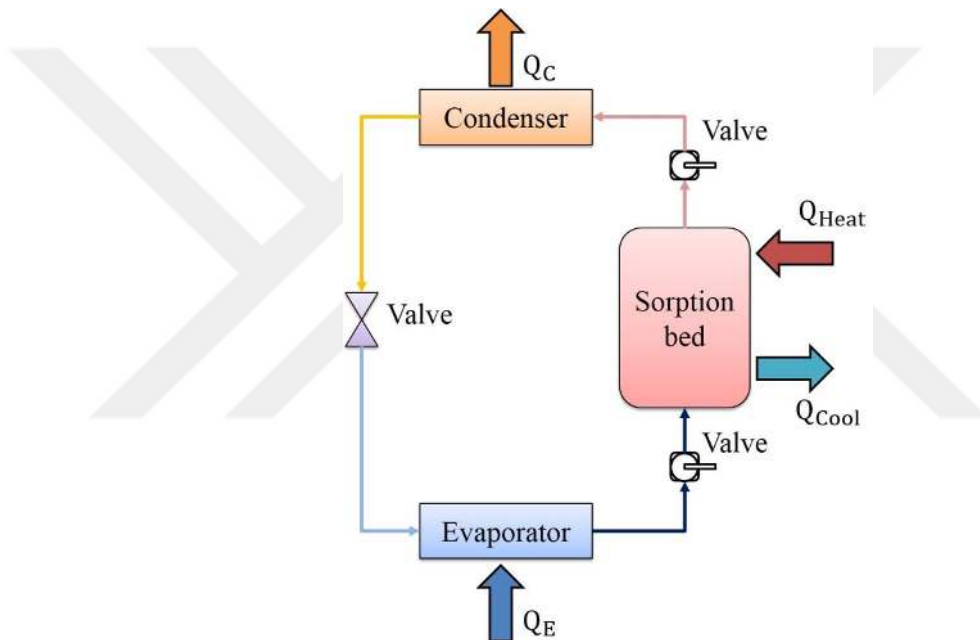
Figure 2. 3. A basic adsorption cooling system.
