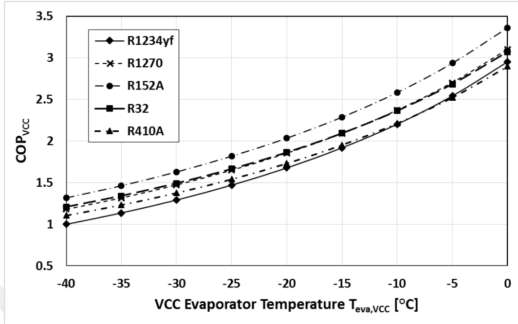
Figure 4. 2. Comparisons of the variation of COP_{VCC} with respect to VCC evaporator temperature for different refrigerants.
