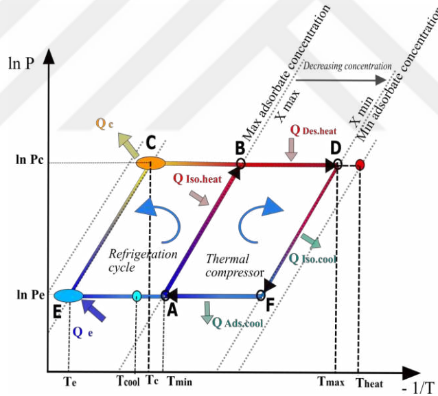
Figure 2. 4. Fundamental adsorption thermodynamic cycle for adsorption cooling cycle (Kilic & Anjrini, 2020).
