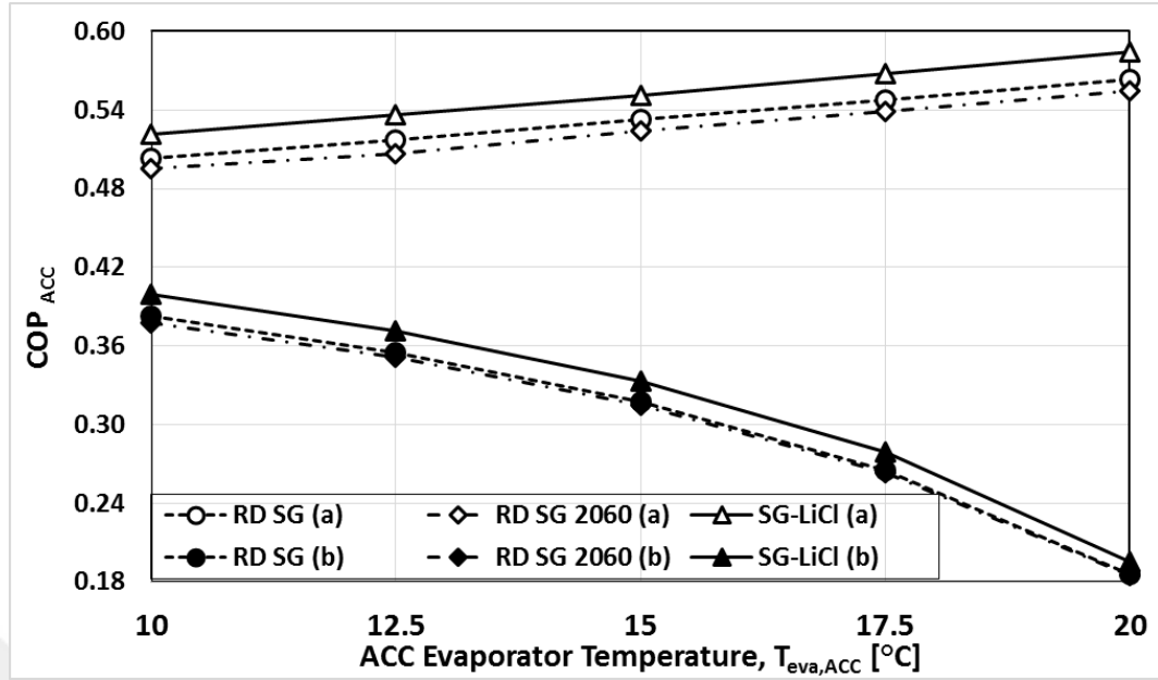
Figure 4. 19. Comparisons of the variation of COP_{ACC} with respect to ACC evaporator temperature for various adsorbents and the two system configurations series and parallel.
