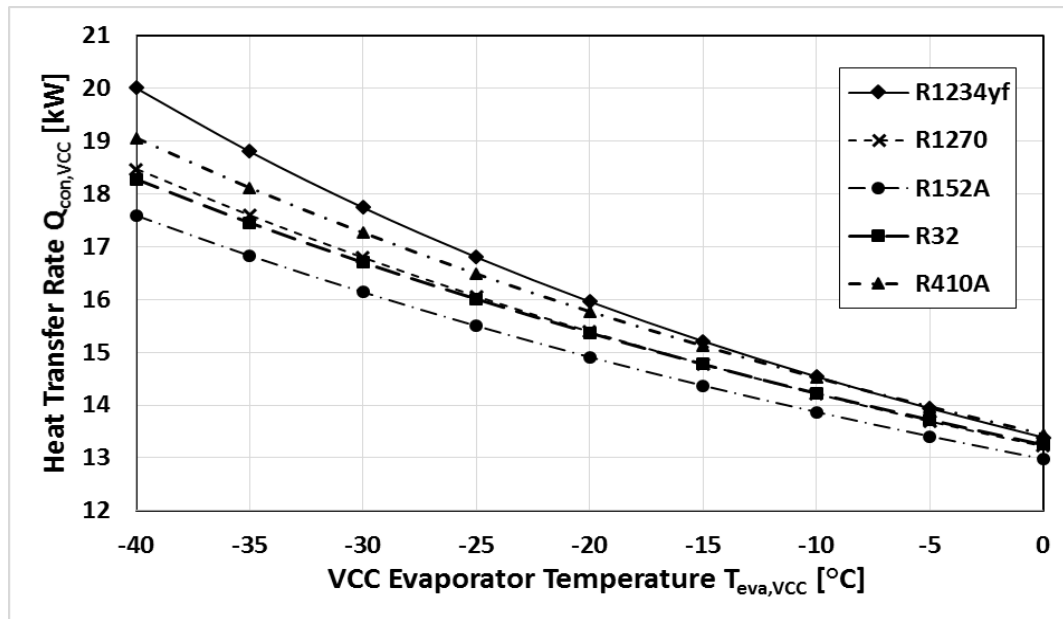
Figure 4. 1. Comparisons of the variation of heat transfer rate in the VCC condenser with respect to VCC evaporator temperature for various refrigerants.
