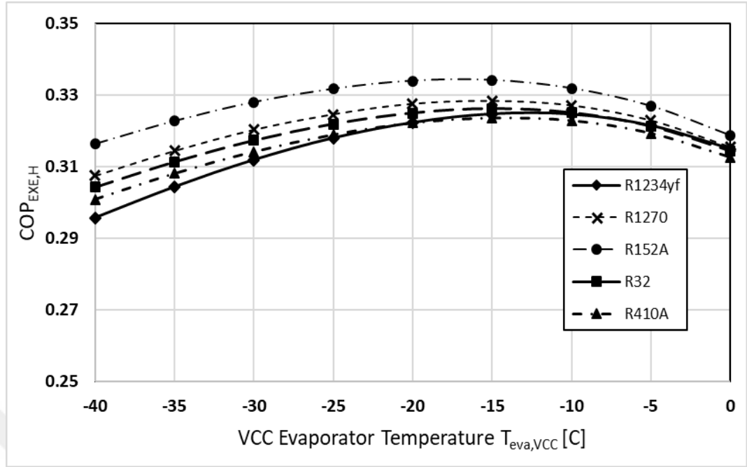
Figure 4. 7. Comparisons of the variation of COP_{EXE,H} with respect to VCC evaporation temperature for various refrigerants.
