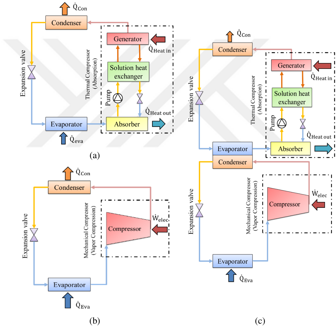
Figure 2. 10. General schematic of (a) absorption cooling system (ABC), (b) vapor compression cooling system (VCC), (c) ABC-VCC combined cooling system.
