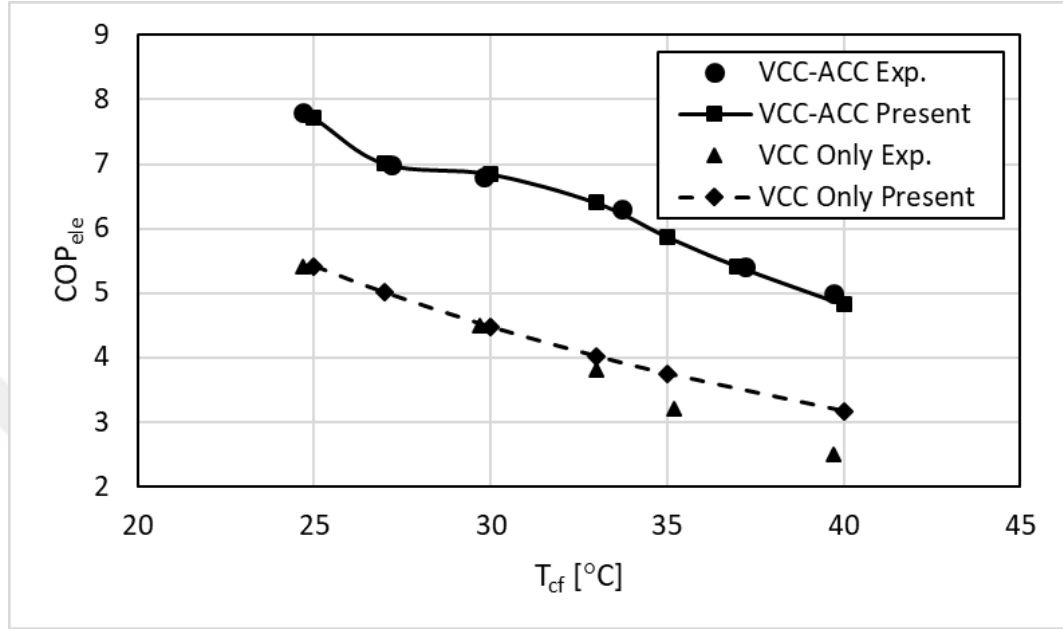
Figure 3. 3. Comparisons of COP_{VCC,H} and COP_{VCC} for different ambient air (cooling fluid) temperatures (Kilic & Anjrini, 2020).
