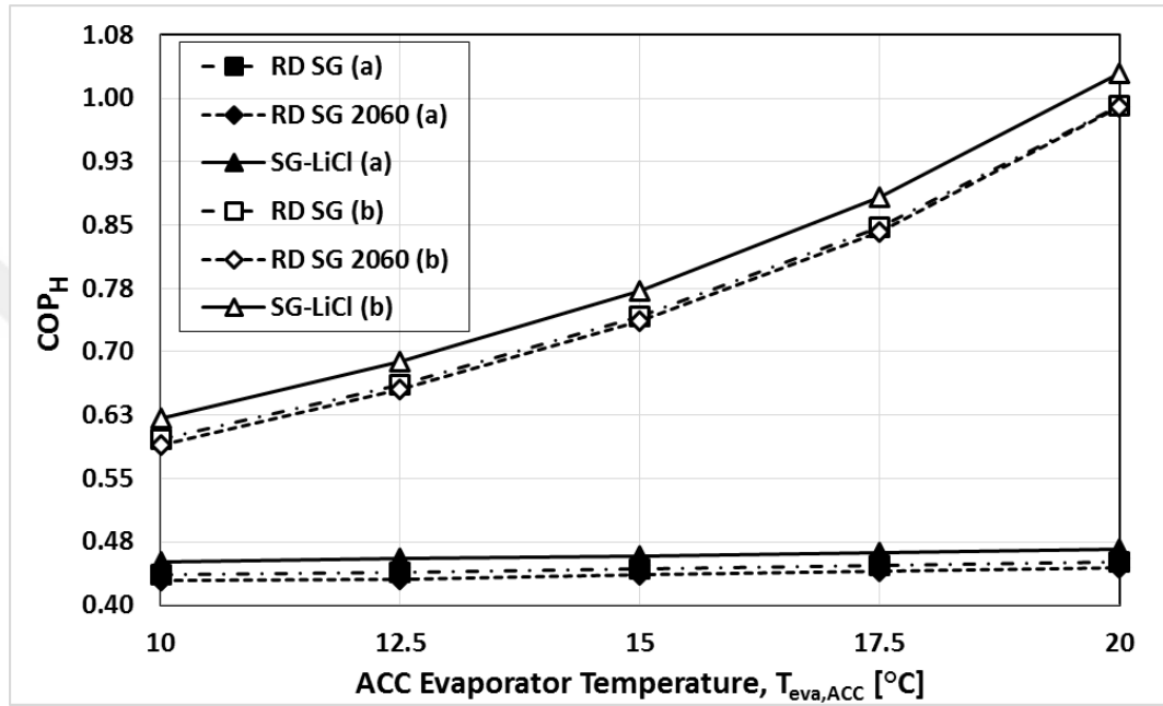
Figure 4. 16. Comparisons of the variation of COP_H with the respect to ACC evaporator temperature for various adsorbents and the two system configurations (a) and (b).
