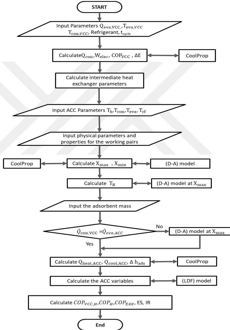
Figure 3. 2. Flow chart of calculating the mathematical model (Kilic & Anjrini, 2020)
