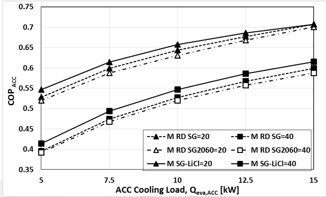
Figure 4. 21. Comparisons of the variaiton of COP_{ACC} with respect to ACC cooling load for different adsorbents and two different adsorbent mass values.
