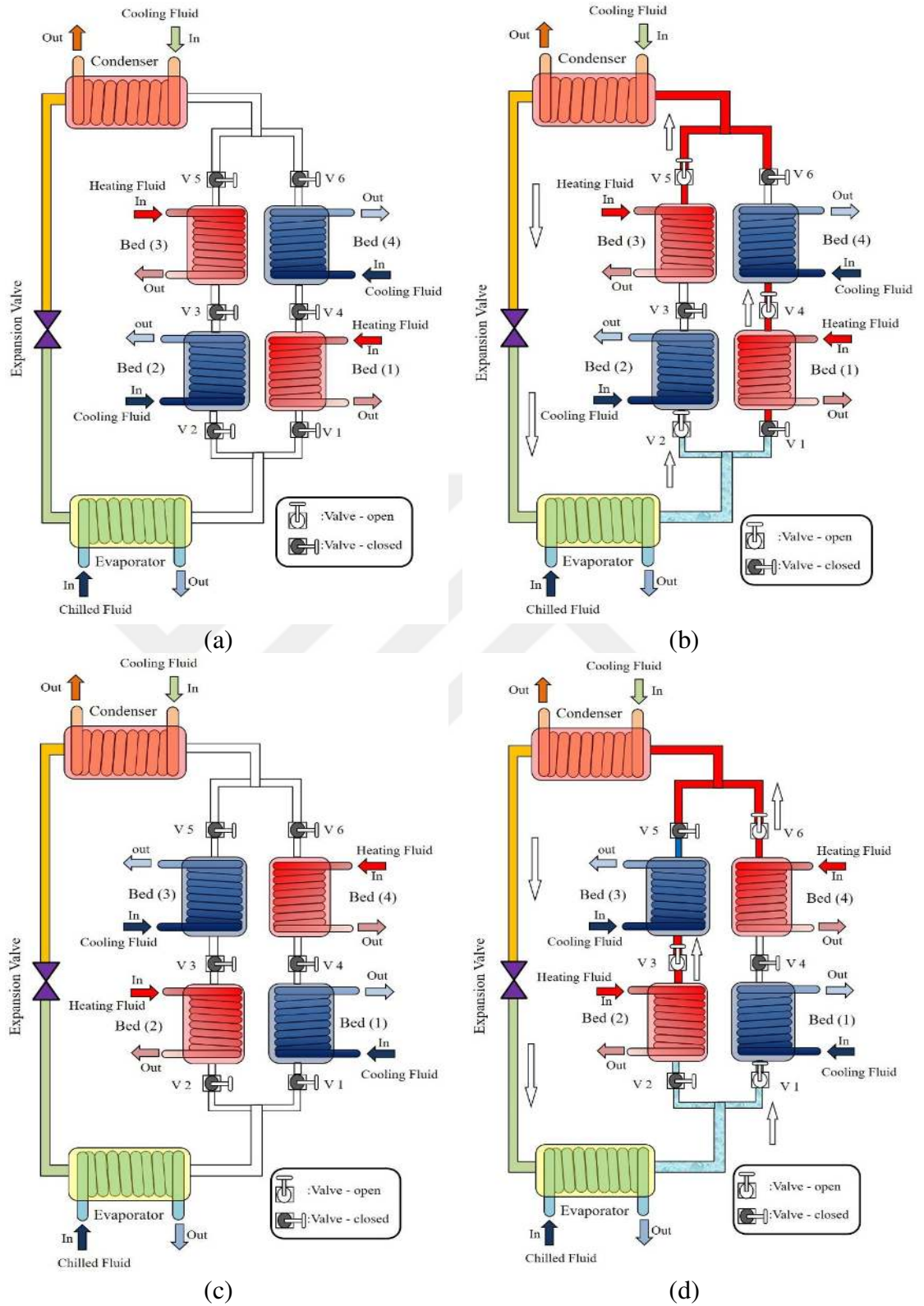
Figure 2. 6. Schematic of the two-stage adsorption cooling unite modes (a, b, c, d).
