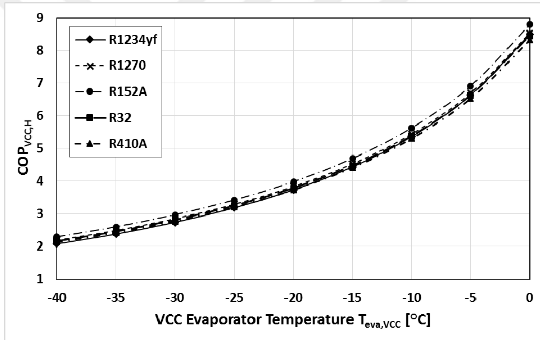
Figure 4. 5. Comparisons of the variation of COP_{VCC,H} with respect to VCC evaporator temperature for various refrigerants.
