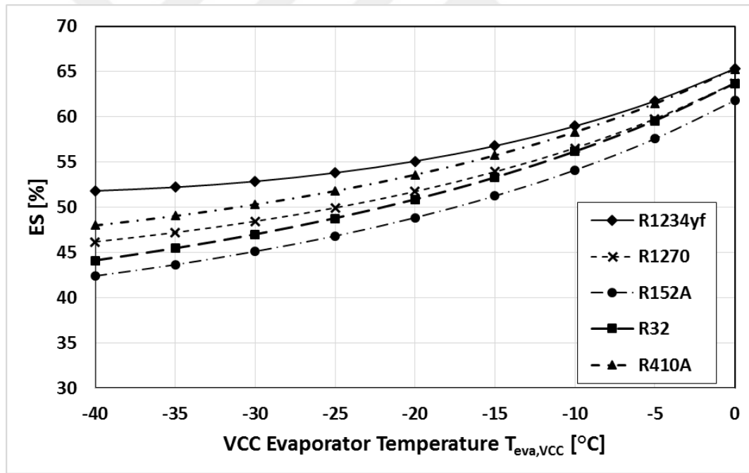
Figure 4. 8. Comparisons of the variation of ES with respect to VCC evaporation temperatures for different refrigerants.
