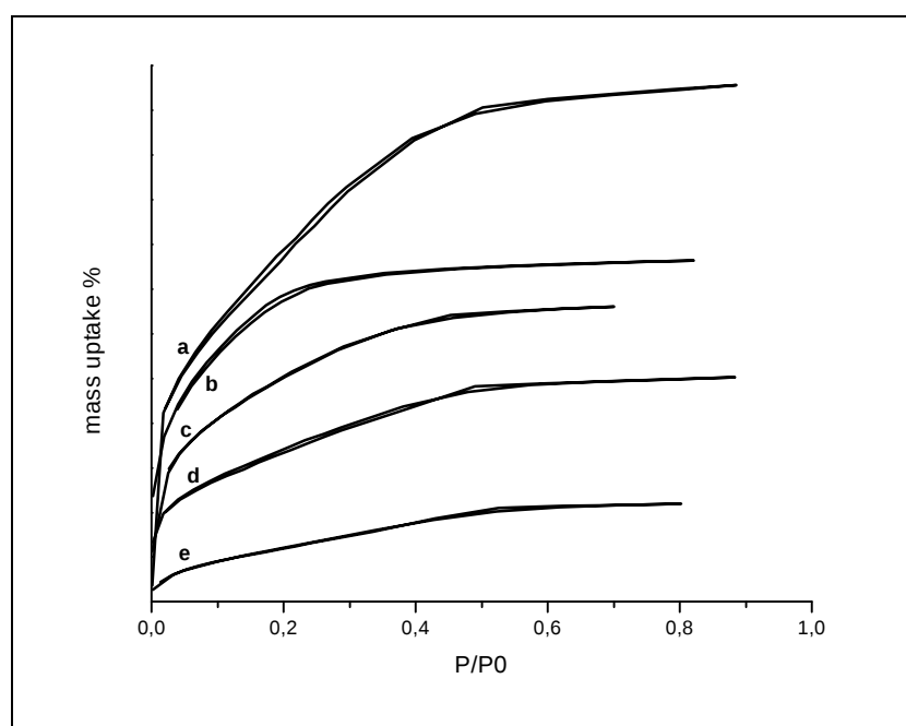
Fig. 3.5.3. N_2 sorption isotherms of calcined silica-sulfated zirconia samples with different zirconia content wt% (a) 80, (b) 60, (c) 90, (d) 98, (e) 100 templated by P85.
