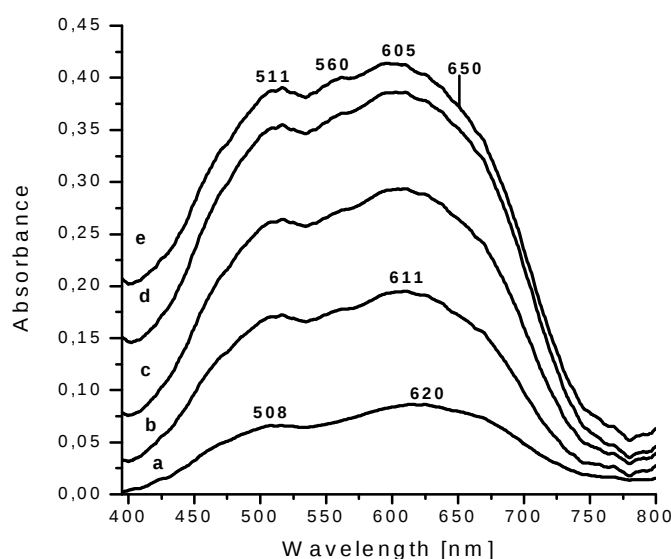
Figure 3.6.2. UV-Visible diffuse reflectance spectra of the calcined at 550^{\circ}\text{C} X wt% Co-Si-SZr (Zr/Si = 3) samples, where X = 1 wt%, cobalt is impregnated (a), 1 wt % (b) 2 wt % (c), 4 wt % (d), 6 wt % (e) cobalt is introduced during the synthesis.
