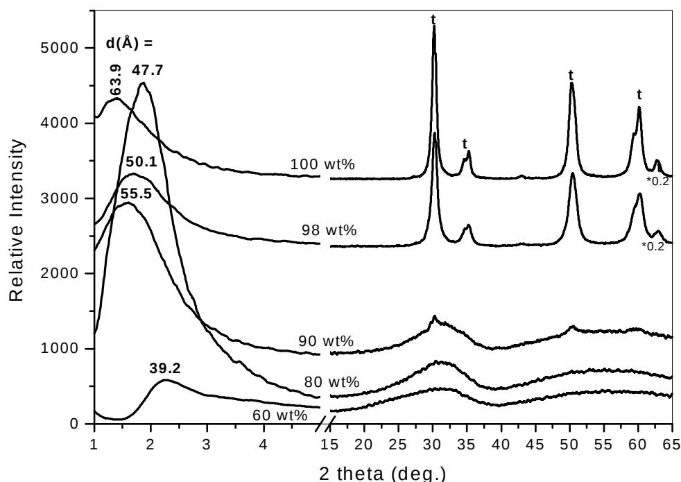
Figure 3.2.3. Powder XRD patterns of calcined at 550°C silica-sulfated zirconia samples containing ~ 8wt% sulfate, prepared with P85. Concentration of ZrO 2 (wt%) is indicated along the lines. The numbers assigned on top of the peaks on the left is the d-spacing values in Å.
