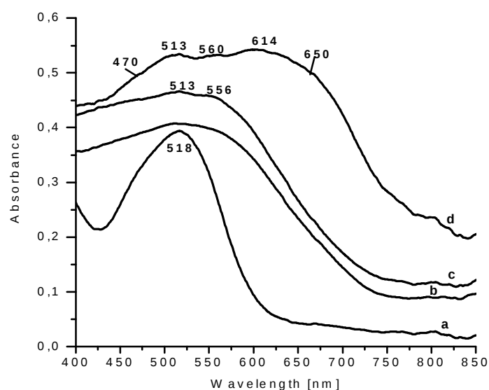
Figure 3.6.1. DR UV-Vis absorption spectra of 1 wt% Co-SZr (a) dried at ambient conditions, (b) calcined at 550^\circ\text{C} , and calcined at 550^\circ\text{C} (c) 1 wt% Co-Si-SZr ( \text{Zr/Si} = 28 ), (d) 6 wt% Co-Si-SZr ( \text{Zr/Si} = 28 ).
