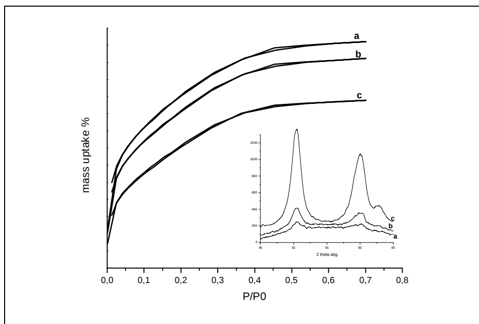
Fig. 3.5.5. N 2 sorption isotherms of Si-SZr (Zr/Si = 4) sample heated stepwise at a) 550 0 C, b) 600 0 C, c) 650 0 C dwelling at each temperature for 3 hrs. Inset shows corresponding powder XRD patterns.
