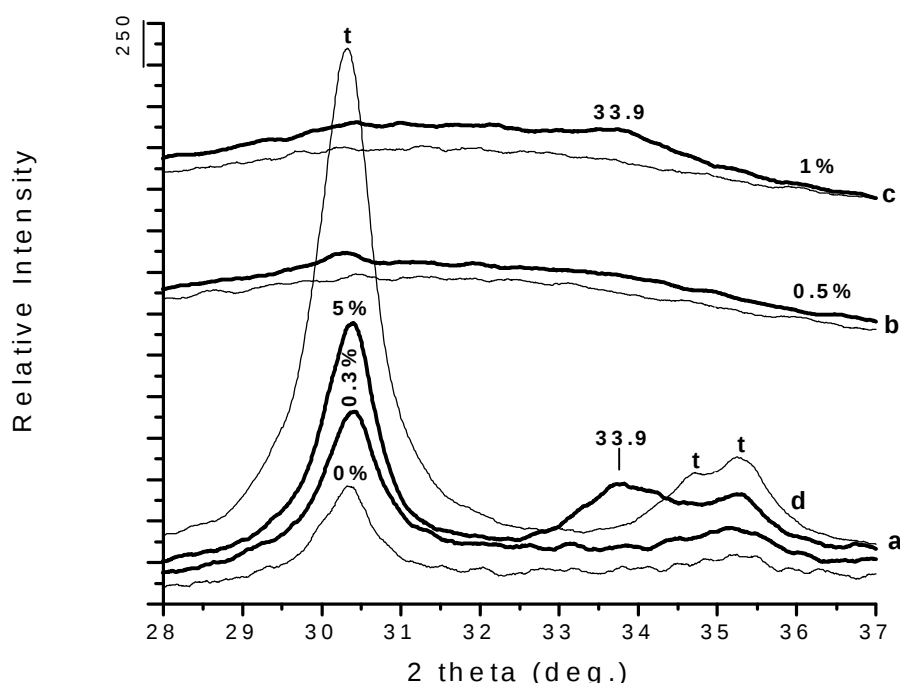
Figure 3.2.5. Powder XRD patterns of calcined at 550°C Pd-6 wt% Co-Si-SZr (Zr/Si = 2) (a), Pd-Si-SZr (Zr/Si = 2) (b), Pd-Si-SZr (Zr/Si = 3) (c), Si-SZr (Zr/Si = 28) (d). Thick lines correspond to palladium containing samples and normal lines to palladium free samples. Concentration of palladium is indicated along the lines. All samples are templated by P85. t stands for tetragonal ZrO 2 .
