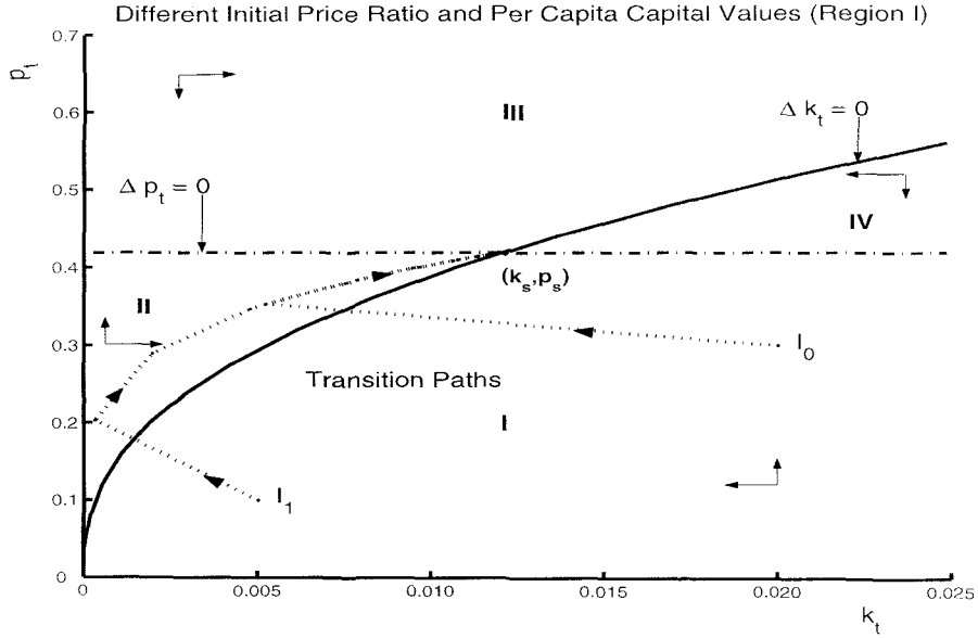
Figure 4.4: Phase Diagram for Per Capita Capital and the Price Ratio for Different Initial Values in Region I
