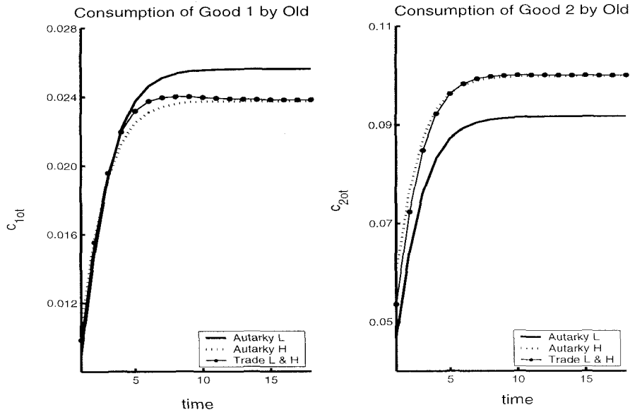
Figure 6.5: Time Paths for the Second Period Consumptions
