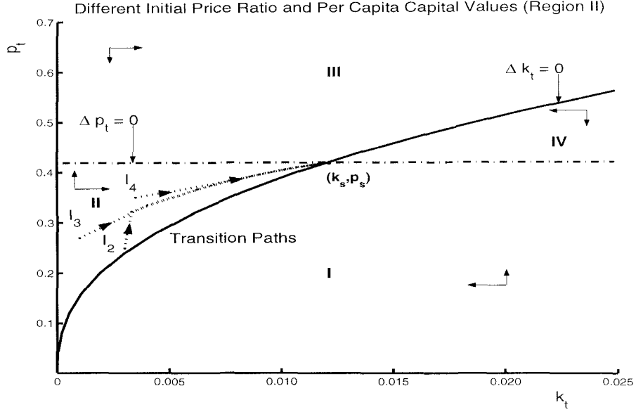
Figure 4.5: Phase Diagram for Per Capita Capital and the Price Ratio for Different Initial Values in Region II
