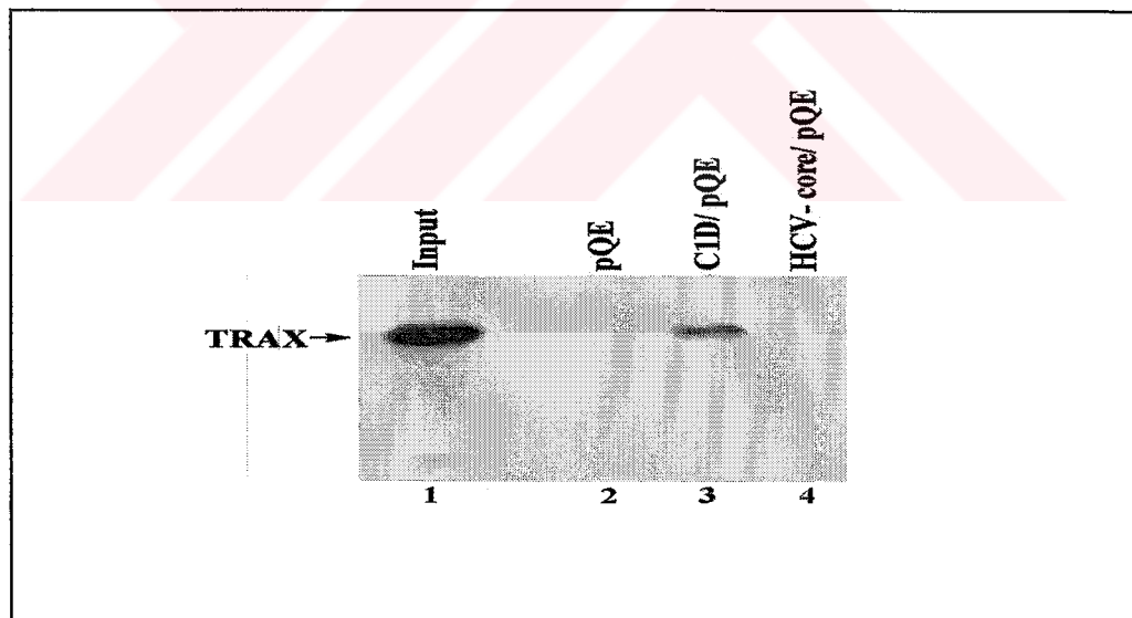
Figure 8: C1D and TRAX interact in vitro . IVTT TRAX was incubated with the indicated fusion proteins immobilized on Ni-NTA coulumn
