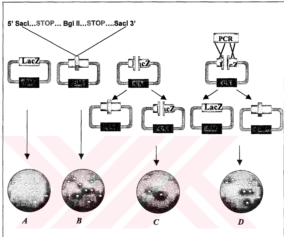
Figure 25: Schematic view of in vivo homologous recombination assay
