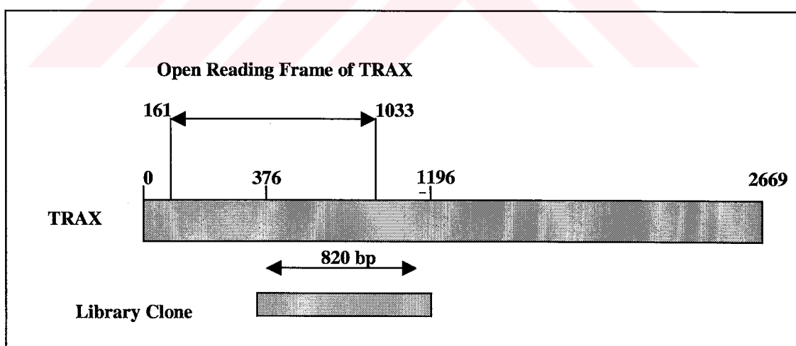
Figure 6: Alignment of Clone41 Against full length TRAX
