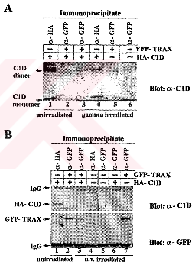
Fig. 5. SDS-resistant C1D homodimers interact with TRAX upon \gamma -irradiation. (A) Transiently transfected COS 7 cells were immunoprecipitated using the antibodies indicated. For lanes 3-6 the cells were treated with 20 Gy of ionizing irradiation before lysate preparation. Western blotting was performed by an anti-C1D antibody. The monomer and dimer forms of C1D are indicated. (B) Transiently transfected COS 7 cells were immunoprecipitated using the indicated antibodies. For lane 3-7, the cells were treated with 50 J/m 2 UV irradiation. The top panel shows the western blotting using an anti-C1D antibody, and in the bottom panel, the blot was stripped and reprobed with an anti-GFP antibody to demonstrate the presence of GFP-TRAX. For each lane, immunoprecipitations were performed using the cell lysates obtained from 3 \times 10^5 cells.
