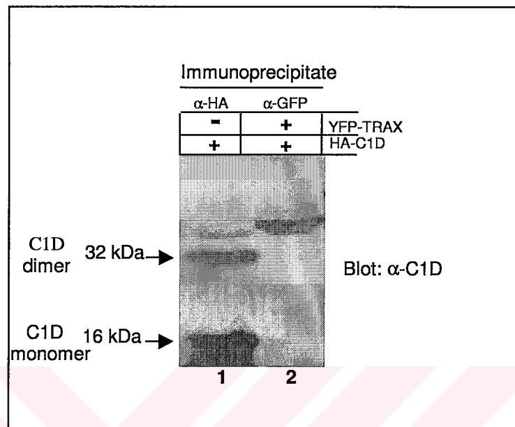
Figure 15: In mammalian cells TRAX and C1D don't interact under normal conditions. Plasmids used in transfections are indicated on the right hand side. Antibodies used for immunoprecipitation are as indicated. Western blot was performed by anti-C1D antibody. The upper band detected above C1D dimer is as a non-specific band.
