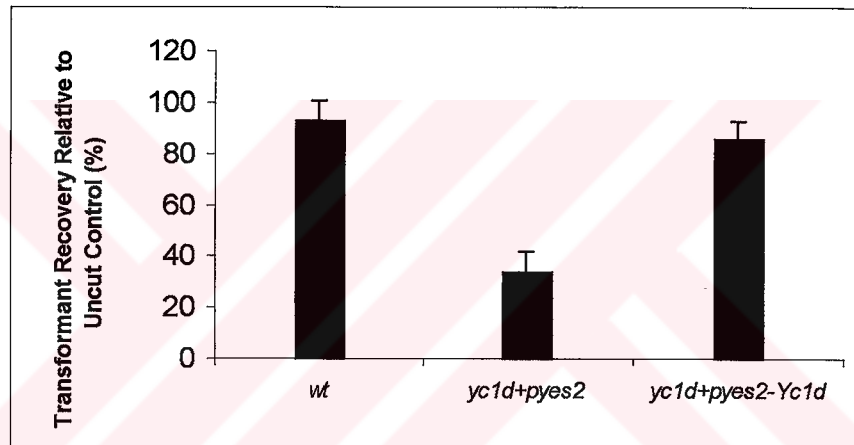
Figure 23: yc1d mutant strain is defective in NHEJ as demonstrated by a plasmid-based in vivo DNA end joining assay. A) Transformant yield of linearized plasmids with the indicated restriction enzymes in wild type and different mutant backgrounds. B) Transformant yield of SacI or PstI -linearized plasmid in yc1d mutant strain is restored to wild type levels when a plasmid expressing Yc1d is introduced.
