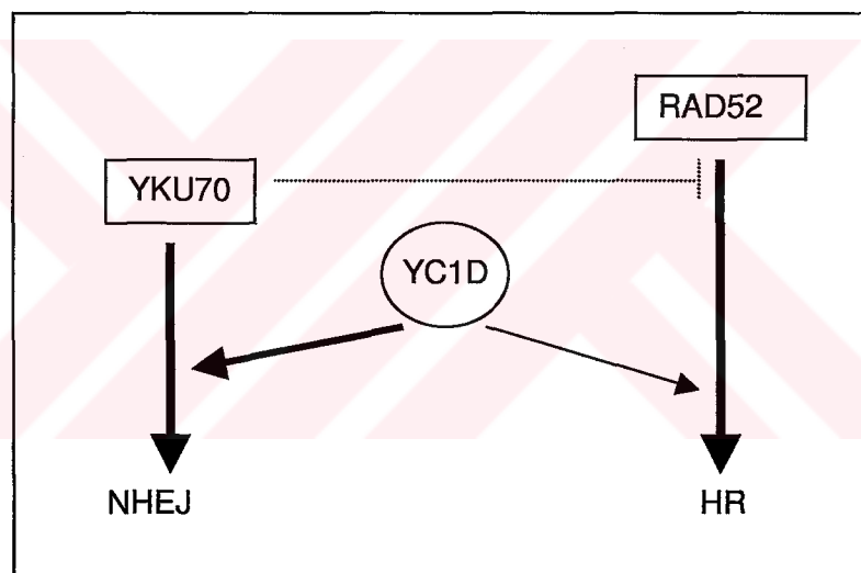
Figure 34: Effect of Yc1d on NHEJ and HR
