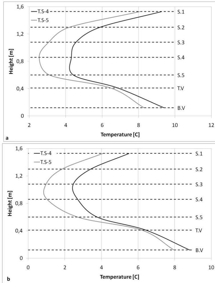
Figure 3.16 The effect of the evaporator surface temperature on the average inner air temperatures (a) Without fan experiments, (b) With fan experiments
