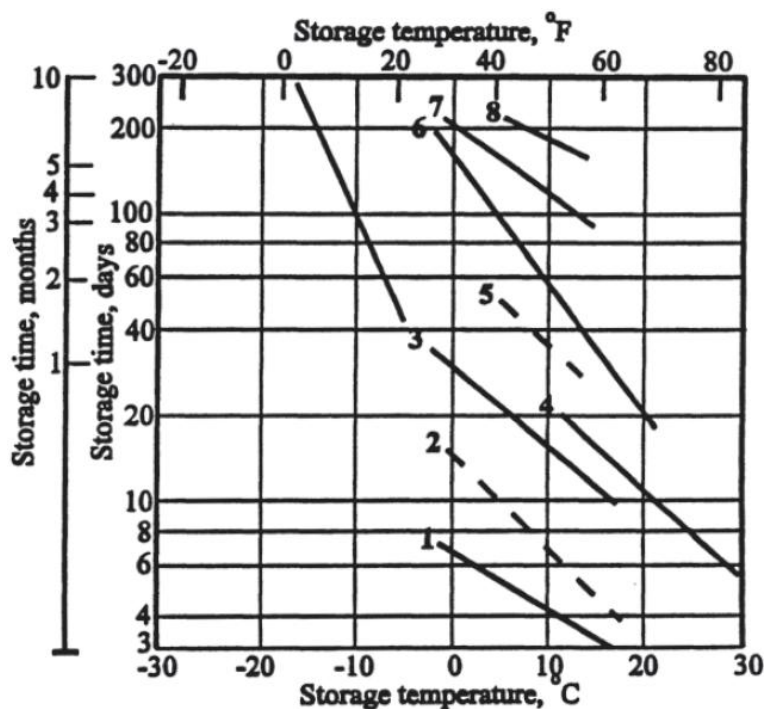
Figure 1.1 Shelf life of several foodstuffs as a function of temperature. (1-chicken, 2-lean fish, 3-beef, 4-bananas, 5-oranges, 6-apples, 7-eggs, 8-apples) (Lorentzen, 1971)
