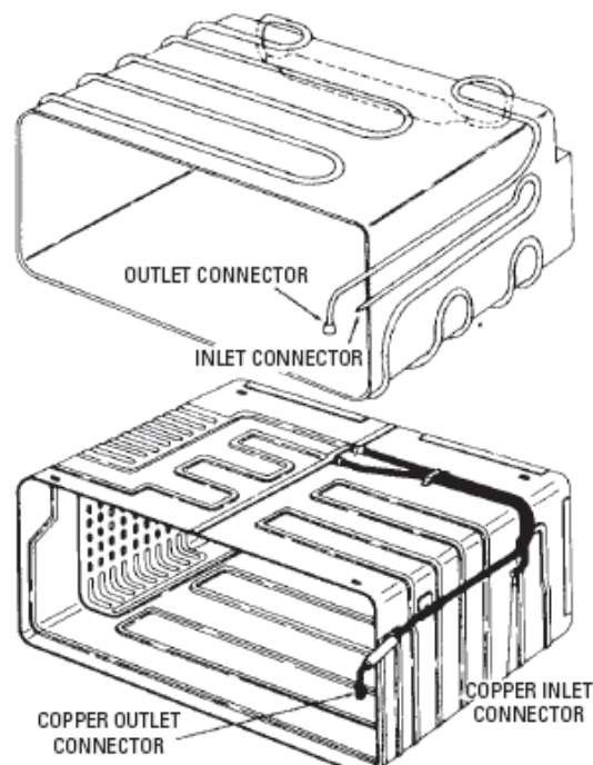
Figure 1.9 Roll-bonded or box plate evaporator (Anderson, 2004), (chap. 4)
