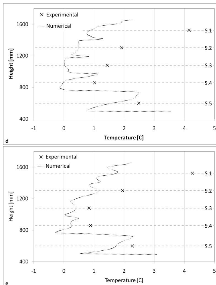
Figure 4.19 (continued) The temperature distributions on lines for simulation and experimental results at fifth thermostat stage and with fan case: (d) Vertical Line-3, (e) Vertical Line-4
