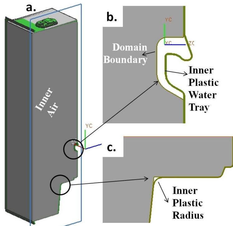
Figure 4.2 (a) Cross section of the inner air and plastic, (b, c) Simplification region examples
