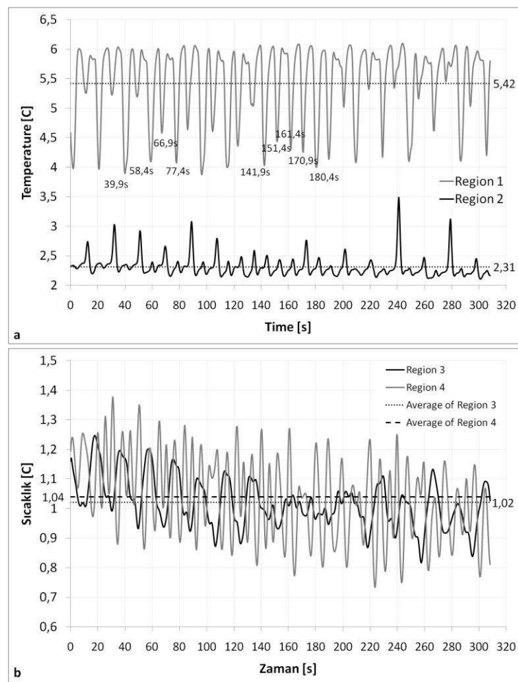
Figure 4.21 Temperature-time curves at region points for fifth stage with fan simulation: (a) Region 1 and 2, (b) Region 3 and 4
