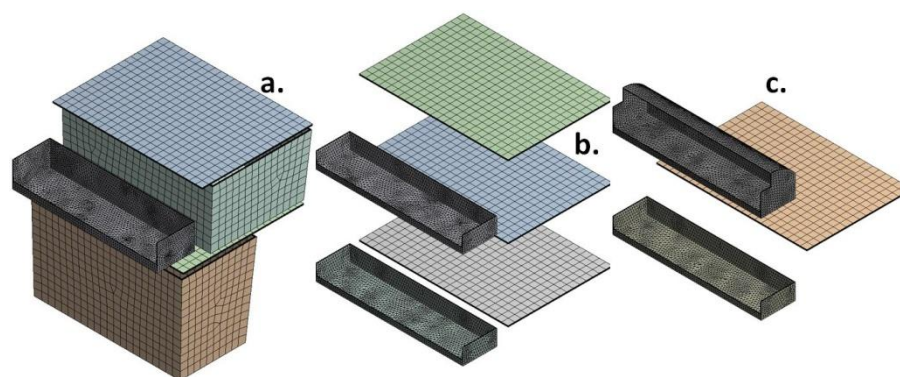
Figure 4.9 Solid domains mesh views: (a) Vegetable compartment baskets, bottom vegetable compartment lid, bottom door shelf and shelf-5, (b) Shelf-2, 3, 4 and middle door shelves, (c) Shelf-1 and top door shelves
