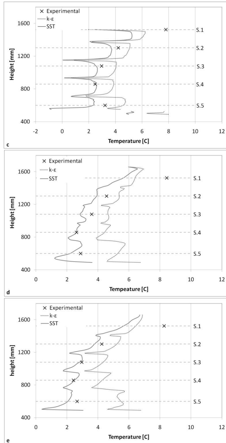
Figure 4.16 (continued) The temperature distributions on lines for simulations with k-ε and SST and experimental results at fifth thermostat stage without fan case: (c) Vertical Line-2, (d) Vertical Line-3, (e) Vertical Line-4
