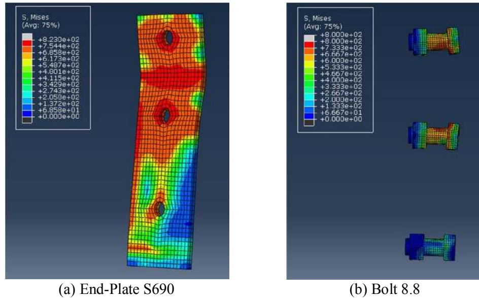
Figure 29: Specimen P10-S690-B8.8
