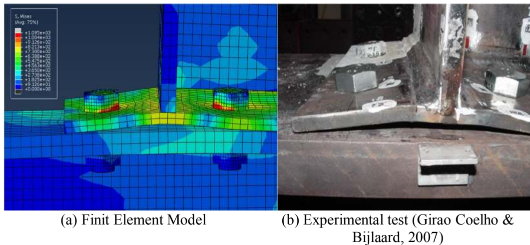
Figure 49: Comparison between Finite Element Model and Experimental Test
