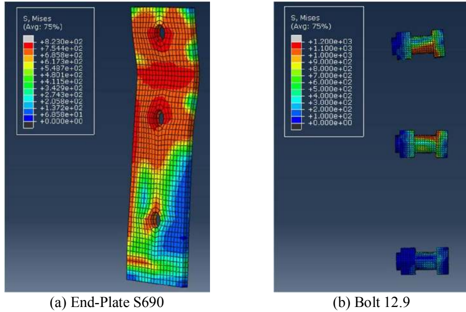
Figure 37: Specimen P10-S690-B12.9
