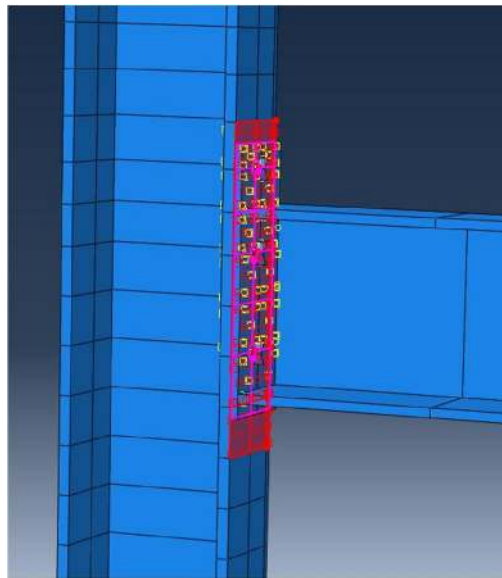
(C) Surface Contact between Plate and Column
