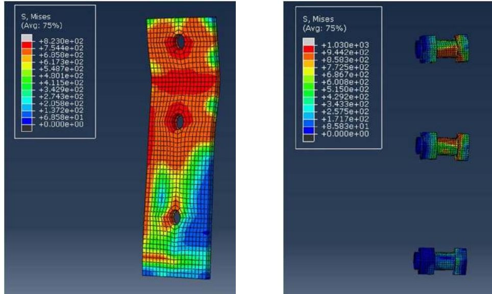
Figure 35: Specimen P10-S690-B10.9
