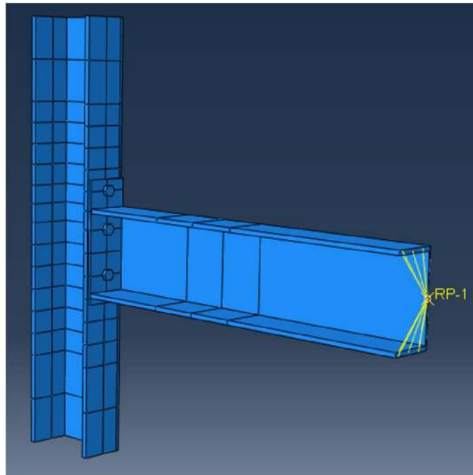
Figure 27: Coupling Point for Reference-Point 1
