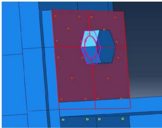
(a) Intraction between Bolt Head and Column
