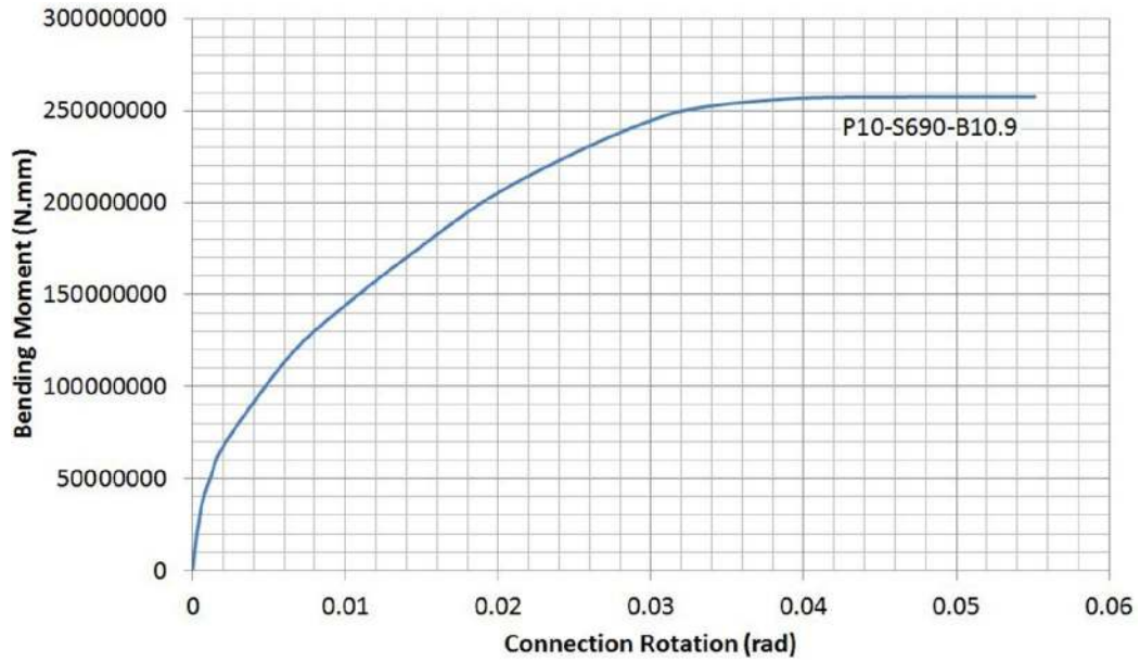
Figure 36: Moment-Rotation Curvature for Specimen P10-S690-B10.9
