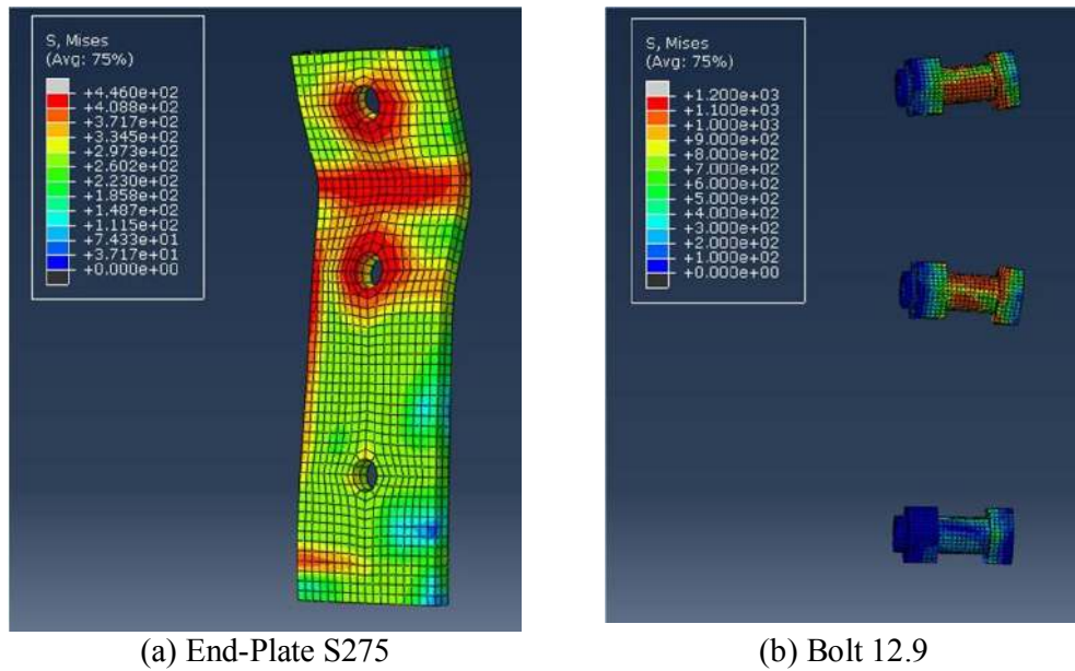
Figure 43: Specimen P15-S275-B12.9
