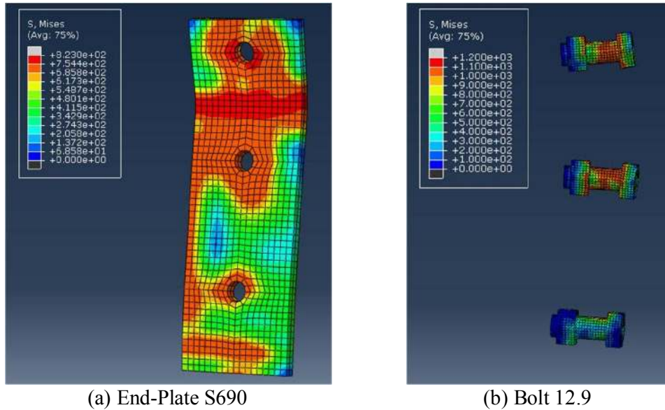
Figure 39: Specimen P15-S690-B12.9
