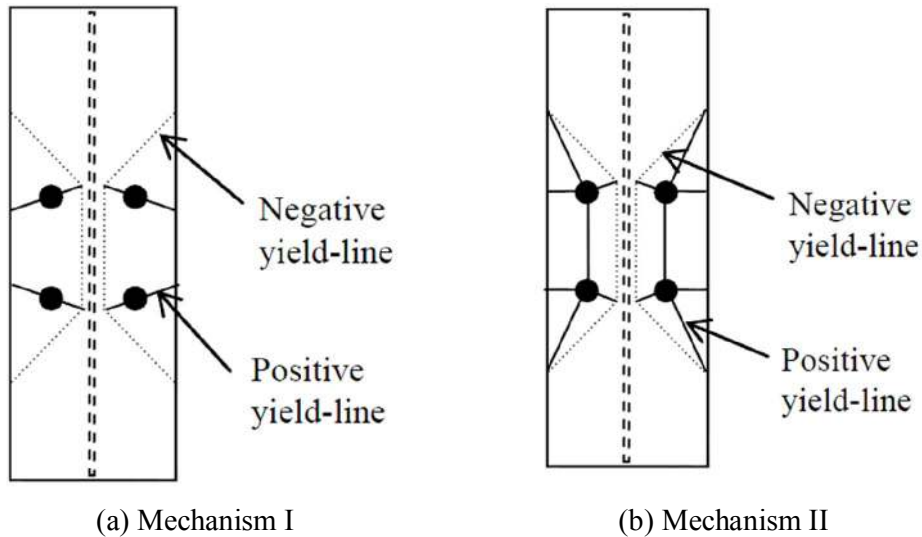
(a) Mechanism I (b) Mechanism II Figure 6: Zoetemeijer's Column Flange Collapse Mechanisms (Source: Zoetemeijer, 1974)
