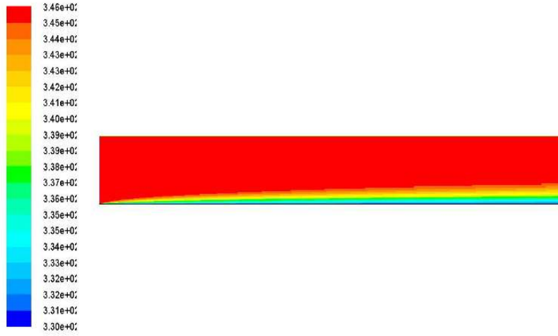
Figure 4.8 Contour of temperature distribution on plate of case 1 (K)
