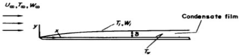
Figure 2.1 Physical model and coordinate system (Sparrow,1967)
