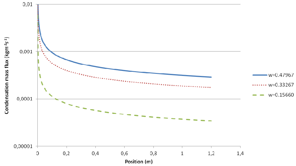
Figure 4.1 Condensation mass flux ( u=0.1 m/s)
