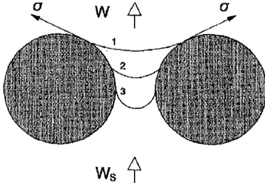
Figure 2.3 Drying shrinkage mechanism according to Power's theory – Stresses pushing water meniscus down between two cement particles (Radocea, 1992)
