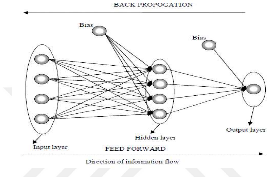
Figure 2.4 Multilayered artificial neural network (Özbay, 2007)
