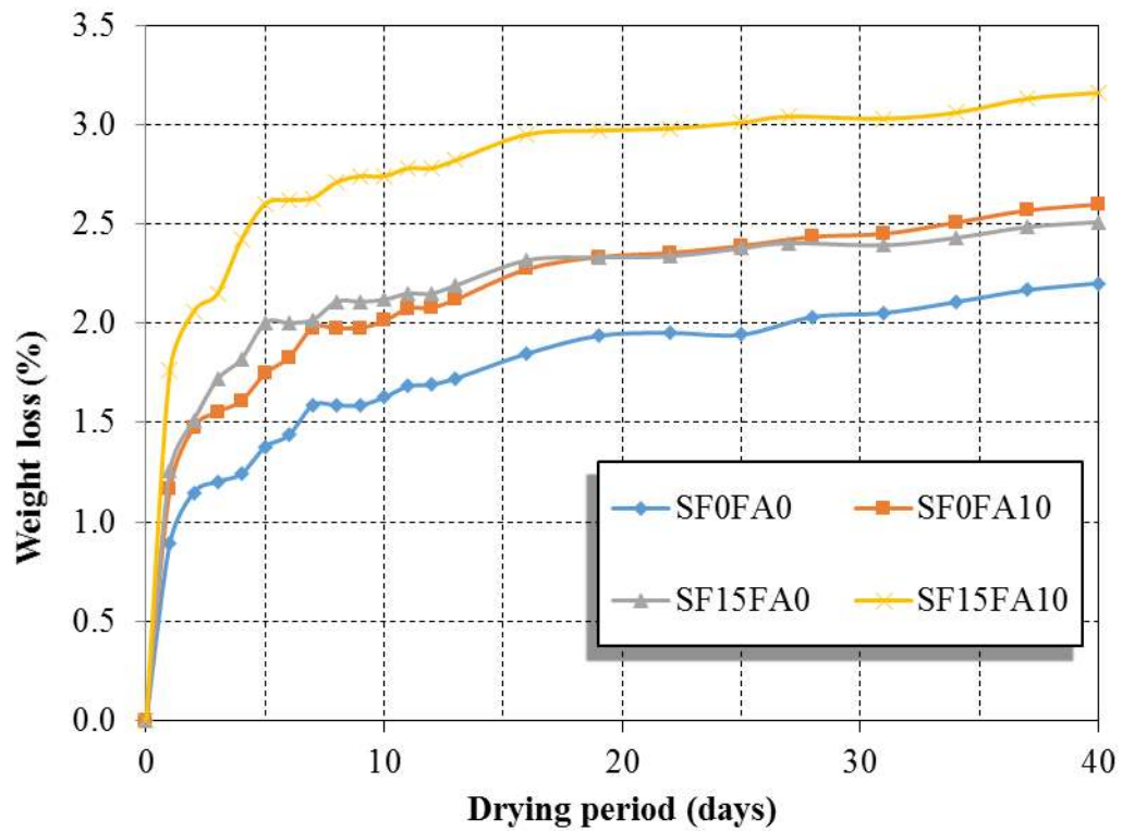
Figure 4.3 Weight loss of concrete
