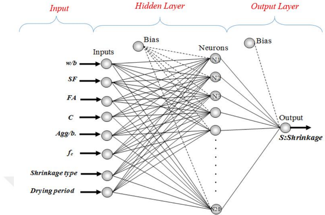
Figure 3.7 Architecture of neural network
