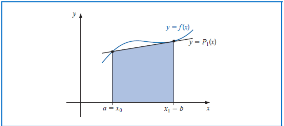
Figure 1 Trapezoidal rule [57]
