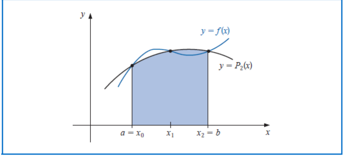
Figure 2 Simpson's rule [57]
