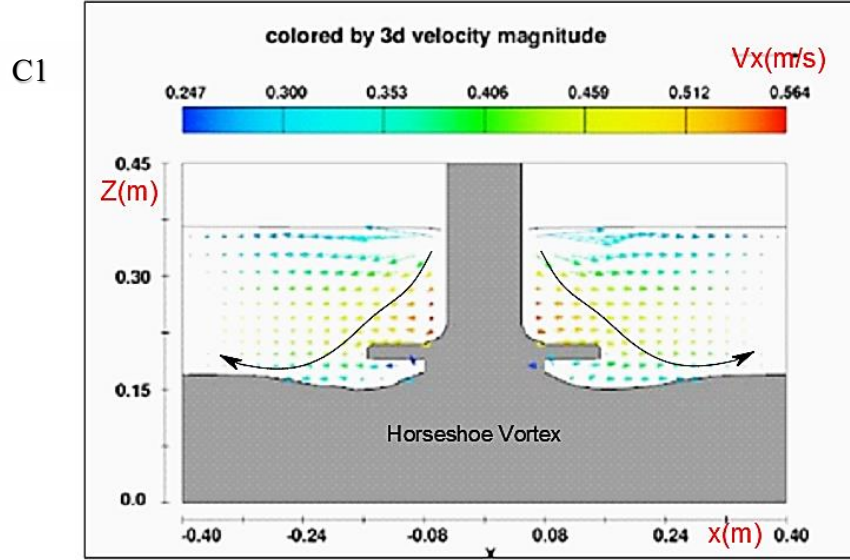
Figure 4.21 Flow field and velocity vectors around the bridge pier model (CPC-3).
