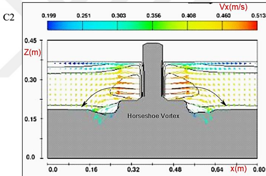
Figure 4.22 Flow field and velocity vectors around the bridge pier model (NPC-3).
