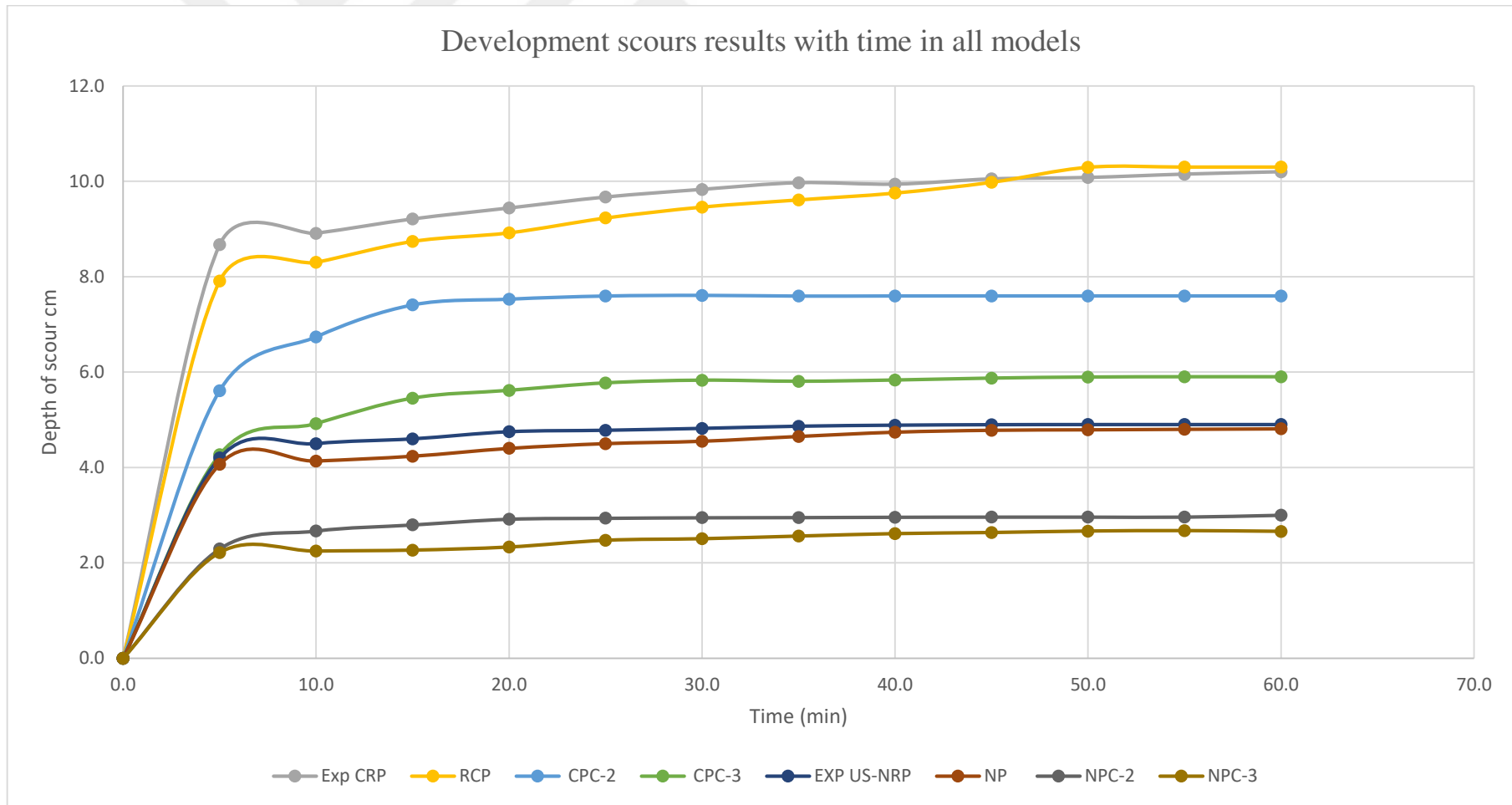
Figure 4.24 Development scours results with time in all models.
