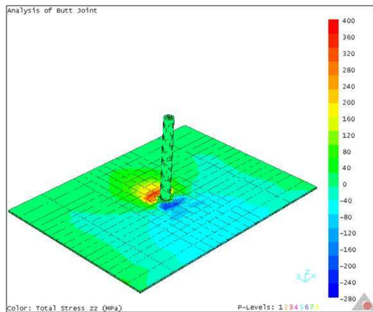
Figure 4.28 \sigma_z stress distribution in the AA 6061 alloy plates during welding for \omega=1000 rpm and v=5 mm/s.
