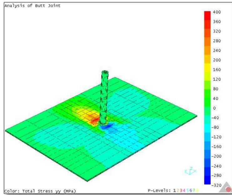
Figure 4.27 \sigma_y stress distribution in the AA 6061 alloy plates during welding for \omega=1000 rpm and v=5 mm/s.
