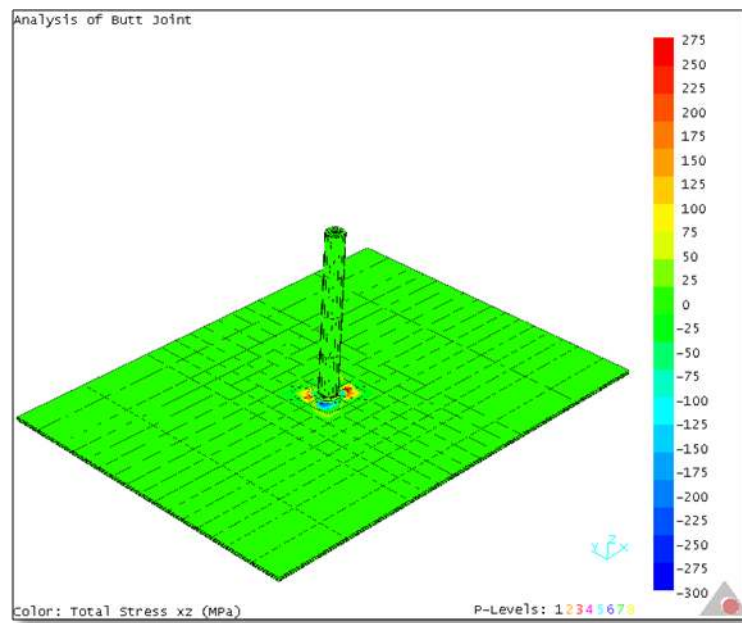
Figure 4.62 \tau_{xz} stress distribution in the AA 7075 alloy plates during welding for \omega=800 rpm and v=5 mm/s.
