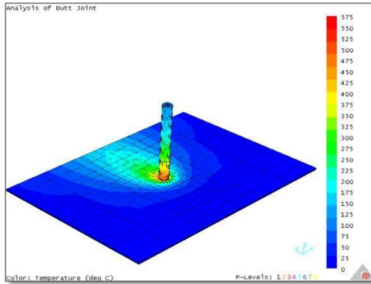
Figure 4.73 Temperature of AA 7075 \omega = 1000 rpm V = 5 mm/s
