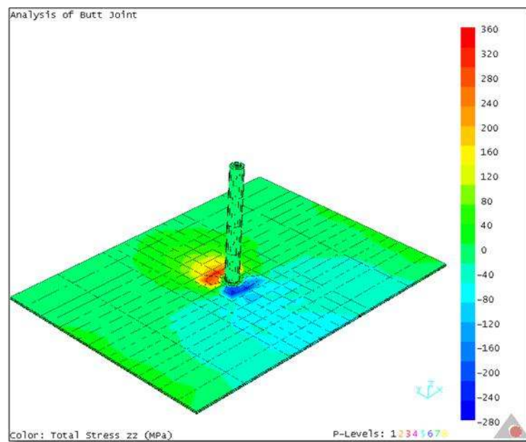
Figure 4.44 \sigma_z stress distribution in the AA 6061 alloy plates during welding for \omega=1200 rpm and v=5 mm/s.
