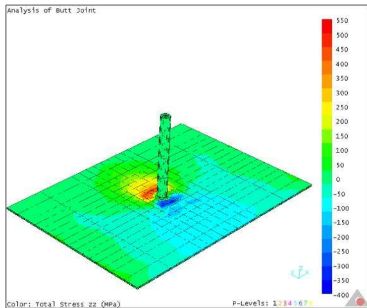
Figure 4.76 \sigma_z stress distribution in the AA 7075 alloy plates during welding for \omega=1000 rpm and v=5 mm/s.
