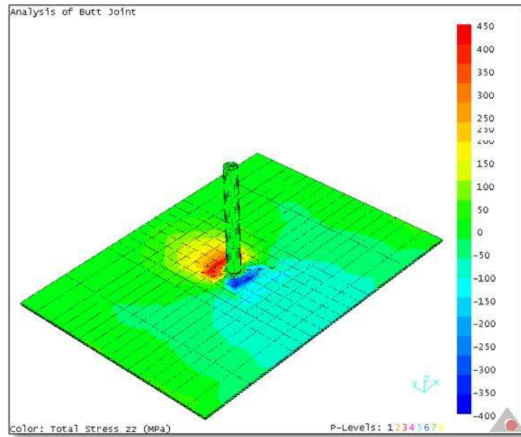
Figure 4.84 \sigma_z stress distribution in the AA 7075 alloy plates during welding for \omega=1200 rpm and v=2.5 mm/s.
