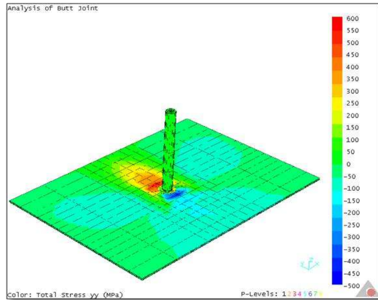
Figure 4.59 \sigma_y stress distribution in the AA 7075 alloy plates during welding for \omega=800 rpm and v=5 mm/s.
