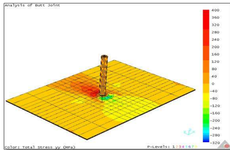
Figure 4.35 \sigma_y stress distribution in the AA 6061 alloy plates during welding for \omega=1200 rpm and v=2.5 mm/s.
