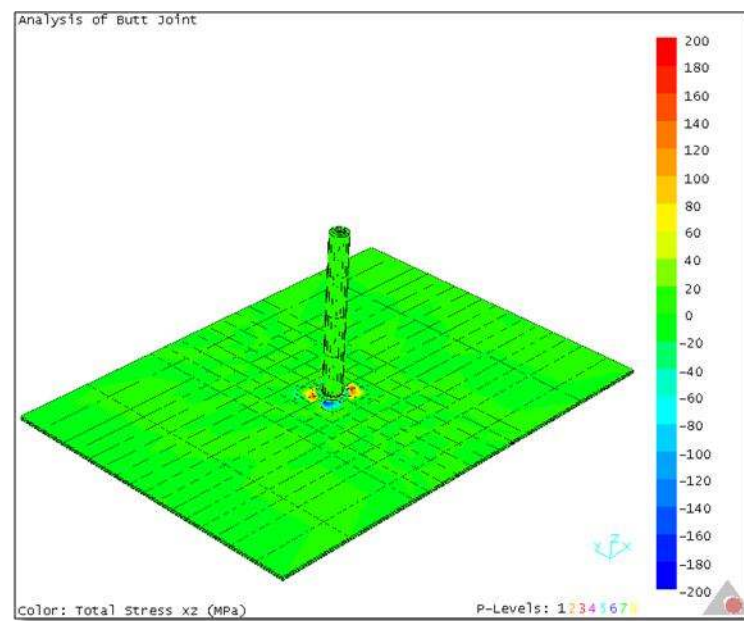
Figure 4.30 \tau_{xz} stress distribution in the AA 6061 alloy plates during welding for \omega=1000 rpm and v=5 mm/s.
