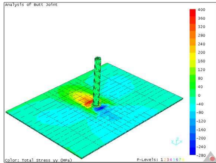
Figure 4.3 \sigma_y stress distribution in the AA 6061 alloy plates during welding for \omega=800 rpm and v= 2.5 mm/s.
