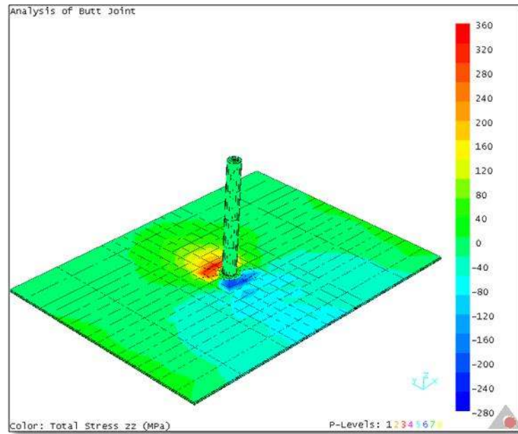
Figure 4.20 \sigma_z stress distribution in the AA 6061 alloy plates during welding for \omega=1000 rpm and v=2.5 mm/s.
