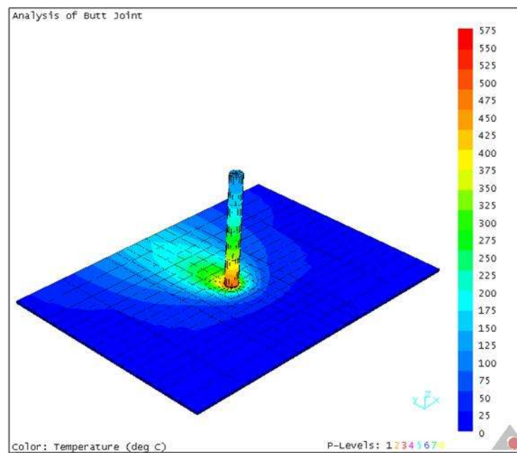
Figure 4.65 Temperature of AA 7075 \omega = 1000 rpm V = 2.5 mm/s
