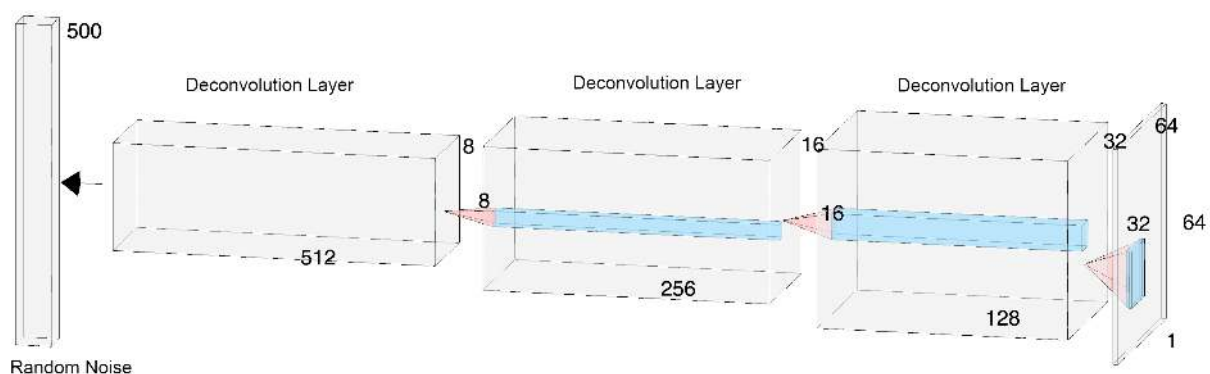
Figure 3. 16 Generator Architecture
