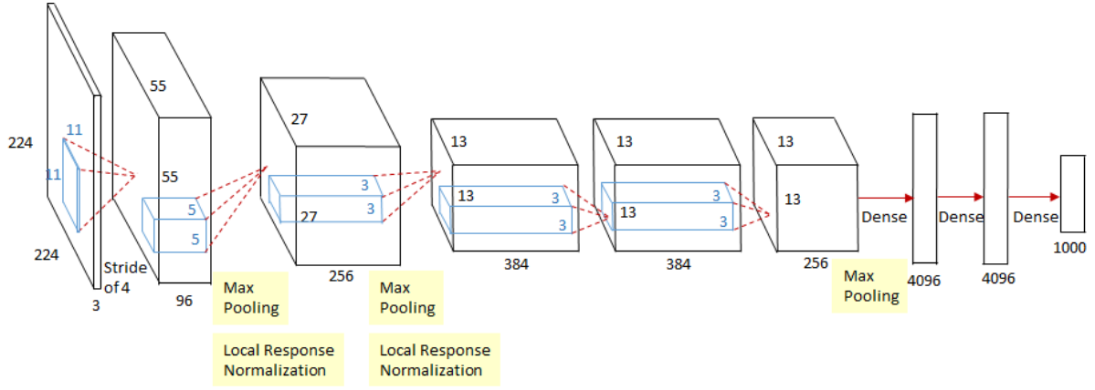
Figure 2. 13 CaffeNet Architecture
