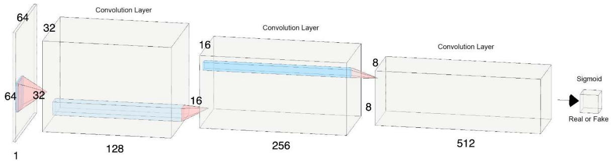
Figure 3. 17 Discriminator Architecture
