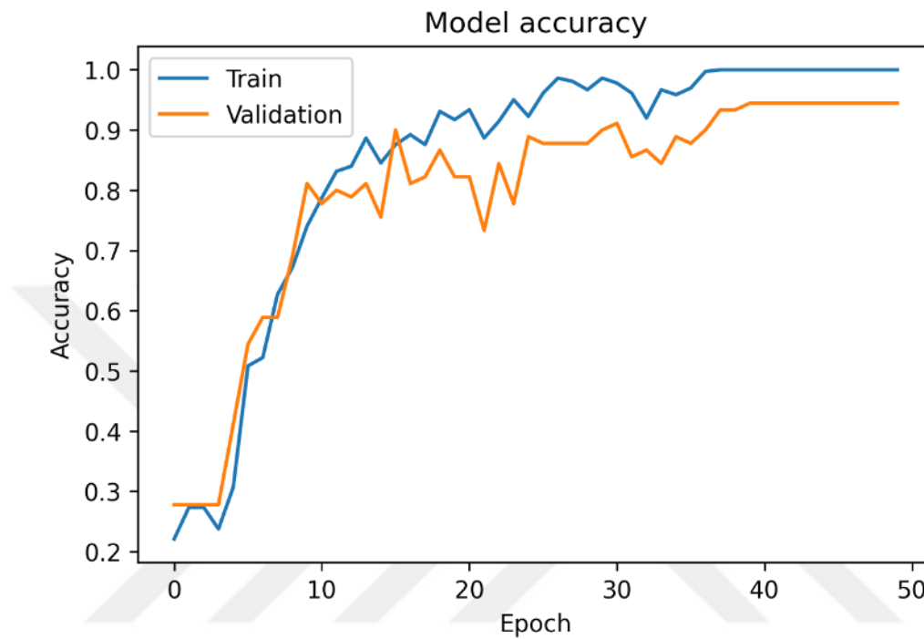
Figure 4. 9 Accuracy over Epoch
