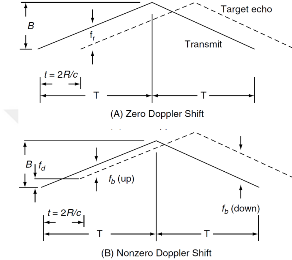
Figure 2. 5 Principle of Triangular FMCW Ranging [4]
