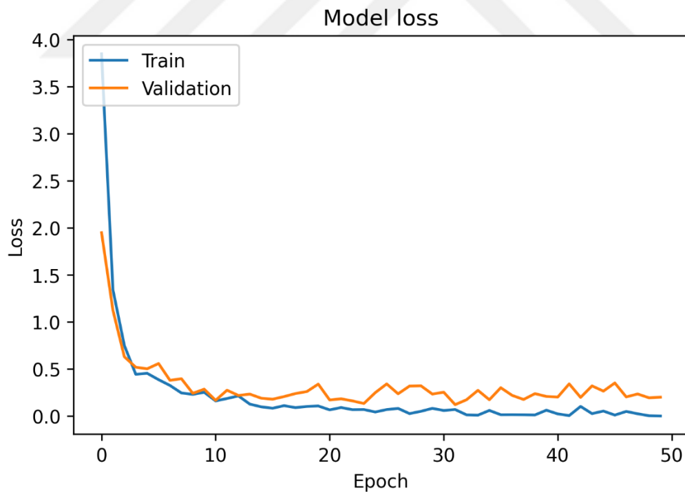
Figure 4. 32 Loss over Epoch
