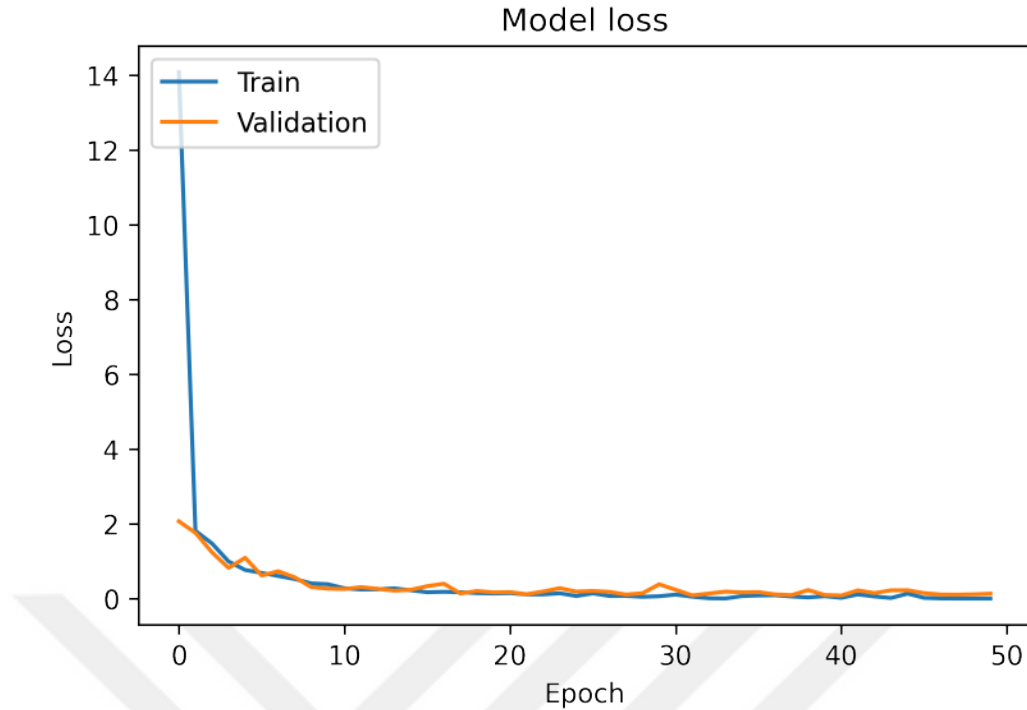
Figure 4. 24 Loss over Epoch
