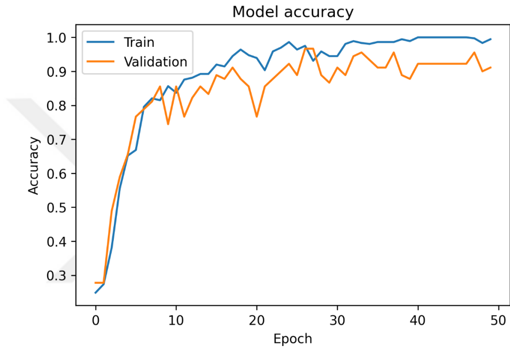
Figure 4. 1 Accuracy over Epoch
