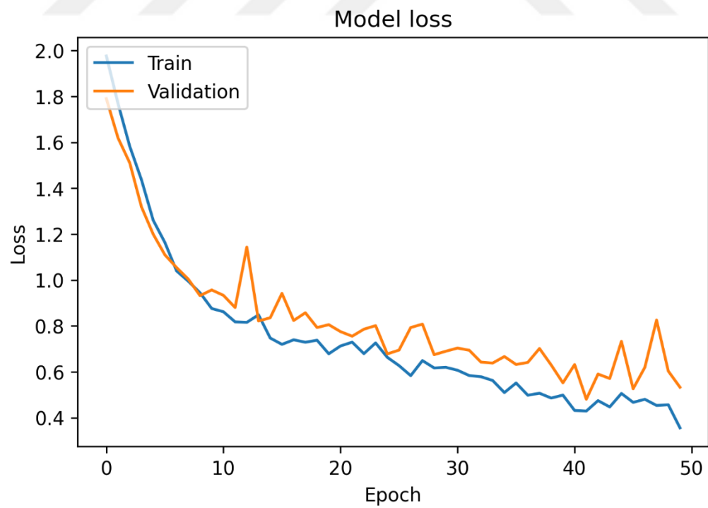
Figure 4. 34 Loss over Epoch
