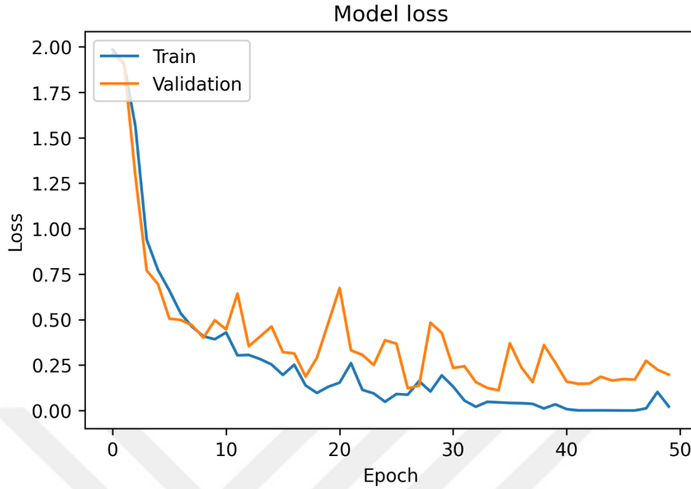
Figure 4. 2 Loss over Epoch
