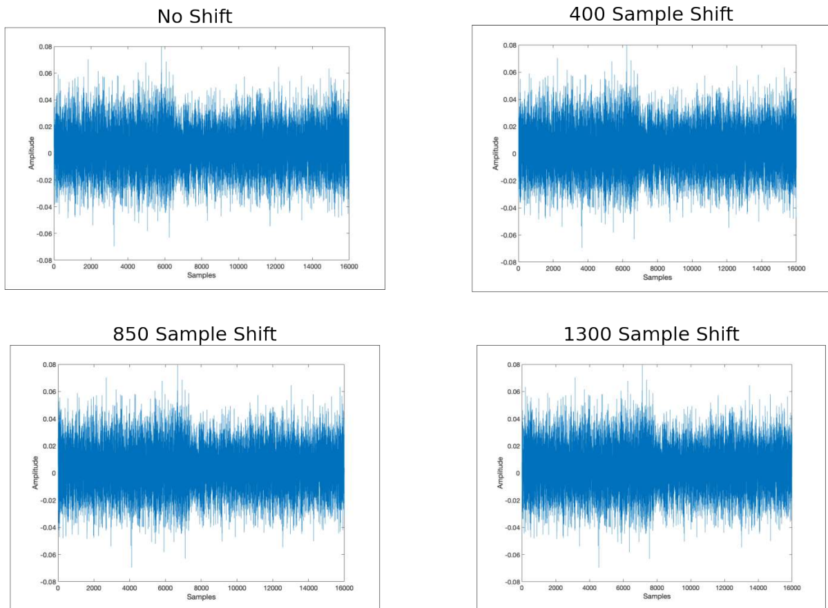
Figure 3. 12 Sample Shifting
