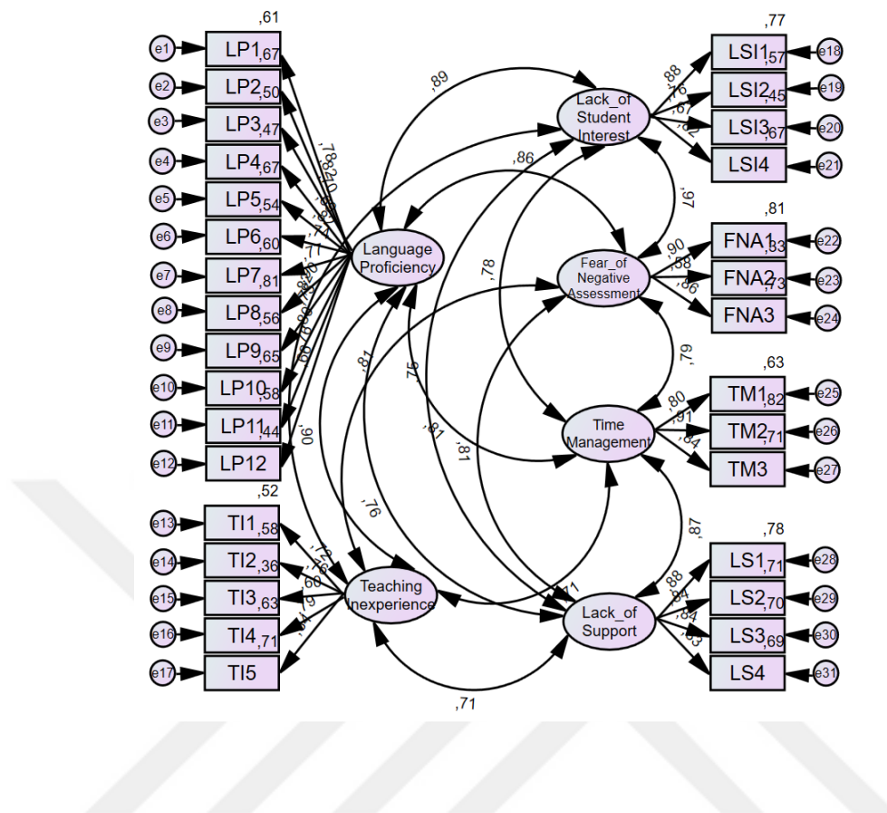
Figure 4.1. Confirmatory factor analysis of EFL teacher anxiety scale
