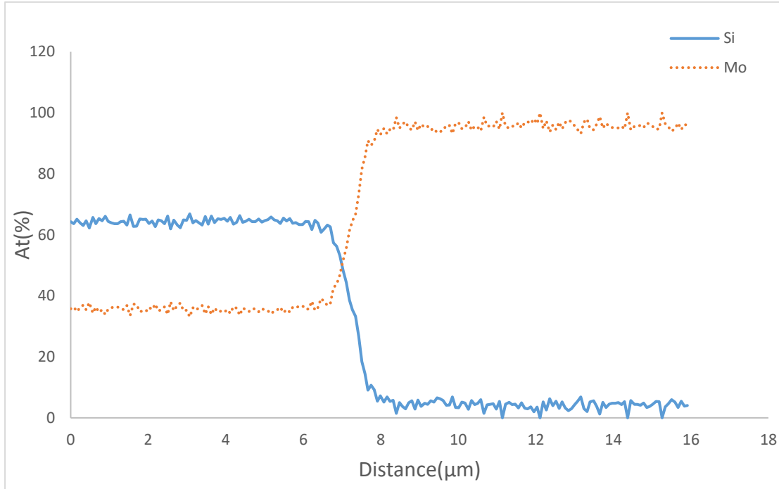
Figure 17 Silicon and molybdenum dispersion results obtained by line analysis in scanning electron microscope.
