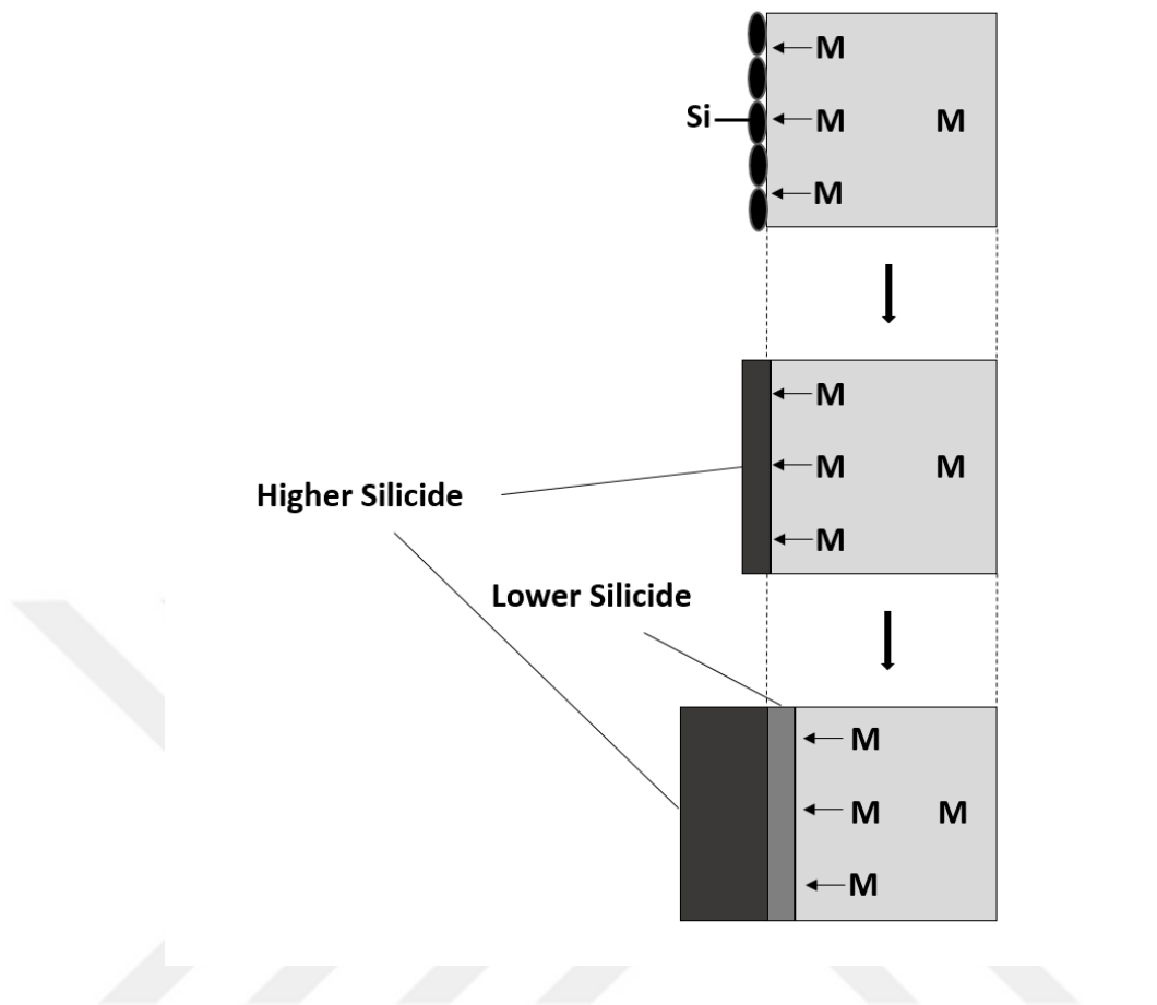
Figure 5 Mechanism of lower and higher silicide formation on refractory metals. Reproduced from reference [32].
