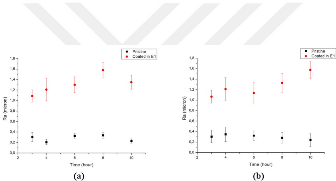
Figure 22 The change of average surface roughness of pure molybdenum samples that coated in E1 at 800°C (a) and at 900°C (b).
