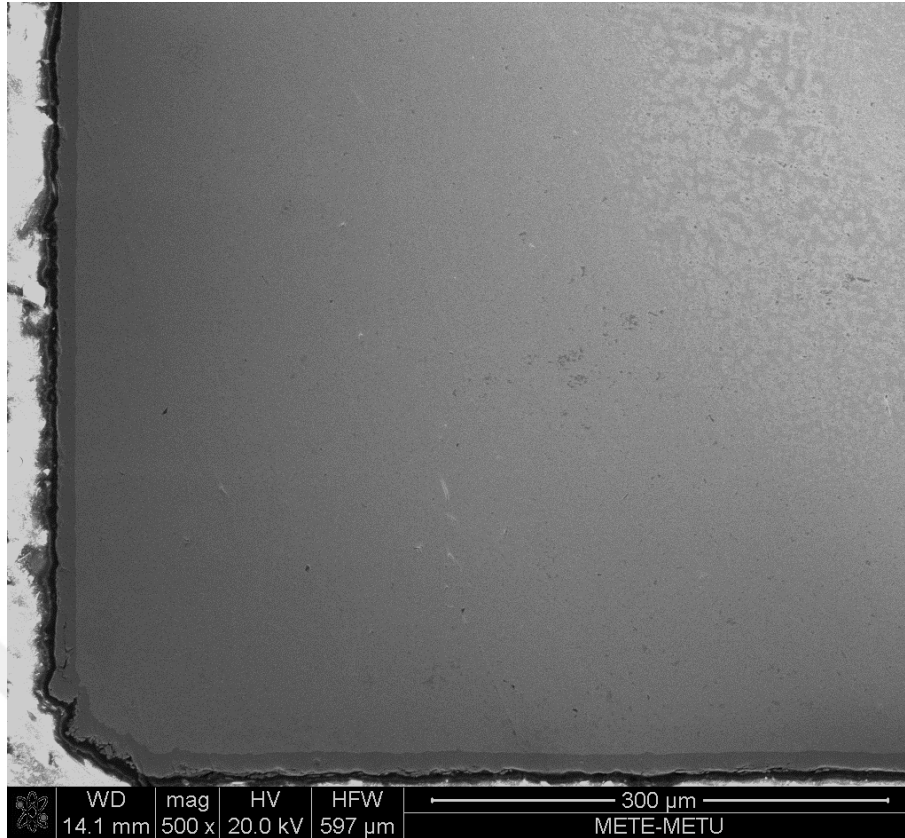
Figure 18 SEM image of the section of silicide coated pure molybdenum sample at 900°C for 4 hours.
