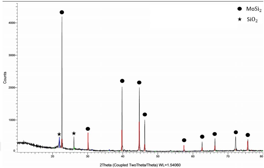
Figure 38 X-Ray Diffraction result of coated TZM Alloy sample after oxidation test at 800°C for 6 hours.
