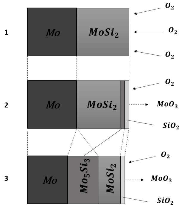
Figure 3 Oxidation mechanism of molybdenum di-silicide layer at elevated temperature and formation of silica layer and molybdenum rich phases. Reproduced from reference [34].
