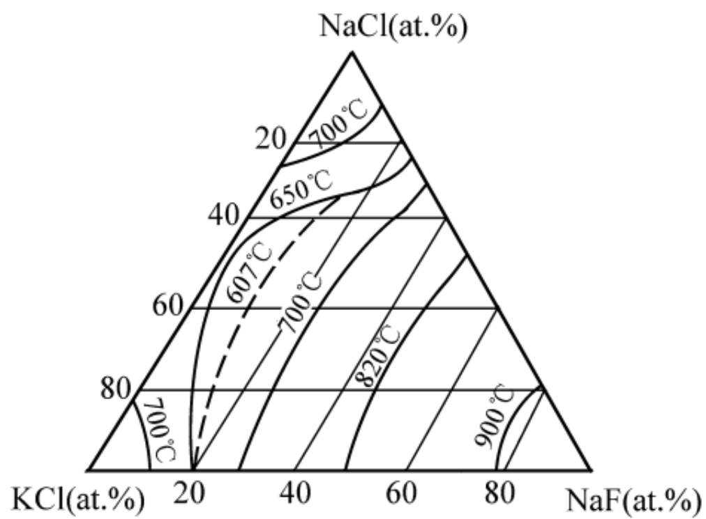
Figure A.2 NaCl-KCl-NaF ternary phase diagram [90].
