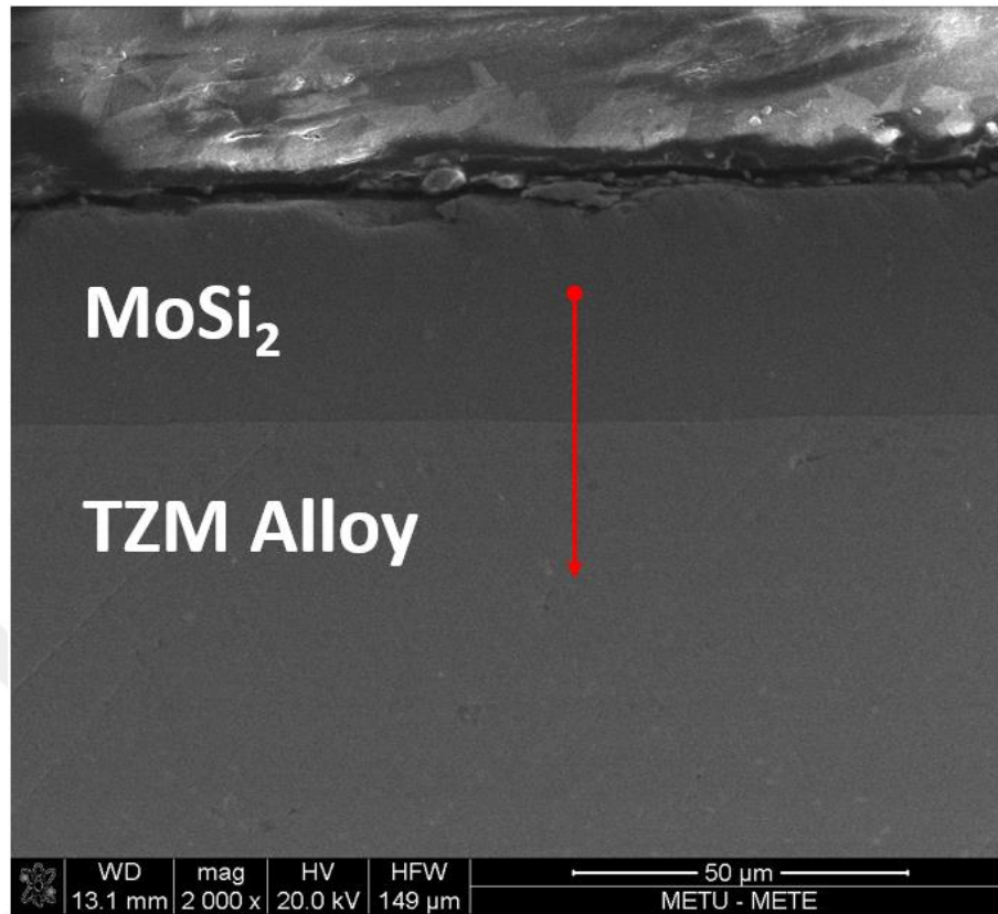
Figure 25 SEM image of the section of silicide coated TZM Alloy sample at 800°C for 3 hours and line on which EDS line analysis was done.
