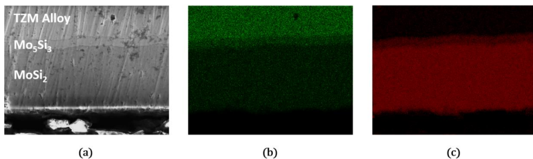
Figure 44 The EDS mapping results: (a) SEM image of the region EDS mapping performed; (b) distribution of molybdenum atoms and (c) distribution of silicon atoms.
