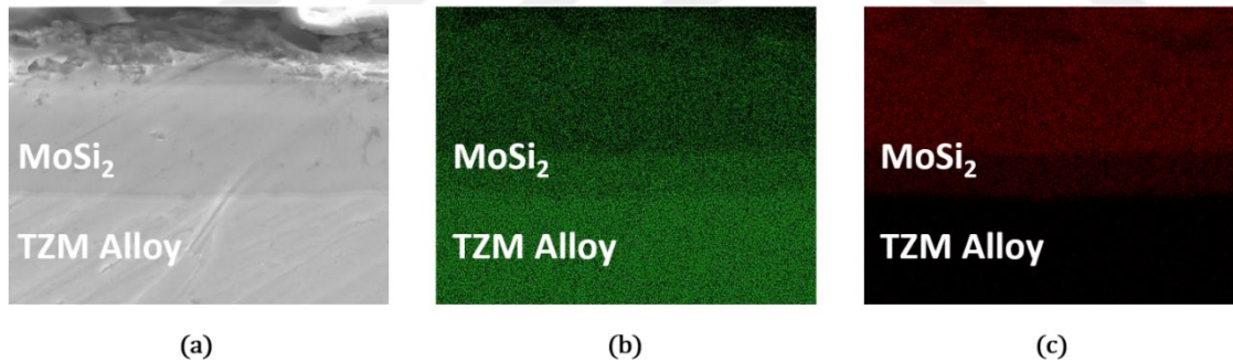
Figure 40 The EDS mapping results: (a) SEM image of the region EDS mapping performed; (b) distribution of molybdenum atoms and (c) distribution of silicon atoms.
