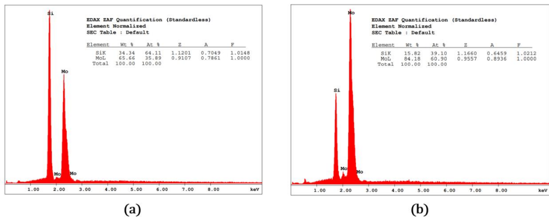
Figure 42 EDS analysis of silicide layers: (a) taken from region 1 in Figure 39 and (b) taken from region 2 Figure 39.
