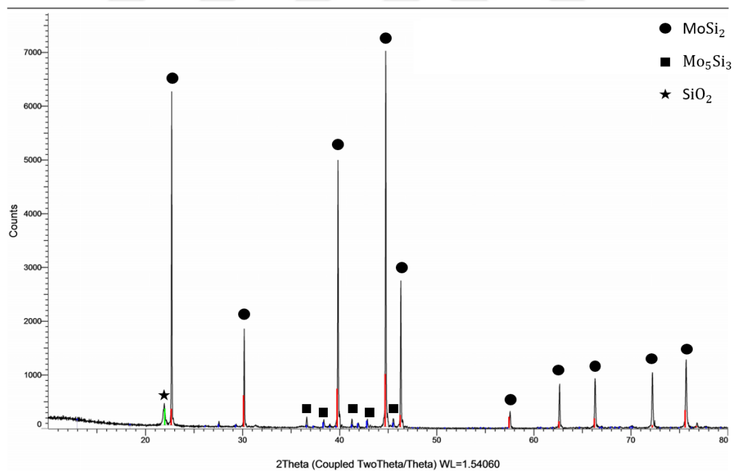
Figure 45 X-Ray Diffraction result of oxidized coated TZM Alloy sample at 1200°C for 1 hours.
