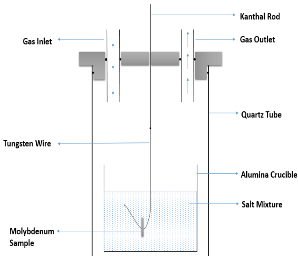
Figure 10 Schematic representation of cross-section of experimental setup.
