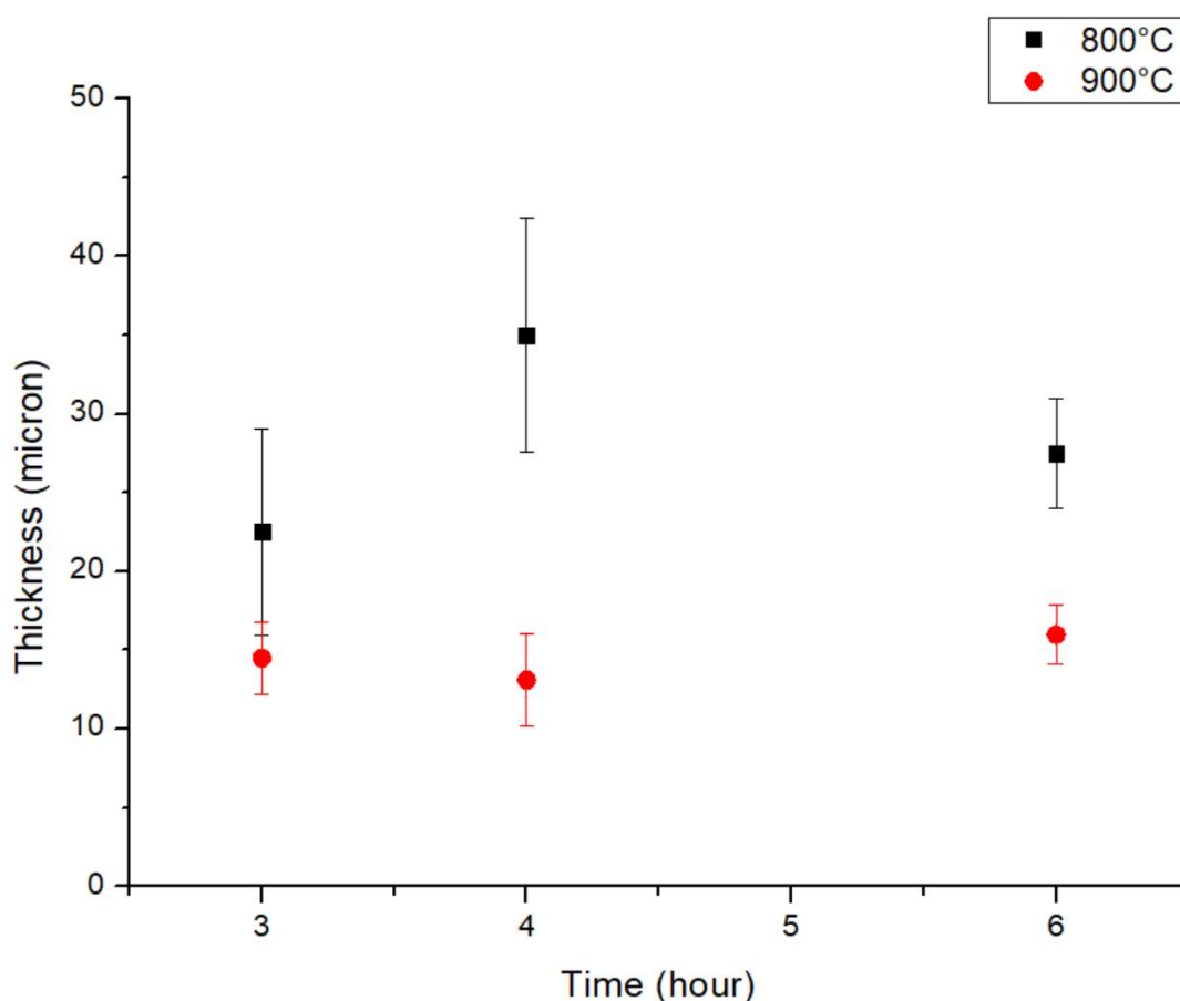
Figure 28 Time-dependent thickness changes of coatings on TZM Alloy substrates at 800°C and 900° C.
