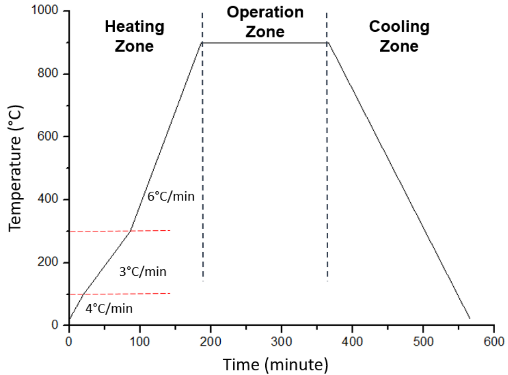
Figure 12 Temperature profile used during heating and cooling the samples.
