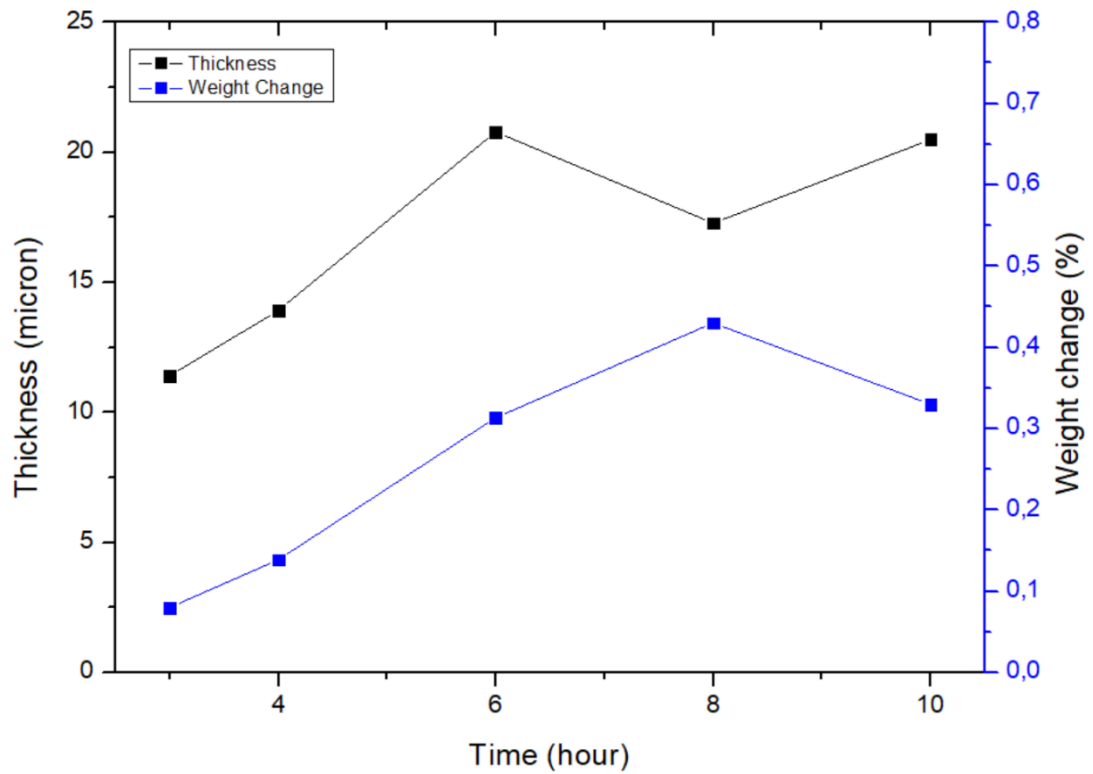
Figure 21 The relationship between mass change and coating thickness over time for the coated pure molybdenum samples at 900°C.
