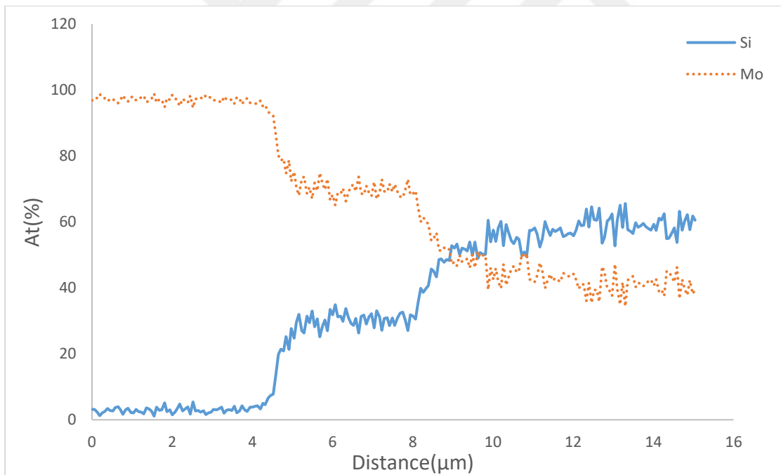
Figure 43 Silicon and molybdenum dispersion results obtained by line analysis in scanning electron microscope.
