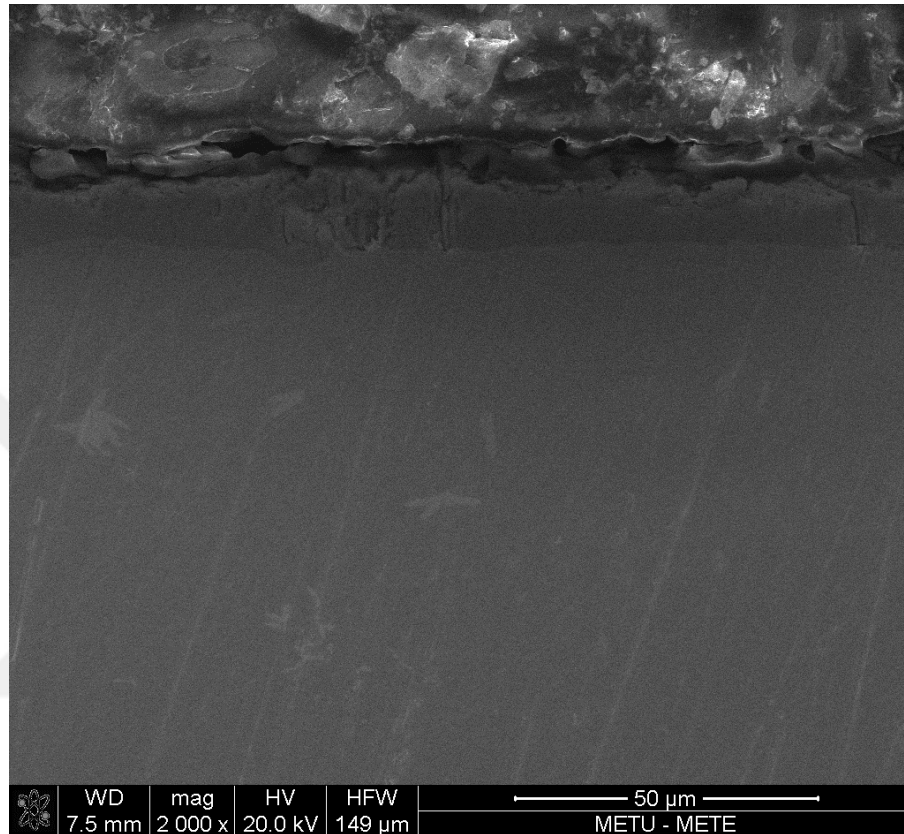
Figure 34 SEM image of the section of oxidized pure molybdenum sample at 800°C for 6 hours.
