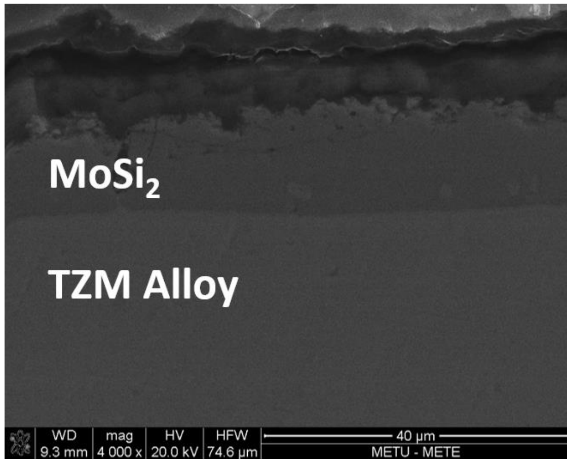
Figure 37 SEM image of the section of coated TZM Alloy sample after oxidation test at 800°C for 6 hours.
