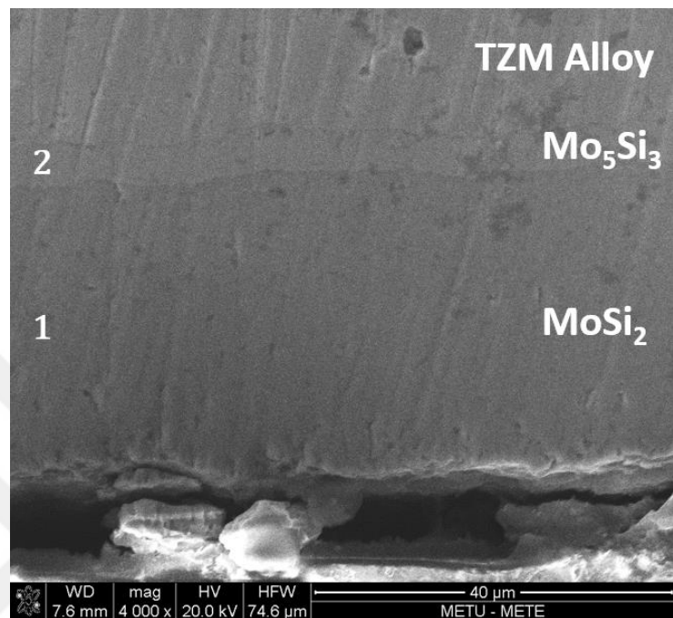
Figure 41 SEM image of the section of oxidized coated TZM Alloy sample at 1200°C for 1 hour.
