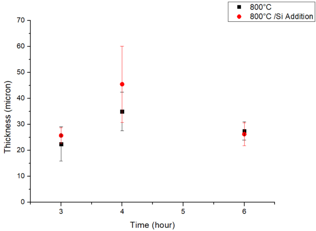
Figure 29 Time-dependent thickness changes of coatings using E1 and E2 mixtures on TZM alloy substrates at 800°C.
