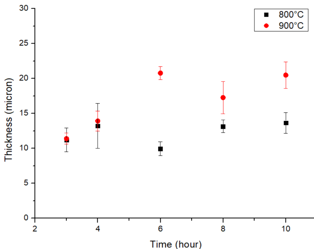
Figure 19 Time-dependent thickness changes of coatings on pure molybdenum substrates at 800°C and 900° C.
