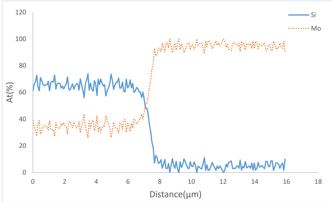
Figure 26 Silicon and molybdenum dispersion results obtained by line analysis in scanning electron microscope.
