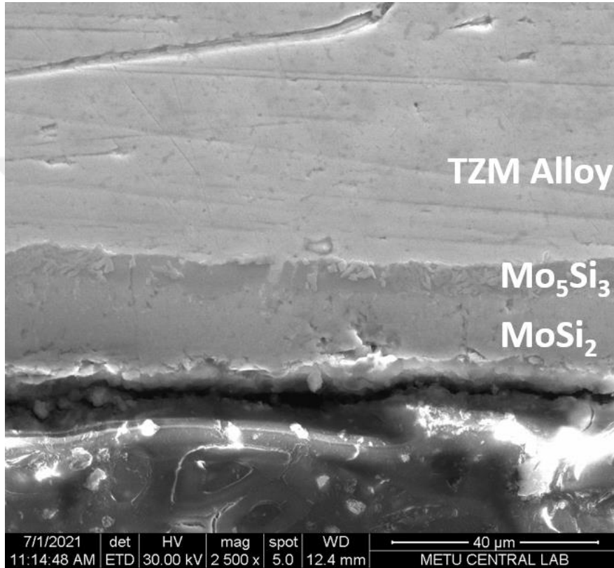
Figure 46 SEM image of the section of oxidized coated TZM Alloy sample at 1200°C for 3 hours.
