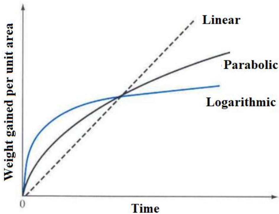
Figure 2 Illustration of linear, parabolic, and logarithmic rate laws of metals in terms of weight gain vs. time.
