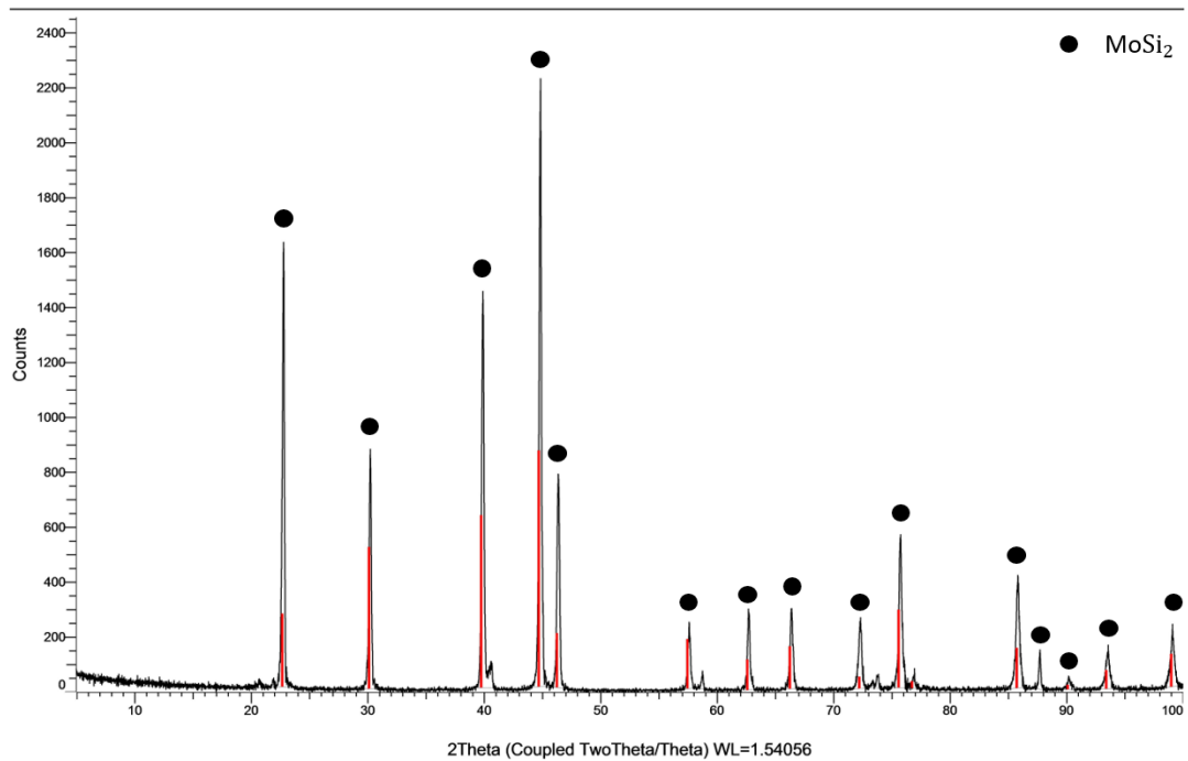
Figure 14 X-Ray Diffraction result of pure molybdenum sample coated at 800°C for 10 hours.
