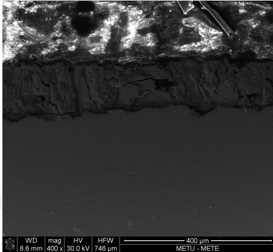
Figure 36 SEM image of the section of oxidized pure TZM Alloy sample at 800°C for 6 hours.
