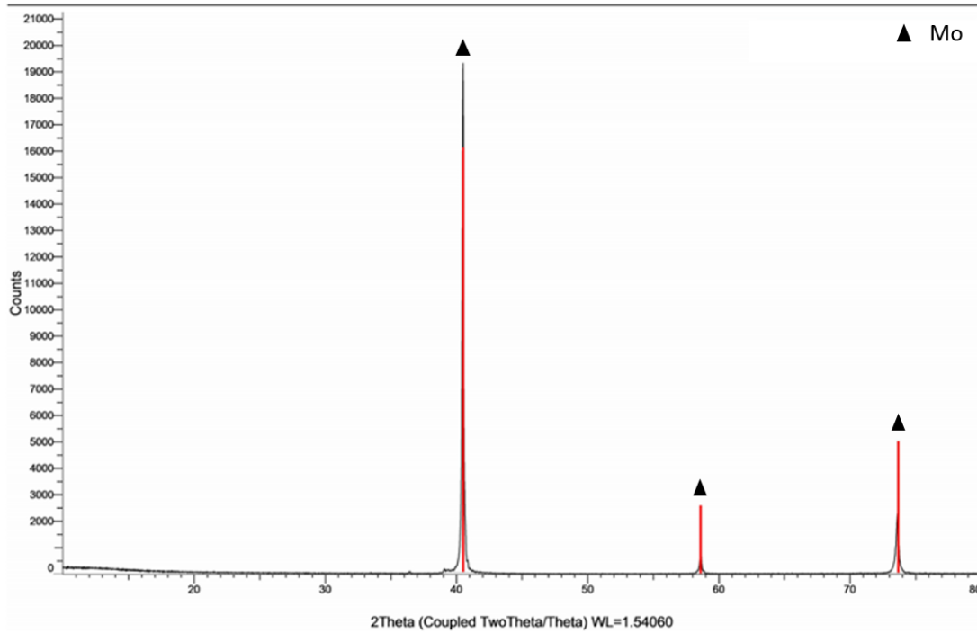
Figure 9 X-Ray Diffraction result of TZM alloy sample before the experiment.
