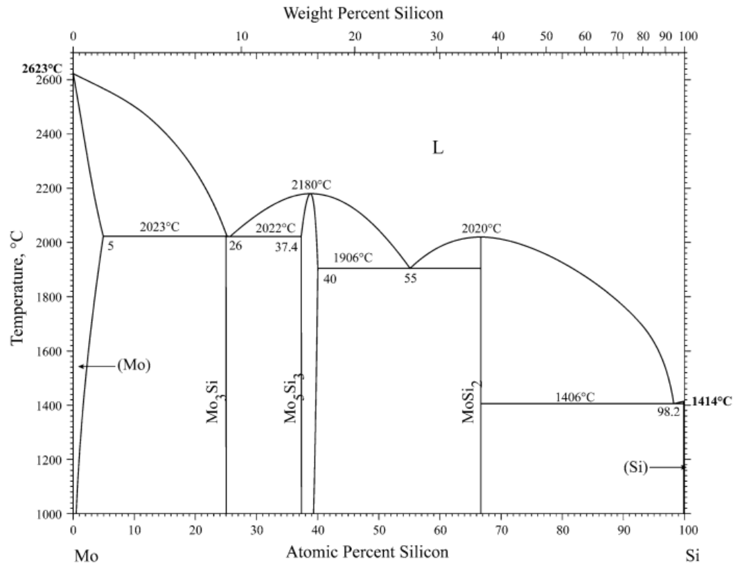
Figure 49.1 Mo-Si phase diagram [89].
