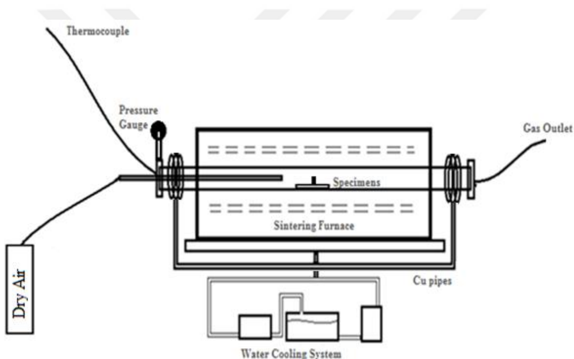
Figure 13 Schematic illustration of the system used in high temperature oxidation tests.
