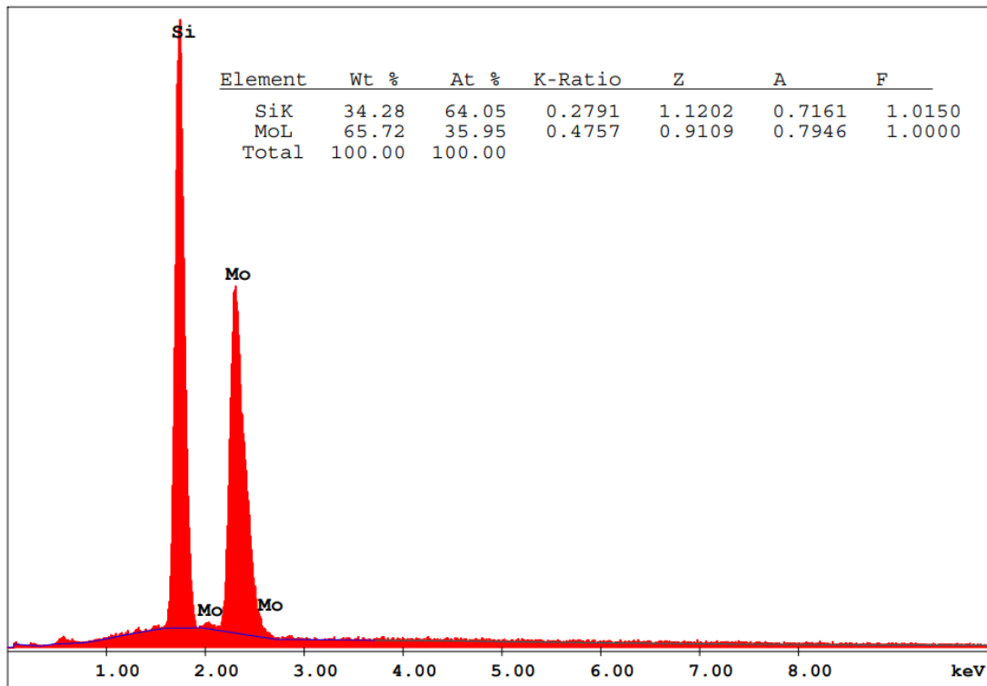
Figure 35 EDS analysis of oxidized coated pure molybdenum sample at 800°C for 6 hours.
