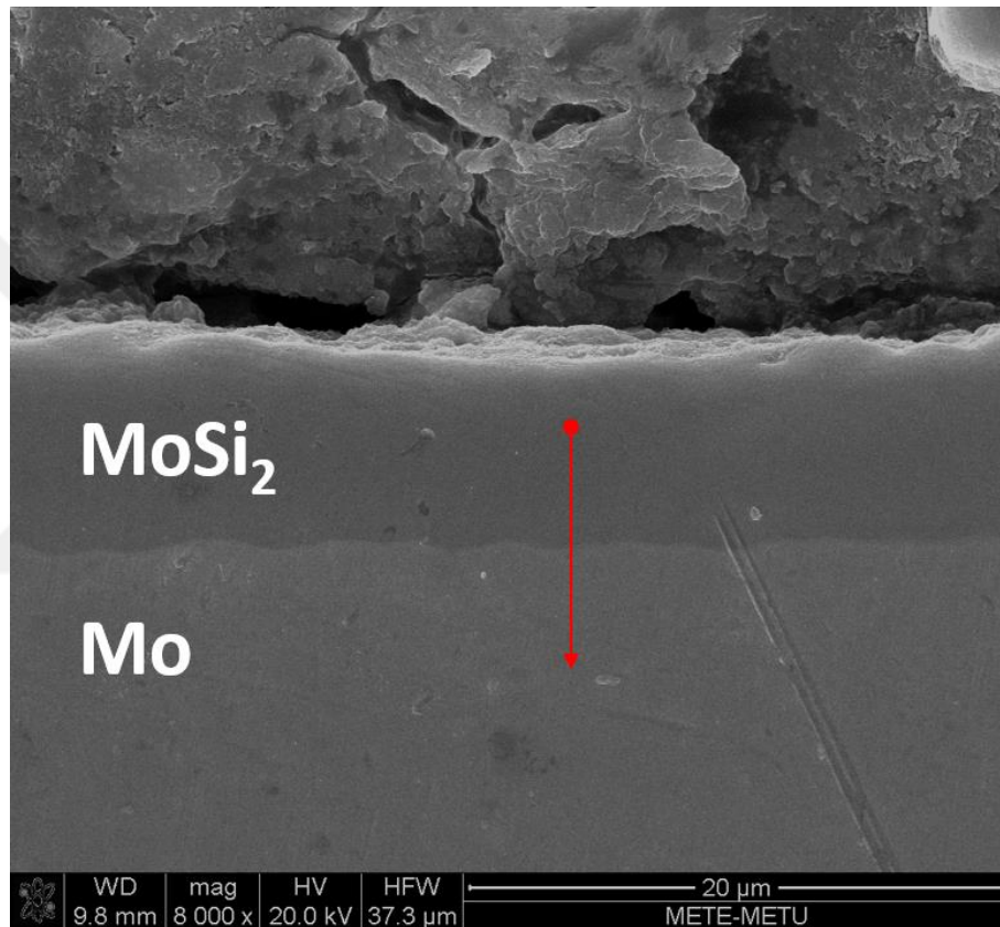
Figure 16 SEM image of the section of silicide coated pure molybdenum sample at 800°C for 10 hours and line on which EDS line analysis was done.
