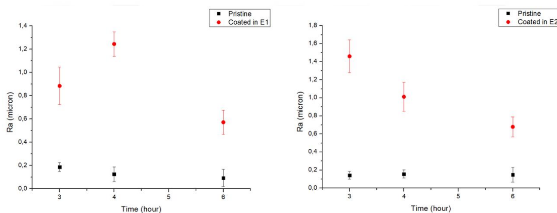
Figure 33 The change of average surface roughness of TZM Alloy samples that coated in E1 and E2 mixture at 900°C.
