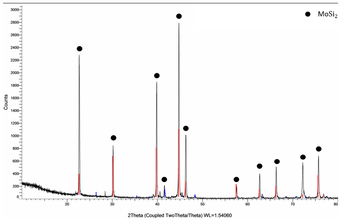
Figure 23 X-Ray Diffraction result of TZM Alloy sample coated at 800°C for 3 hours.
