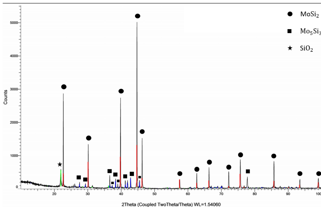
Figure 48 X-Ray Diffraction result of oxidized coated TZM Alloy sample at 1200°C for 3 hours.
