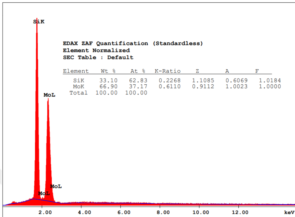
Figure 47 EDS analysis of oxidized coated TZM Alloy sample at 1200°C for 3 hours.
