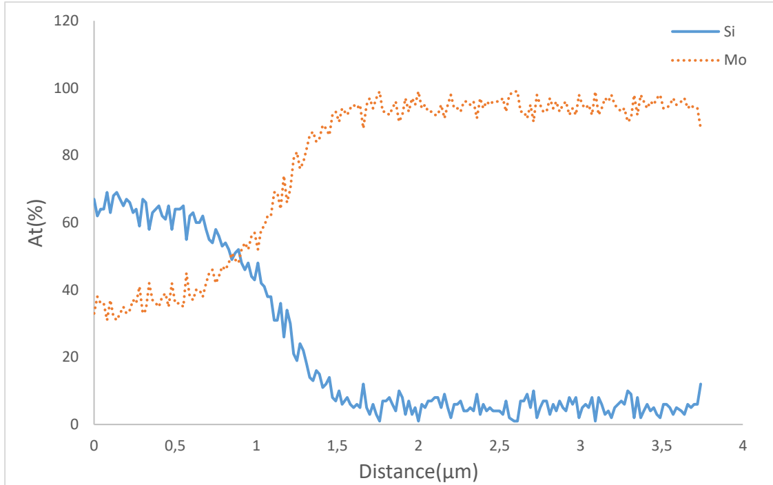
Figure 39 Silicon and molybdenum dispersion results obtained by line analysis in scanning electron microscope.
