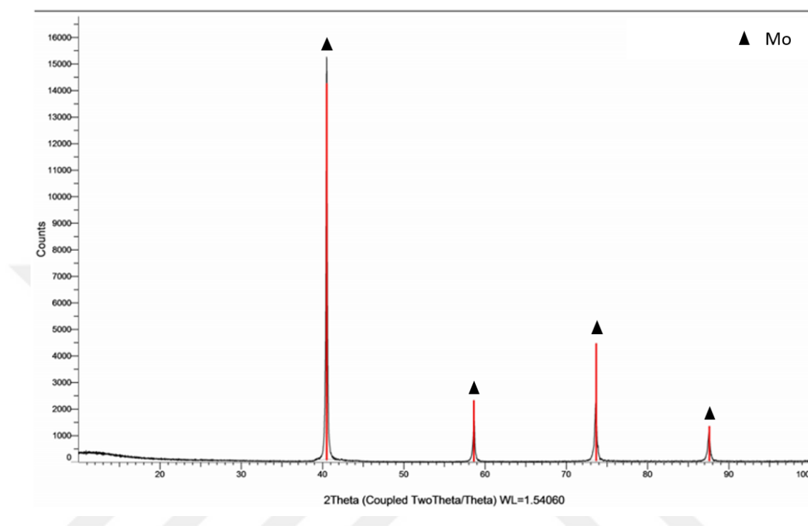
Figure 8 X-Ray Diffraction result of pure molybdenum sample before the experiment.
