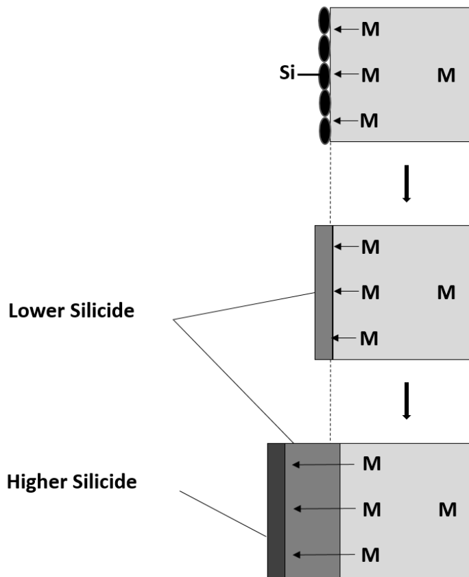
Figure 4 Mechanism of lower and higher silicide formation on non-refractory metals. Reproduced from reference [32].
