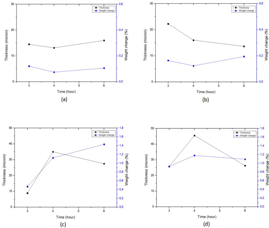
Figure 31 The relationship between mass change and coating thickness over time for the coated TZM Alloy samples: (a) at 900°C, (b) E2 mixture at 900°C, (c) at 800°C and (d) E2 mixture at 800°C.
