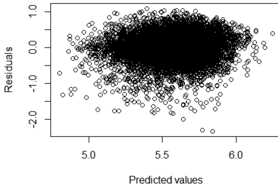
Figure C 4 Predicted values vs. Residuals of LMM of FFD (oral reading)
