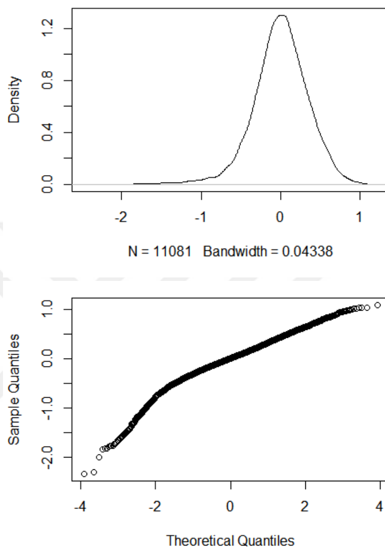
Figure C 3 Distribution of the residuals of LMM of FFD (oral reading)
