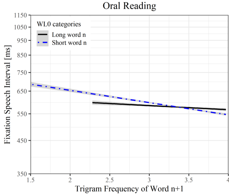
Figure 5.5 The interaction effect of WL0 and TF2 on FSI values. Units of FSI on the y-axis are log-transformed values of FSI, and units of TF2 on the x-axis are log-10 transformed values of frequency per million. The categories of WL0 are short word n (4-8 characters), and long word n (10-14 characters). Line and 95% confidence band (shown in grey) are partial effects, retrieved from LMM estimates by using the remef package (Hohenstein & Kliegl, 2015).
