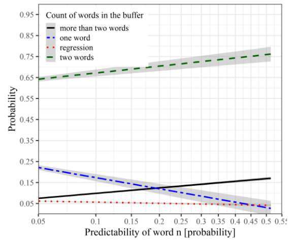
Figure D 5 The effect of P0 on memory buffer load.
