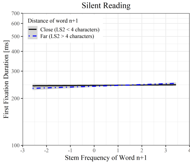
Figure 5.25 The interaction effect of LS2 and SF2 on FFD during silent reading. Units of FFD on the y-axis are log-transformed values, and units of SF2 on the x-axis are log-10 transformed values of frequency per million. Line and 95% confidence band (shown in grey) are partial effects, retrieved from LMM estimates by using the remef package (Hohenstein & Kliegl, 2015).
