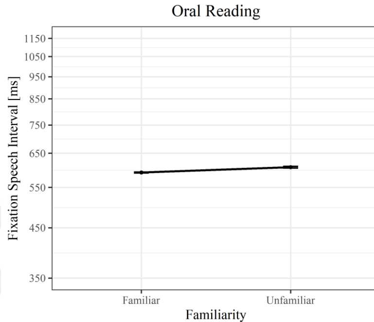
Figure 5.7 The effect of familiarity on FSI values. Units of FSI on the y-axis are log-transformed values of FSI. The partial effect of familiarity was retrieved from LMM estimates by using the remef package (Hohenstein & Kliegl, 2015).
