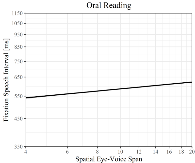
Figure 5.2 The effect of EVS on FSI values. Units of EVS on the x-axis and of FSI on the y-axis are log-transformed values of EVS (base 2) and FSI. Line and 95% confidence band are partial effects, retrieved from LMM estimates by using the remef package (Hohenstein & Kliegl, 2015).
