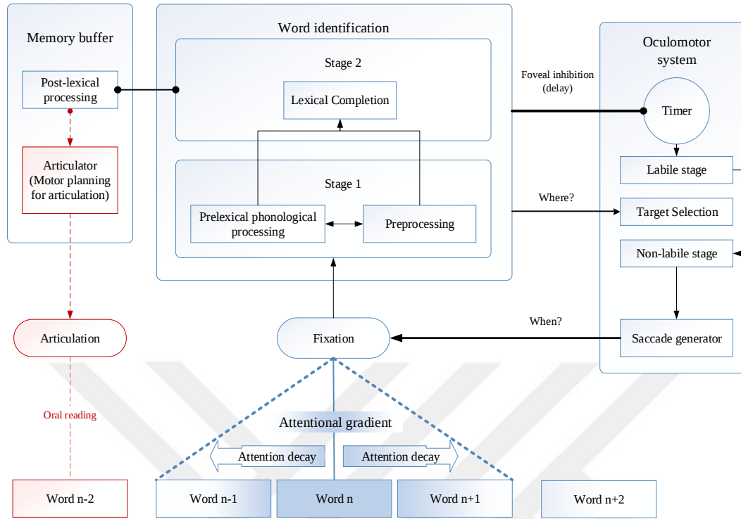
Figure 3.1 Illustration of the P-GAG (Phonological-Mediation in Guidance by Attentional Gradient) model of reading.
