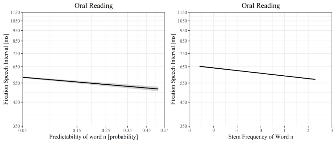
Figure 5.3 The effects of P0 and SF0 on FSI values. Units of FSI on the y-axis are log-transformed values of FSI. Units of SF0 on the x-axis are log-10 transformed values of frequency per million. Units of P0 on the x-axis are logit-transformed values of probabilities. Line and 95% confidence band (shown in gray) are partial effects, retrieved from LMM estimates by using the remef package (Hohenstein & Kliegl, 2015).
