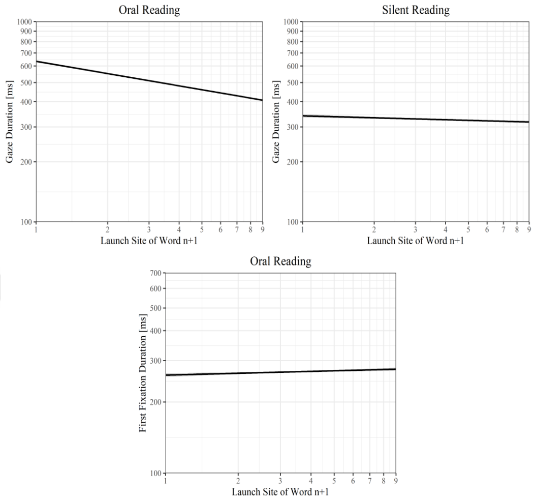
Figure 5.24 The effect of LS2 on fixation durations. Units of fixation durations on the y-axis are log-transformed values. Units of LS2 on the x-axis are log-transformed (base 2) values. Line and 95% confidence band (shown in grey) are partial effects, retrieved from LMM estimates by using the remef package (Hohenstein & Kliegl, 2015).
