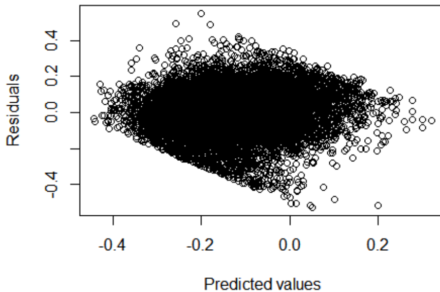
Figure C 8 Predicted values vs. Residuals of LMM of RFLP (oral reading)
