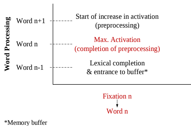
Figure 5.9 Illustration of processing of word n-1, word n, and word n+1 during fixation n, according to P-GAG assumptions.
