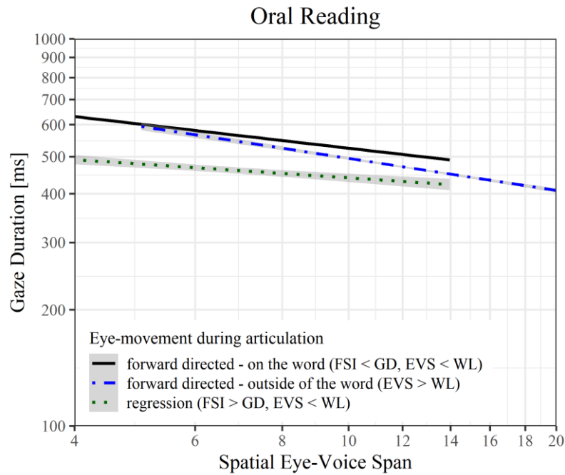
Figure 5.11 The interaction effect of EVS and FSI on GD. Units of GD on the y-axis and units of EVS on the x-axis are log-transformed values of them. Line and 95% confidence band (shown in grey) are partial effects, retrieved from LMM estimates by using the remef package (Hohenstein & Kliegl, 2015).
