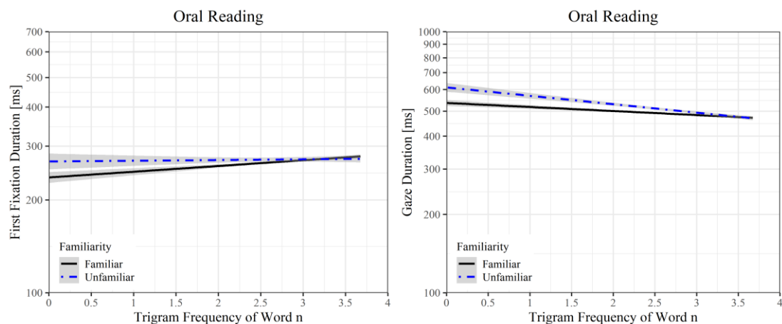
Figure 5.29 The interaction effect of familiarity and TF0 on fixation durations during reading aloud. Units of fixation durations on the y-axis are log-transformed values, and units of TF0 on the x-axis are log-10 transformed values of frequency per million. Line and 95% confidence band (shown in grey)
