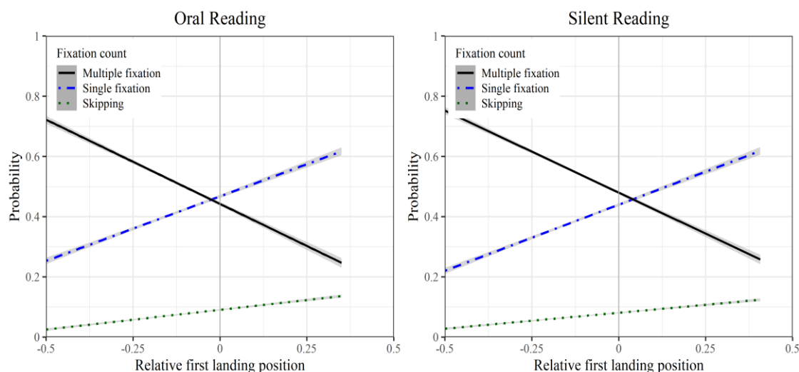
Figure 5.13 The relationship between fixation count probabilities and RFLP. RFLP values of 0 indicate the middle, RFLP values below 0 indicate the left half, and RFLP values above 0 indicate the right half of the word n. Line and 95% confidence band (shown in grey) are calculated over raw data using the ggplot2 package (Wickham, 2009).
