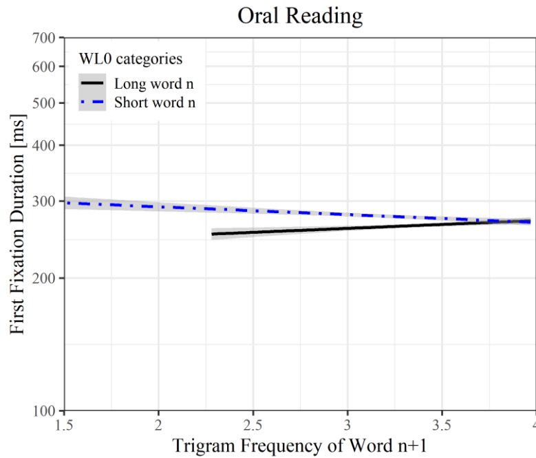
Figure 5.23 The interaction effect of WL0 and TF2 on FFD during oral reading. The units of FFD on the y-axis are log-transformed values, and units of TF2 on the x-axis are log-10 transformed values of frequency per million. The categories of WL0 are short word n (4-8 characters), and long word n (10-14 characters). Line and 95% confidence band (shown in grey) are partial effects, retrieved from LMM estimates by using the remef package (Hohenstein & Kliegl, 2015).
