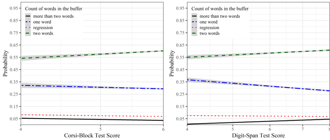
Figure D 2 Memory test scores and the memory buffer load.
