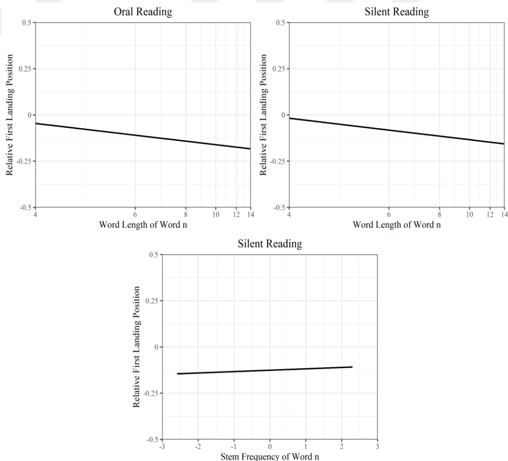
Figure 5.33 The effects of WL0 (both modalities) and SF0 (silent reading) on RFLP. RFLP values of 0 indicate the center, RFLP values below 0 indicate the left half, and RFLP values above 0 indicate the right half of the word n . Units of WL0 on the reversed x-axis are reciprocal lengths of word n . Units of SF0 on the x-axis are log-10 transformed values of frequencies per million. Line and 95% confidence band (shown in grey) are partial effects, retrieved from LMM estimates by using the remef package (Hohenstein & Kliegl, 2015).
