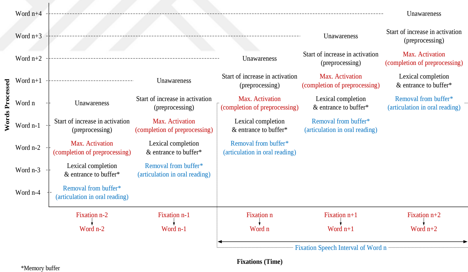
Figure 3.2 Illustration of processing in five successive fixations on five successive words according to P-GAG.
