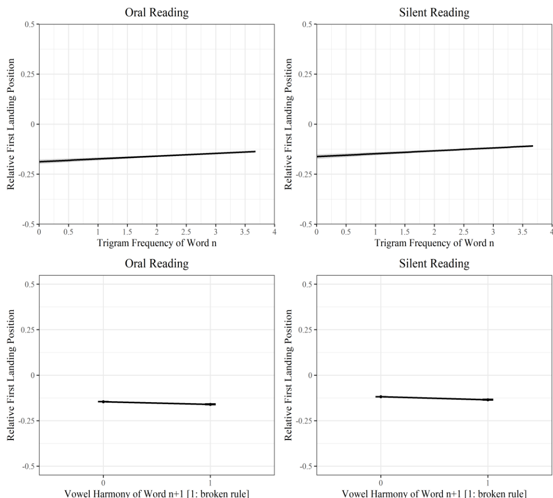
Figure 5.36 The effect of TF0 and VH2 on RFLP. RFLP values of 0 indicate the center, RFLP values below 0 indicate the left half, and RFLP values above 0 indicate the right half of the word n . Units of TF0 on the x-axis are log-10 transformed values of frequency per million. Line and 95% confidence band (shown in grey) are partial effects of TF0. The partial effects of TF0 and VH2 were retrieved from LMM estimates by using the remef package (Hohenstein & Kliegl, 2015).
