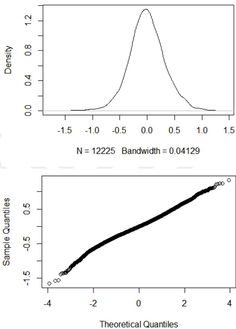
Figure C 11 Distribution of the residuals of LMM of GD (Silent Reading)
