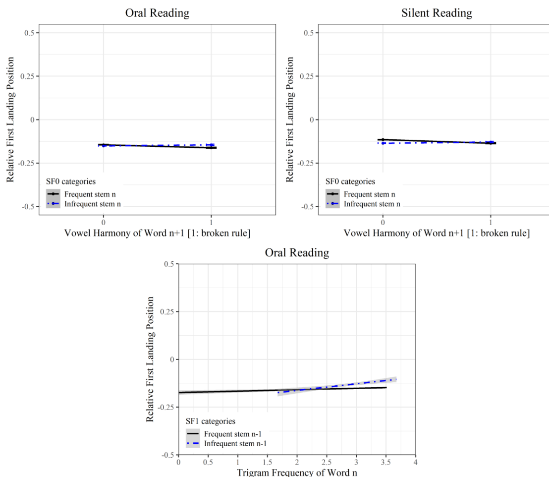
Figure 5.40 The interaction effects of SF0 and VH2, and SF1 and TF0 on RFLP. RFLP values of 0 indicate the center, RFLP values below 0 indicate the left half, and RFLP values above 0 indicate the right half of the word n . Units of TF0 on the x-axis are log-10 transformed values of frequency per million. Categories of SFs are frequent stems ( SF > 1.17 ) and infrequent stems ( SF < 1.17 ). Line and 95% confidence band (shown in grey) are partial effects of TF0. The partial effects of TF0 and VH2 were retrieved from LMM estimates by using the remef package (Hohenstein & Kliegl, 2015).
