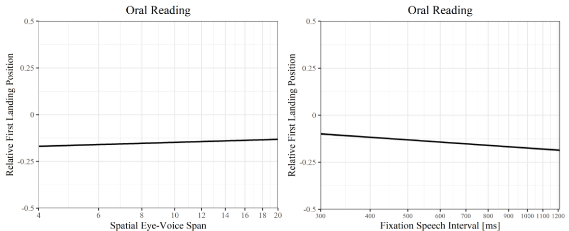
Figure 5.31 The effects of EVS and FSI on RFLP. RFLP values of 0 indicate the center, RFLP values below 0 indicate the left half, and RFLP values above 0 indicate the right half of the word n . Units of EVS and FSI on the x-axis are log-transformed values. Line and 95% confidence band (shown in grey) are partial effects, retrieved from LMM estimates by using the remef package (Hohenstein & Kliegl, 2015).
