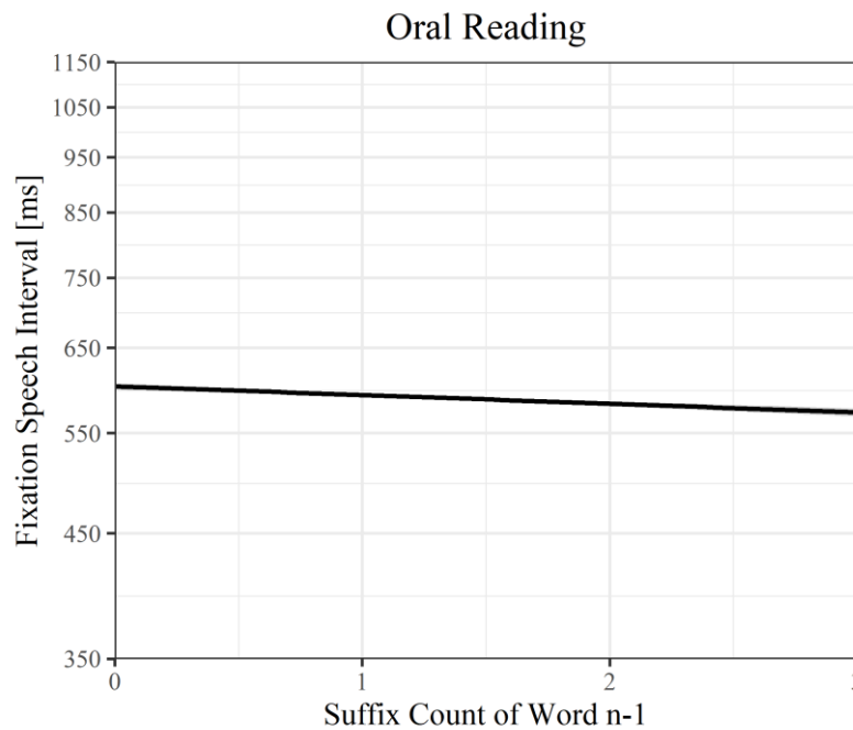
Figure 5.8 The effect of SC1 on FSI values. Units of FSI on the y-axis are log-transformed values of FSI. Line and 95% confidence band (shown in grey) are partial effects, retrieved from LMM estimates by using the remef package (Hohenstein & Kliegl, 2015).
