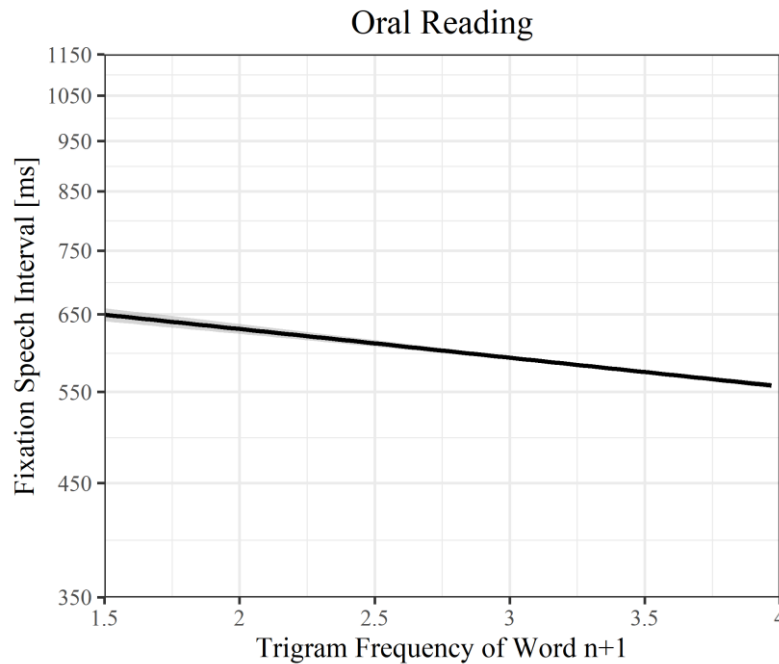
Figure 5.4 The effect of TF2 on FSI values. Units of FSI on the y-axis are log-transformed values of FSI, and units of TF2 on the x-axis are log-10 transformed values of frequency per million. Line and 95% confidence band (shown in grey) are partial effects, retrieved from LMM estimates by using the remef package (Hohenstein & Kliegl, 2015).
