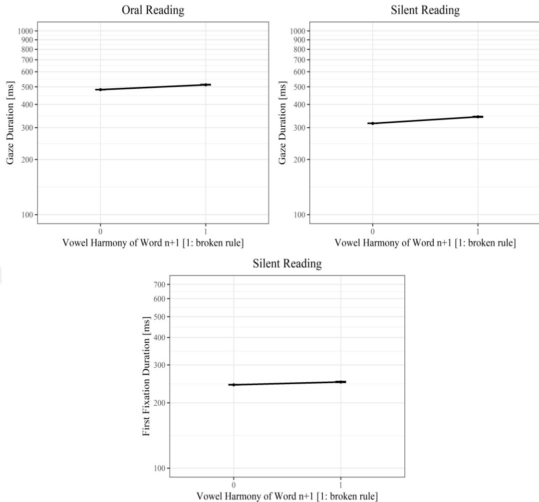
Figure 5.22 The effect of VH2 on fixation durations. Units of fixation durations on the y-axis are log-transformed values. The partial effect of VH2 was retrieved from LMM estimates by using the remef package (Hohenstein & Kliegl, 2015).
