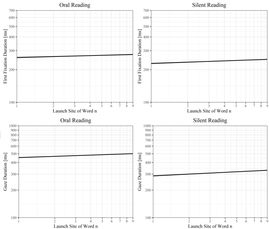
Figure 5.14 The effect of LS0 on fixation durations. Units of fixation durations on the y-axis are log-transformed values. Units of LS0 on the x-axis are log-transformed (base 2) values. Line and 95% confidence band (shown in grey) are partial effects, retrieved from LMM estimates by using the remef package (Hohenstein & Kliegl, 2015).
