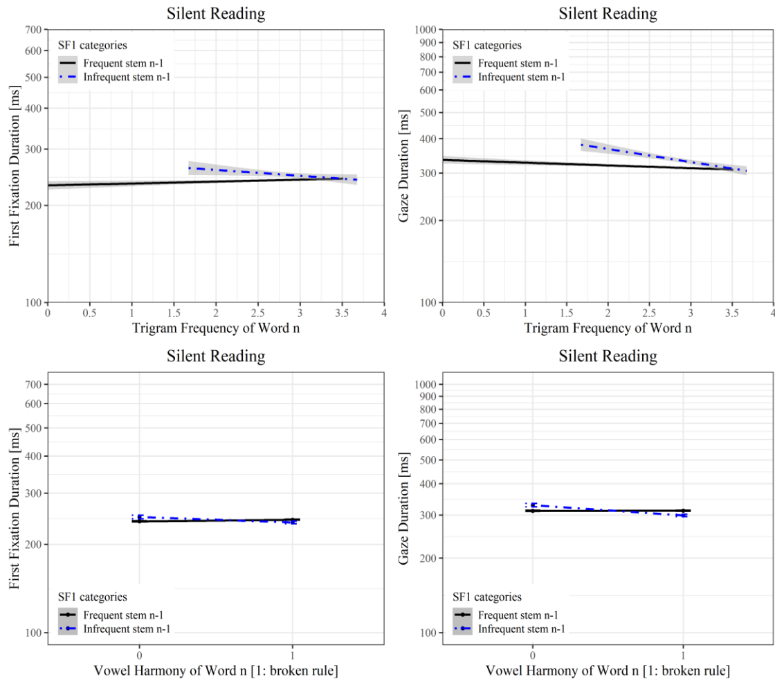
Figure 5.27 The interaction effect of SF1 and TF0, and that of SF1 and VH0 on fixation durations. Units of fixation durations on the y-axis are log-transformed values, and units of TF0 on the x-axis are log-10 transformed values of frequency per million. Categories of SF1 are frequent stems ( SF1 > 1.17 ), and infrequent stems ( SF1 < 1.17 ). Line and 95% confidence band (shown in grey) and the means in the categories of VH0 are partial effects, retrieved from LMM estimates by using the remef package (Hohenstein & Kliegl, 2015).
