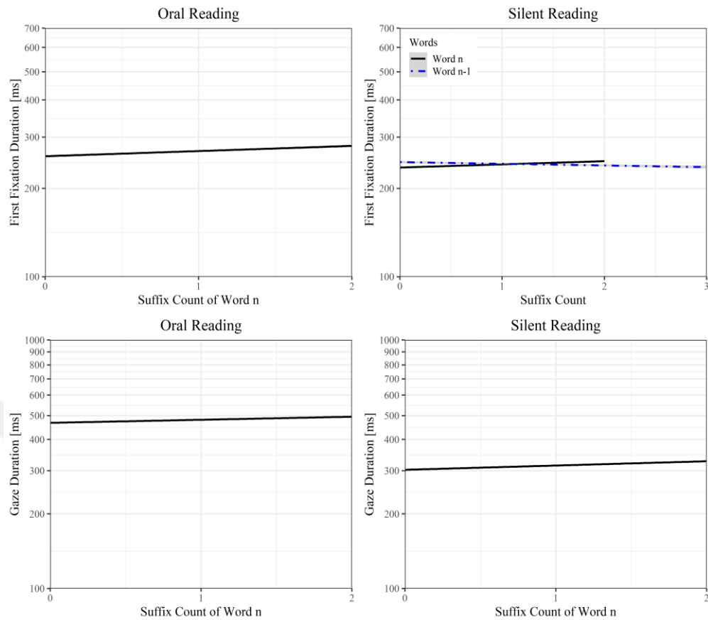
Figure 5.30 The effects of suffix counts on fixation durations. Units of fixation durations on the y-axis are log-transformed values. Line and 95% confidence band (shown in grey) are partial effects, retrieved from LMM estimates by using the remef package (Hohenstein & Kliegl, 2015).
