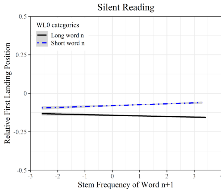
Figure 5.37 The interaction effect of WL0 and SF2 on RFLP. RFLP values of 0 indicate the center, RFLP values below 0 indicate the left half, and RFLP values above 0 indicate the right half of the word n . Units of SF2 on the x-axis are log-10 transformed values of frequency per million. Categories of WL0 are short words (4-8 characters) and long words (10-14 characters). Line and 95% confidence band (shown in grey) are partial effects retrieved from LMM estimates by using the remef package (Hohenstein & Kliegl, 2015).
