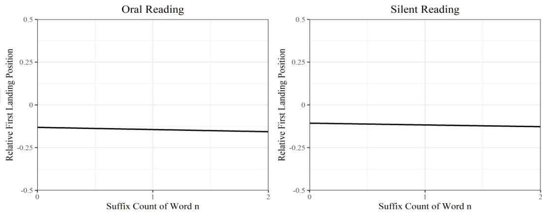
Figure 5.41 The effect of SC0 on RFLP. RFLP values of 0 indicate the center, RFLP values below 0 indicate the left half, and RFLP values above 0 indicate the right half of the word n . Line and 95% confidence band (shown in grey) are partial effects, retrieved from LMM estimates by using the remef package (Hohenstein & Kliegl, 2015).
