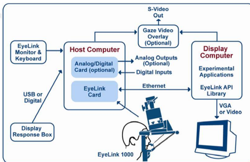
Figure 4.1 SR Research EyeLink 1000 Tower Mount (EyeLink 1000 User Manual version 1.5.0, Figure 1-1, p. 2).
