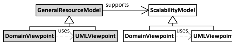
Figure 7: Conceptual model representing relation between General Resource Model and Scalability Model
