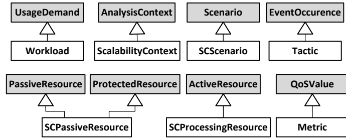
Figure 11: The relationship between the scalability concepts and GRM
