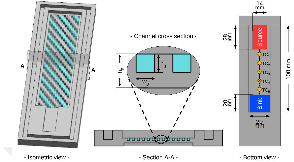
Figure 4.1: Multichannel heat pipe model
