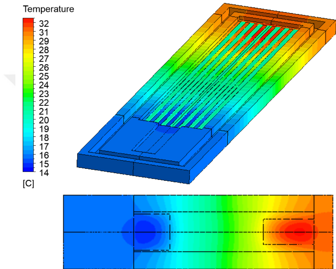
Figure 4.4: Temperature distribution on the G-1600 model for the 21\text{kW/m}^2 heat load
