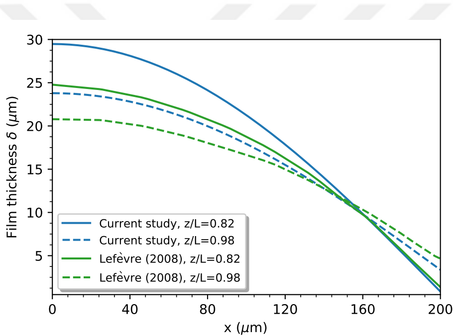
Figure 2.9: Liquid film thickness variations for the current study and validation case-2 for the different axial positions
