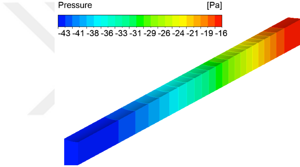
Figure 2.16: Pressure distribution along the channel
