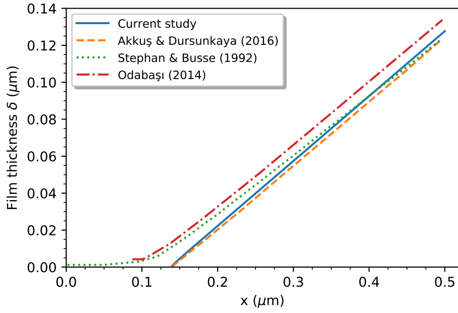
Figure 2.5: Comparison of film thickness variations in micro-region
