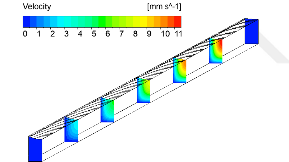
Figure 2.18: Velocity distribution at different sections along the channel
