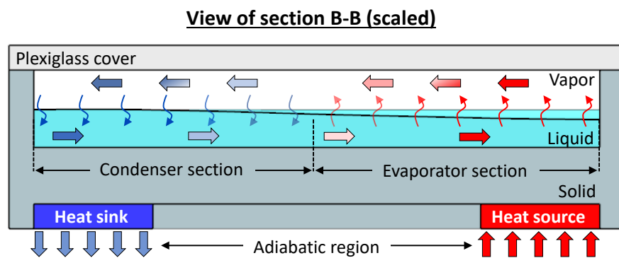
Figure 1.1: Detailed view of a flat grooved heat pipe
