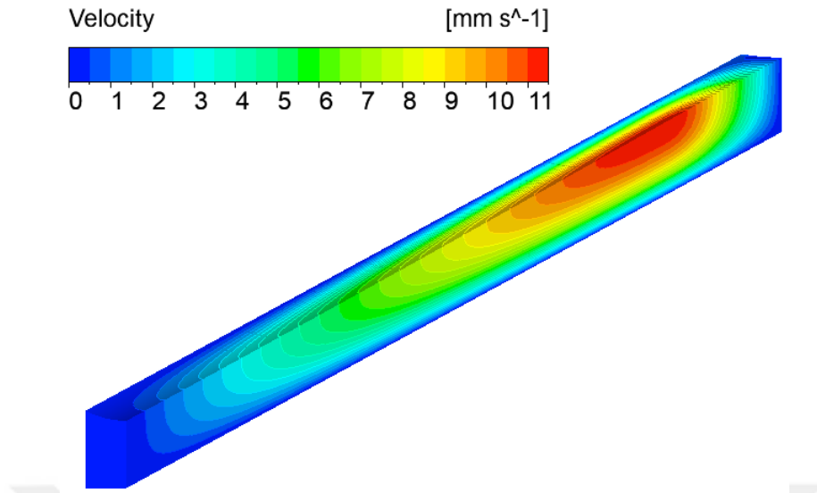
Figure 2.17: Velocity distribution along the channel
