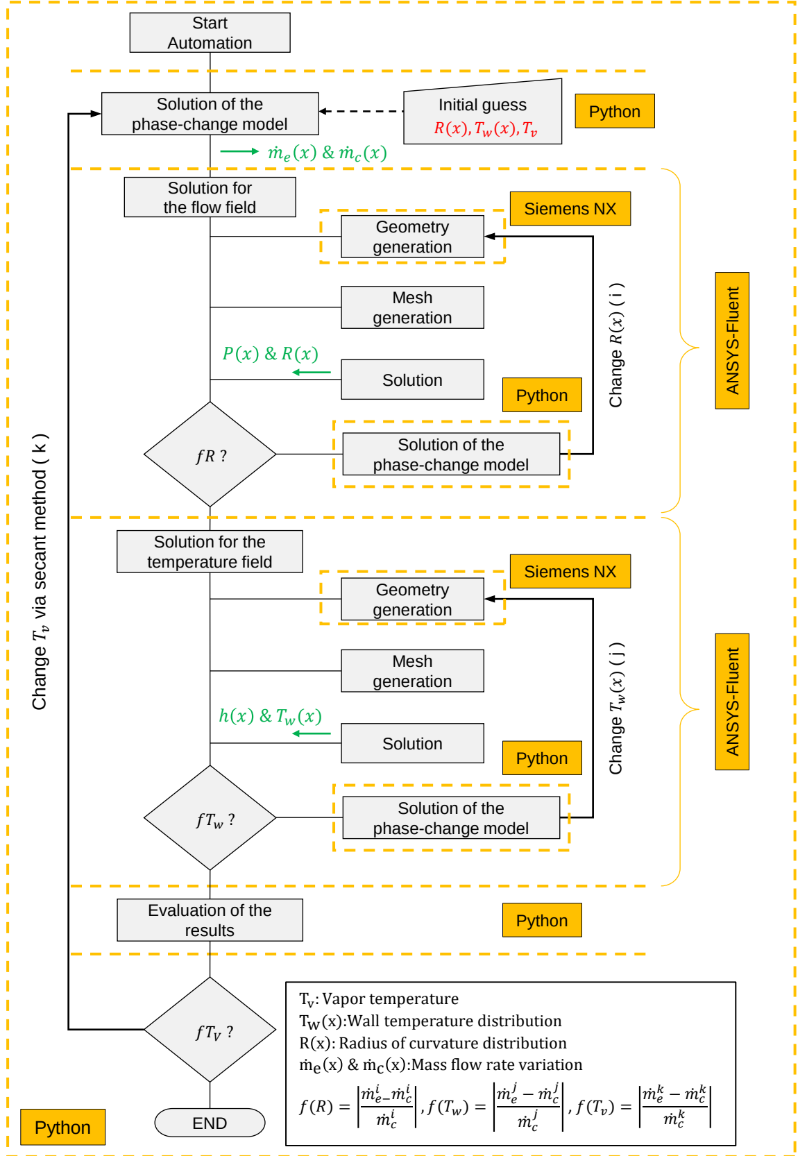
Figure 2.3: Solution procedure
