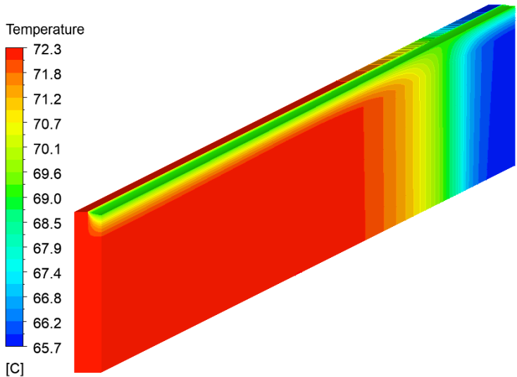
Figure 2.22: Temperature distribution along the channel
