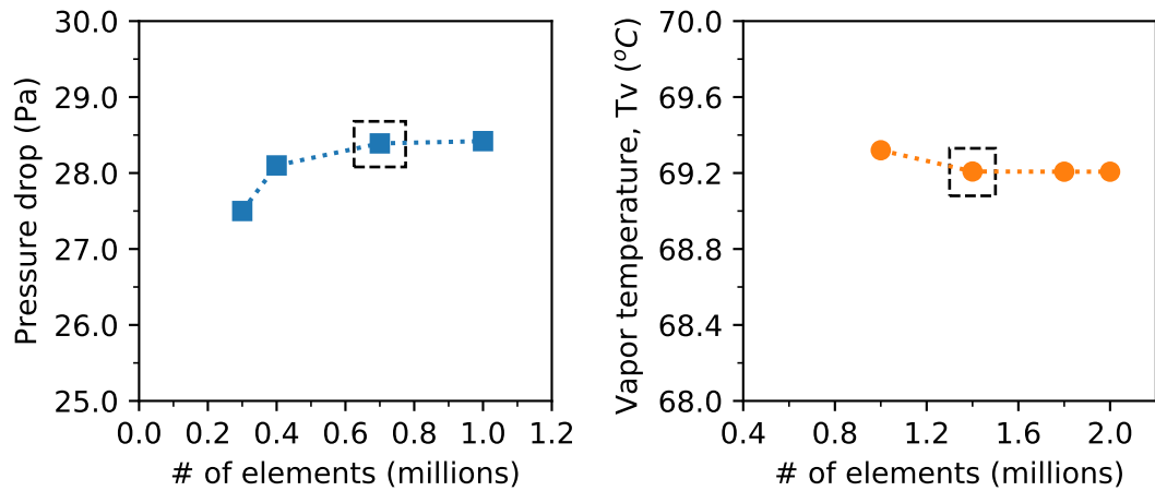
Figure 2.12: Various case studies to find optimum mesh
