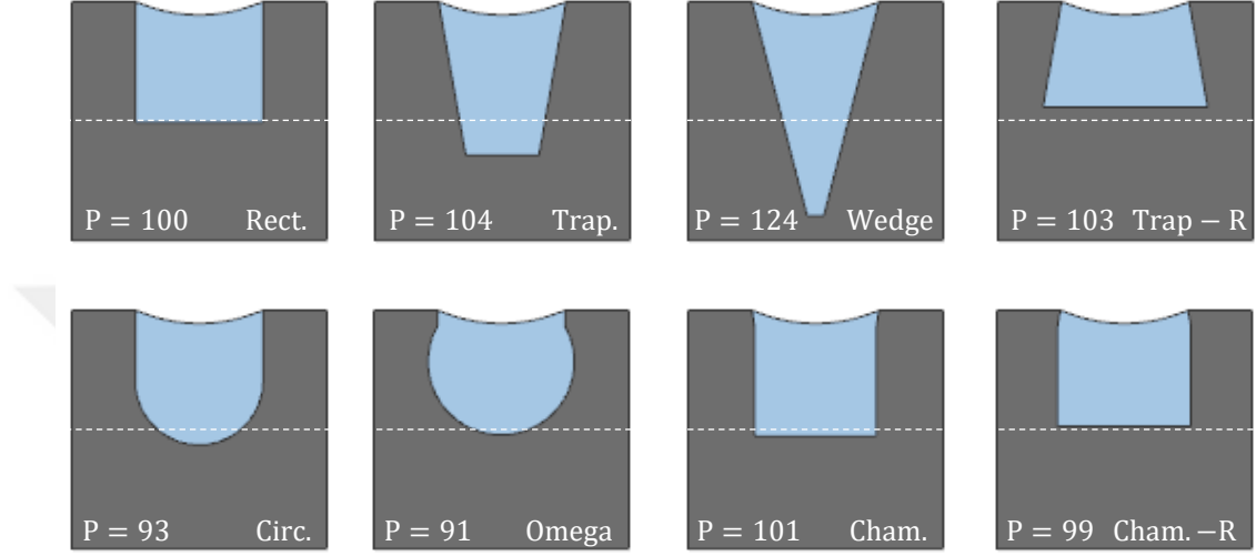
Figure 3.2: Normalized perimeters of various cross-sectional geometries with identical fin top width and cross-sectional area
