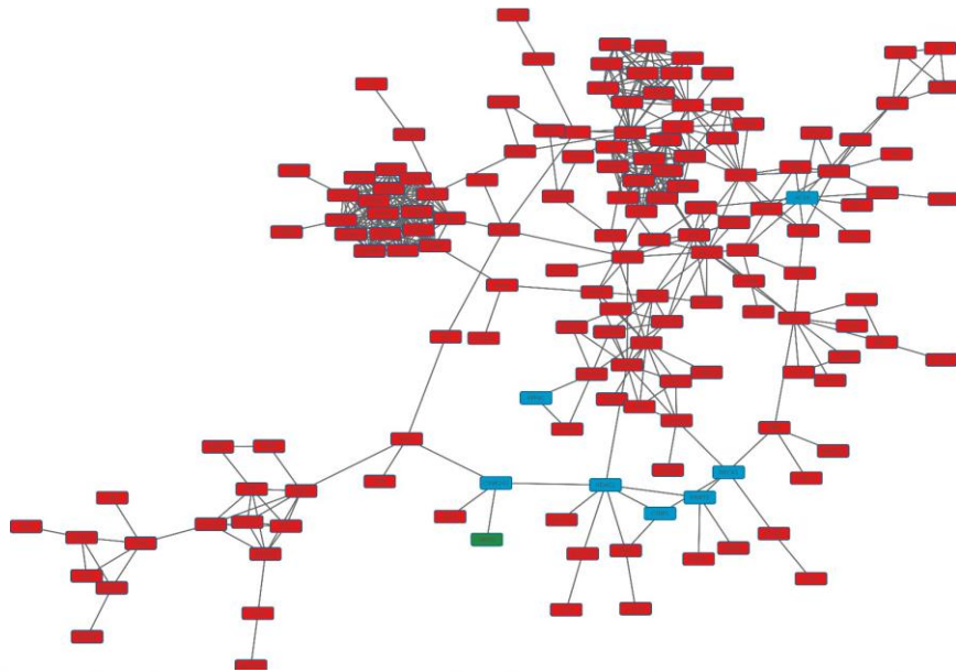
Figure 4.11b. IDH mut pTERTwt - Protein complex focused subnetwork
