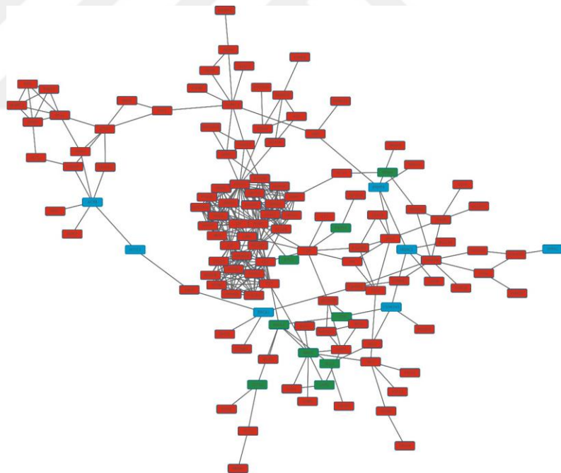
Figure 4.11a. IDH mut pTERTmt - Protein complex focused subnetwork
