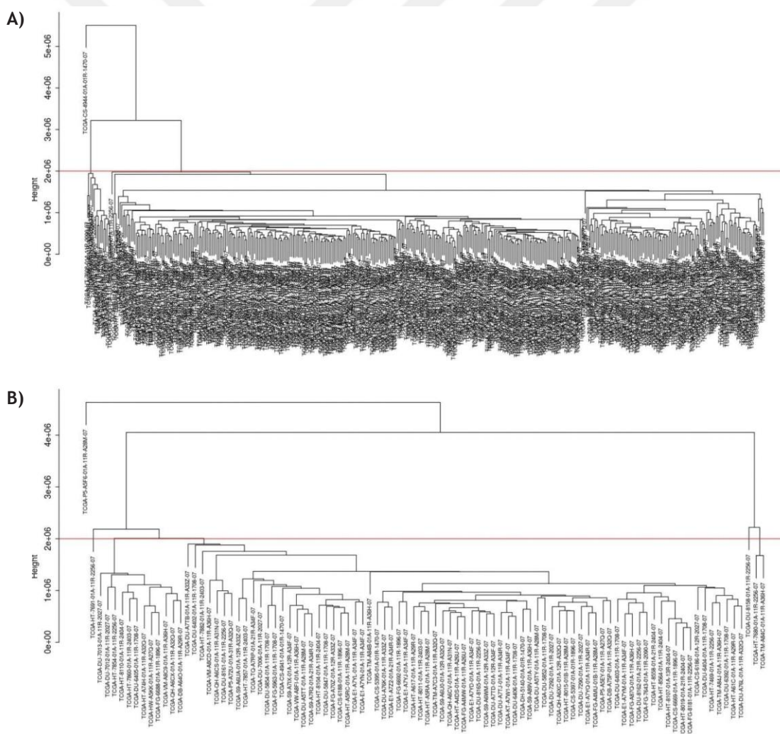
Supplementary Figure 1. Sample clustering of TCGA LGG IDHmt samples by average methodology A) IDHmt samples, B) IDHwt samples
