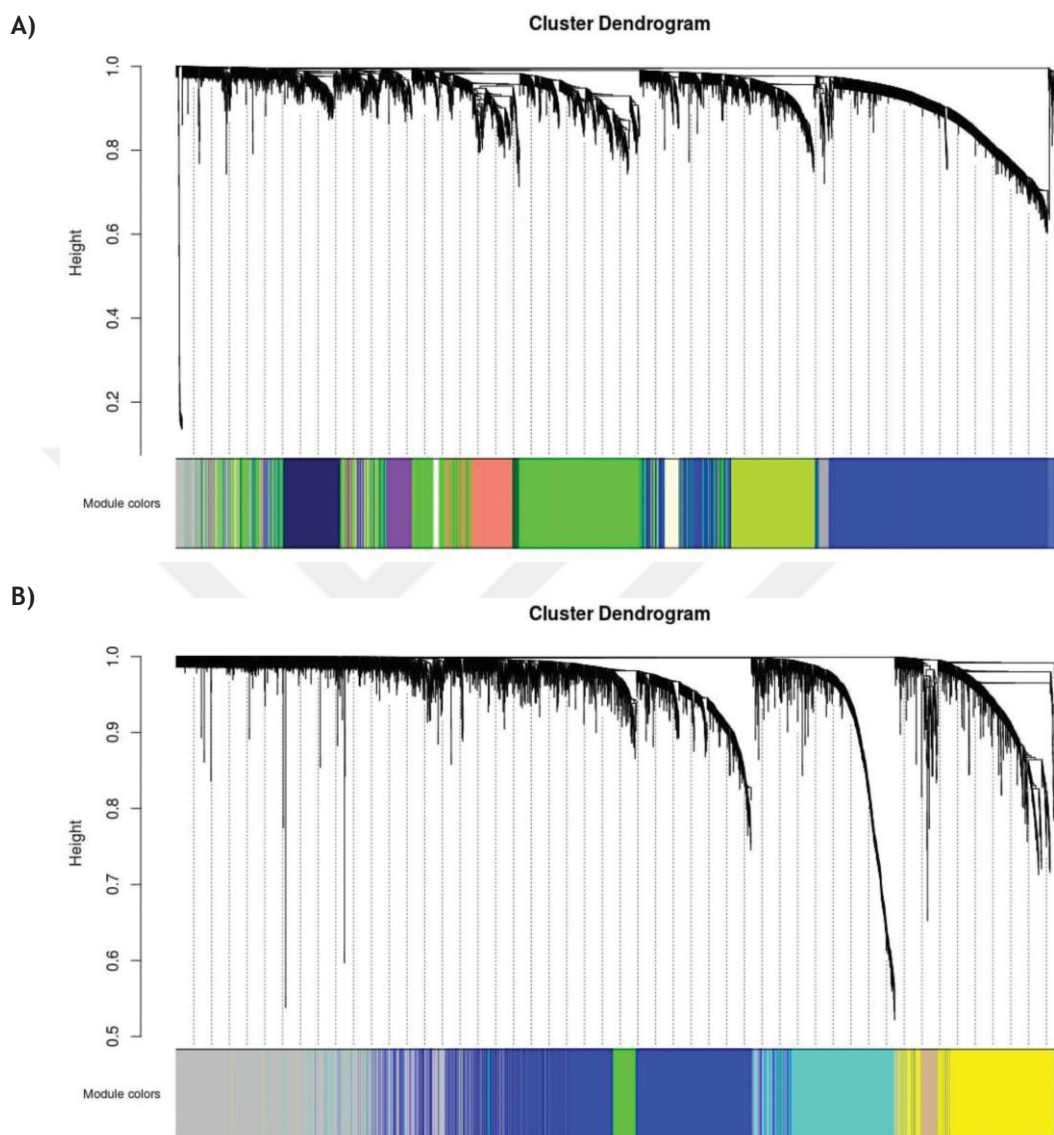
Supplementary Figure 3. Hierarchical clustering of genes with module colors A) IDHmt samples, B) IDHwt samples IDHmt: Isocitrate dehydrogenase mutated, IDHwt: Isocitrate dehydrogenase wild-type
