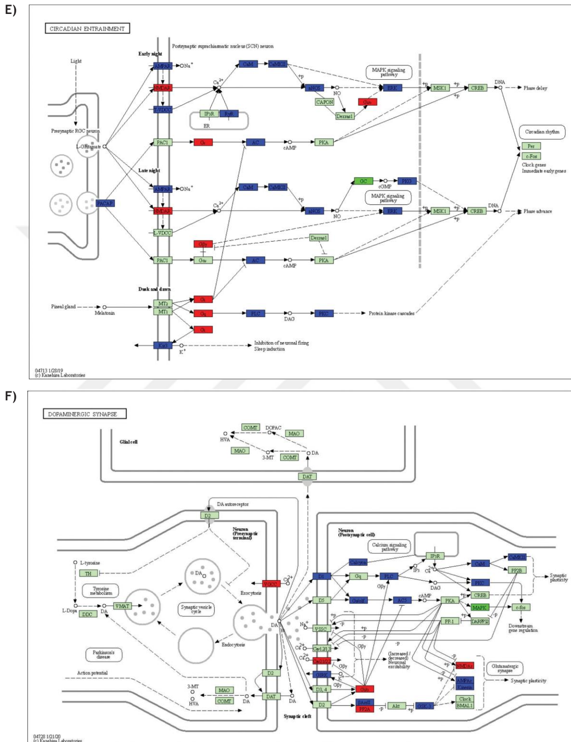
Supplementary Figure 4. Selected common KEGG pathway schemes of the IDHwt pTERT- blue module and IDHmt pTERT+ greenyellow module. A) Glutamatergic synapse, B) Retrograde endocannabinoid signaling, C) GABAergic synapse, D) Cholinergic synapses, E) Circadian entrainment, F) Dopaminergic synapse
