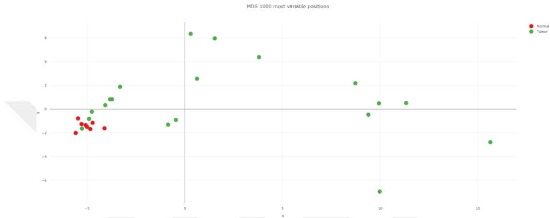
Figure 4.9a. MDS plot of IDH wt pTERTwt samples for IDH wt pTERTwt subtype.
