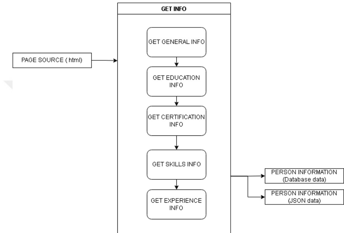
Detailed Profile Information Extraction Flowchart
