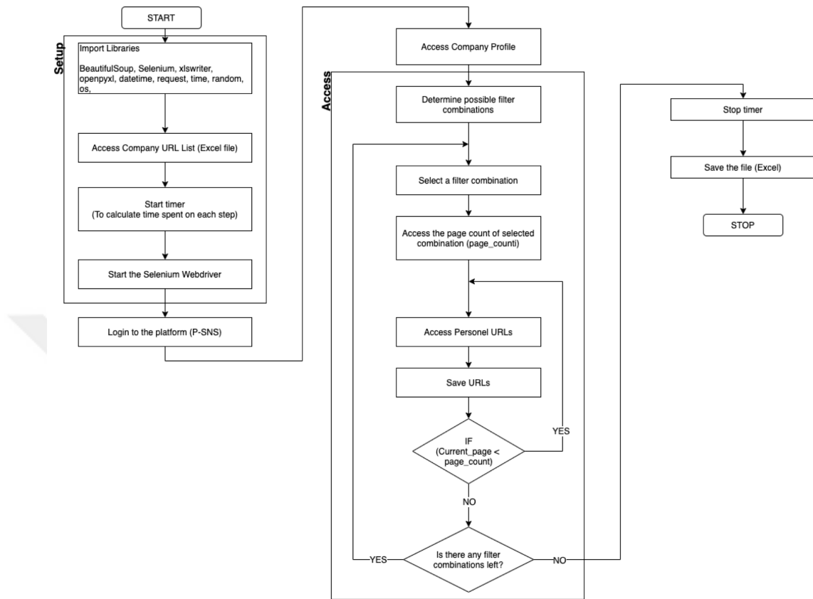
Automated Personnel URL Extraction Process Flowchart
