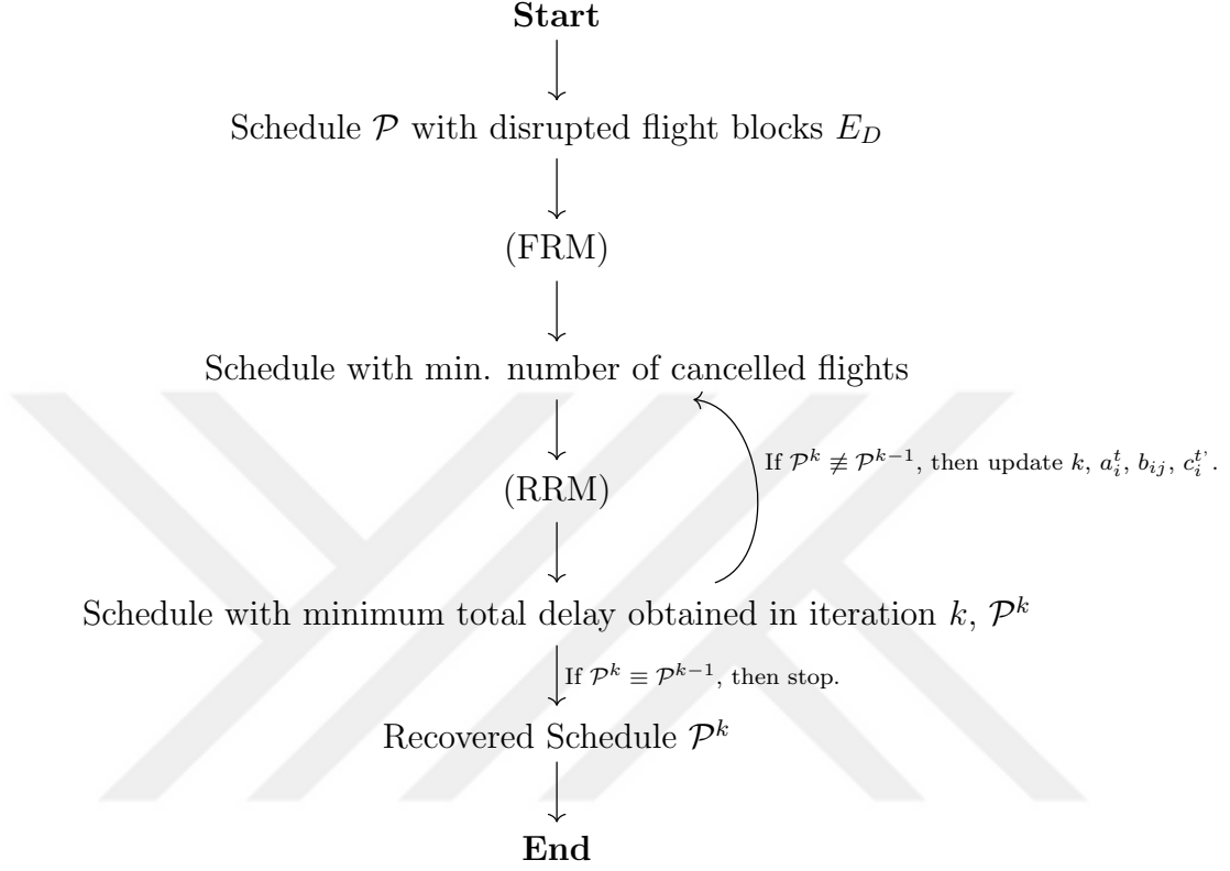
Figure 6.1: Integrated Flight and Passenger Recovery Algorithm
