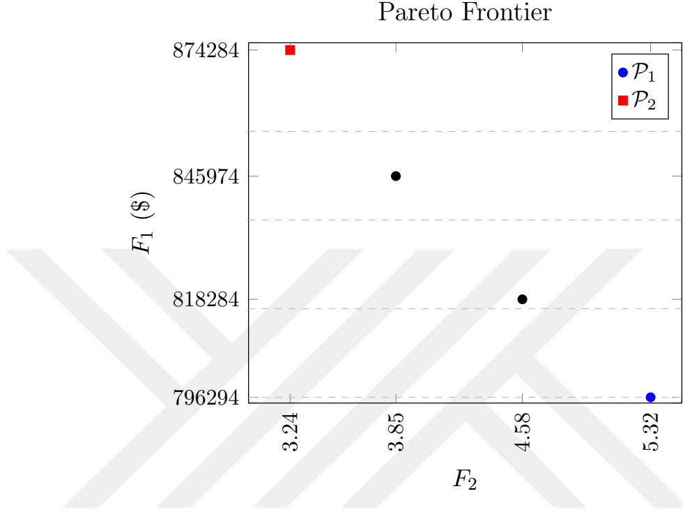
Figure 7.1: Deviation from the Average Variability vs. Total Operational Cost for 50 Flights
