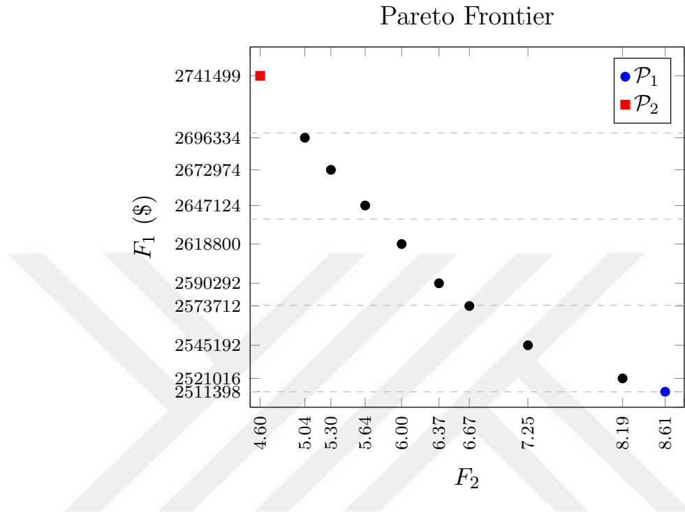
Figure 7.5: Deviation from the Average Variability vs. Total Operational Cost for 150 Flights
