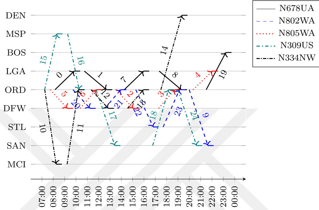
Figure 5.2: Time-Space Network of the Minimum Cost Schedule \mathcal{P}_1
