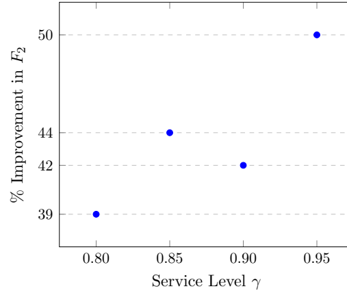
Figure 7.9: Service Level \gamma vs. Improvement in F_2 for 50 Flights
