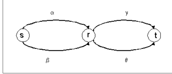
Figure 4.1: Path matchings
