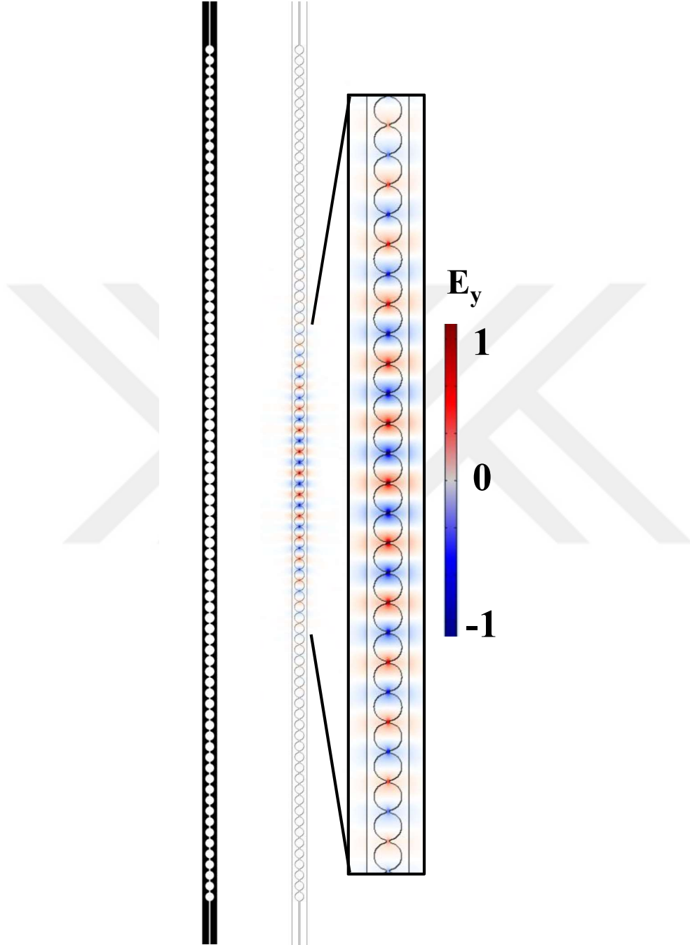
Figure 3.9 FDTD analysis of the designed cavity. (a) The refractive index distribution of the simulation environment. (b) The E_y mode profile of the fundamental resonance of the cavity. Inset: Zoom-in to the cavity center.
