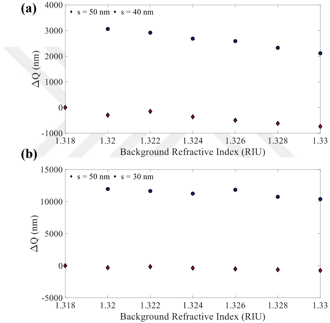
Figure 4.9 The presentation of the Q-factor enhancement of the cavity with an initial slot width of 50 nm for (a) 10 nm (b) 20 nm beam deflection.
