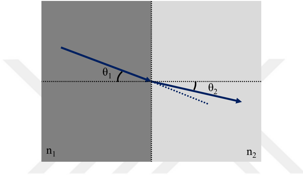
Figure 2.1. Demonstration of the light propagation from one medium to another.
