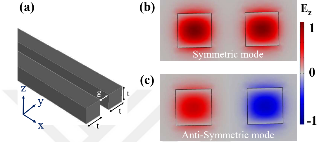
Figure 2.8 Transverse optical force mechanics in two coupled straight waveguide system. (a) The schematic of a coupled two straight waveguide system. (b) Symmetric mode for E_z polarization at a wavelength of 1550 nm. (c) Anti-symmetric mode for E_z polarization at a wavelength of 1550 nm.
