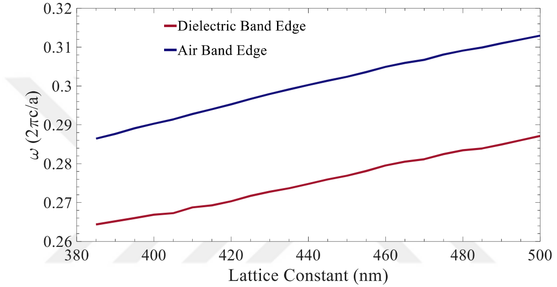
Figure 3.3 The characteristics of band edge frequencies with respect to the lattice constant.
