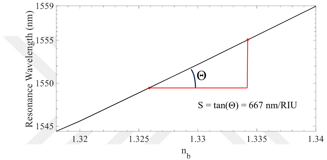
Figure 3.12 The variation of resonance wavelength with respect to the background refractive index.
