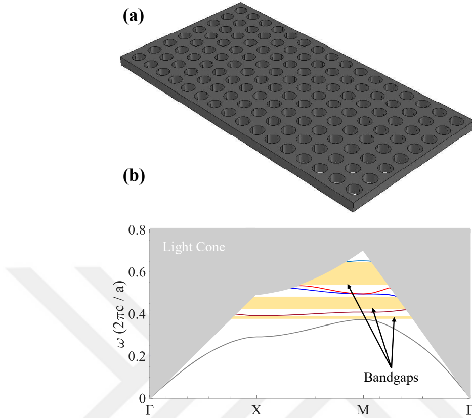
Figure 2.7 2D PhC slab band diagram analysis. (a) Representative schematic of the device geometry. (b) Corresponding band diagram.
