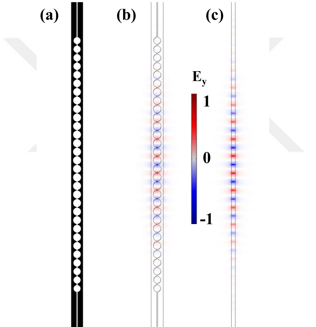
Figure 3.11 FDTD analysis of simplified cavity. (a) The schematic of the simplified configuration. (b) Mode profile in the x-y plane. (c) Mode profile in the x-z plane.
