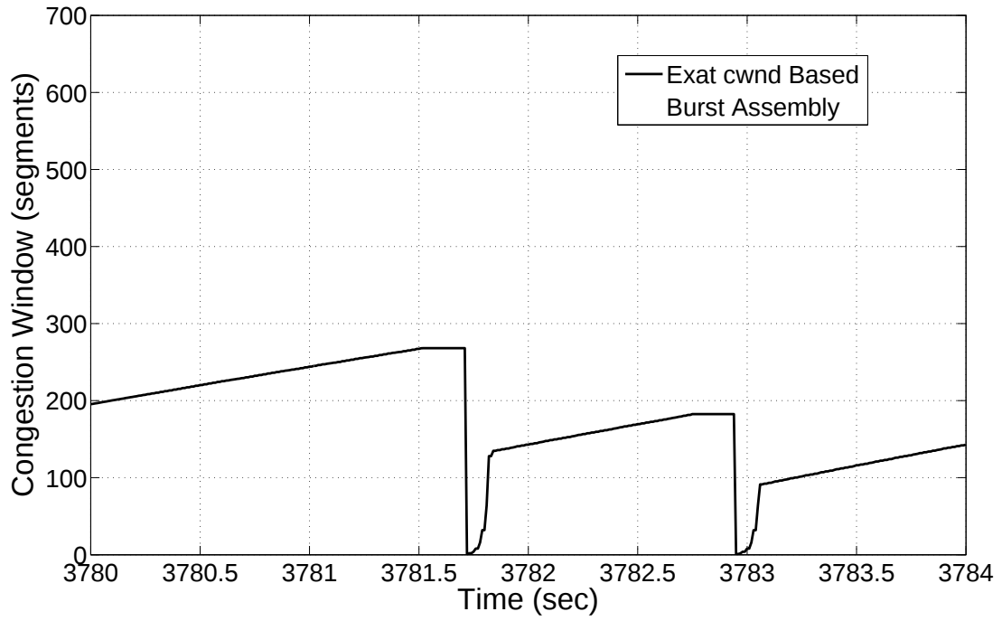
Figure 4.4: Congestion window evolution of CWBA algorithm
