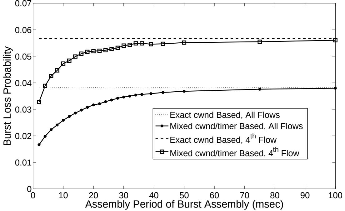
Figure 4.14: Burst loss probabilities for CWBA and MCWBA algorithms in the mesh OBS network topology
