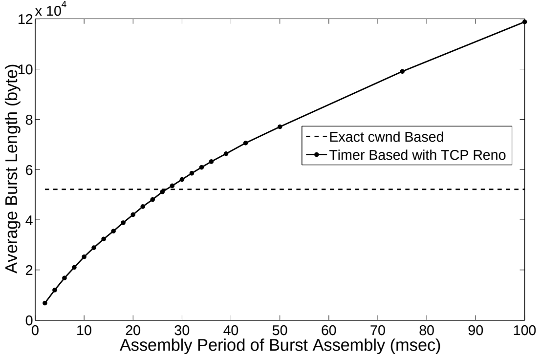
Figure 4.8: Average burst lengths for timer based and CWBA algorithms in the mesh OBS network topology
