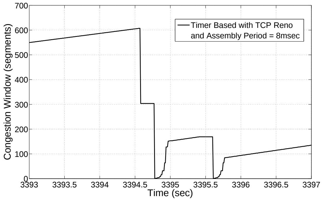
Figure 4.5: Congestion window evolution of timer based assembly algorithm
