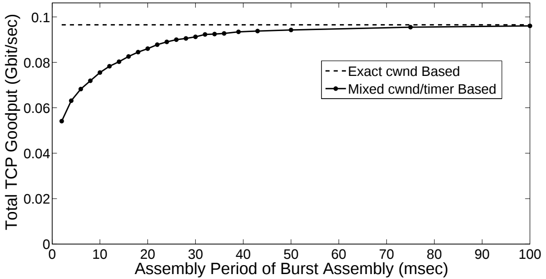
Figure 4.12: TCP performance of CWBA and MCWBA algorithms for the mesh OBS network topology
