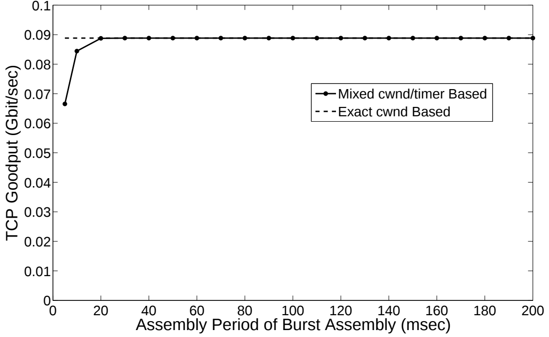
Figure 4.11: TCP performance of CWBA and MCWBA algorithms (pessimistic case) in the simple OBS network topology
