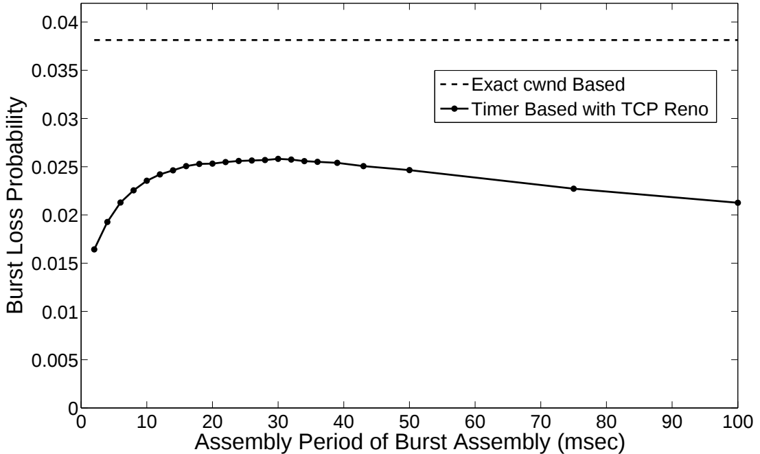
Figure 4.7: Burst loss probabilities for timer based and CWBA algorithms in the mesh OBS network topology
