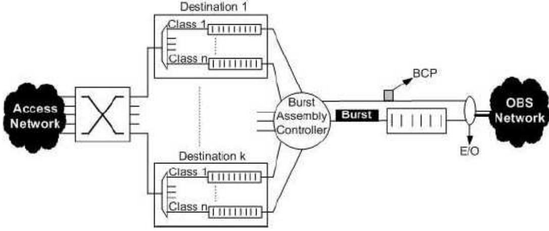
Figure 2.4: OBS ingress node architecture
