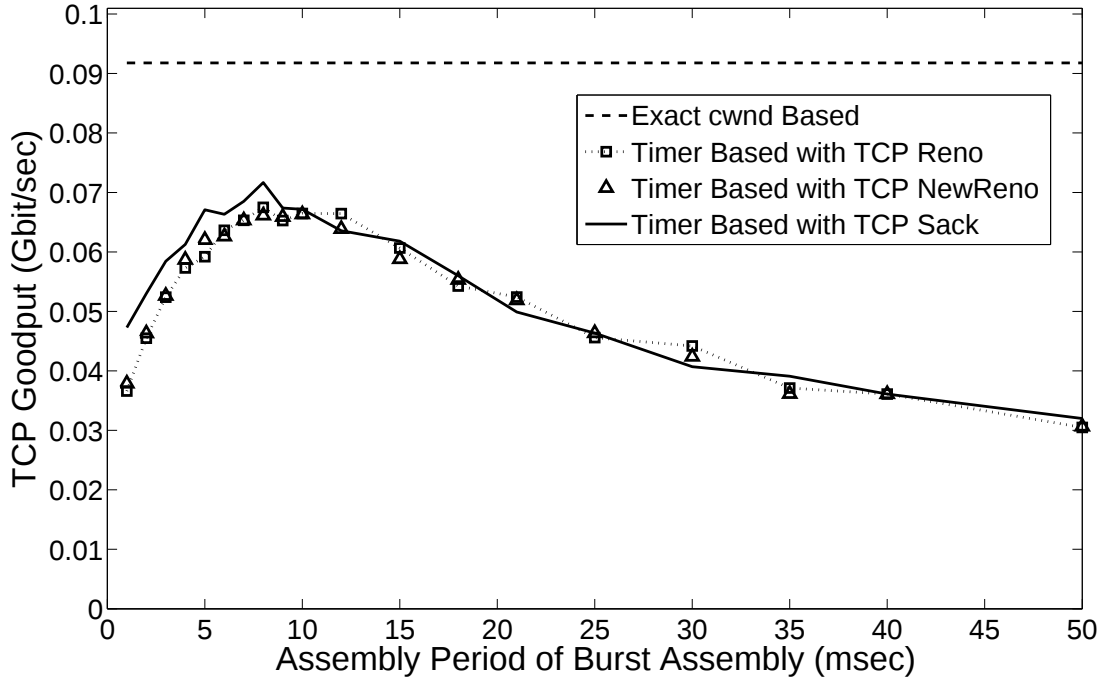
Figure 4.3: Performances of timer based and CWBA algorithms for the simple OBS network topology
