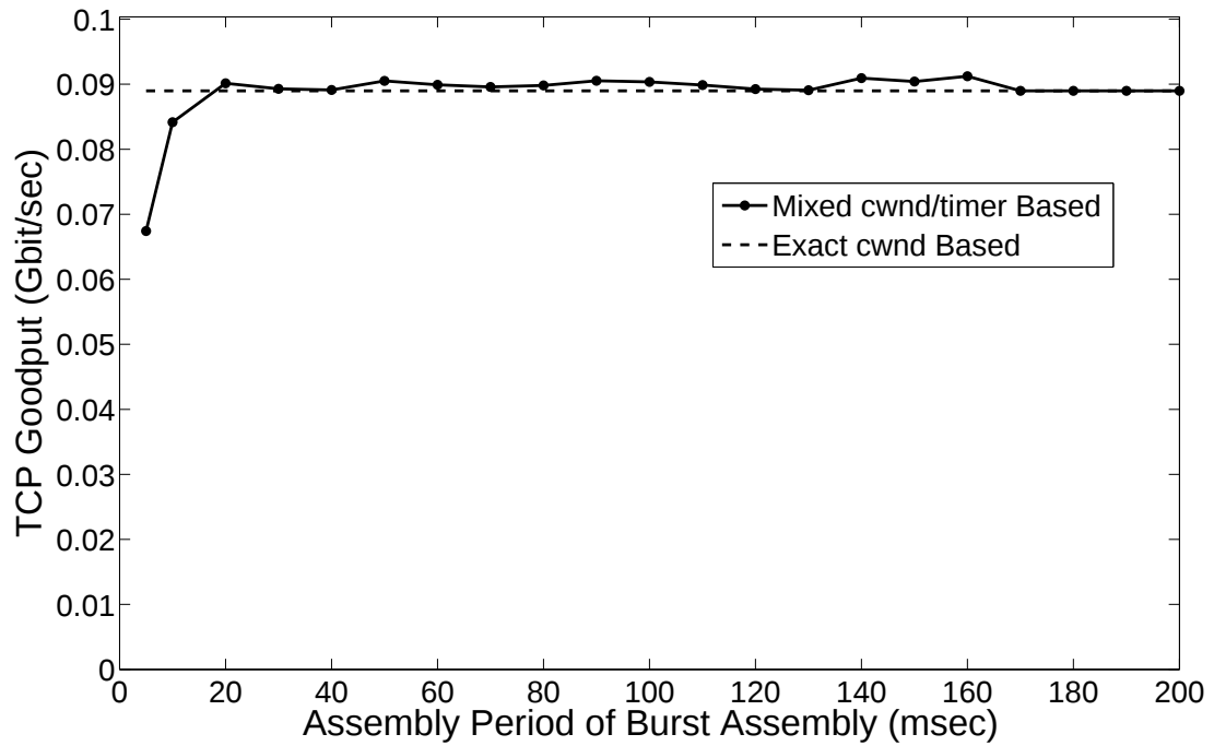
Figure 4.9: TCP performance of CWBA and MCWBA algorithms (average of 5 simulations) in the simple OBS network topology
