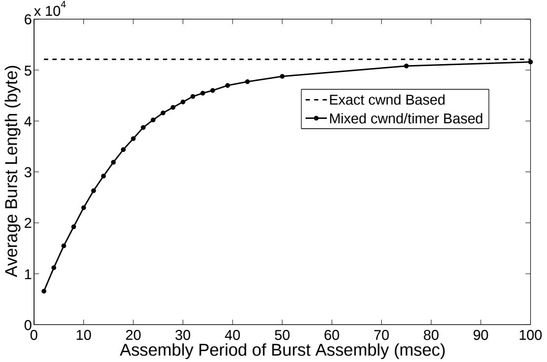
Figure 4.15: Average burst lengths for CWBA and MCWBA algorithms in the mesh OBS network topology
