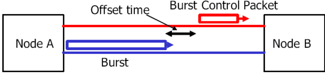
Figure 2.1: Optical burst and control packet
