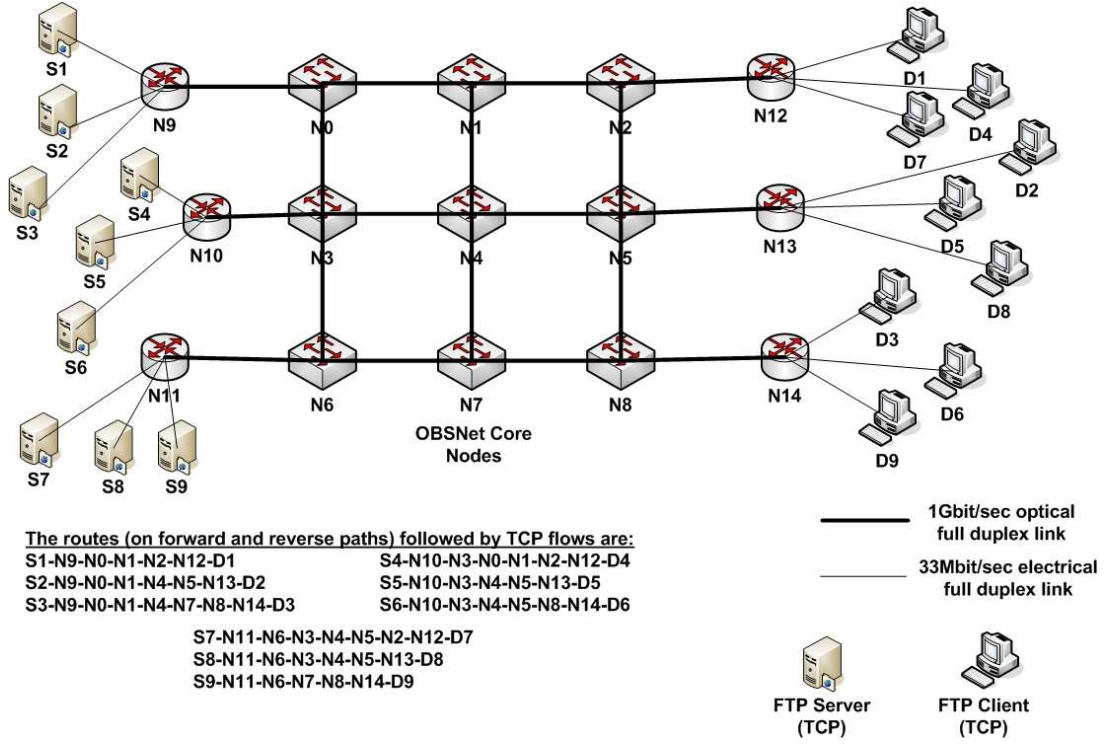
Figure 4.2: Mesh OBS network topology
