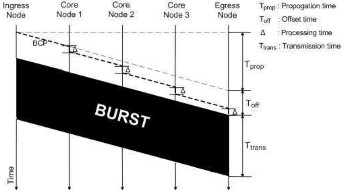
Figure 2.2: Timing diagram of a BCP and the corresponding burst
