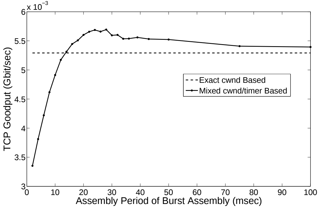
Figure 4.13: TCP performance of CWBA and MCWBA algorithms for the 4 th TCP flow for the mesh OBS network topology
