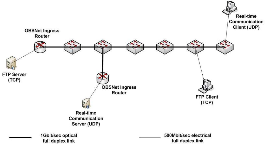
Figure 4.1: Simple OBS network topology
