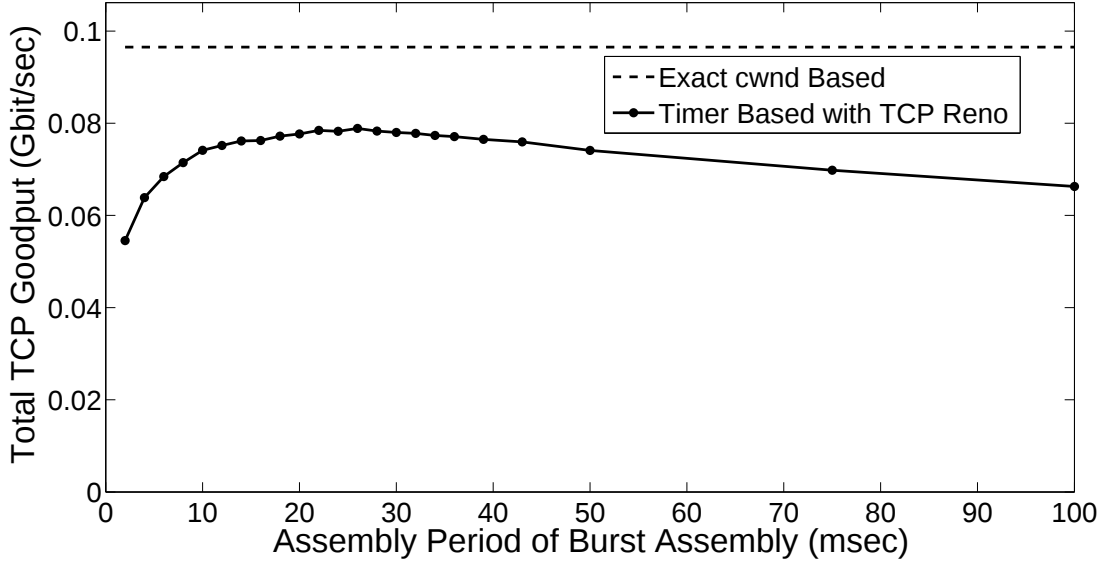
Figure 4.6: TCP performance of timer based and CWBA algorithms in the mesh OBS network topology
