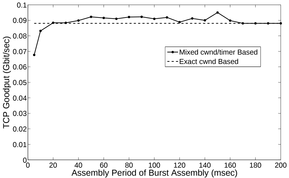
Figure 4.10: TCP performance of CWBA and MCWBA algorithms (optimistic case) in the simple OBS network topology
