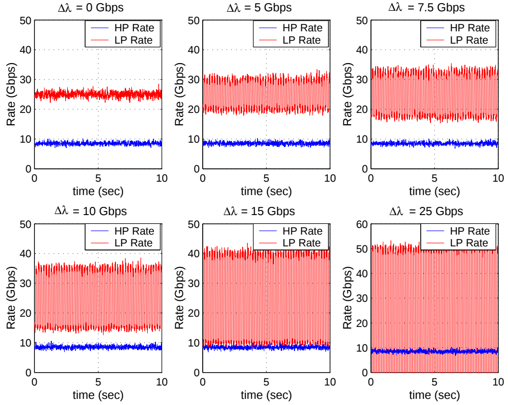
Figure 4.24: HP and LP transmission rates for OBS without flow control.
