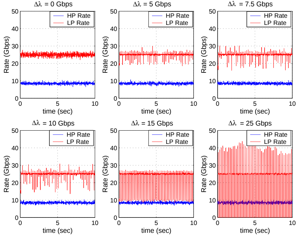
Figure 4.23: HP and LP transmission rates for flow controlled OBS.
