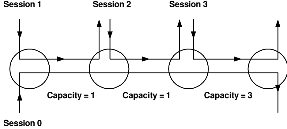
Figure 3.4: Illustration of Max-Min Fairness.
