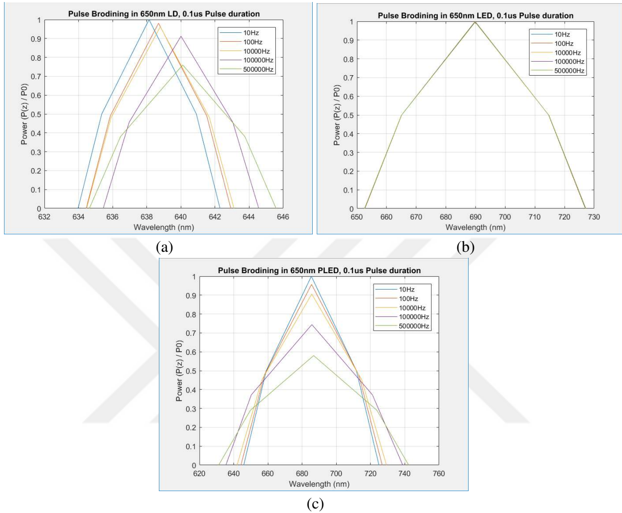
Figure 4.13: The pulse broadening and distortion for different frequencies at 0.1\mu s pulse duration for: (a) 650nm LD, (b) 650nm LED, (c) 650nm PLED
