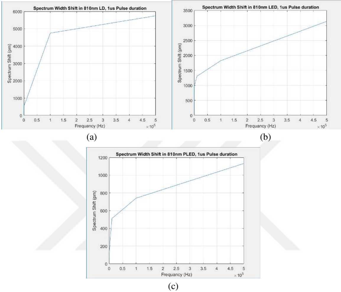
Figure 4.28: The spectrum shift changes at 1\mu\text{s} pulse duration for: (a) 810nm LD, (b) 810nm LED, (c) 810nm PLED
