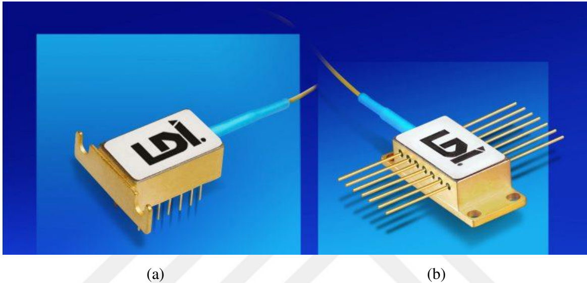
Figure 2.6: Two types of telecommunication LD: (a) DIL (b) butterfly
