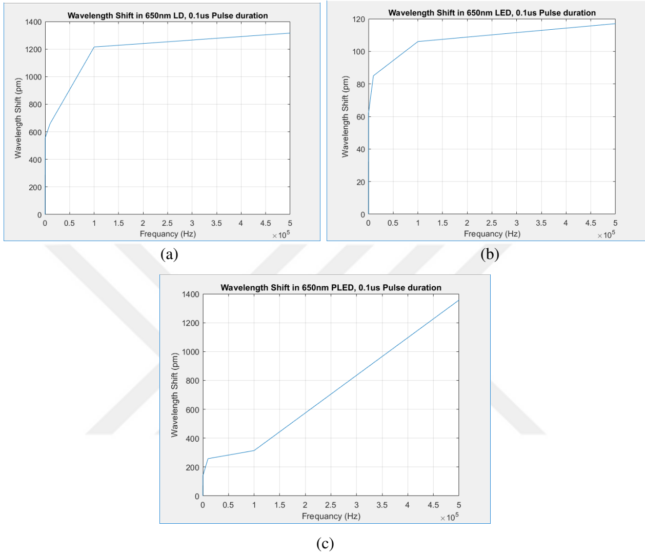
Figure 4.2: The wavelength shift at 0.1\mu\text{s} pulse duration for 650nm: (a) LD, (b) LED, (c) PLED
