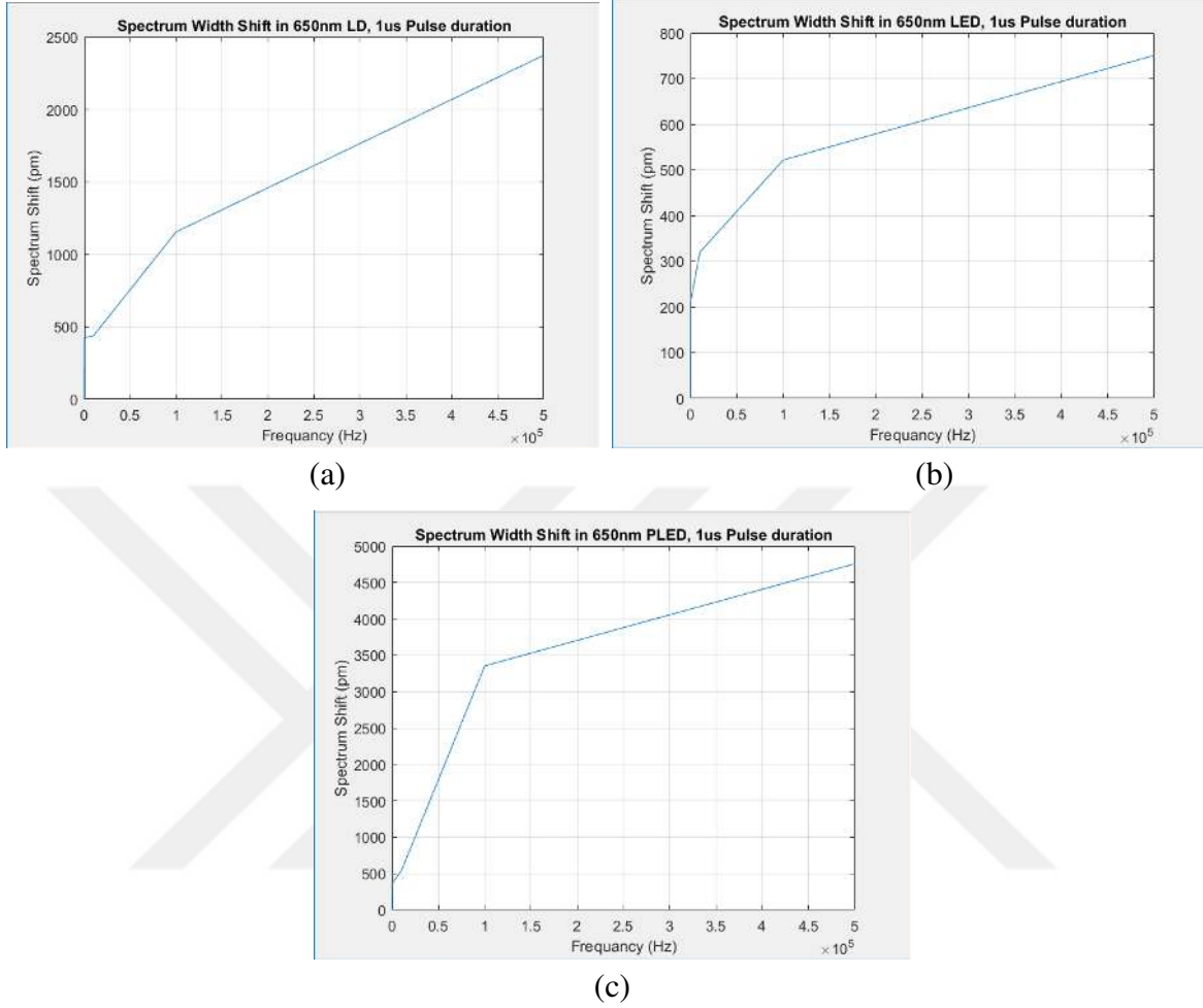
Figure 4.24: The spectrum shift changes at 1\mu\text{s} pulse duration for: (a) 650nm LD, (b) 650nm LED, (c) 650nm PLED
