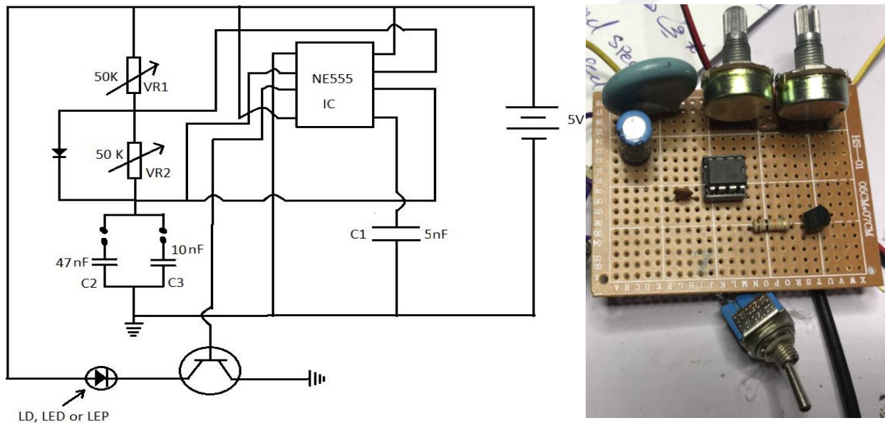
Figure 3.2. oscillation circuit diagram
