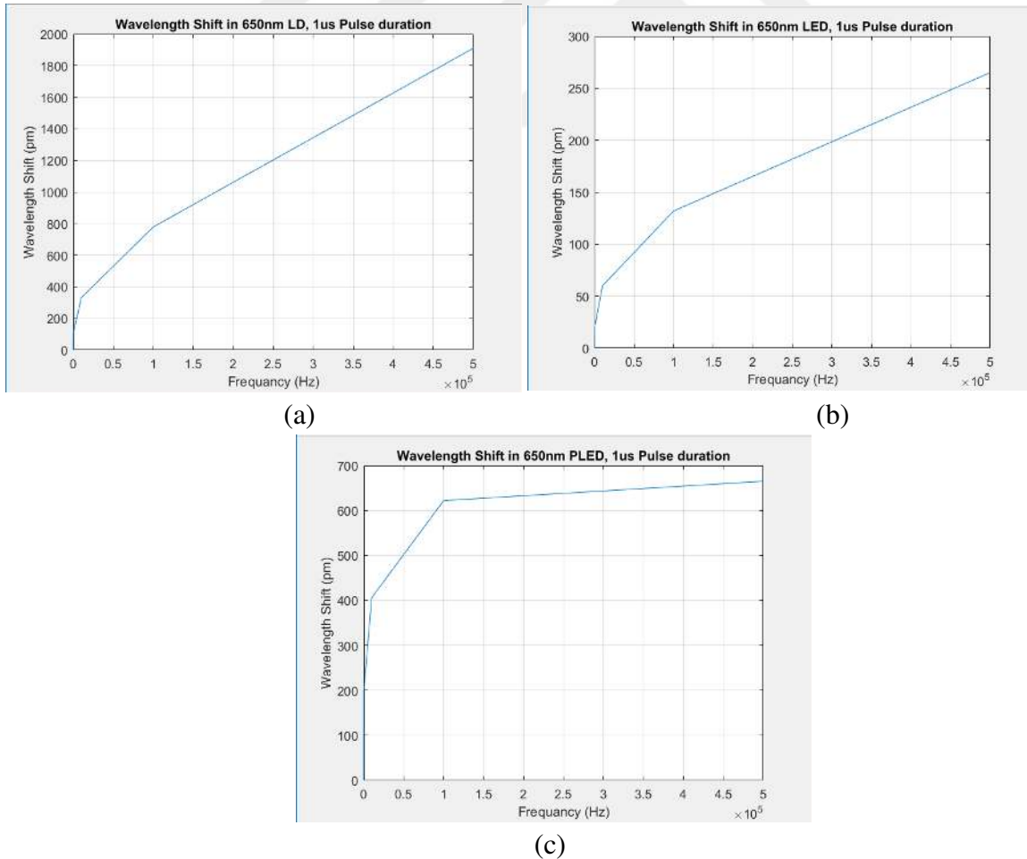
Figure 4.8: The wavelength shift at 1 \mu s pulse duration for 650nm: (a) LD, (b) LED, (c) PLED
