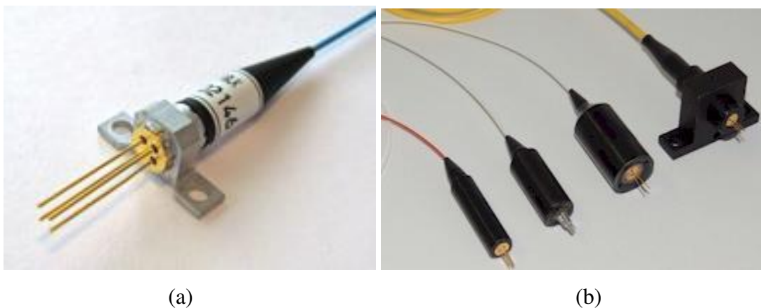
Figure 2.7: (a) coaxial LD (b) fiber pigtailed LD
