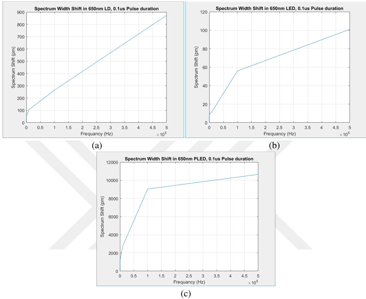
Figure 4.12: The spectrum width shift changes at 0.1 \mu s pulse duration for: (a) 650nm LD, (b) 650nm LED, (c) 650nm PLED
