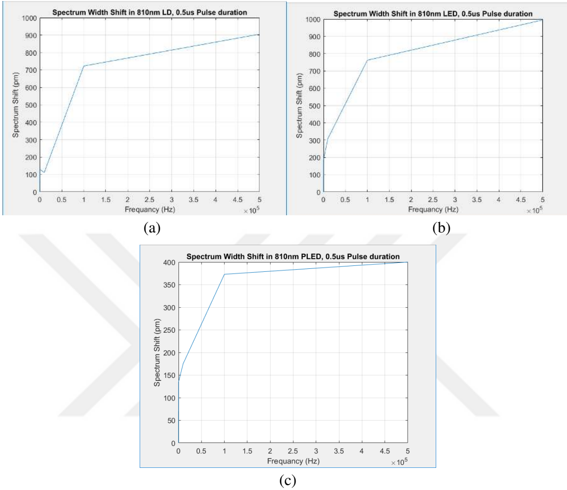
Figure 4.22: The spectrum shift changes at 0.5μs pulse duration for: (a) 810nm LD, (b) 810nm LED, (c) 810nm PLED
