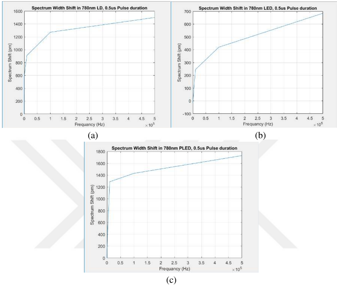
Figure 4.20: The spectrum shift changes at 0.5\mu\text{s} pulse duration for: (a) 780nm LD, (b) 780nm LED, (c) 780nm PLED
