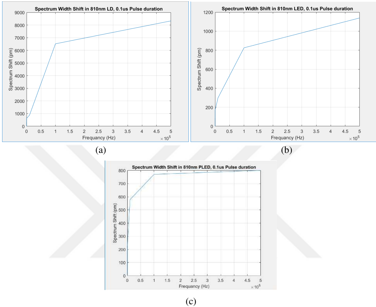
Figure 4.16: The spectrum shift changes at 0.1\mu\text{s} pulse duration for: (a) 810nm LD, (b) 810nm LED, (c) 810nm PLED
