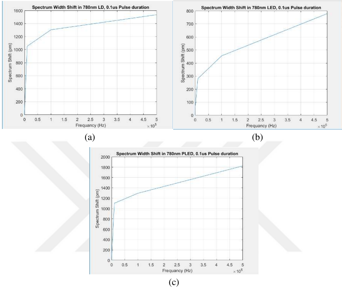
Figure 4.14: The spectrum width shift changes at 0.1 \mu s pulse duration for: (a) 780nm LD, (b) 780nm LED, (c) 780nm PLED
