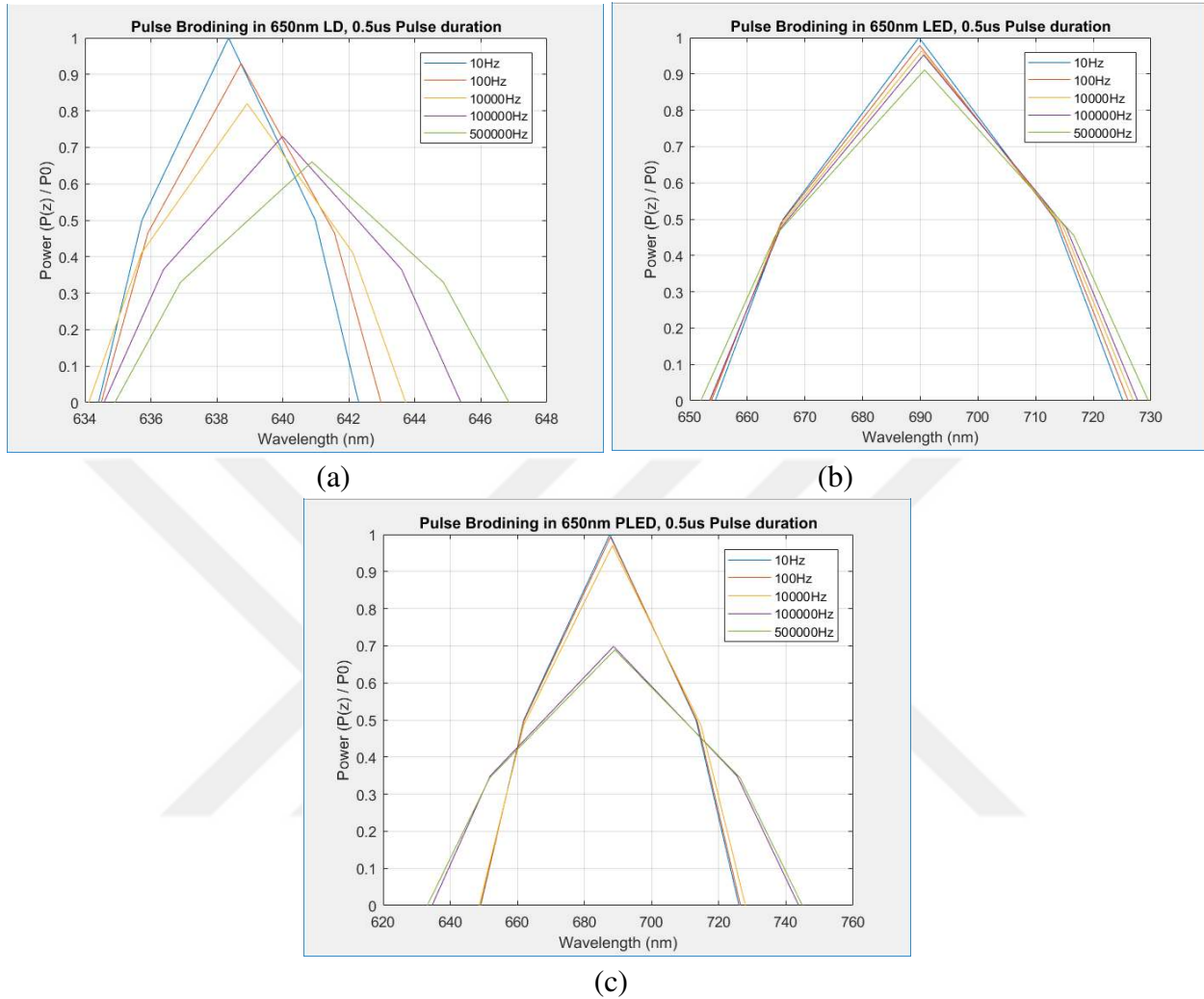
Figure 4.19: The pulse broadening and distortion for different frequencies at 0.5μs pulse duration for: (a) 650nm LD, (b) 650nm LED, (c) 650nm PLED
