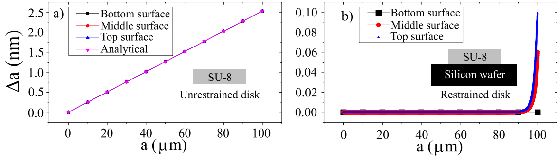
Figure 3.5: Humidity expansion simulations of a) unrestrained SU-8 microdisk and b) SU-8 microdisk fixed on a rigid substrate. Unrestrained case matches well with the analytical formula whereas the fixed case has expansion only around the edges of the microdisk. The bottom surface of the microdisk is not expanded, since it is fixed on the rigid substrate. However, the middle and the top parts of the microdisk expand by a smaller amount than the unrestrained case. Expansion at the middle part is taken to be the effective expansion "felt" by the WGM. Indicators of bottom, middle and top surfaces are chosen to be in different sizes for better visualization because they overlap over the region, where 0 \mu\text{m} < a < 90 \mu\text{m}
