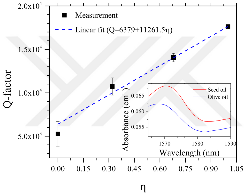
Figure 6.5: Measured Q-factor as a function of volume fraction of olive oil, \eta , inside the mixture droplet. The expected linear trend is observed and a linear fit is provided. Based on the fit, pure sunflower seed oil has a Q-factor of \sim 6400 whereas, for pure olive oil, it is \sim 17500 . In the inset, absorption measurement from pure sunflower seed oil and pure olive oil are provided. Sunflower seed oil absorption is more, therefore the Q-factor for sunflower seed oil is less as compared to the olive oil.
