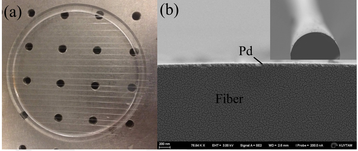
Figure 7.1: a) OFRs prepared for sputtering in a grill configuration for two-sided coating of Pd. b) SEM image of the OFR after Pd coating. OFRs are cut in the perpendicular direction to the fiber axis and SEM image is taken from the cut cross section, as depicted in the inset.
