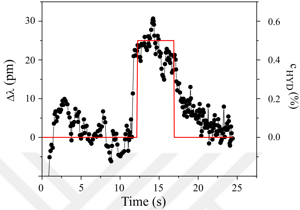
Figure 4.6: H_2 sensing results under humid N_2 . Although the fluctuations are higher than dry N_2 environment, still c_{HYD} = 0.5\% is detected under humid environment.
