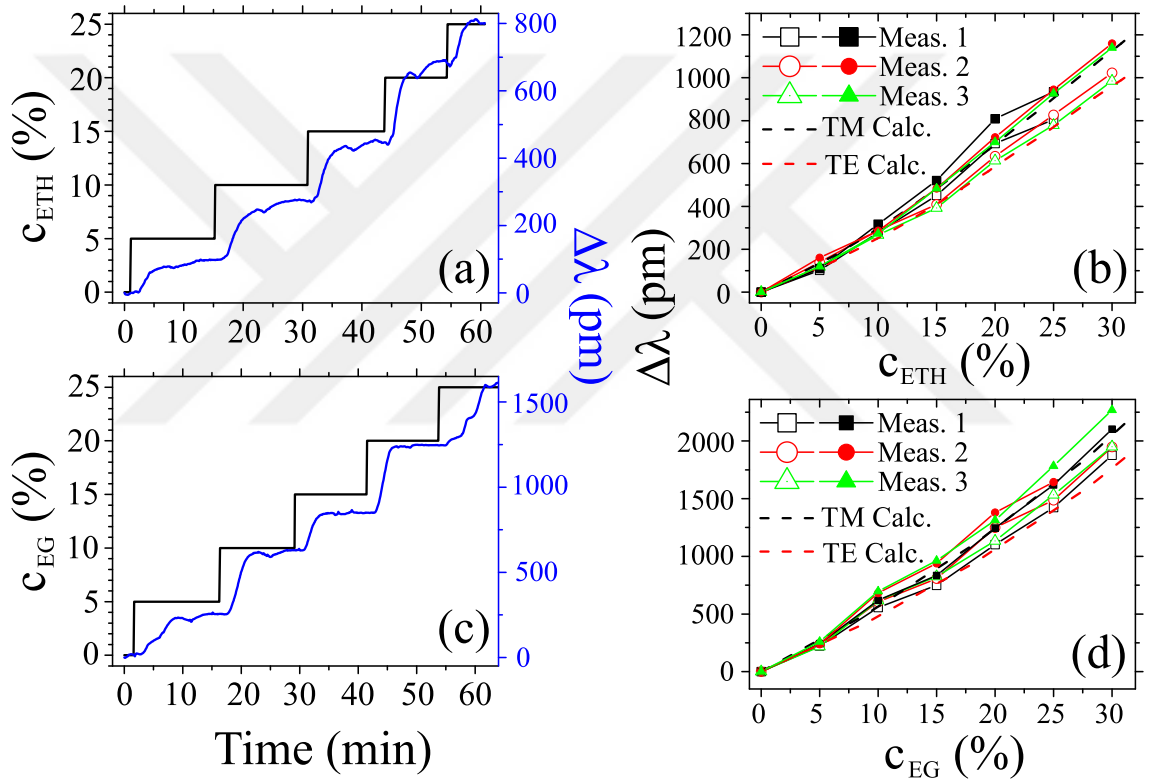
Figure 5.9: Time traces of a) Ethanol and c) EG sensing experiments. Respective results are depicted in b) and d), together with the analytical calculations.
