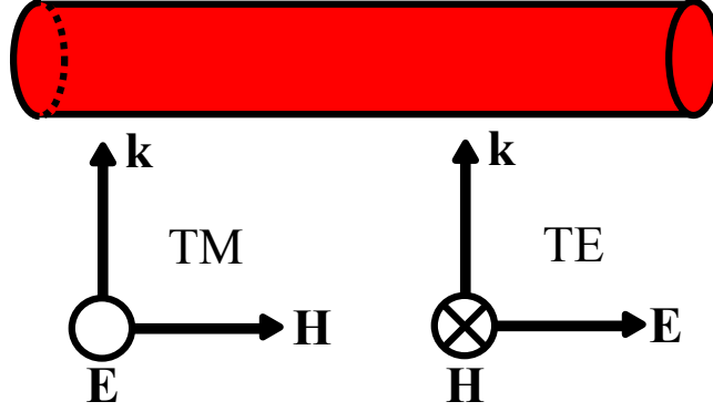
Figure 2.1: A sketch indicating the TM and TE polarizations in cylindrical coordinates. The definition of the polarization is based on the orientation of the electric field \mathbf{E} with respect to the WGM plane. If \mathbf{E} is in the same plane as the WGM, polarization is TM, whereas if they are perpendicular, then the polarization is TE.
