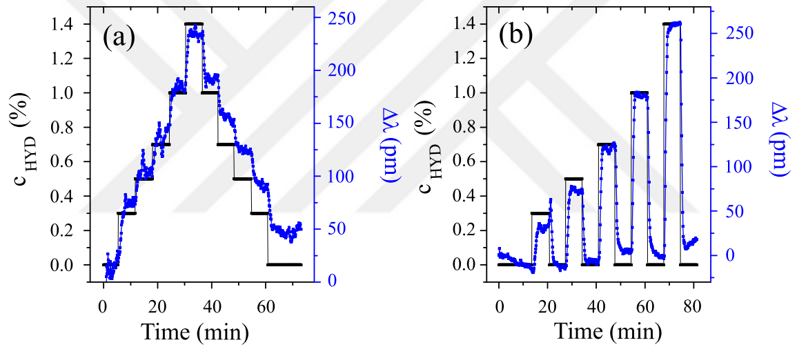
Figure 7.11: a) Staircase manner and b) On-off manner hydrogen detection results using Pd and polymer-coated OFR.
