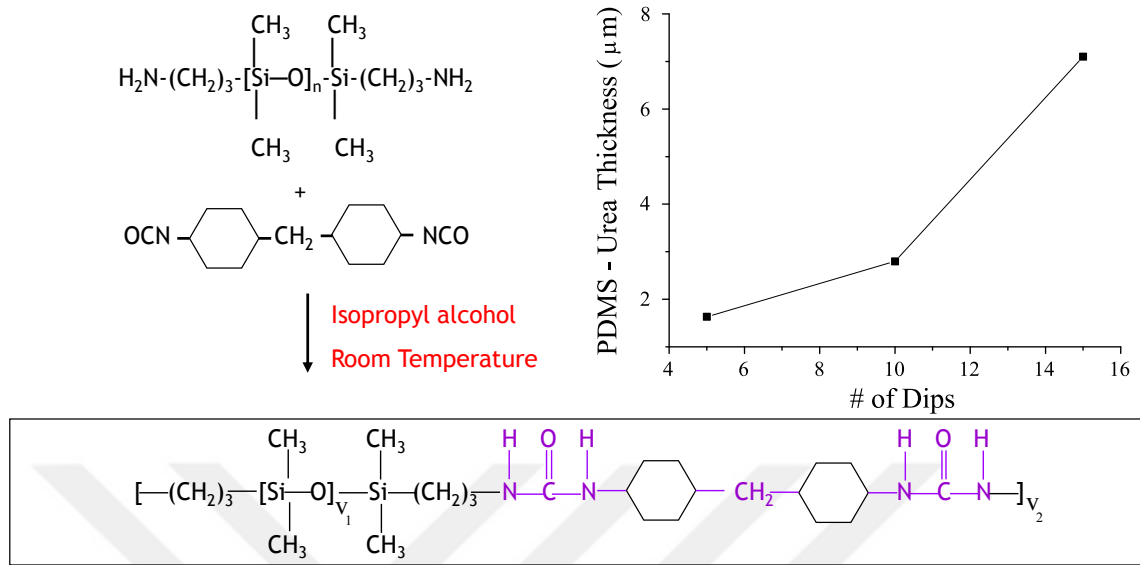
Figure 7.3: Schematic representation of PDMS-urea preparation. As the inset shows, PDMS-urea thickness increases with increasing number of dips.
