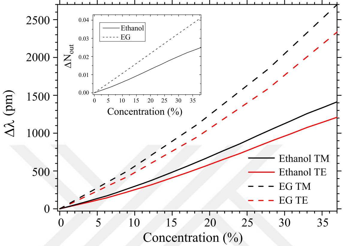
Figure 5.6: Spectral shifts expected from the analytical calculation with respect to ethanol/EG concentration for both TM and TE polarizations. Since EG has higher relative refractive index, slope belonging to EG is higher than the slope of ethanol. Also, TM slope is slightly higher than TE slope. The inset shows the change in the ambient refractive index ( \Delta N_{out} ) with respect to the ethanol/EG concentration. These values are used in calculation of the main figure.
