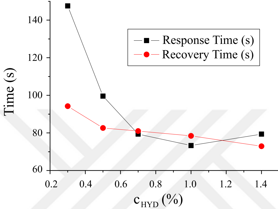
Figure 7.7: Response and recovery times of the sensor. The response of the sensor becomes quicker as c_{HYD} increases up to 1%. Then remains constant around 80 s. Recovery time is constant around 80 s over a larger c_{HYD} region.
