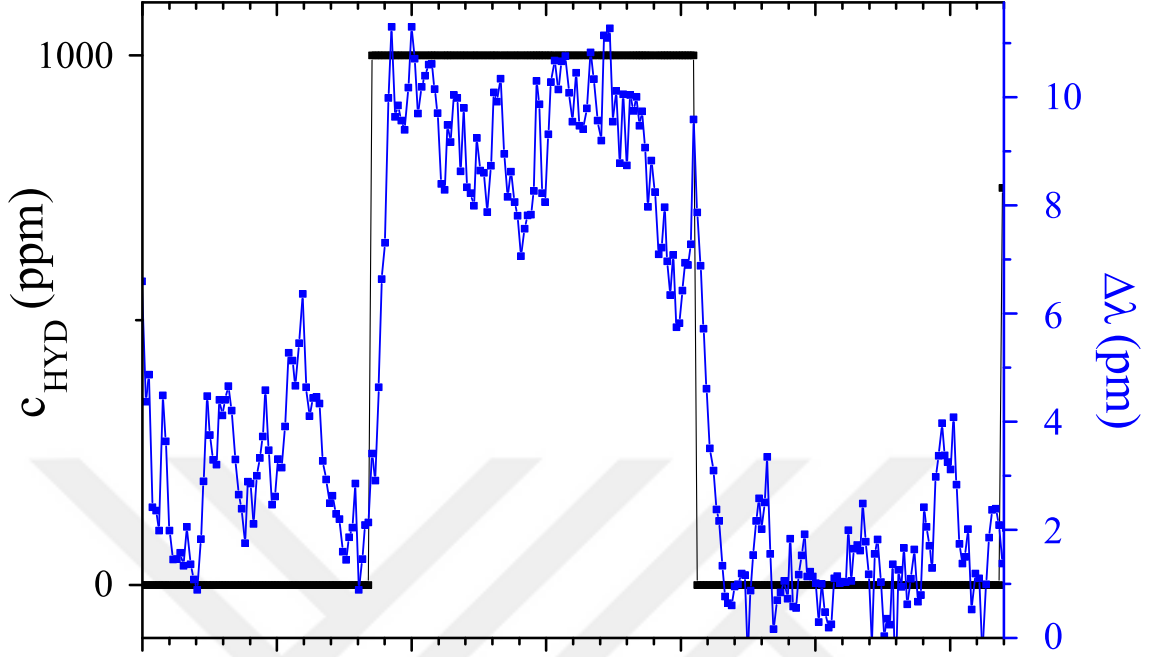
Figure 7.9: An exemplary measurement when c_{HYD} = 1000 \text{ ppm} = 0.1\%
