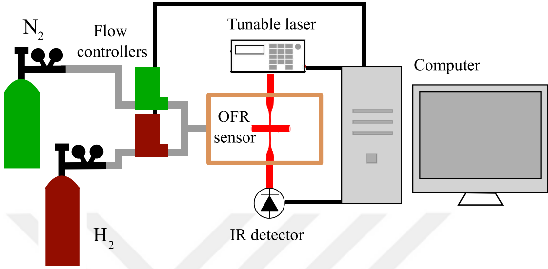
Figure 7.5: Experimental setup for hydrogen gas detection using Pd and polymer-coated OFR. The sensor is exposed to dilute hydrogen gas concentrations. In the meanwhile, tunable laser light is coupled to the OFR through the tapered fiber. Collected transmission spectra are analyzed using a computer. Hydrogen concentrations are adjusted using computer-controlled flow controllers. In the figure, green gas cylinder and the flow controller are associated with the nitrogen gas, whereas the brown ones are with the hydrogen gas.
