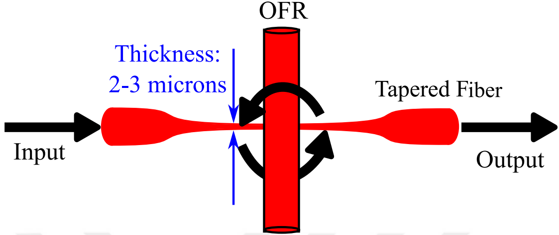
Figure 5.1: A sketch depicting the perpendicular geometry for exciting the WGMs using tapered fiber, as well as the azimuthally propagating WGMs inside the OFR. Black arrows represent the propagation direction of the excitation light.
