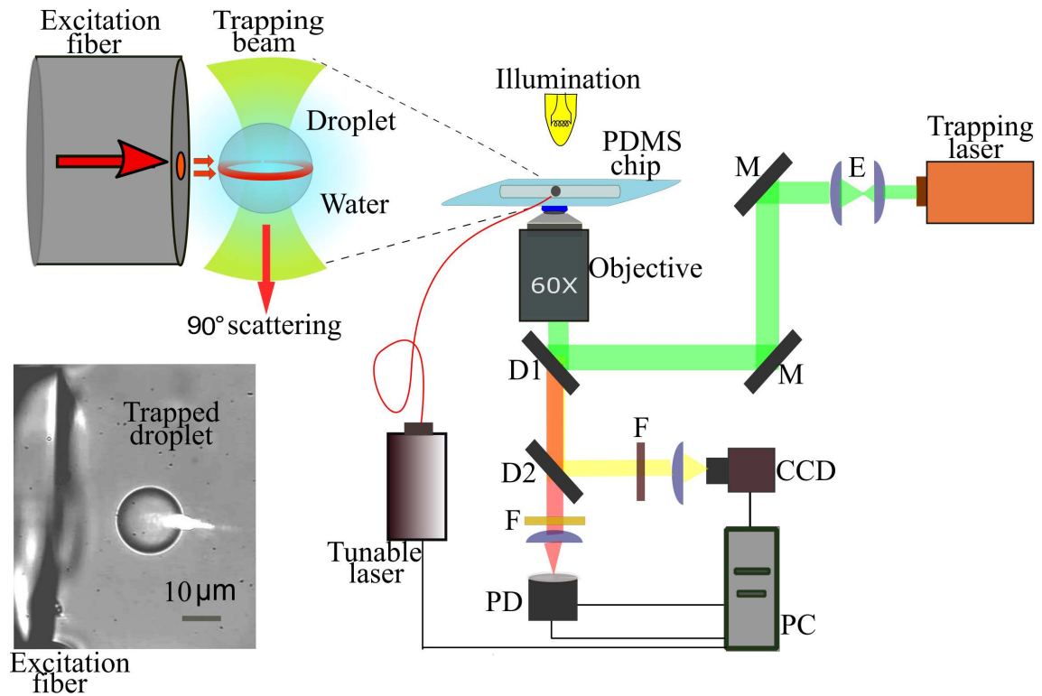
Figure 6.1: Experimental setup used for droplet experiments. PDMS chip involving the microchannel and excitation fiber is held on an inverted microscope. Using one dichroic mirror (D1), trapping laser is reflected and directed onto the droplet whereas the scattered light in the telecom wavelength and the optical image in the visible range are transmitted through. These two are separated using another dichroic mirror (D2). In the inset at the top, a schematic description of the trapped droplet and the excitation fiber is presented. The lower inset is an optical image of the trapped droplet and the scattered light. Red laser through the excitation fiber is used just for imaging purposes. During experiments, tunable telecom light is used through the excitation fiber.
