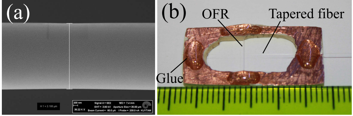
Figure 5.3: a) SEM image of the tapered fiber. The scale shows a thickness of < 3.2 \mu\text{m} . b) Photograph of a tapered fiber and OFR pair perpendicularly placed and fixed using epoxy glue. Metric ruler is also provided for scaling.
