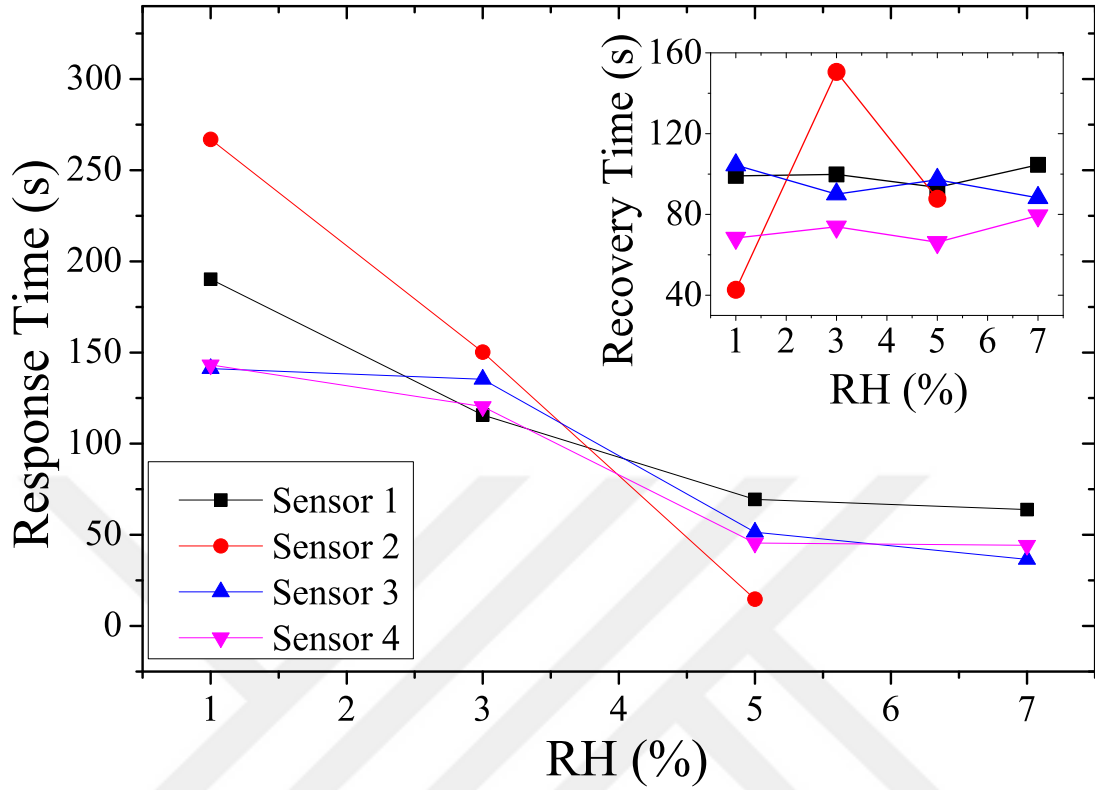
Figure 3.8: Response times of the sensors depicted in Figure 3.7. Response of the sensors become faster as the RH is increased from 1% to 5%, and stays constant afterwards. The inset shows the recovery times of the sensors. Recovery of the sensors stay more or less constant throughout the range of 1% to 7% RH.
