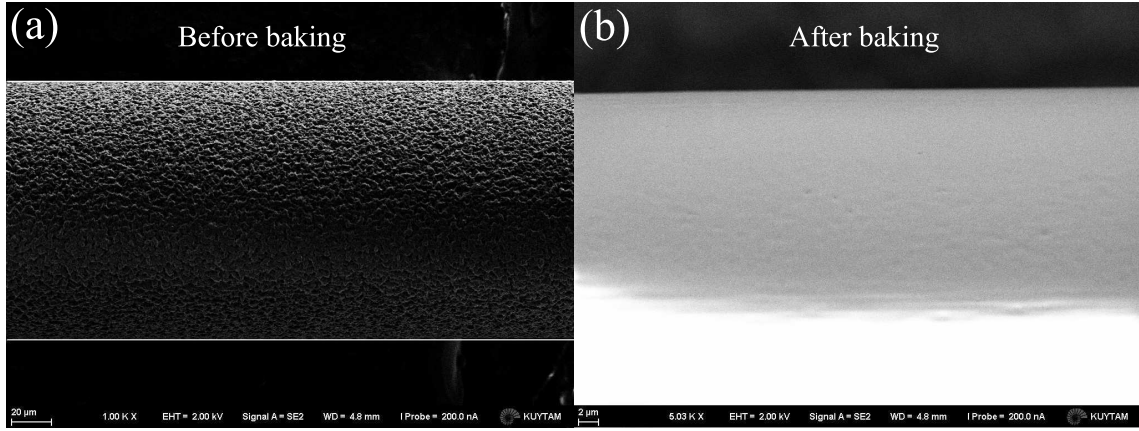
Figure 7.4: SEM images of dip coated OFR a) before and b) after baking. Improvement towards achieving smooth surfaces with baking is clearly visible.
