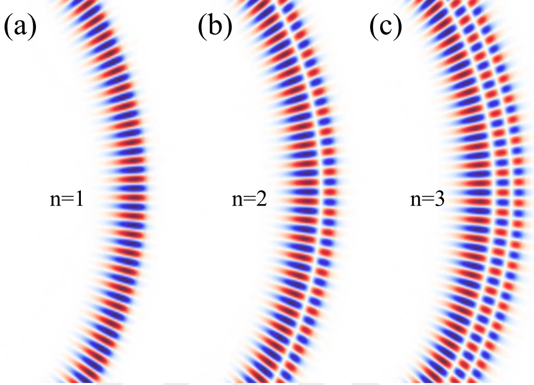
Figure 2.3: MEEP simulation results for a 2D disk. Parameters are kept constant and \lambda is adjusted such that a) first, b) second, and c) third-order radial modes are excited for a = 20 \mu m and N = 1.5 [Eryürek, 2013].
