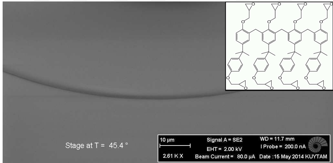
Figure 3.2: SEM image of an edge of an SU-8 microdisk resonator. The measurement reveals an SU-8 thickness of 1.86 \mu m . The monomer of the SU-8 is depicted in the inset.
