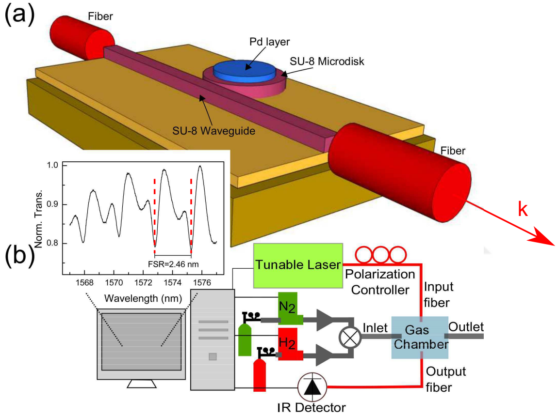
Figure 4.2: a) Schematic visualization of end-face coupling. b) Experimental setup for H_2 sensing experiments. H_2 and N_2 gases are mixed to obtain desired concentrations of H_2 using computer-controlled gas flow controllers, similar to the humidity sensing setup. The inset shows an exemplary transmission spectrum of the SU-8.
