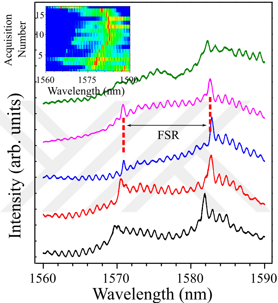
Figure 6.3: Consecutive WGM scattering spectra for a BB emulsion droplet inside water. Between each spectrum, there is a time delay of \sim 10 s. FSR is \sim 12 nm, in agreement with the calculation. Ripples with smaller intensity are due to Fabry-Pérot-like interference because of optical components in the experimental setup. The inset shows a color plot of the WGM around 1580 nm in a wider time window, where red (blue) means higher (lower) intensity. Clear back and forth fluctuation of the spectral position of the WGM is an indication of diffusion of small particles in and out of the BB droplet.
