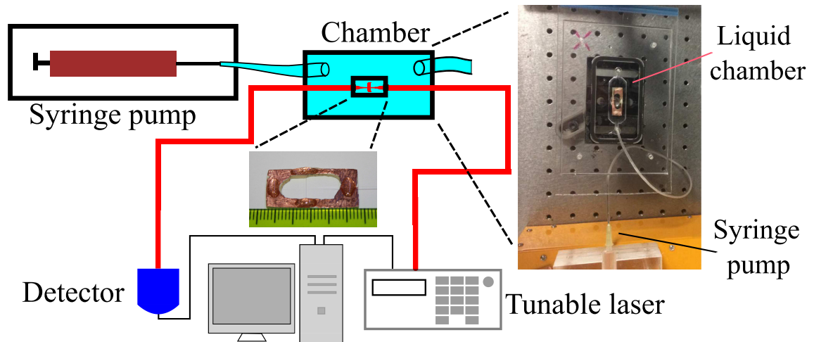
Figure 5.5: Experimental setup for liquid refractometric measurements using OFRs. Water solutions of ethanol or EG are introduced using a syringe pump into the liquid chamber where OFR and tapered fiber are held in perpendicular geometry (see the inset). Tunable laser light coming from the optical fiber is coupled to the OFR in the tapered region.
