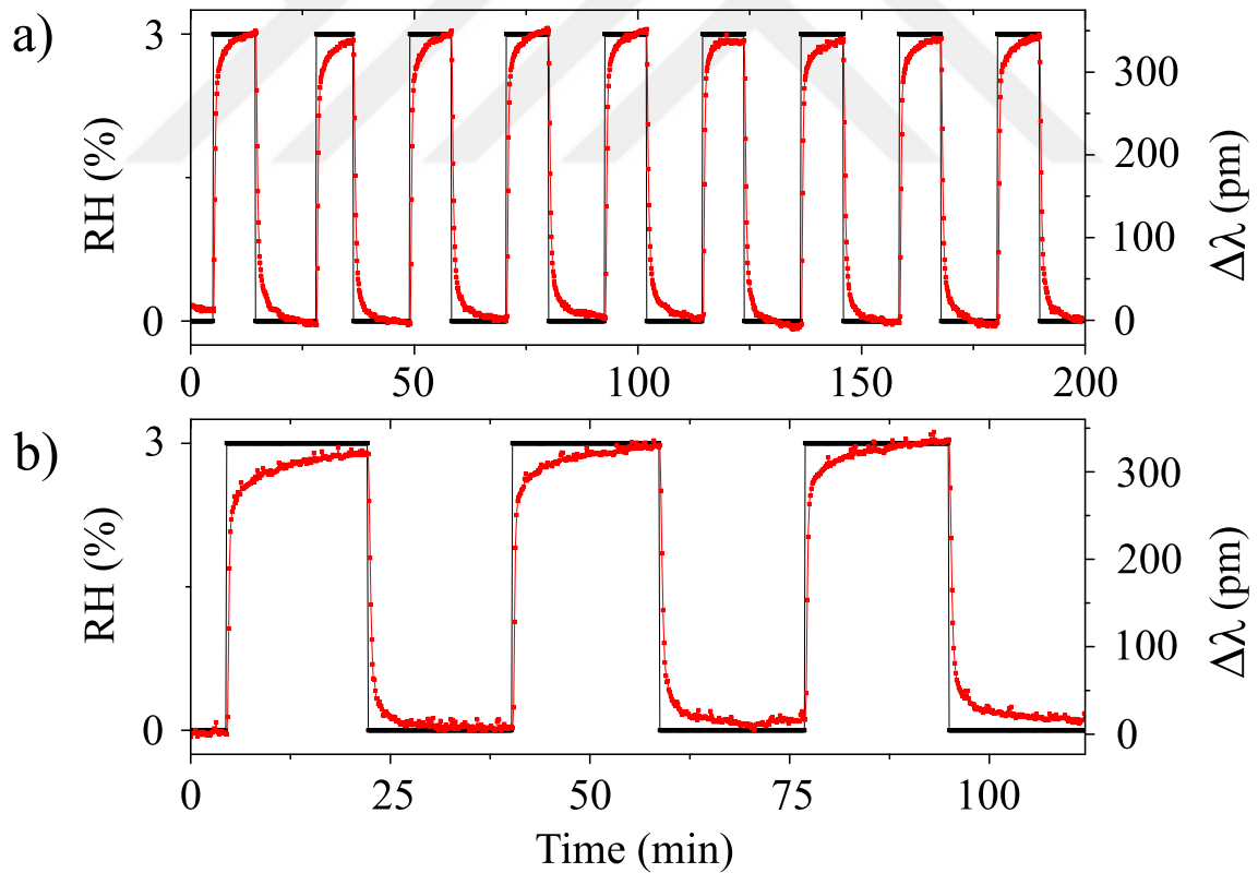
Figure 3.10: a) Multiple on-off cycles performed on a sensor. b) More on-off cycles 45 days after the experiment depicted in a). \Delta\lambda is between 334 and 340 pm for a) and in b) it is between 317 and 322 pm.
