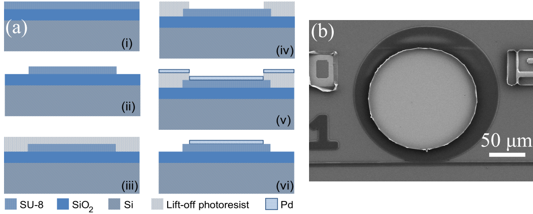
Figure 4.1: a) Fabrication flow of Pd-coated SU-8 microdisk resonators. i) Spin coating of SU-8 on a thick-oxide Si wafer. ii) Fabrication of SU-8 microdisks and waveguides. iii) Spin coating of sacrificial lift-off photoresist. iv) Patterning of the sacrificial photoresist. v) Sputtering Pd. vi) Removal of the sacrificial photoresist. b) SEM image of the fabricated sensor. Pd microdisk can be seen on top of the SU-8 microdisk.
