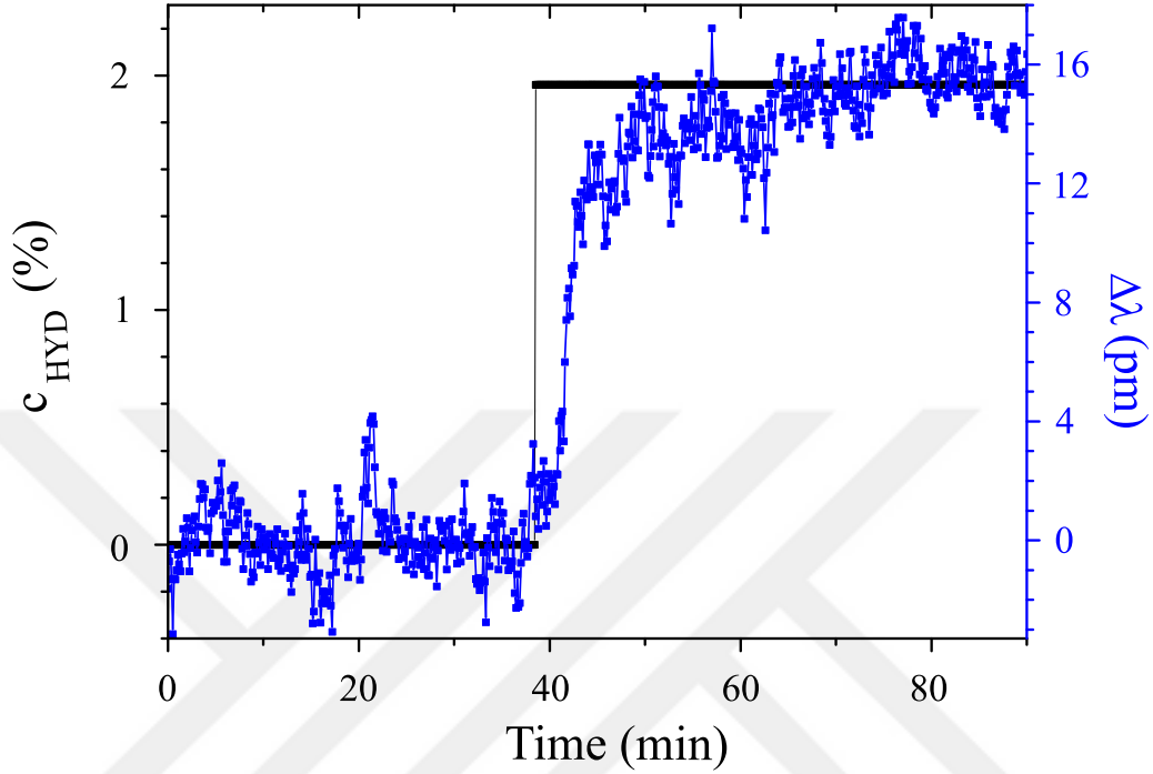
Figure 7.10: Response of only PDMS-urea coated OFR to hydrogen gas. \Delta N effect is present, which is significantly less than \Delta a effect obtained with the PDMS-urea and Pd-coated OFR.
