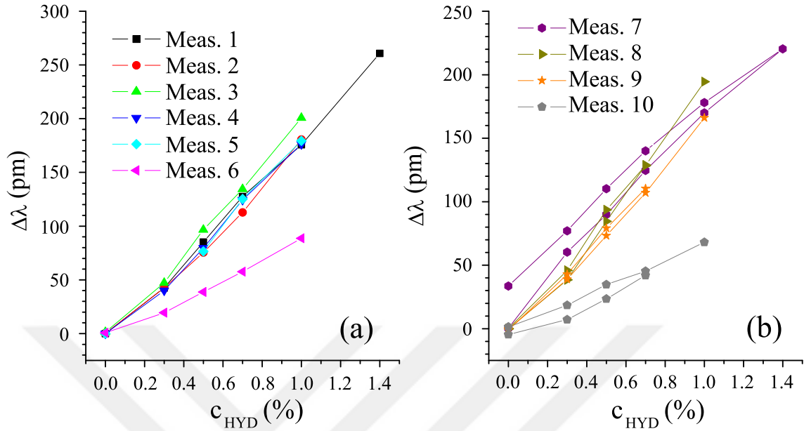
Figure 7.8: Summary of the hydrogen sensing measurements for a) On-off manner measurements and b) Staircase manner measurements.
