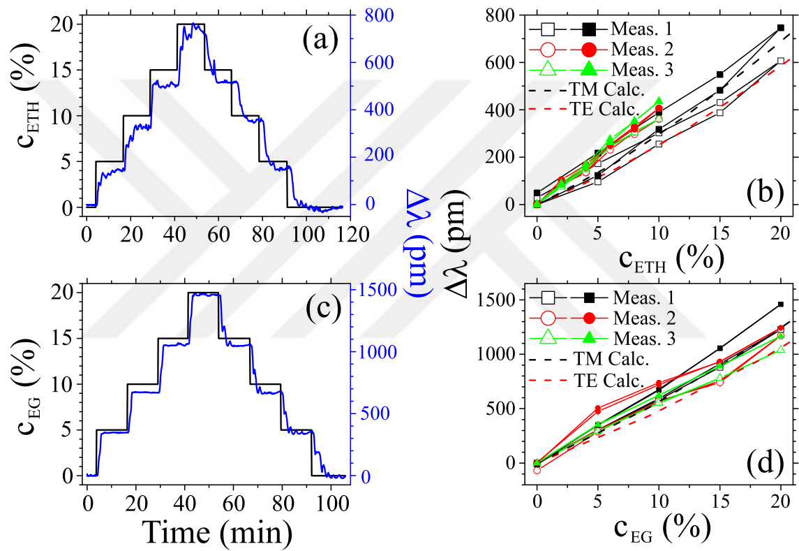
Figure 5.10: Time traces of a) Ethanol and c) EG hysteresis experiments. Respective results are depicted in b) and d), together with the analytical calculations.
