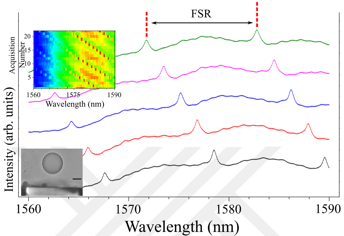
Figure 6.4: WGM spectra of a BB droplet in an unsaturated water host medium. The droplet dissolution results in a constant blue-shift in the WGM spectra, also slowly increasing the FSR. (FSR = 10.83 nm in the first spectrum, increases to 10.92 nm in the fifth spectrum). There is a \sim 10 s time delay between each consecutive spectra. In the color plot inset, the blue-shift is clearly visible. Again, red is higher intensity and blue is lower intensity. In a matter of < 25 scans, WGM positions shifts about three times the FSR. In the other inset, trapped BB droplet is depicted with a scale bar of 20 \mu\text{m} .
