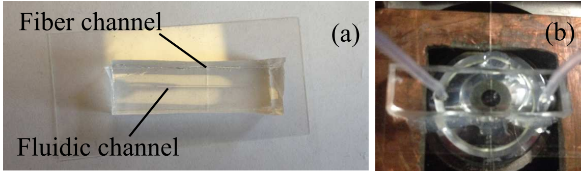
Figure 6.2: a) PDMS microfluidic chip featuring the fluidic and fiber channels used in the droplet experiments. b) Placement of the PDMS chip on the 60x microscope objective. This objective is used for three purposes: for focusing the trapping beam, collecting the scattering spectra from the droplet, and imaging the droplet.
