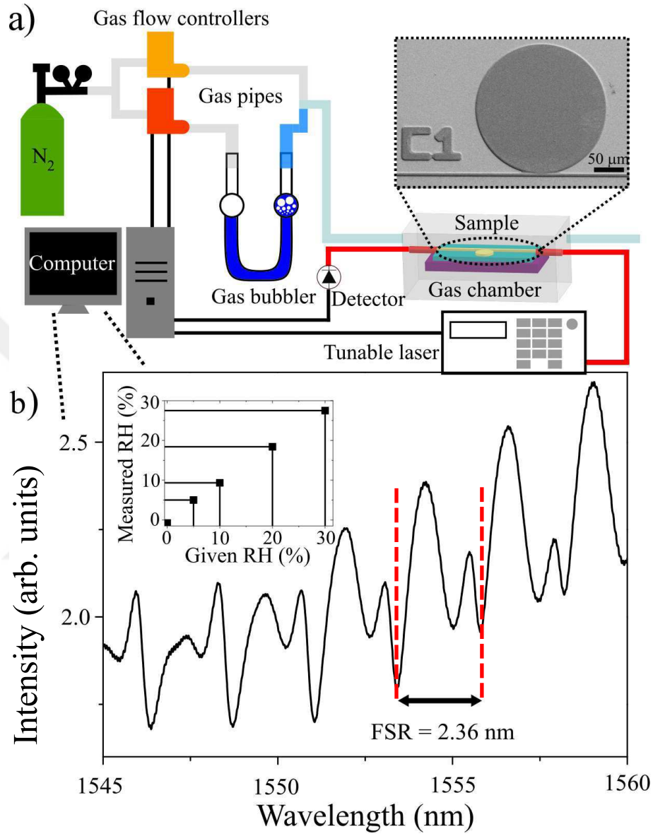
Figure 3.1: a) Experimental setup of humidity sensing measurements. N_2 gas is flown through two separate gas flow controllers. One is directly connected to the gas chamber whereas the other is connected to a bubbler filled with DI water. Using end-face coupling method, tunable laser light is coupled from optical fiber to SU-8 waveguide inside the gas chamber. In the inset, SEM image of the SU-8 humidity sensor is depicted. b) Transmission spectrum obtained from SU-8 microdisk resonator. FSR is measured to be 2.36 nm. The inset shows the comparison between the RH set by the flow controllers and RH measured from the commercial humidity sensor.
