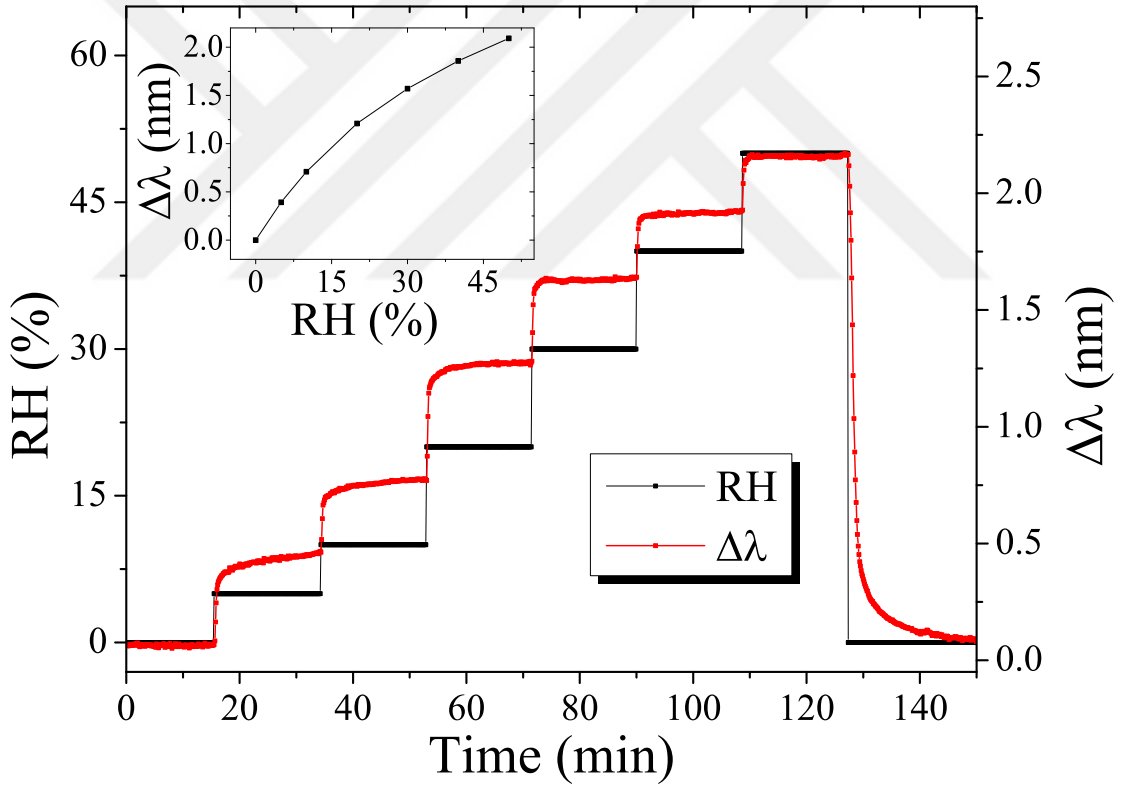
Figure 3.11: Time trace of the response of the sensor to high RH values up to 50%. Although nonlinearly, the spectral shift increases with the humidity. Also, the zero level is conserved. The inset shows the measured values from the time trace in the main figure.
