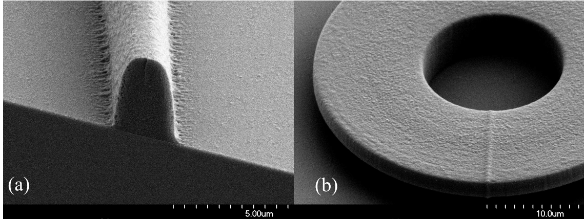
Figure 3.4: a) End-face cross section of a waveguide fabricated using UV laser writing. b) An SU-8 microring fabricated using TPP. A line along the radial direction is observed, because writing starts and ends at these points, resulting slightly higher exposure times along the line.
