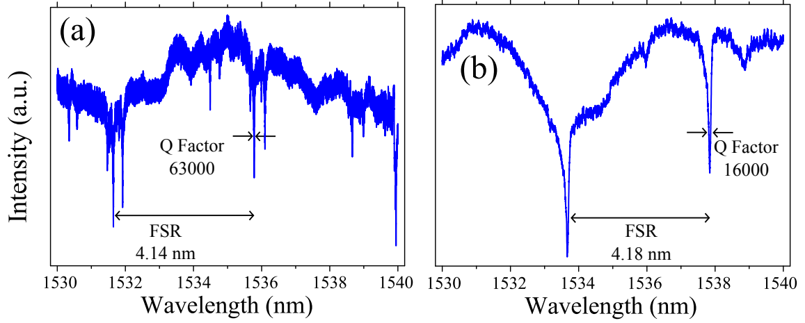
Figure 5.4: Transmission spectra of OFR excited in a) the air, and b) in pure water environment. Q-factor in the air is measured as 63000, but it decreases to 16000 in the water environment because of the absorption of water. FSR is not changed much from the air (4.14 nm) to the water (4.18 nm).
