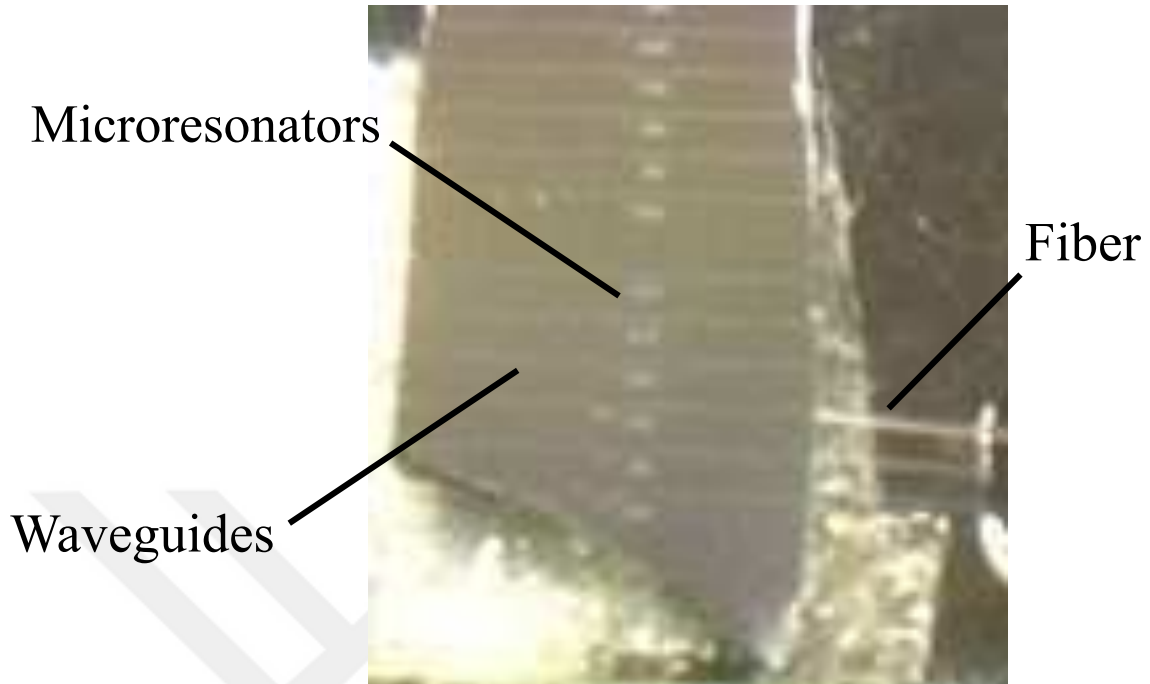
Figure 3.6: Photograph of a chip, on which microresonators and waveguides are seen, as well as the excitation fiber. The orientation of the fabrication of the waveguides is important, because the wafers must be cut perpendicularly to the waveguides to have smooth end faces for good coupling.
