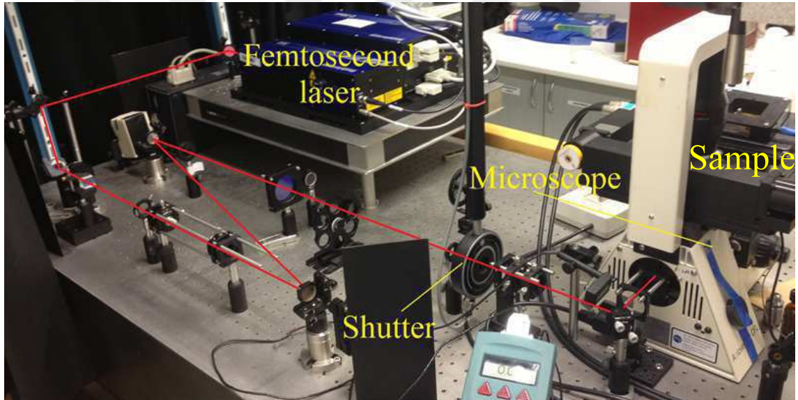
Figure 3.3: Photograph of the TPP setup. Femtosecond laser pulses, whose path is indicated as red are directed into an inverted microscope through a shutter. Then these pulses are focused by an oil-immersion objective. Using a piezo stage, the sample in 3 dimensions for the writing process. The sample is located on the objective during the writing.
