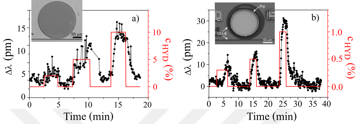
Figure 4.4: H_2 sensing results for a) uncoated SU-8 microdisk resonator and b) Pd-coated SU-8 microresonator. Red lines represent the H_2 concentration whereas black dots represent the \Delta\lambda . For uncoated devices, under c_{HYD} = 10\% , \sim 15 pm resonance shift occurs whereas under c_{HYD} = 1\% , \sim 30 pm is obtained when Pd-coated SU-8 microresonator is used. In the insets, SEM images of the corresponding sensors are depicted.
