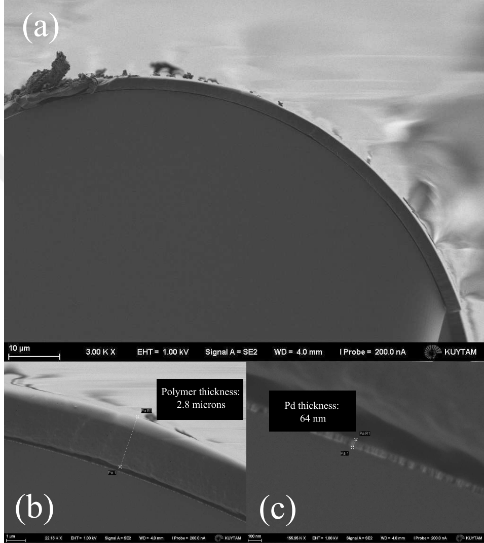
Figure 7.2: SEM images of the cross-section of the sensor. a) A wide view. b) A zoom to the wide view on the PDMS-urea coating. The coating thickness for this particular sample is measured as \sim 2.8 \mu\text{m} . c) Even a deeper zoom that focuses on the Pd coating. Pd thickness is measured as \sim 64 \text{ nm} .
