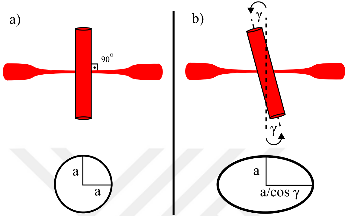
Figure 5.8: Schematic representation of a) perpendicular geometry and b) slightly deviated perpendicular geometry. The deviation is parametrized by the angle \gamma . WGM plane is circular when \gamma = 0 . As \gamma increases, WGM plane becomes an ellipse. The radius of the ellipse in the perpendicular direction, a , is constant, whereas in the other axis radius is equal to a/\cos \gamma .
