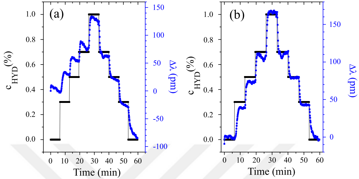
Figure 7.6: a) An exemplary hydrogen gas measurement featuring a constant drift to blue side of the spectrum. b) Measurement becomes better after a correction calculated from a linear fit to the \Delta\lambda values where c_{HYD} = 0 . Equation of the subtracted fit is -1.51526 \times (\text{Time in minutes}) + 8.98045
