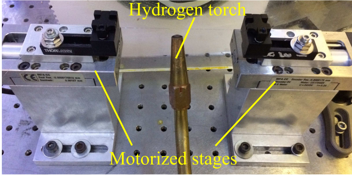
Figure 5.2: Photograph of the fiber tapering setup consisting of hydrogen flame torch, and motorized stages for pulling the fiber.
