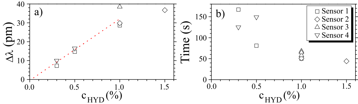
Figure 4.5: a) Sensitivity measured from multiple sensors. The dashed red line is the linear fit to the average of the sensor responses for H_2 concentrations between 0 and 1%. Slope is calculated to be 32 \text{ pm}/\%H_2 . b) Response times of these sensors. Response time decreases with the increasing concentration of H_2 .
