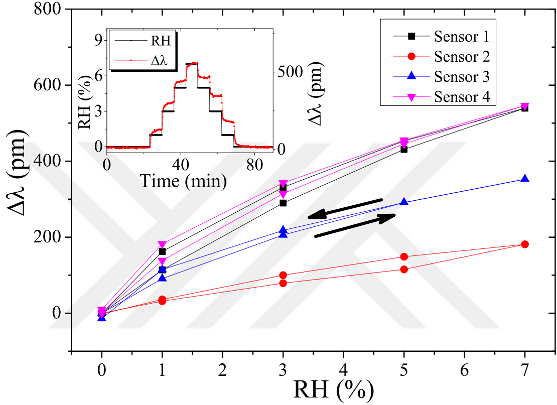
Figure 3.9: Sensing results from multiple sensors when humidity is changed in staircase manner. Sensors 1-4 are the same sensors depicted in Figure 3.7. For all the sensors, humidifying curves are below the dehumidifying curves. This is also indicated by the two black arrows pointing the humidifying and dehumidifying directions. Hysteresis ( Hys ) is calculated to be 17% from the average of 1%, 3% and 5% RH. The inset shows time trace of Sensor 1. Zero level is preserved.
