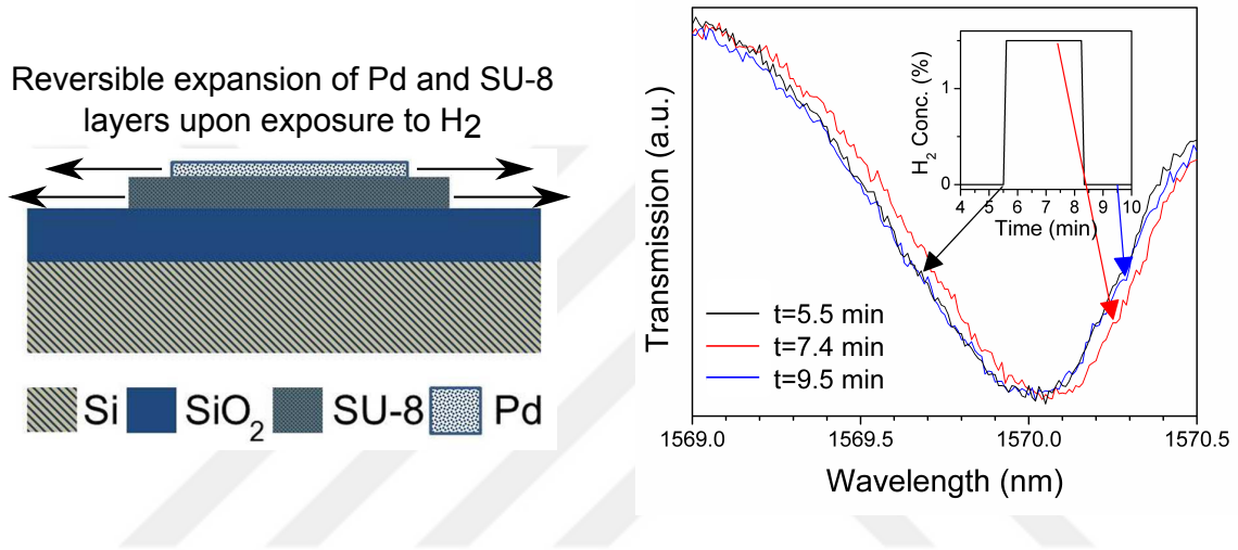
Figure 4.3: a) Schematic cross sectional view of the Pd-coated SU-8 microresonator. Expansion of the Pd induces an expansion for SU-8 microresonator. b) Change in the transmission spectrum while the c_{H_2D} is changed from 0% to 1% and then back to 0%. The inset shows the points where the transmission spectra belong to.
