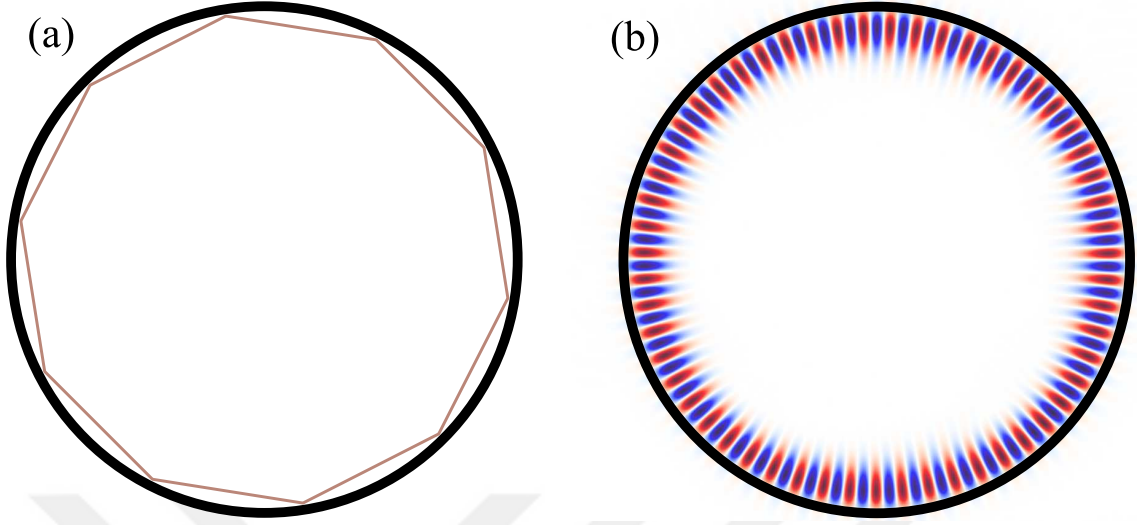
Figure 1.1: a) A sketch of an azimuthally symmetric resonator with light experiencing multiple TIRs in ray optics. b) MEEP (MIT Electromagnetic Equation Propagation) simulation indicating the waves propagating inside the resonator. Successive blue and red regions represent the peaks and dips in the electric field ( \mathbf{E} ) of the WGM. Black circles represent the outer edge of the resonator.
