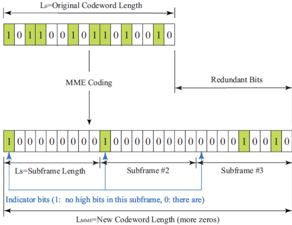
Figure 3.9. MME coding [21].
