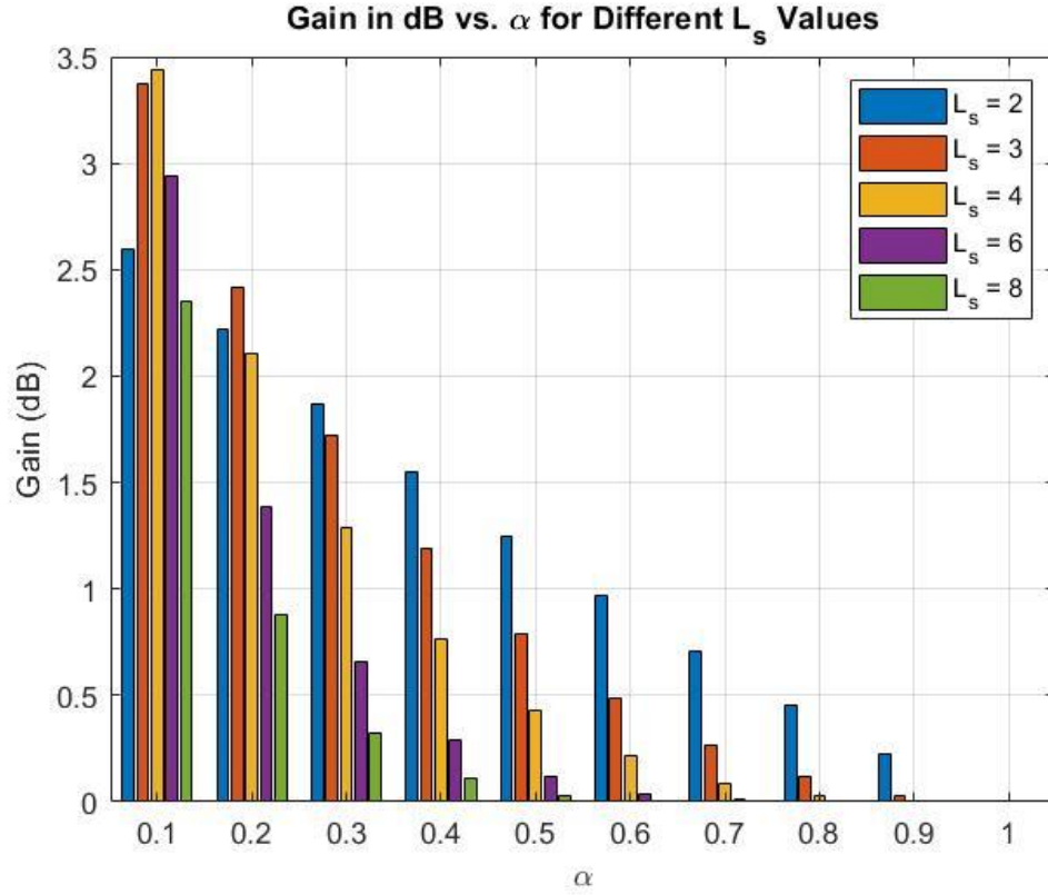
Figure 4.2. Energy gain of MME to ME coding versus the rate of high bits ( \alpha ) between 0.1 and 1.
