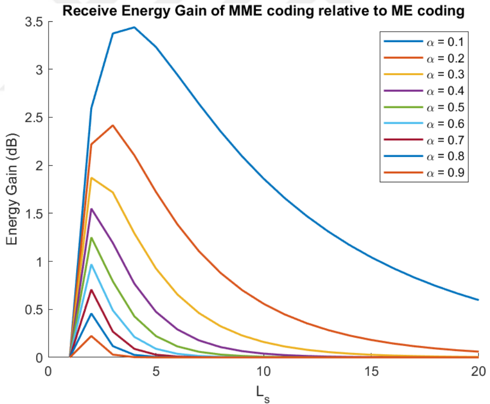
Figure 4.1. Receive energy gain of MME Coding relative to ME coding.
