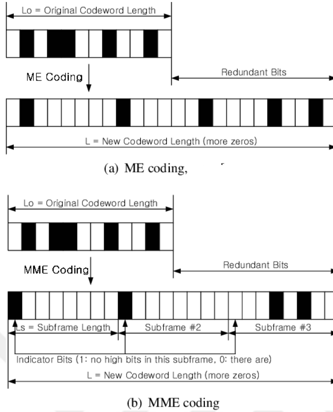
Figure 3.10. The principles of ME and MME coding schemes [13].
