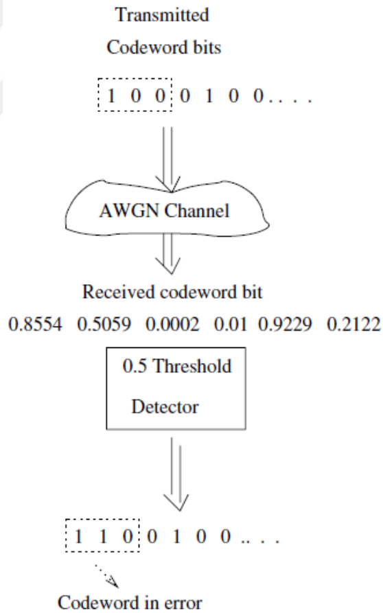
Figure 3.8. Flow of bit-by-bit detection process [11].
