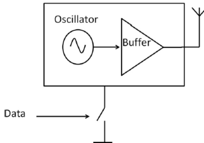
Figure 3.4. The block diagram of the OOK transmitter [12].
