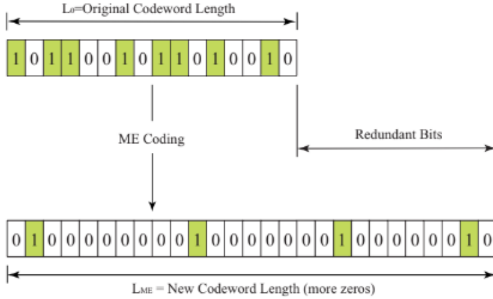
Figure 3.5. Principle of minimum energy coding [21].
