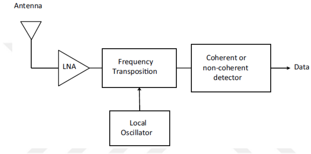
Figure 3.3. Energy consumption model of a realistic OOK Receiver [12].
