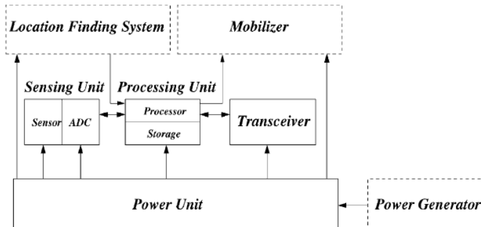
Figure 1.1. The components of a sensor node [3].
