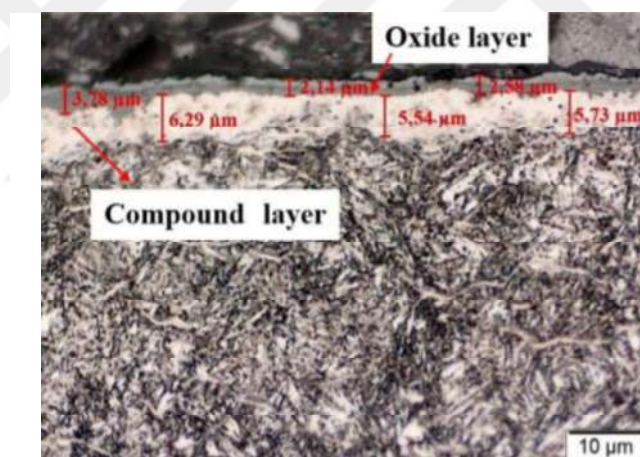
Figure 2.7 Oxidation on compound (white) layer [16]
