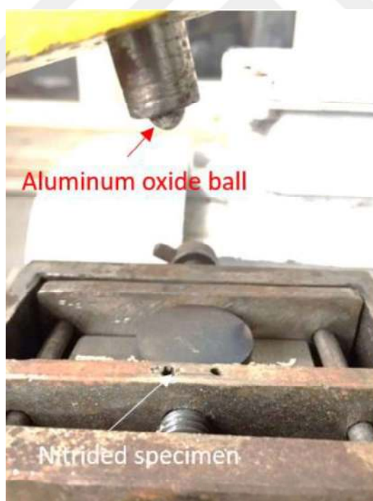
Figure 3.13 Ceramic ball and nitrided specimen
