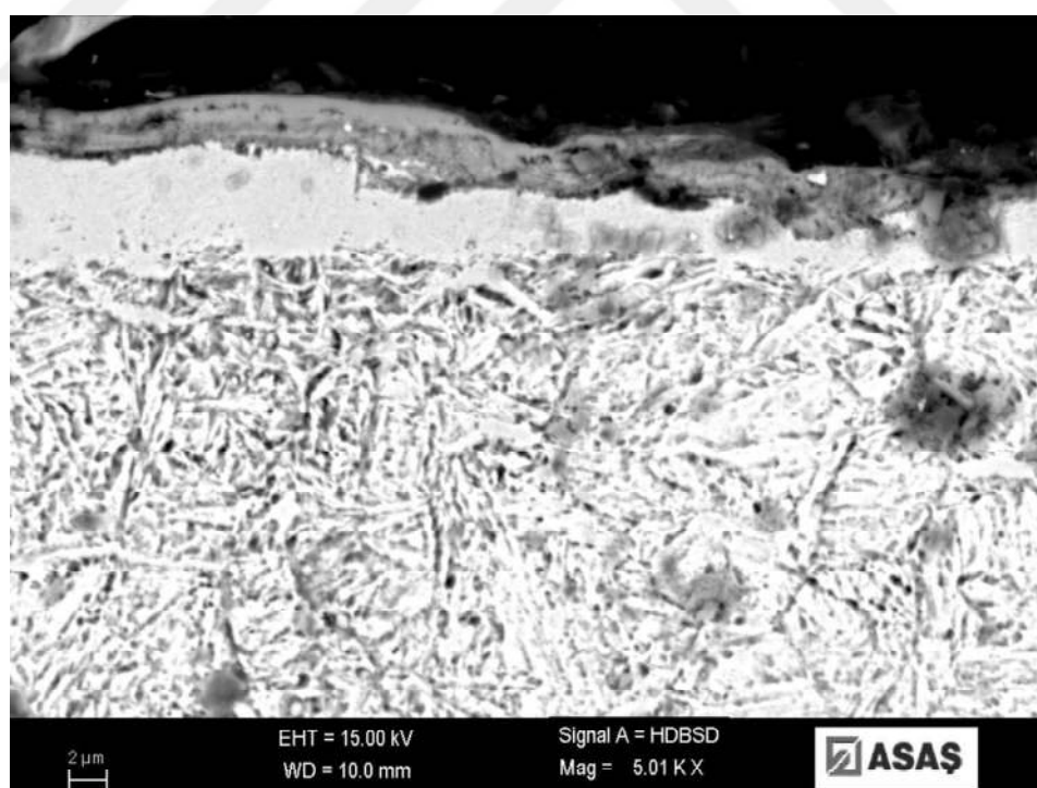
Figure 4.16 1.2344 tool steel after 12 hours of annealing on air (electron microscope) 5. KX
