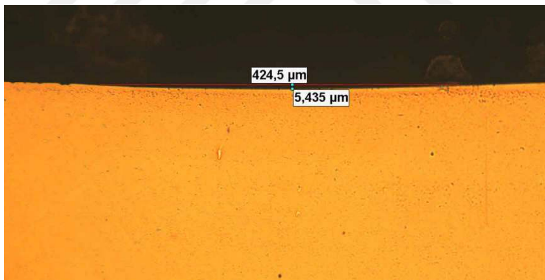
Figure 4.39 1.2344 nitrided specimen without white layer after 200 meters' abrasion test (polished)
