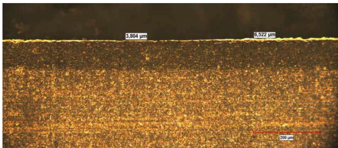
Figure 4.28 1.2344 nitrided specimen with white layer after 100 meters' abrasion (Etched)(400X) (Optical Image)
