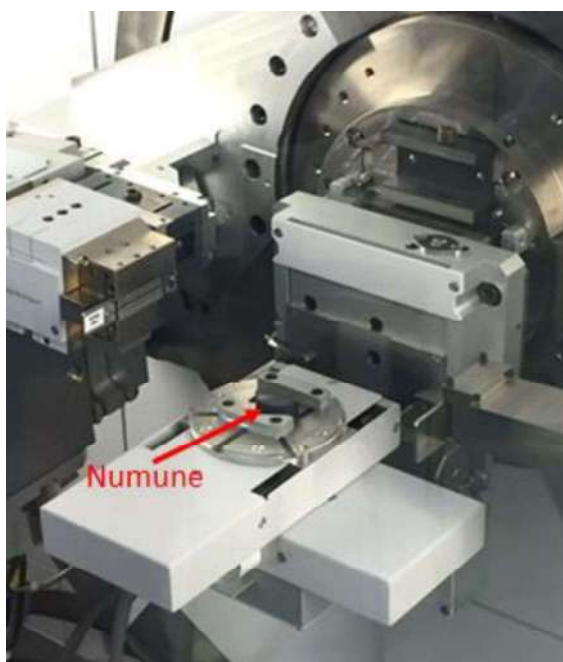
Figure 3.19 XRD method
