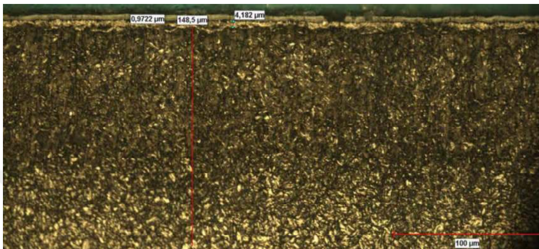
Figure 4.11 1.2344 tool steel after 40 hours annealing in air furnace by optical microscope 500x
