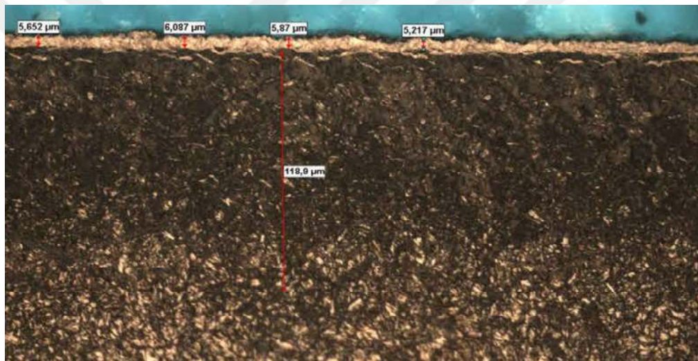
Figure 4.1 1.2344 tool steel nitriding layer before annealing(preheating) by optical microscope 500x
