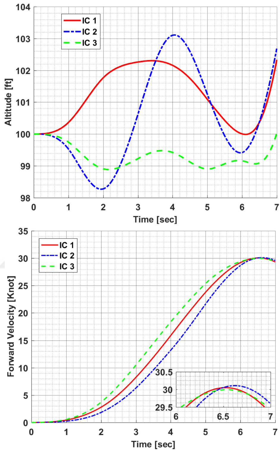
Figure 7.9: Constraint Results of Initial Condition in Hover to Forward Flight Maneuver with SR1 Method
