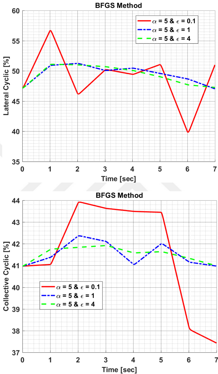
Figure 10.40: Design Variables of Hover to Rightward Flight Maneuver Optimization in Perturbation Constant Sensitivity Analysis for BFGS Method
