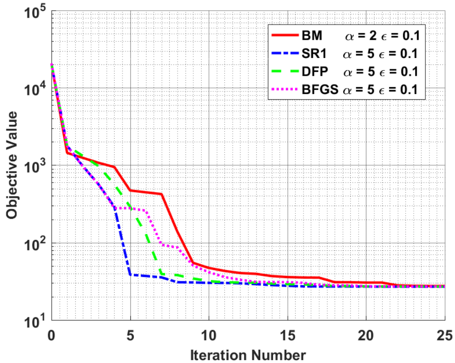
Figure 6.8: Comparison of Objective Change along Iteration Number for the selected quasi-Newton Methods in Hover to Forward Flight Maneuver
