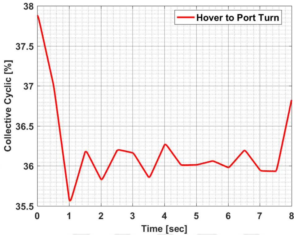
Figure 8.13: Obtained Design Variable for Hover to Port Turn Maneuver with SR1 Method
