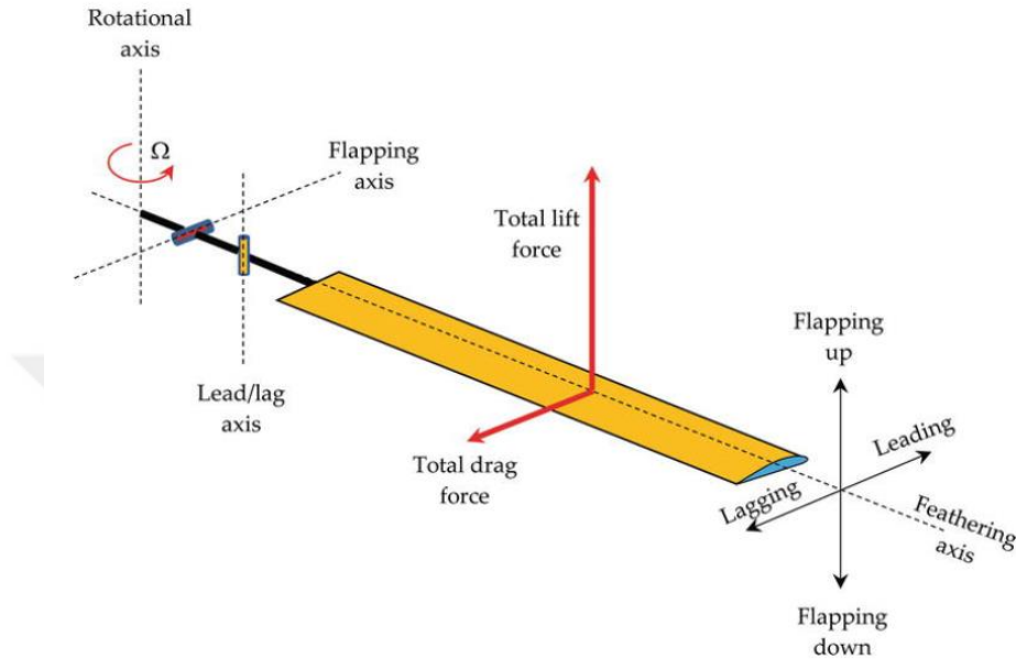
Figure 4.2: Three Main Motions of the Rotor Blade [55]
