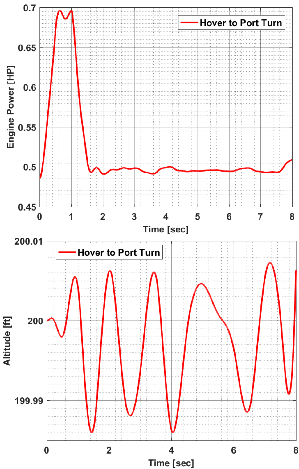
Figure 8.11: Constraint Results for Hover to Port Turn Maneuver with SR1 Method
