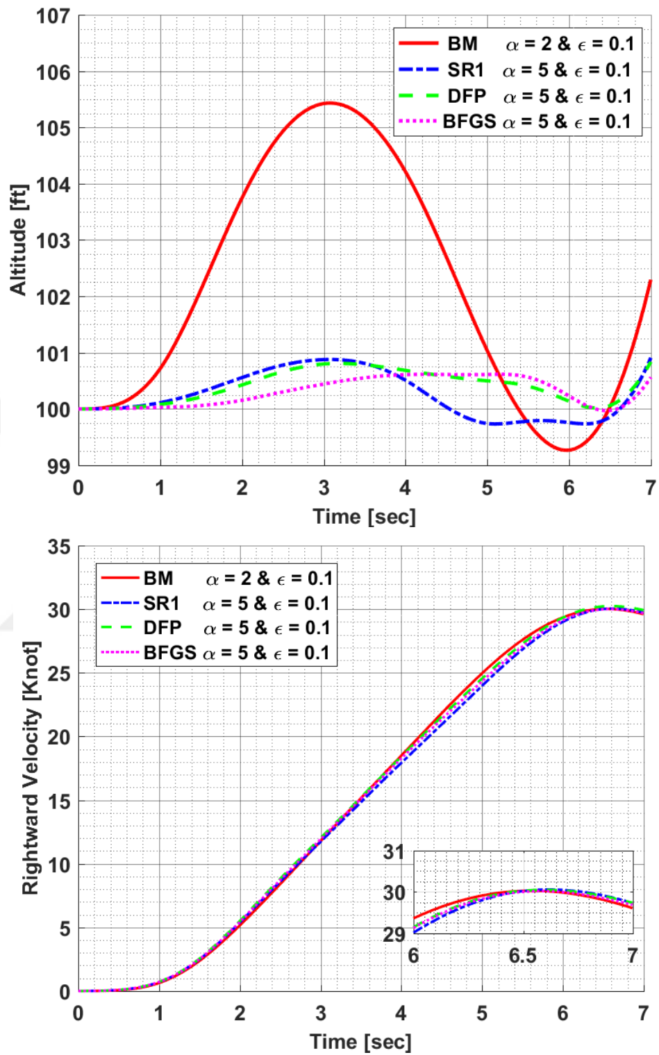
Figure 6.19: Constraint Results of Hover to Rightward Flight Maneuver in Optimization Methods
