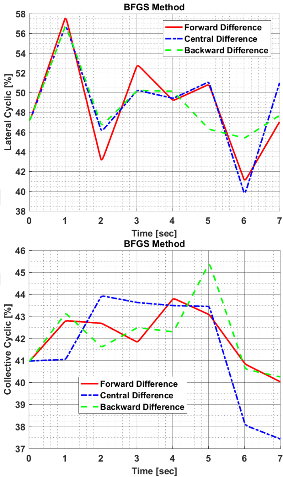
Figure 10.32: Design Variables of Hover to Rightward Flight Maneuver Optimization in Finite Divided Difference Approximation Comparison for BFGS
