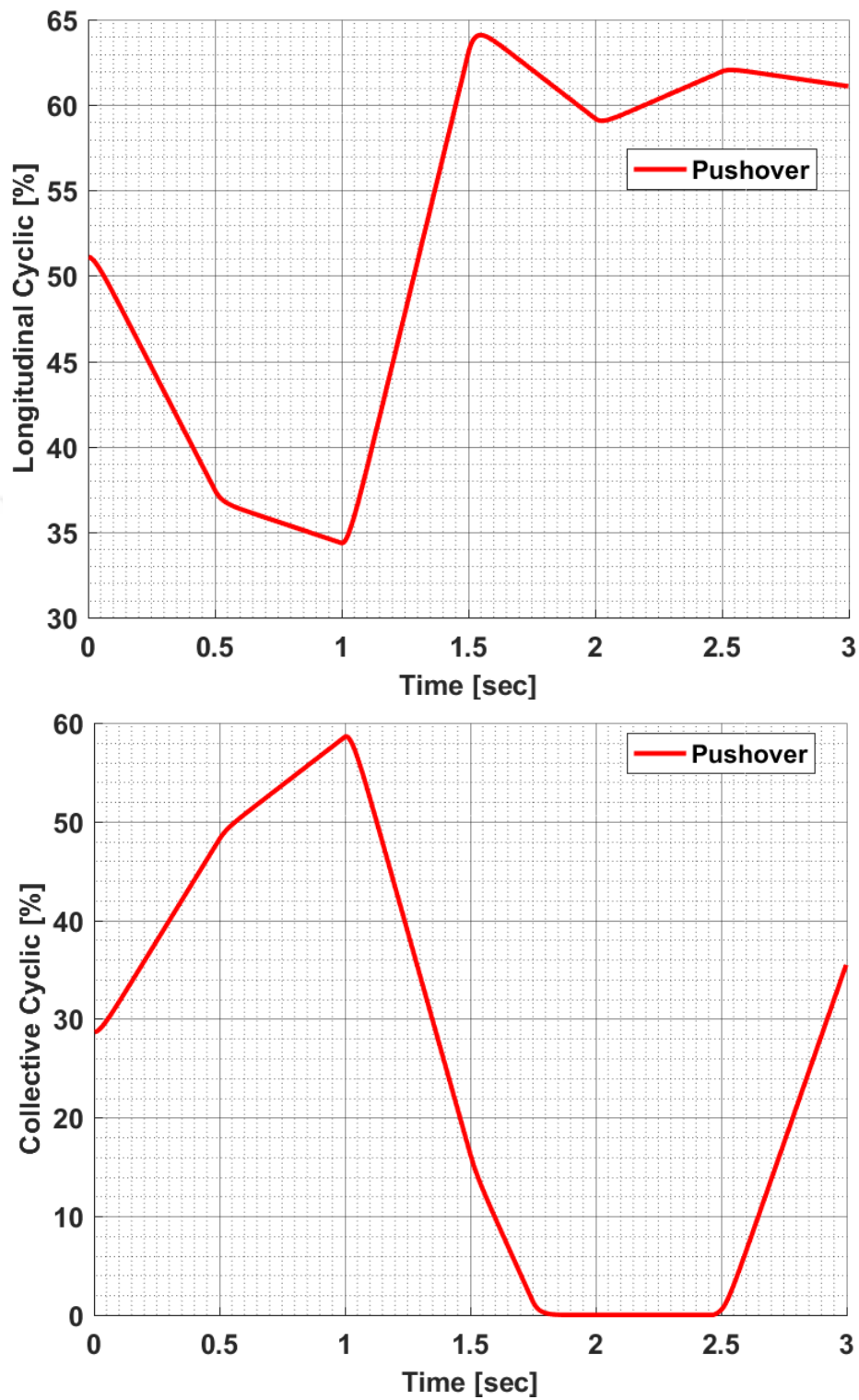
Figure 8.9: Obtained Design Variable for Pushover Maneuver with SR1 Method
