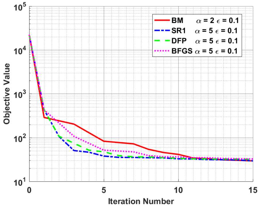
Figure 6.18: Comparison of Objective Change along Iteration Number for the selected quasi-Newton Methods in Hover to Forward Flight Maneuver
