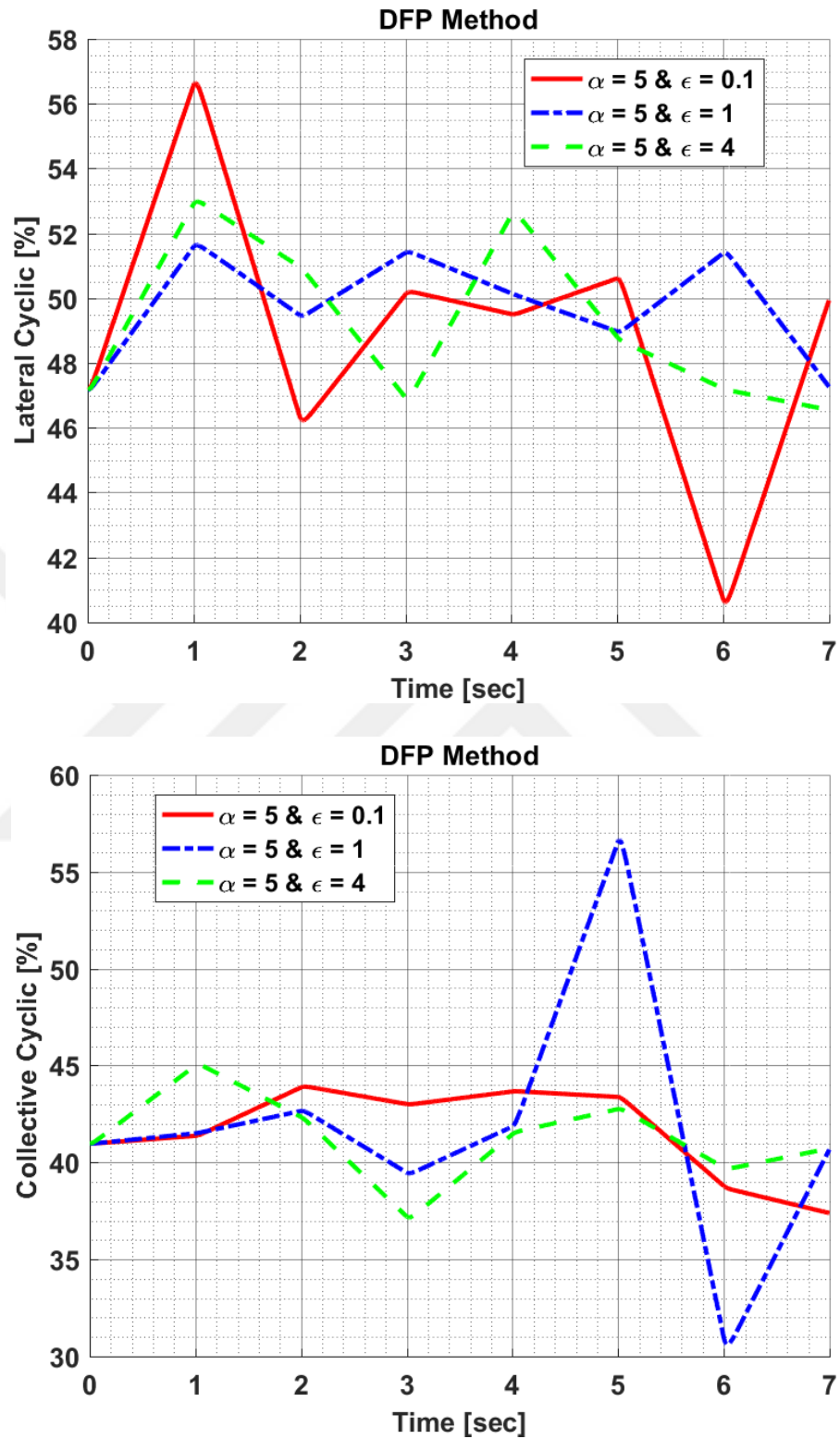
Figure 10.38: Design Variables of Hover to Rightward Flight Maneuver Optimization in Perturbation Constant Sensitivity Analysis for DFP Method
