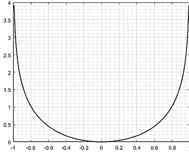
Figure 5.2: Representation of the Logarithmic Barrier Function
